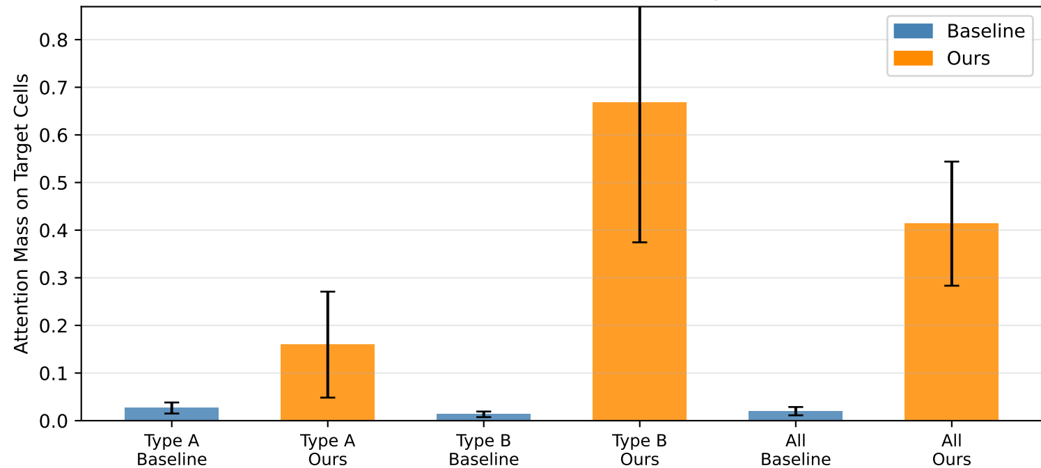
Attention Mass on Ground-Truth Target Cells
