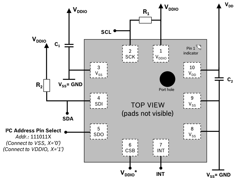
Figure 25: I 2 C connection diagram (Pin1 marking indicated)
