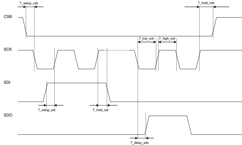
Figure 22: SPI timing diagram
