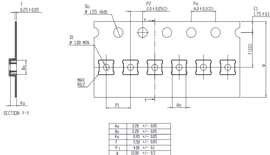
Figure 28: Tape and Reel dimensions
