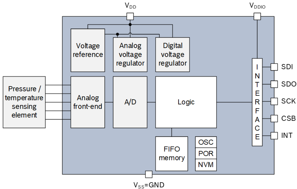
Figure 1: Block Diagram BMP388
