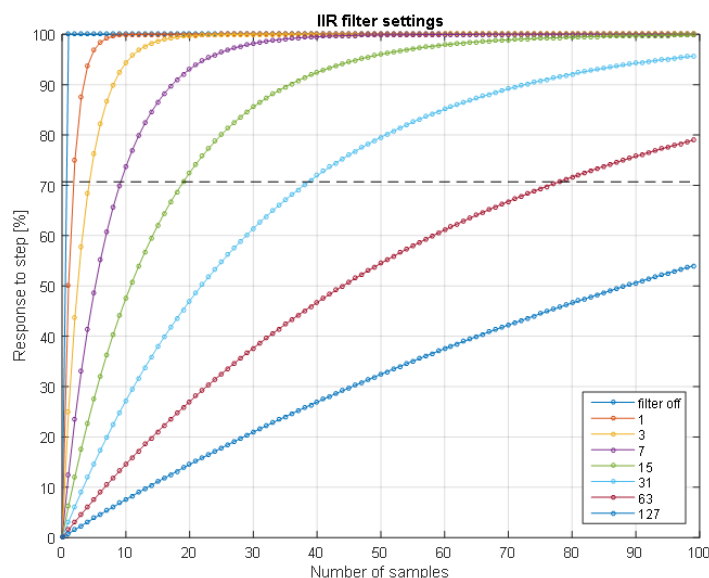
Figure 6: Step response at different IIR filter settings
