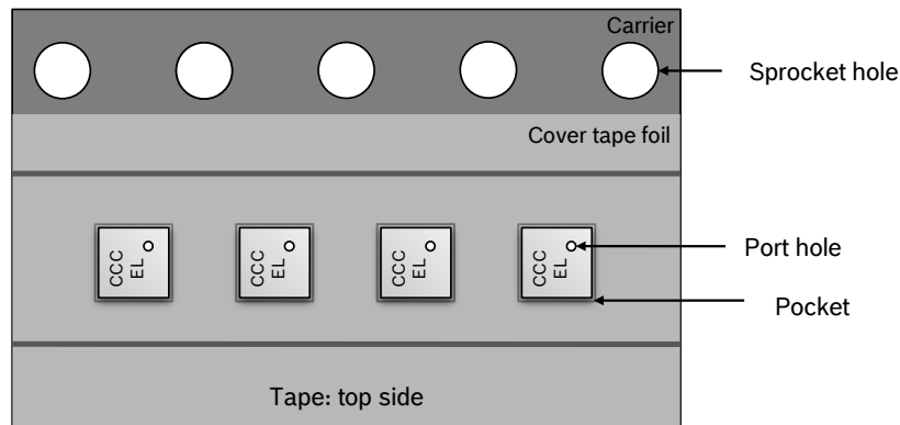
Figure 29: Orientation within tape
