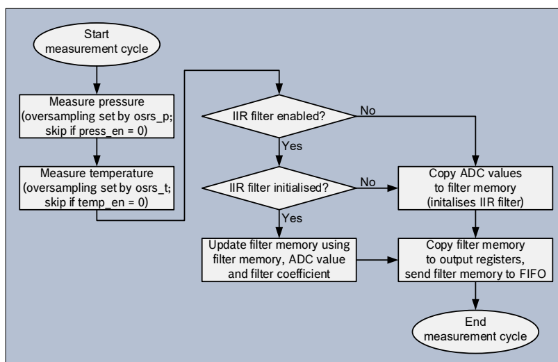
Figure 5: BMP388 measurement cycle
