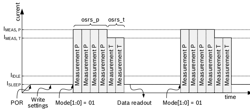
Figure 2: Force mode timing diagram
