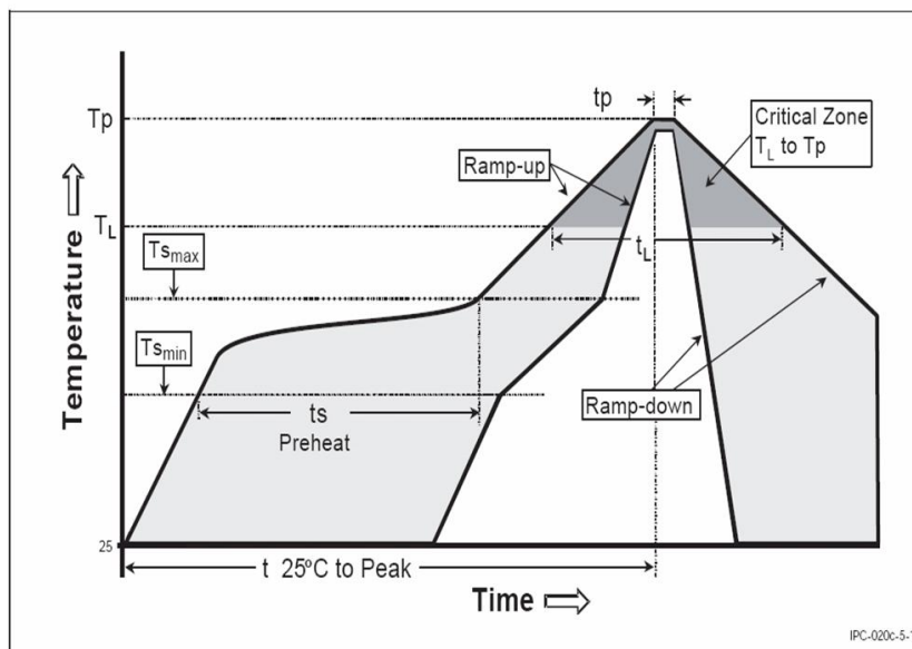
Figure 27: Soldering profile
