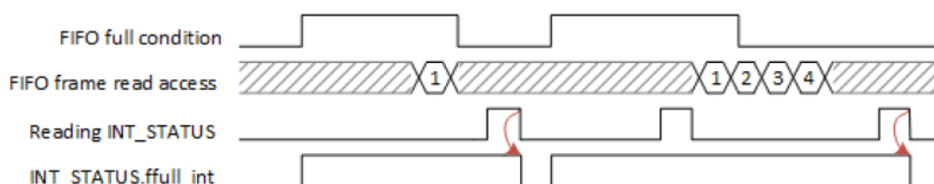
Figure 10: FIFO full interrupt, latched, with reads from FIFO
