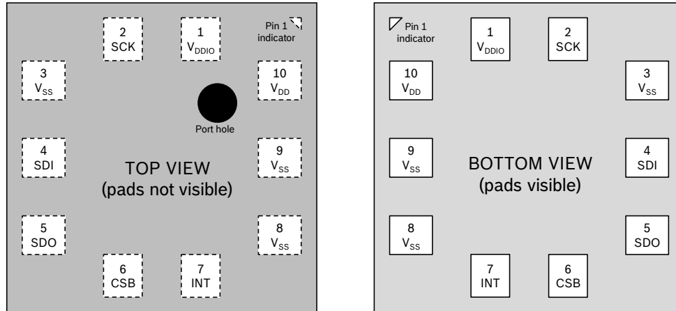
Figure 23: Pin-out top and bottom view
