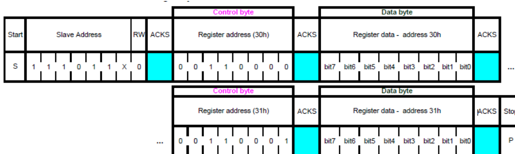
Figure 15: I 2 C write
