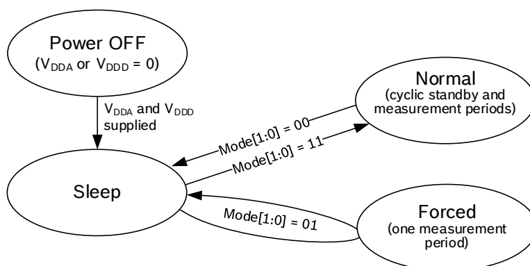
Figure 4: Mode transition diagram
