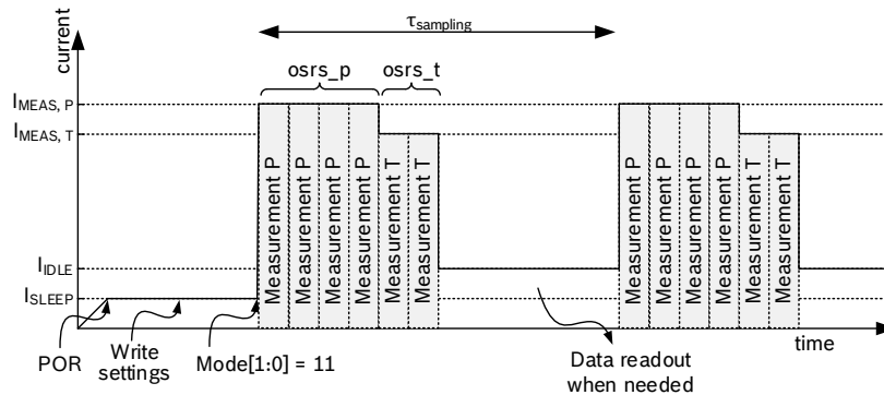
Figure 3: Normal mode timing diagram
