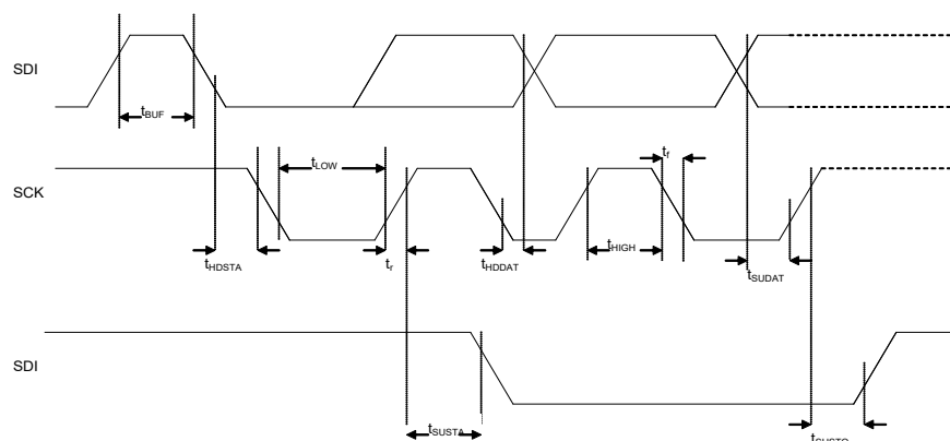
Figure 21: I²C timing diagram
