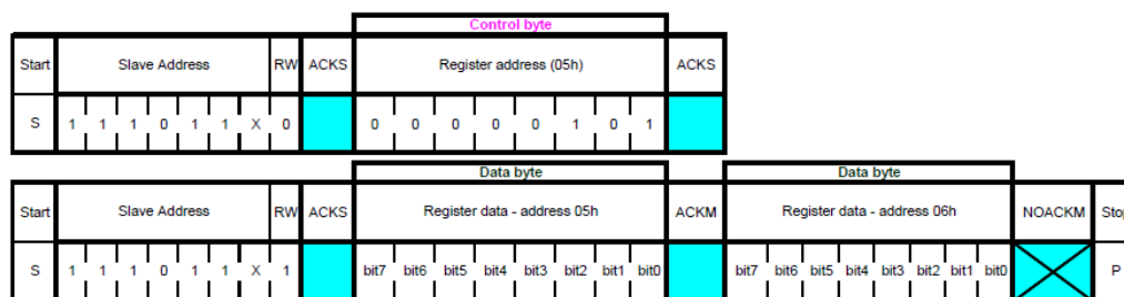
Figure 16: I 2 C multiple byte read
