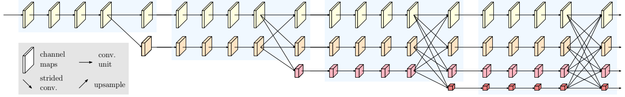
Fig. 13. Illustrating the HRNet architecture. It consists of parallel high-to-low resolution convolution streams with repeated information exchange across multi-resolution streams. There are four stages. The 1st stage consists of high-resolution convolutions. The 2nd (3rd, 4th) stage repeats two-resolution (three-resolution, four-resolution) blocks. From [44].
