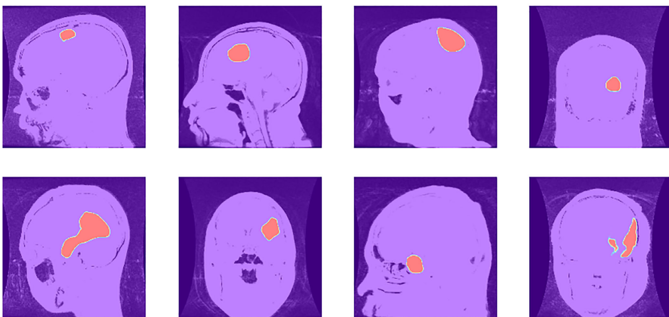
(b) Predicted
