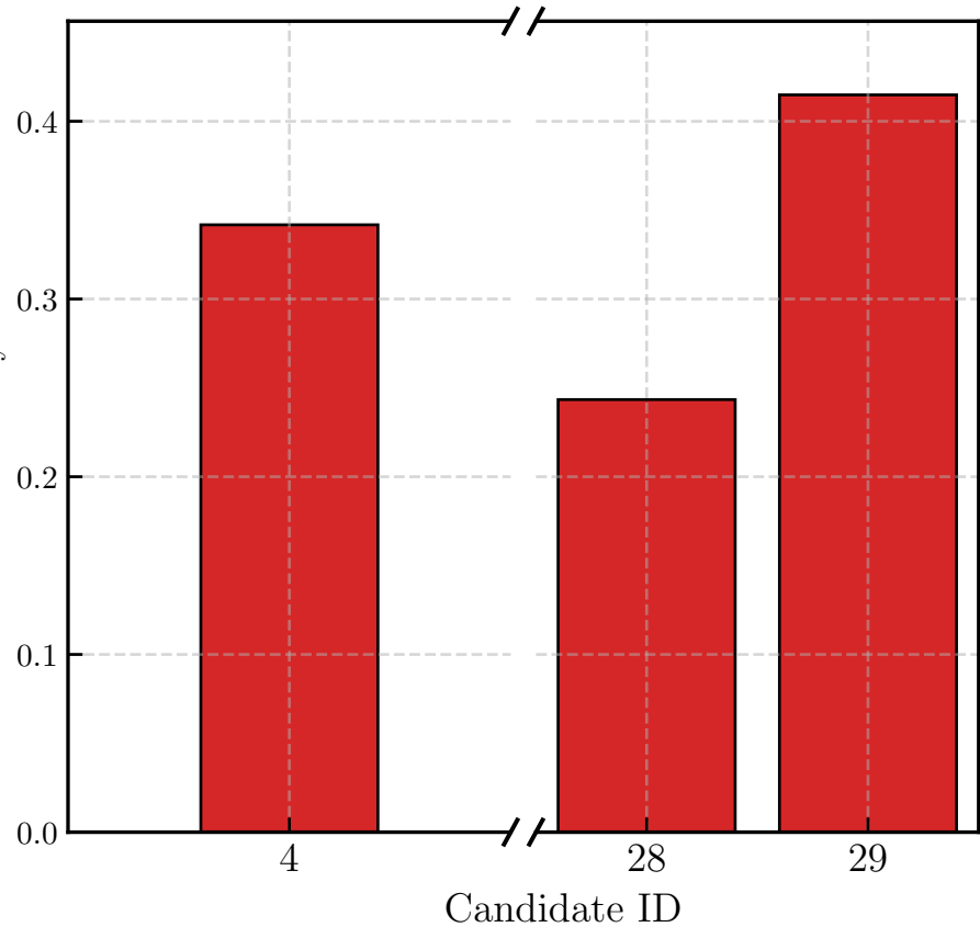
Probability
