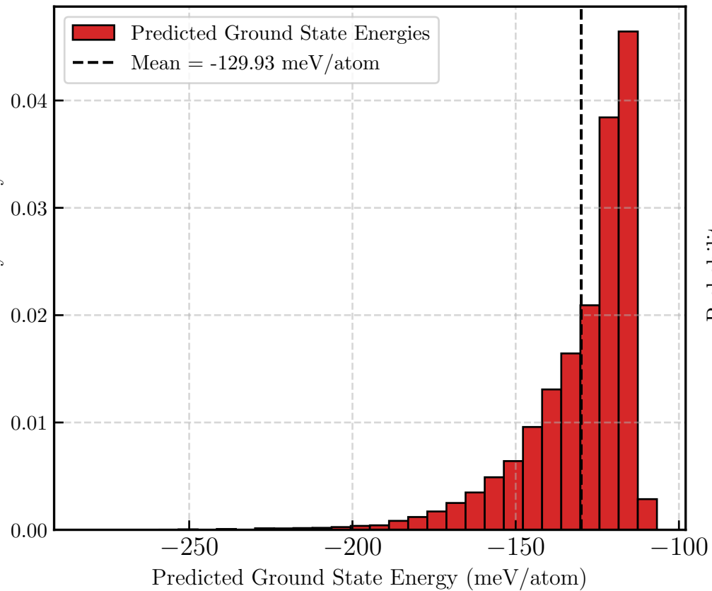
Probability Density
