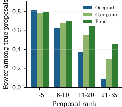
(c) Rank profile, SR = 1.5
