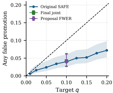
(a) Sign-null calibration
