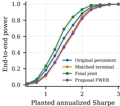
(b) Paired power, \rho = .5
