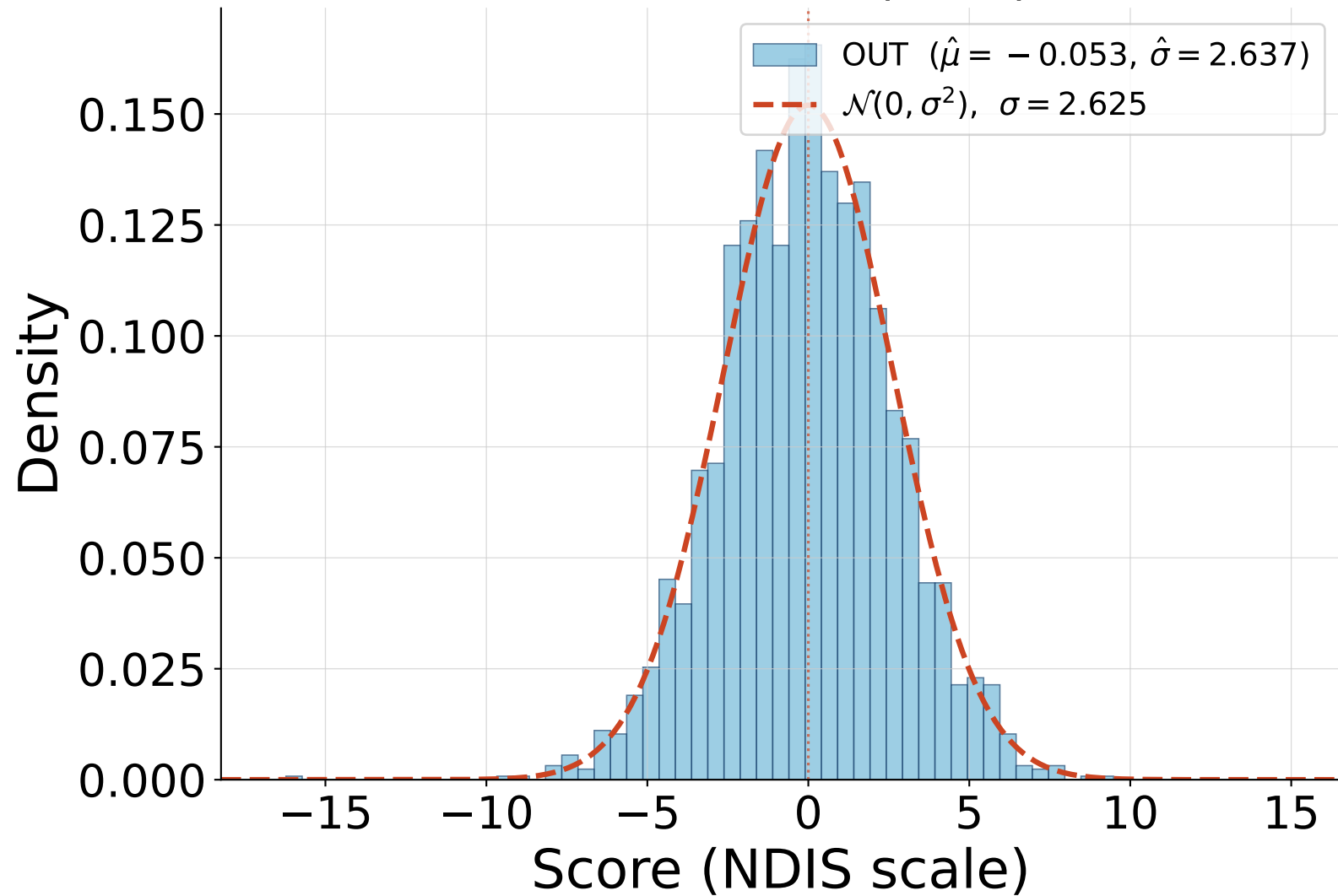
DP-SGD OUT ( \varepsilon = 8 )
