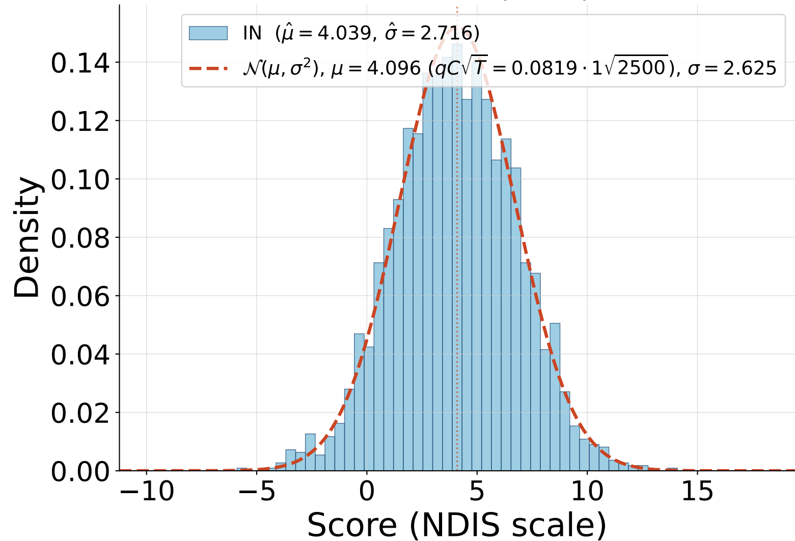
DP-SGD IN ( \varepsilon = 8 )
