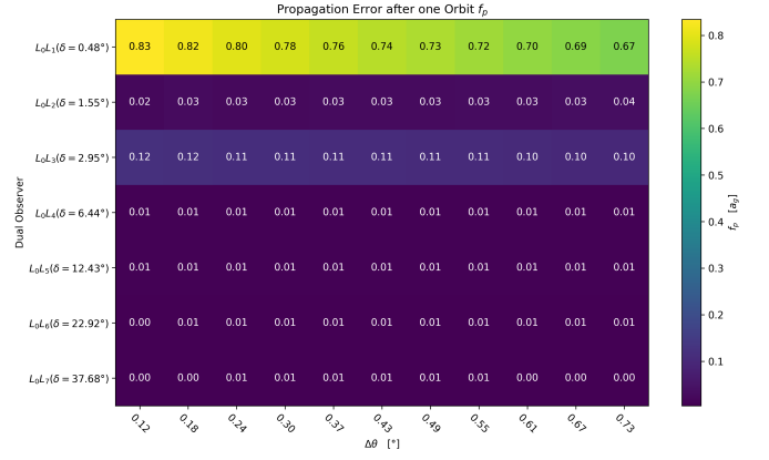
Figure 16: Stereo vision (circular model): Propagation error after one orbit.
