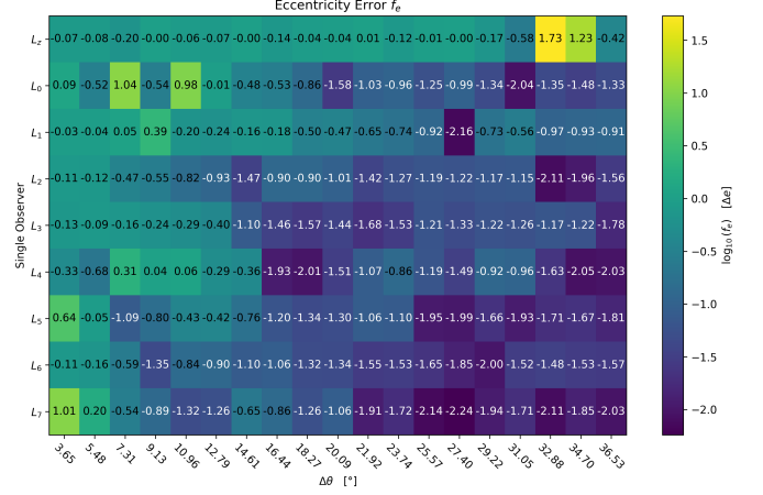
Figure 4: Gaussian method: Stability of eccentricity.
