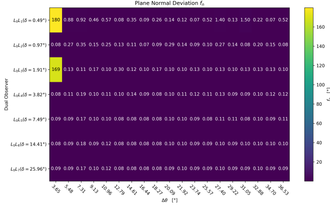
Figure 9: Stereo vision (full parametric model): Plane normal deviation.
