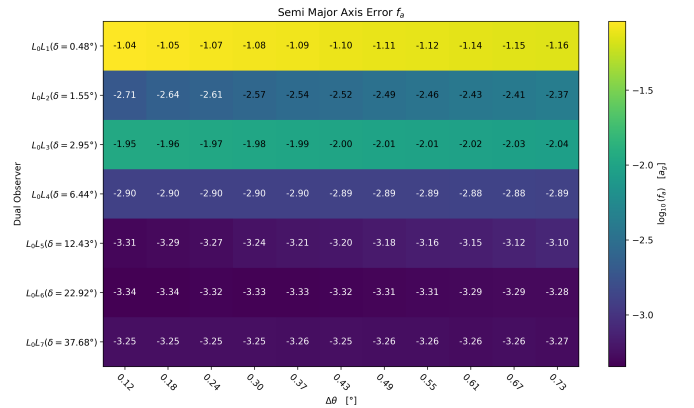
Figure 14: Stereo vision (circular model): Stability of semi major axis.
