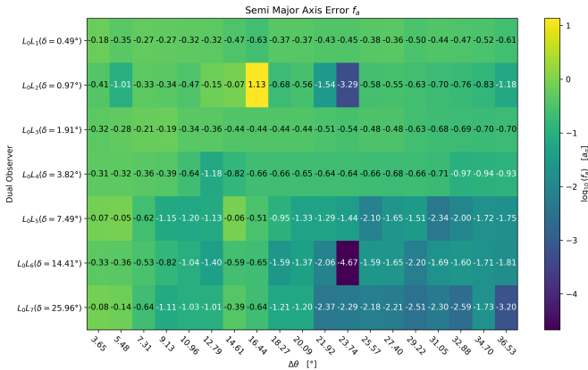
Figure 7: Stereo vision (full parametric model): Stability of semi major axis.
