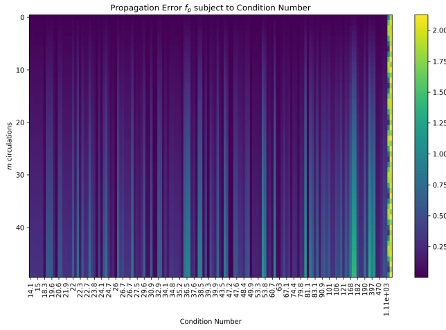
Figure 17: Simplified Gaussian method: Propagation error after m orbits subject to calibration condition number.
