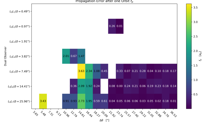
Figure 10: Stereo vision (full parametric model): Propagation error after one orbit.
