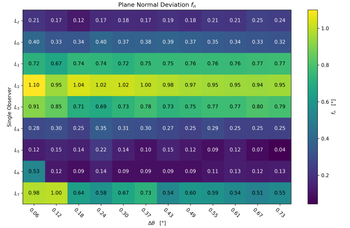
Figure 12: Simplified Gaussian method: Plane normal deviation.
