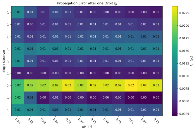
Figure 13: Simplified Gaussian method: Propagation error after one orbit.
