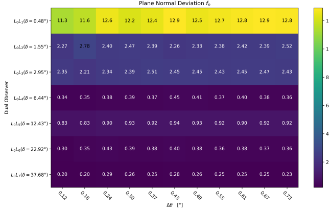
Figure 15: Stereo vision (circular model): Plane normal deviation.
