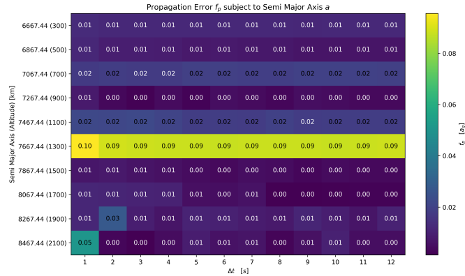
Figure 19: Simplified Gaussian method: Propagation error subject to orbital altitude.
