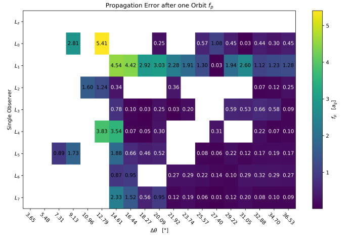
Figure 6: Gaussian method: Propagation error after one orbit.
