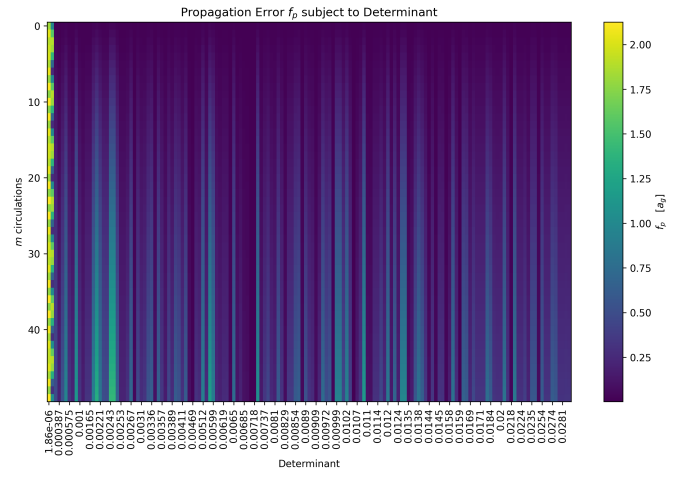
Figure 18: Simplified Gaussian method: Propagation error after m orbits subject to calibration determinant.
