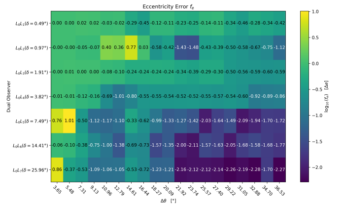
Figure 8: Stereo vision (full parametric model): Stability of eccentricity.
