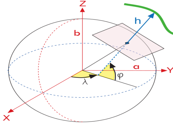
Figure 6: Cartesian and ellipsoidal coordinates on planet earth. [8]
