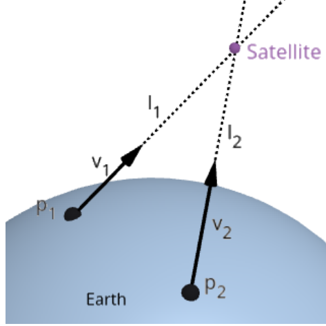
Figure 13: The parametric trajectory in the three dimensional ECI coordinate system.
