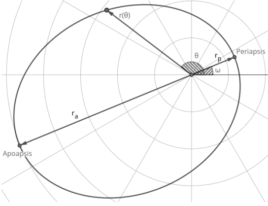
Figure 1: Parametric curve of an elliptic orbit.
