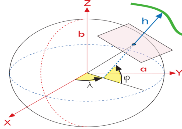
Figure 6: Cartesian and ellipsoidal coordinates on planet earth. [8]
