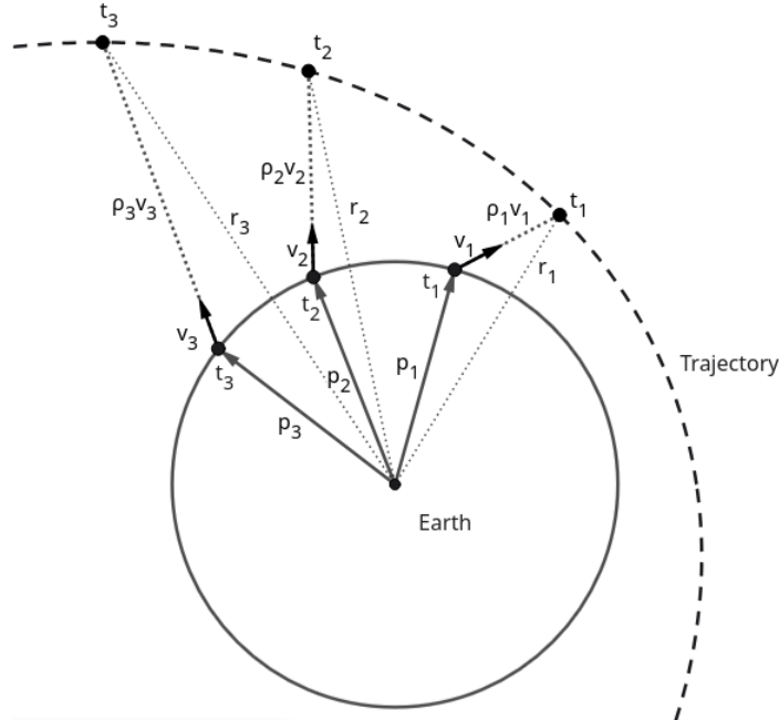
Figure 14: Initially known and unknown properties of Gaussian orbit determination depicted in a two dimensional representation.
