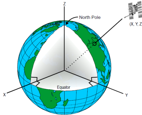
Figure 3: Earth Centered Inertial coordinate system aligned to planet earth. [6]
