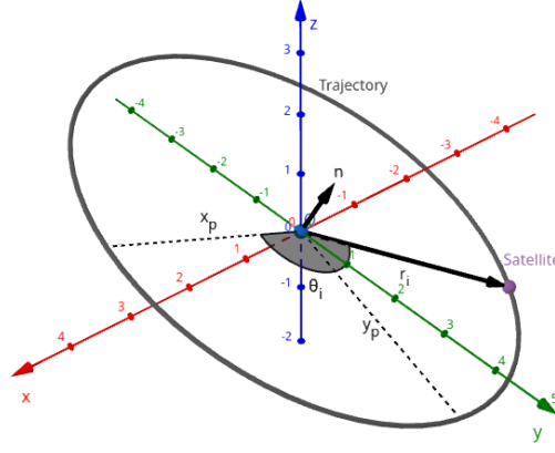
Figure 12: The parametric trajectory in the three dimensional ECI coordinate system.
