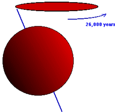
Figure 11: Tumbling movement of earth's rotation axis [12].
