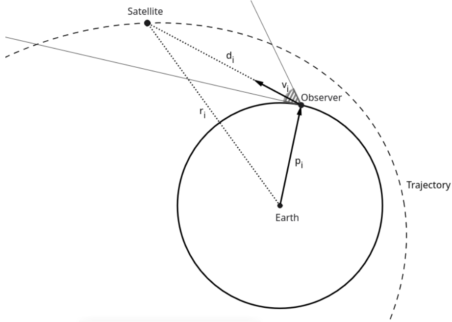
Figure 4: Initially known and unknown properties of earth bound camera based satellite observation depicted in a two dimensional representation.
