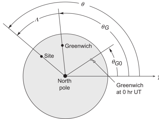
Figure 7: Geometric context of ECI longitude subject to time. [9]
