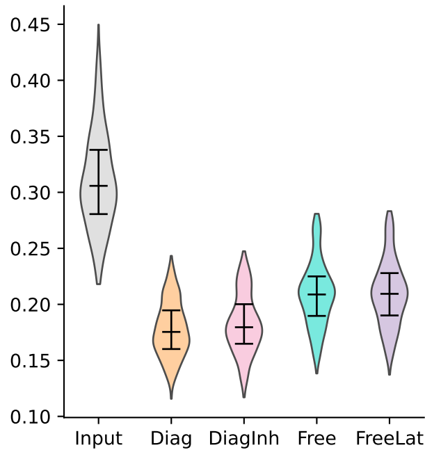
odours inclclass
