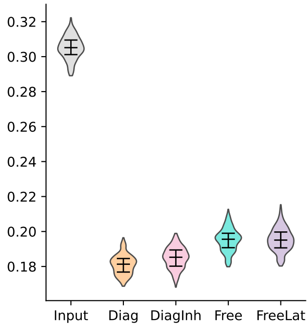
trials random
