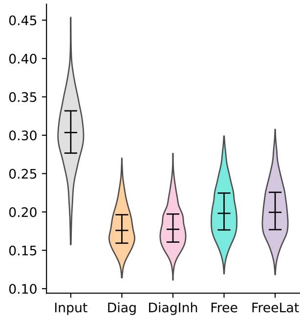
odours outclass
