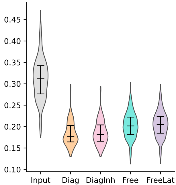
odours random
