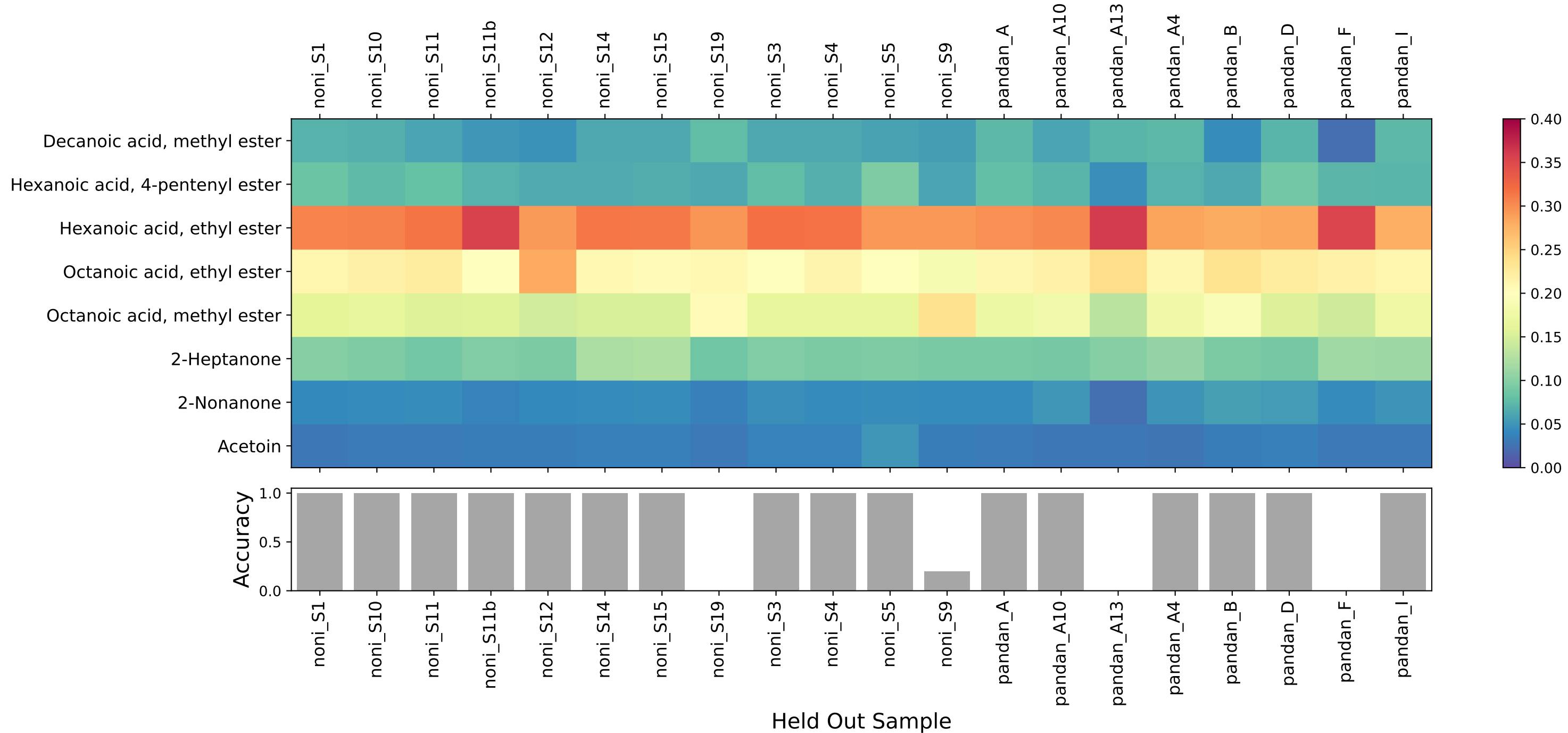
Random Forest Feature (Odour) Importances (colours) and Accuracy (gray)
