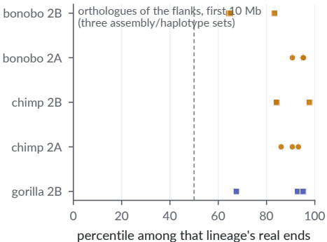
a Substitution end-strength
