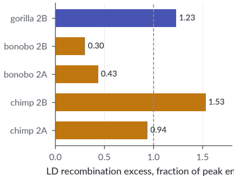
b Recombination today at the orthologues
