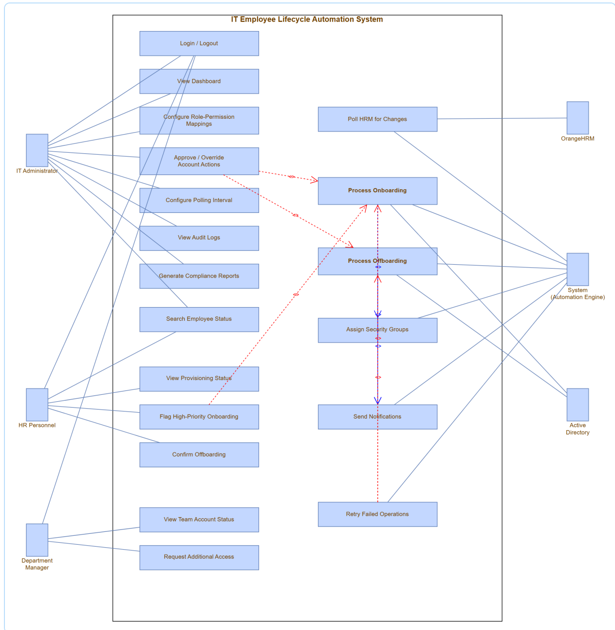
Figure: Use Case Diagram — all actors and use cases for the IT Employee Lifecycle Automation System
