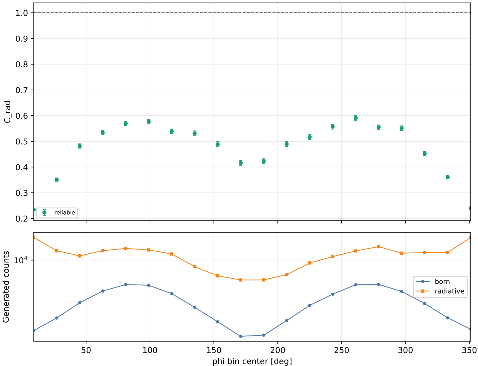
Radiative correction vs phi Q2 2.5-3, xB 0.38-0.48, -t 1-1.5
