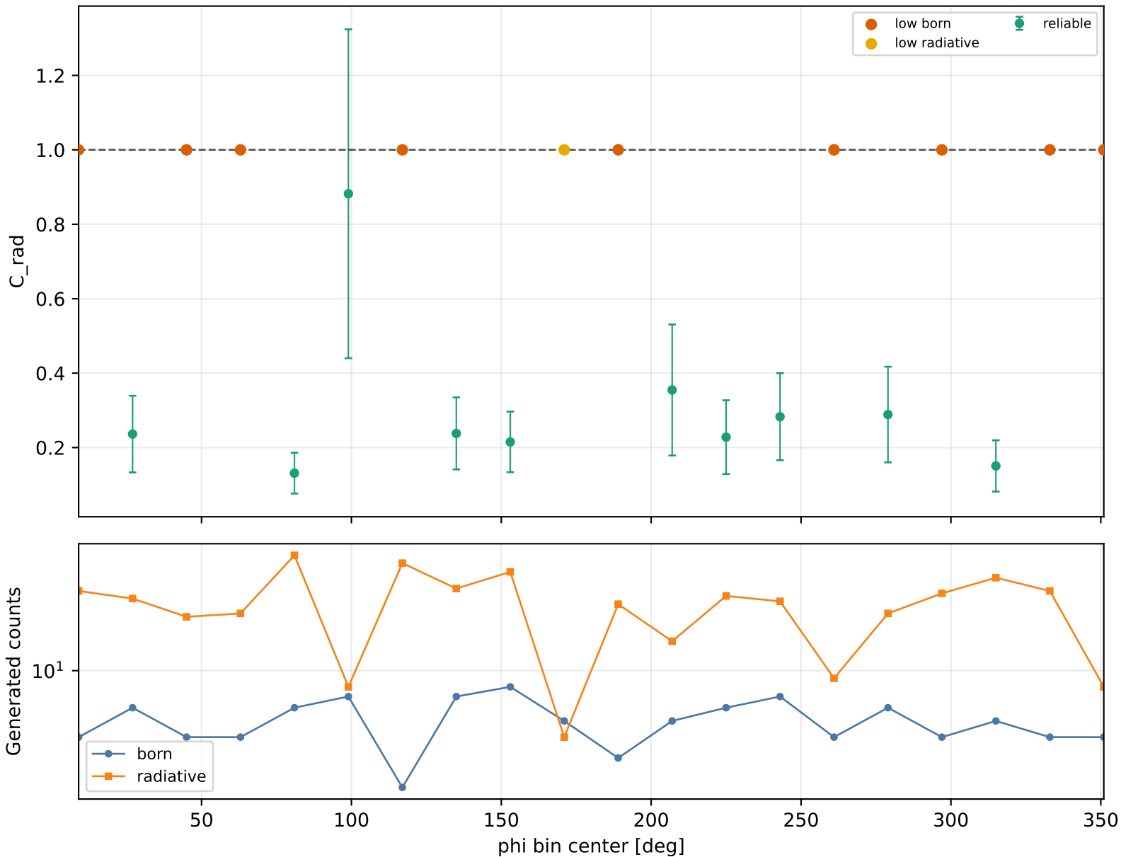
Radiative correction vs phi Q2 2.5-3, xB 0.2-0.25, -t 1-1.5
