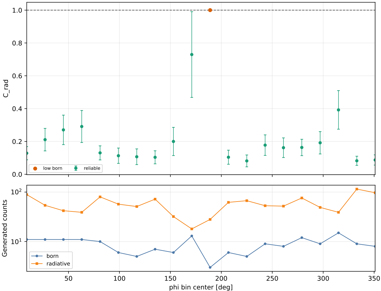
Radiative correction vs phi Q2 1-1.5, xB 0.05-0.1, -t 0.6-1
