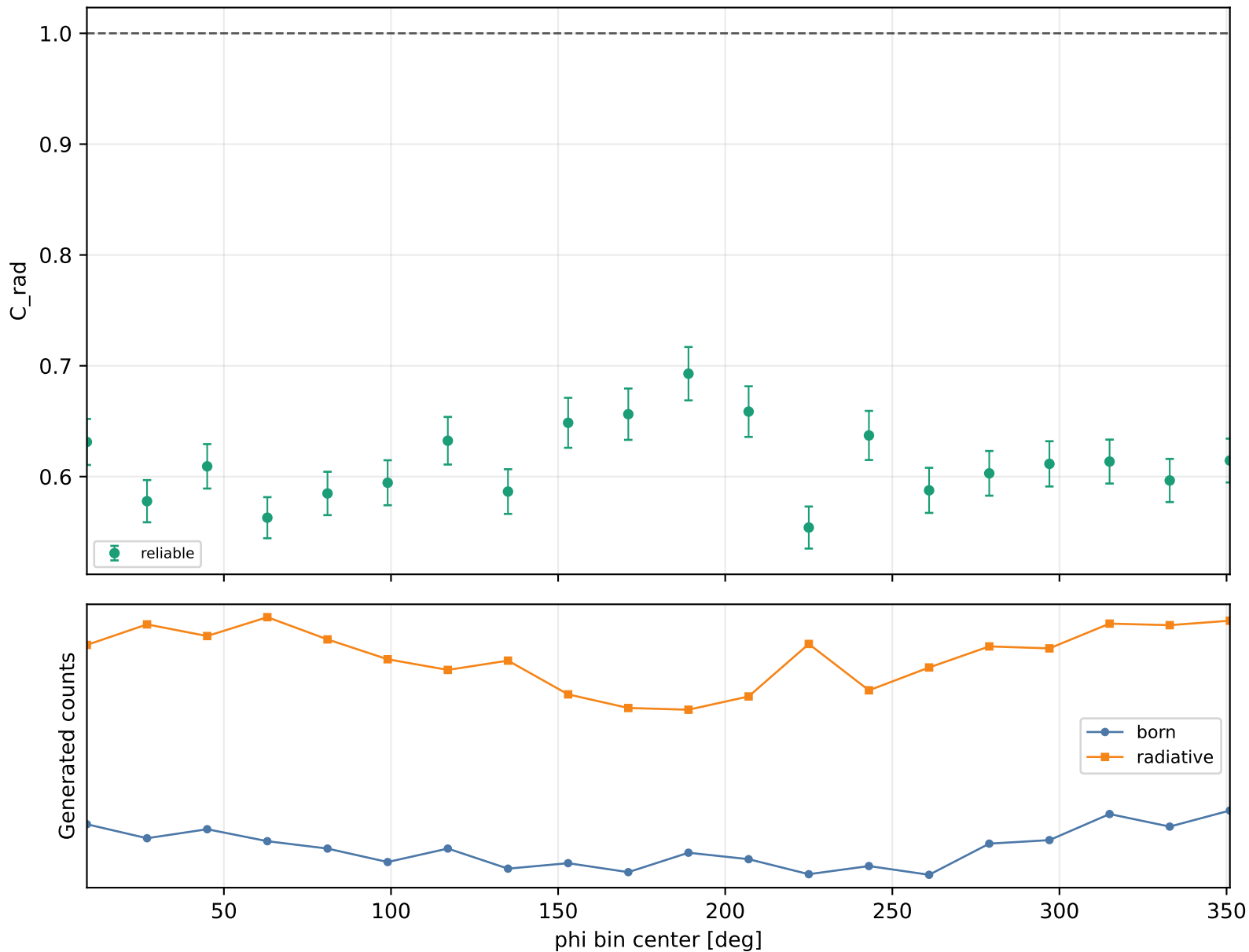
Radiative correction vs phi Q2 3-3.5, xB 0.58-0.7, -t 0.6-1
