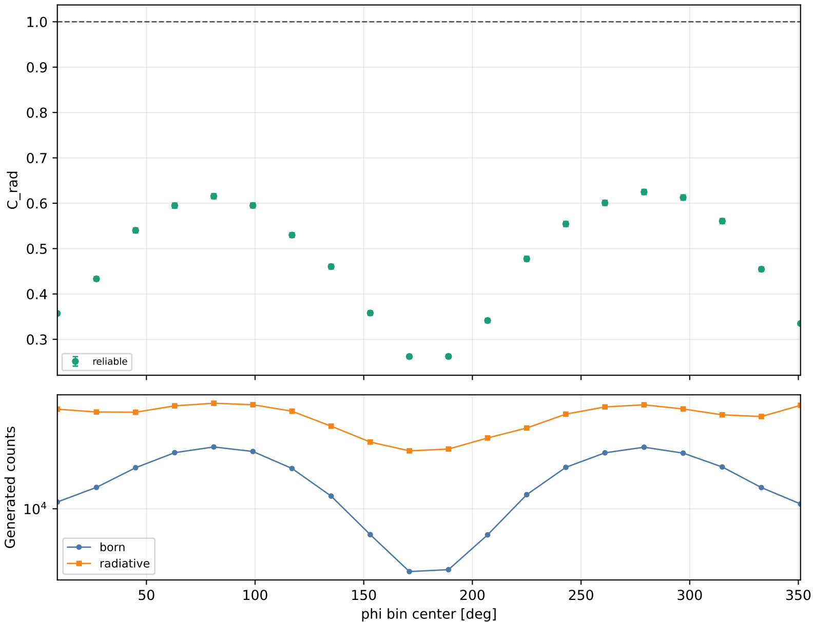
Radiative correction vs phi Q2 1-1.5, xB 0.15-0.2, -t 0.3-0.4
