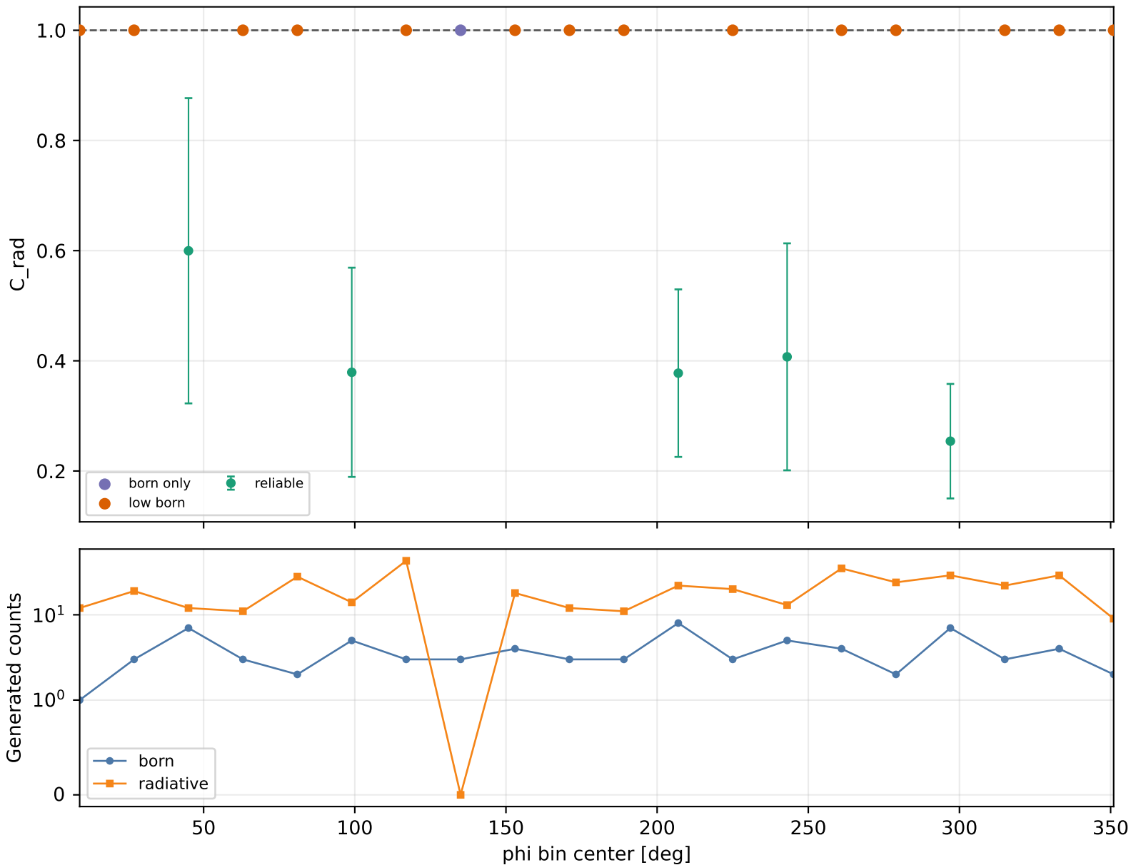
Radiative correction vs phi Q2 2.5-3, xB 0.2-0.25, -t 0.09-0.15
