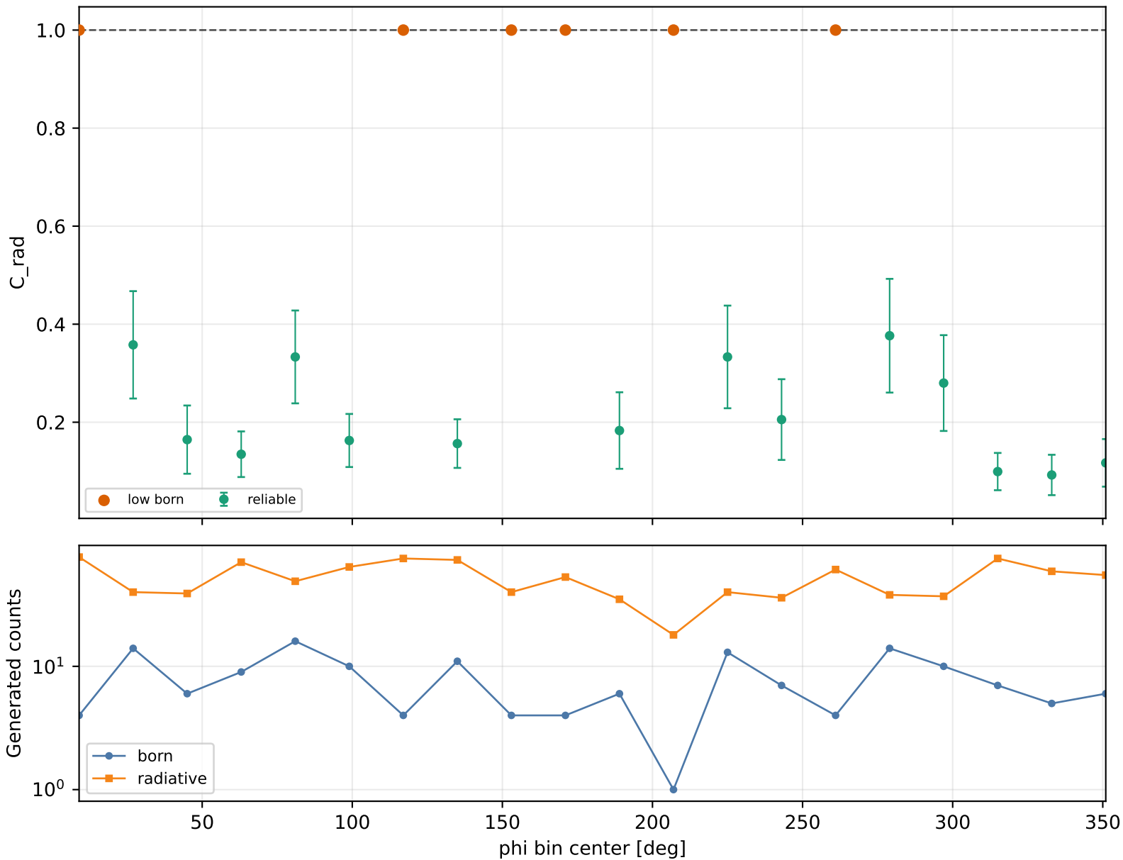
Radiative correction vs phi Q2 2.5-3, xB 0.2-0.25, -t 0.4-0.6
