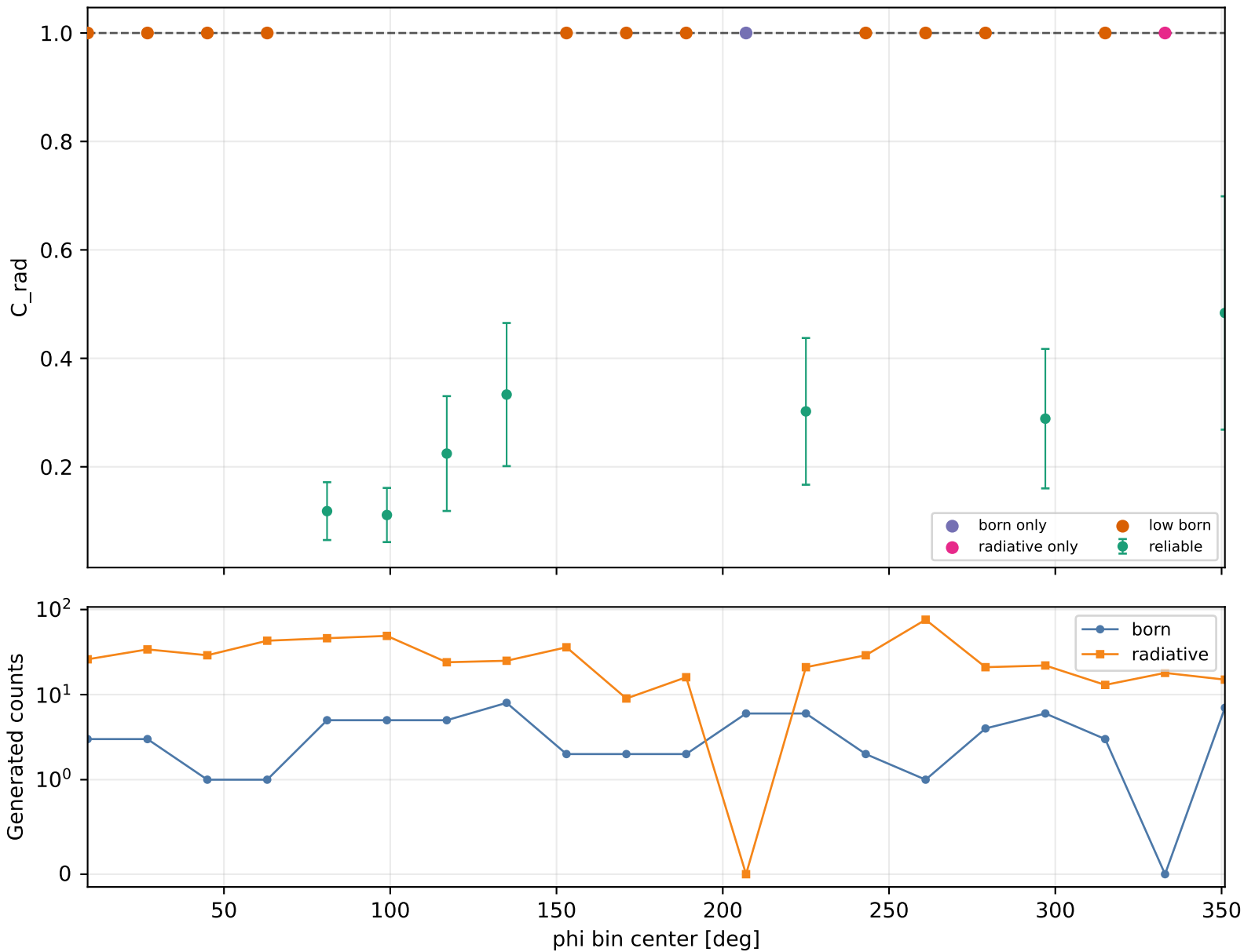
Radiative correction vs phi Q2 3-3.5, xB 0.25-0.3, -t 0.3-0.4
