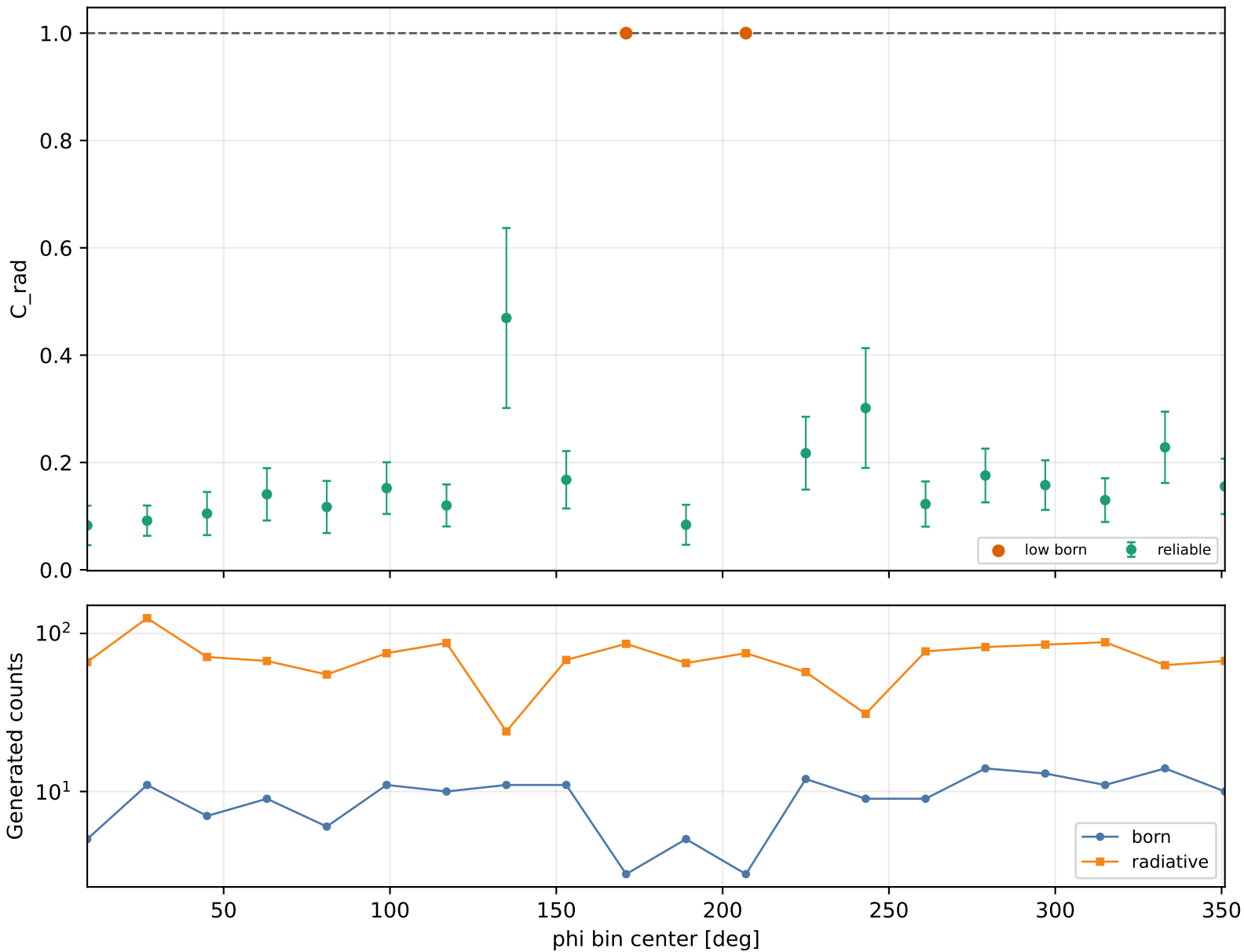
Radiative correction vs phi Q2 1-1.5, xB 0.05-0.1, -t 0.09-0.15
