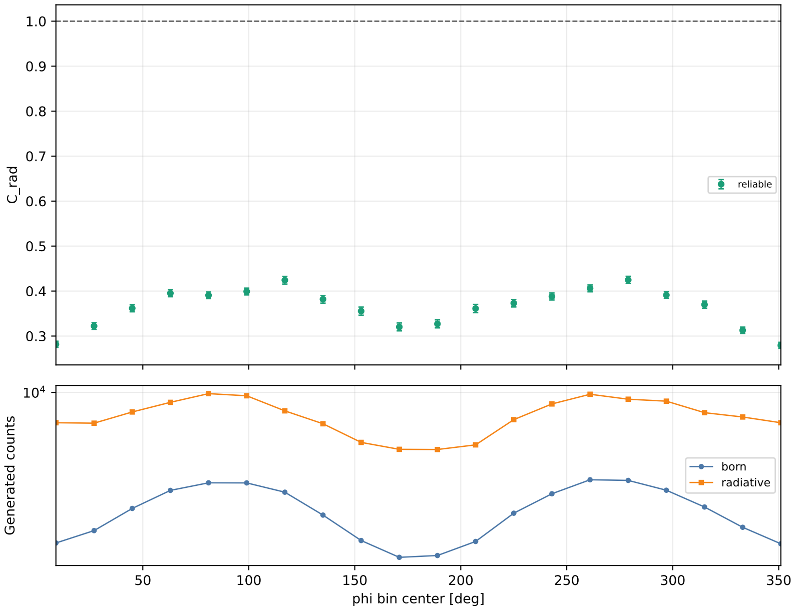
Radiative correction vs phi Q2 3-3.5, xB 0.48-0.58, -t 1-1.5
