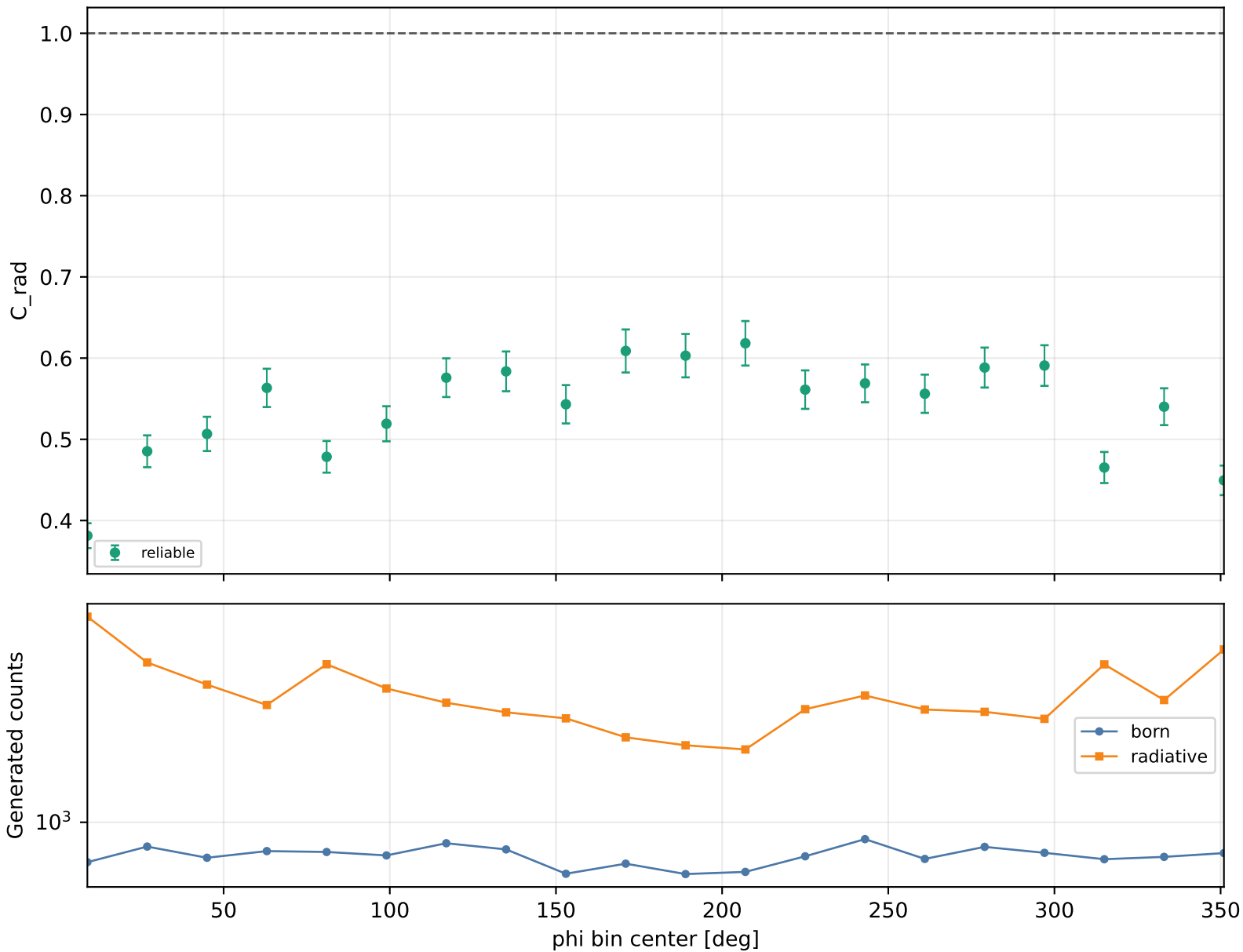
Radiative correction vs phi Q2 2-2.5, xB 0.2-0.25, -t 1-1.5
