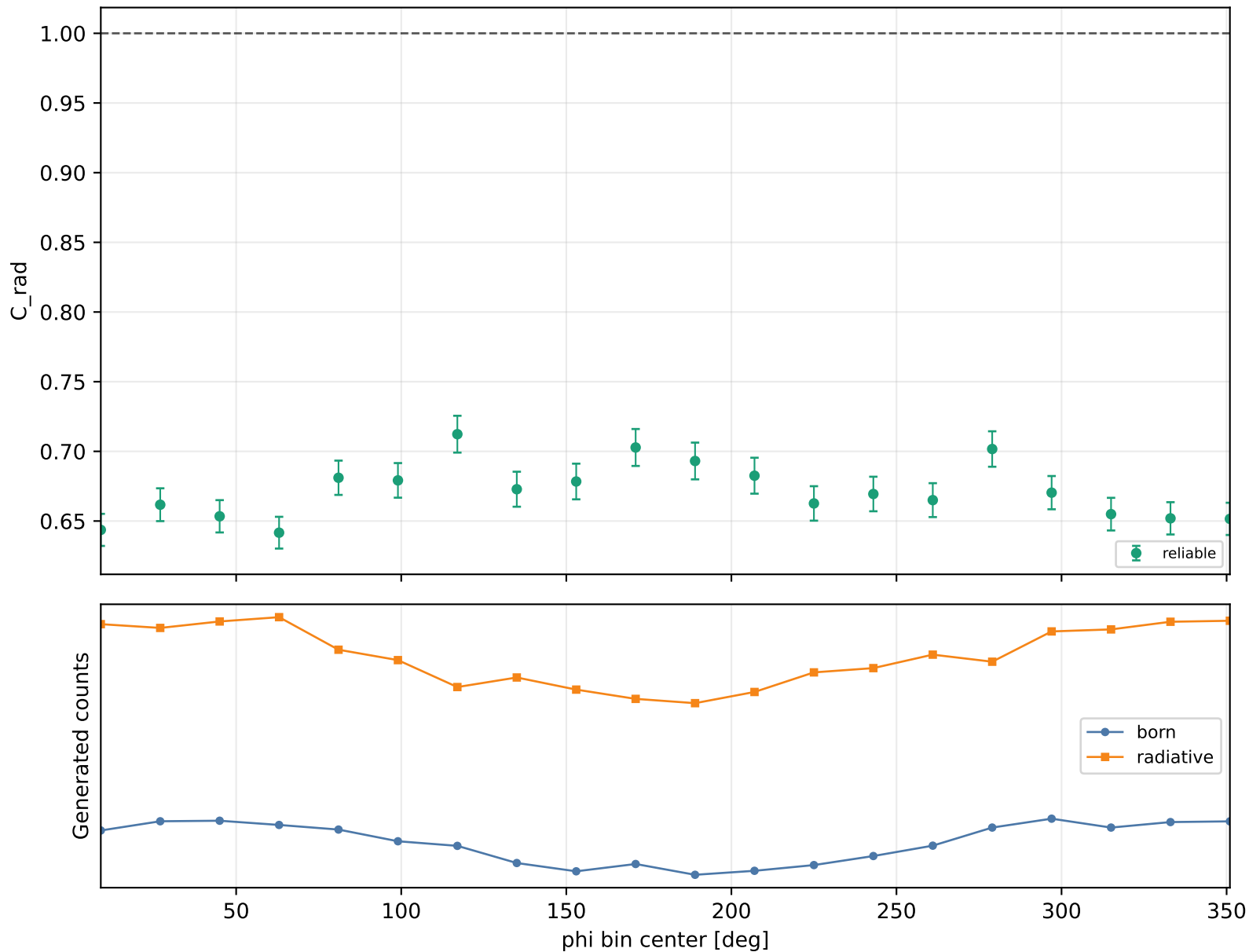
Radiative correction vs phi Q2 2.5-3, xB 0.58-0.7, -t 0.6-1
