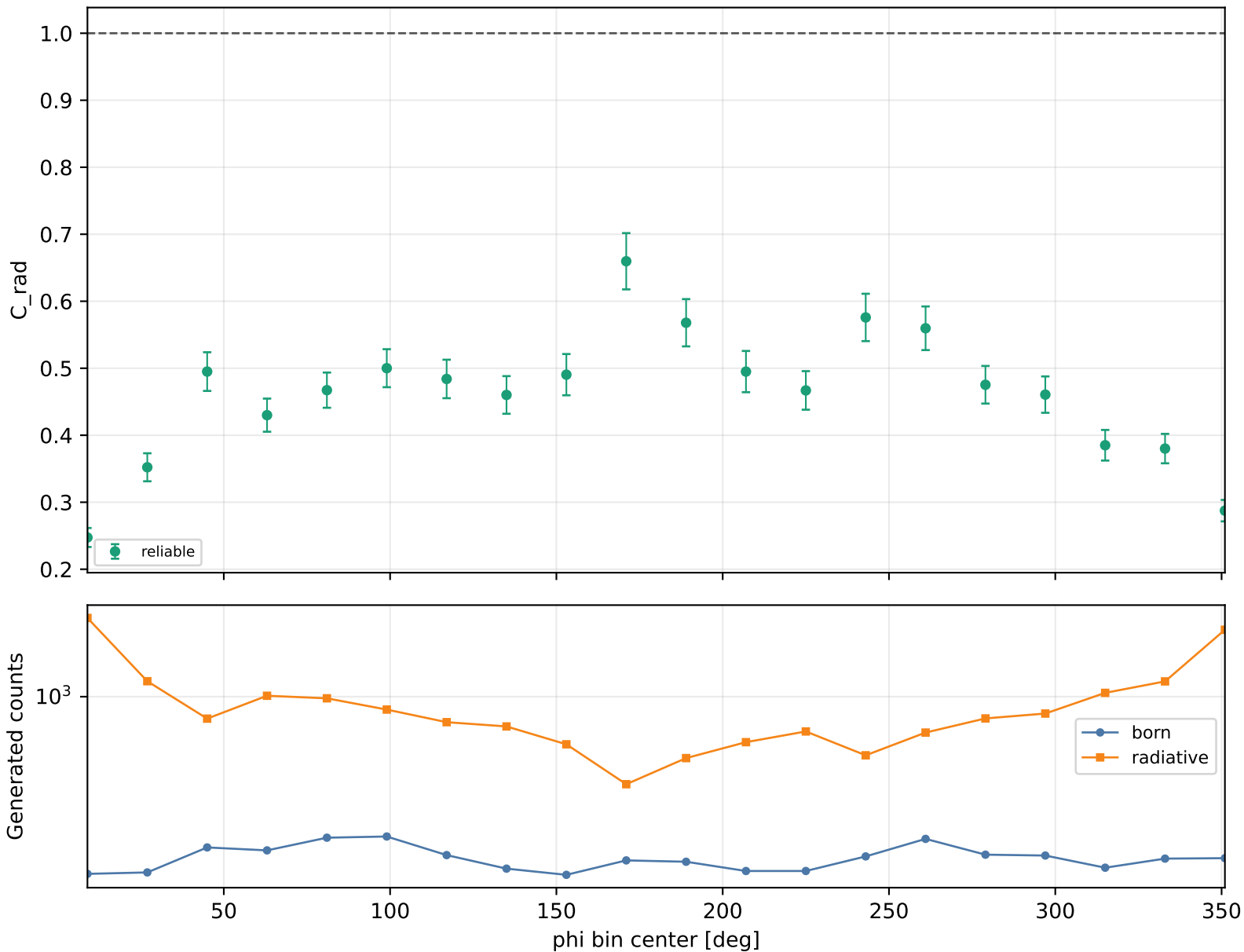
Radiative correction vs phi Q2 3-3.5, xB 0.3-0.38, -t 1.5-2
