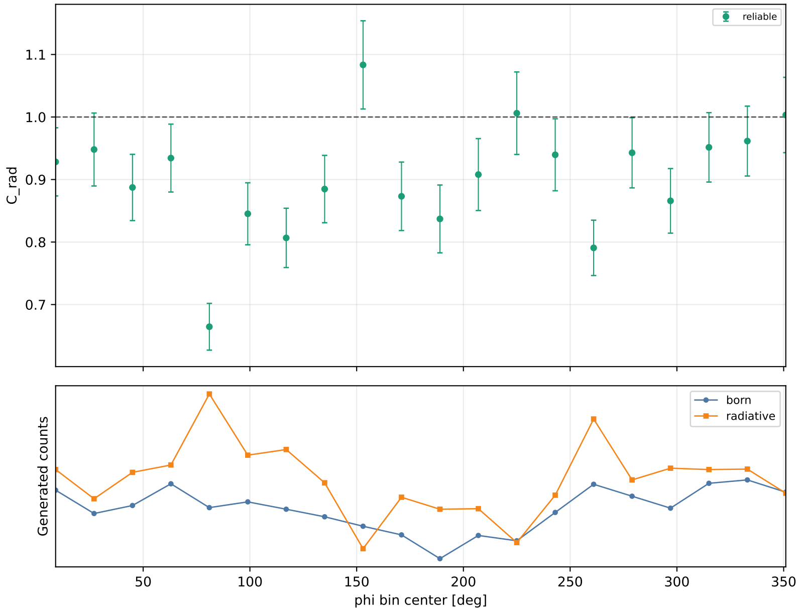
Radiative correction vs phi Q2 3-3.5, xB 0.38-0.48, -t 0.2-0.3
