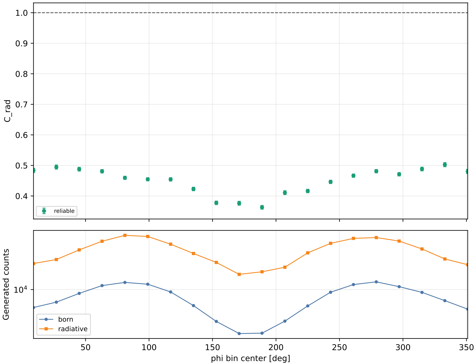
Radiative correction vs phi Q2 2-2.5, xB 0.38-0.48, -t 0.4-0.6
