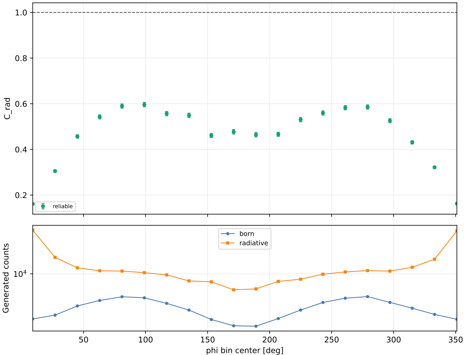
Radiative correction vs phi Q2 2-2.5, xB 0.3-0.38, -t 1-1.5
