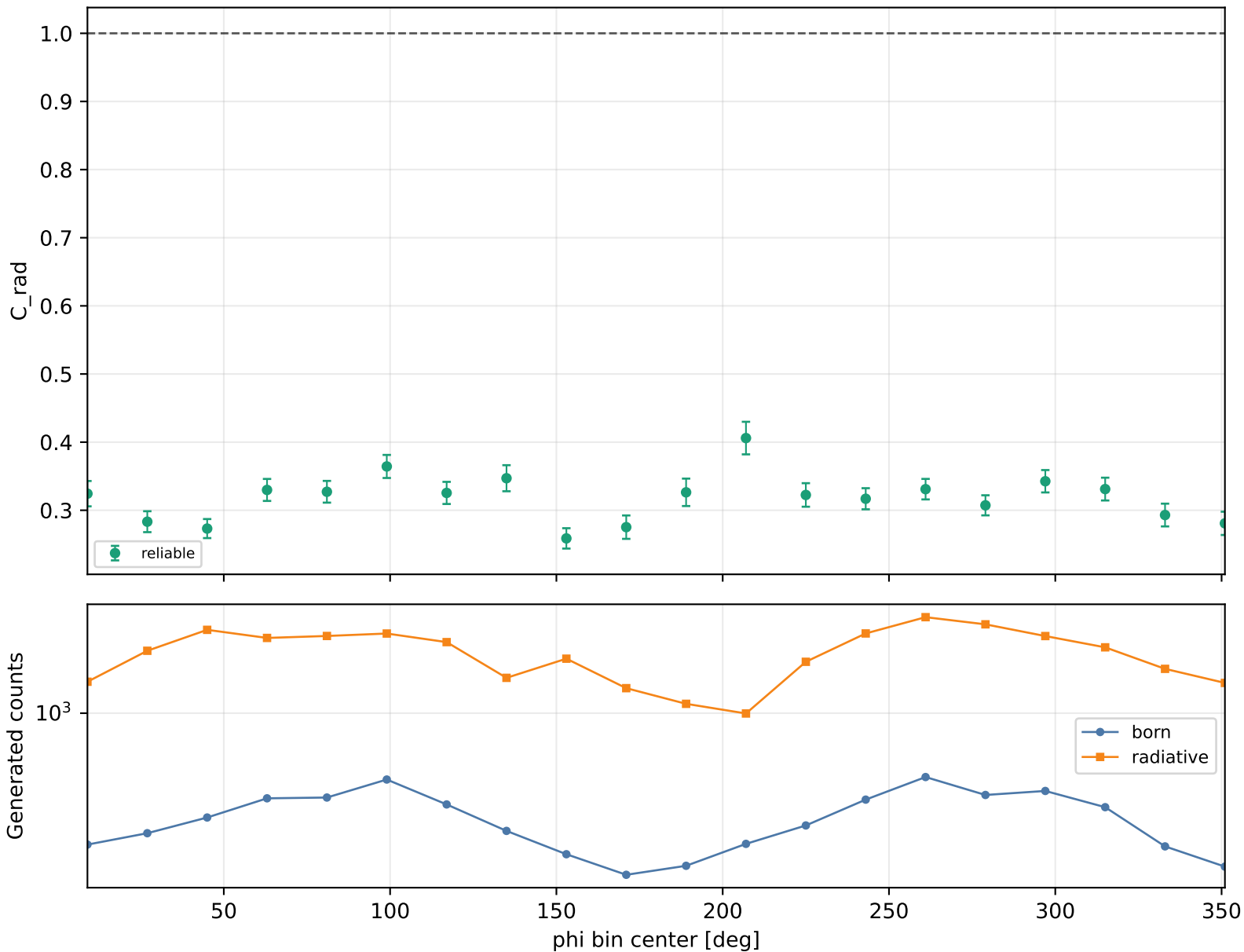
Radiative correction vs phi Q2 4.6-5.5, xB 0.58-0.7, -t 1-1.5
