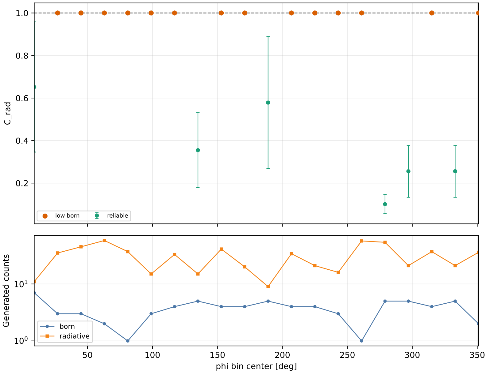
Radiative correction vs phi Q2 2-2.5, xB 0.15-0.2, -t 0.09-0.15
