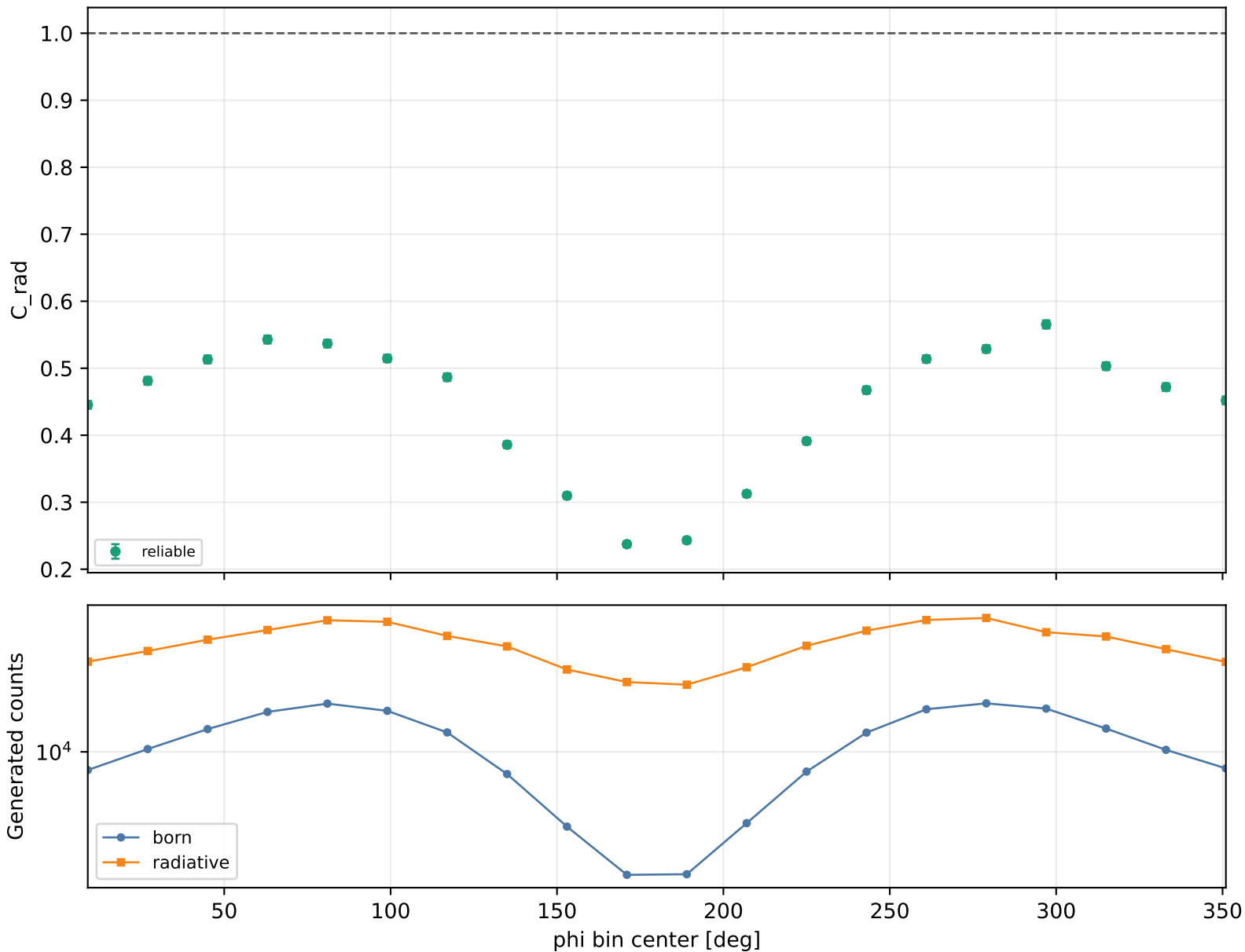
Radiative correction vs phi Q2 1-1.5, xB 0.15-0.2, -t 0.09-0.15
