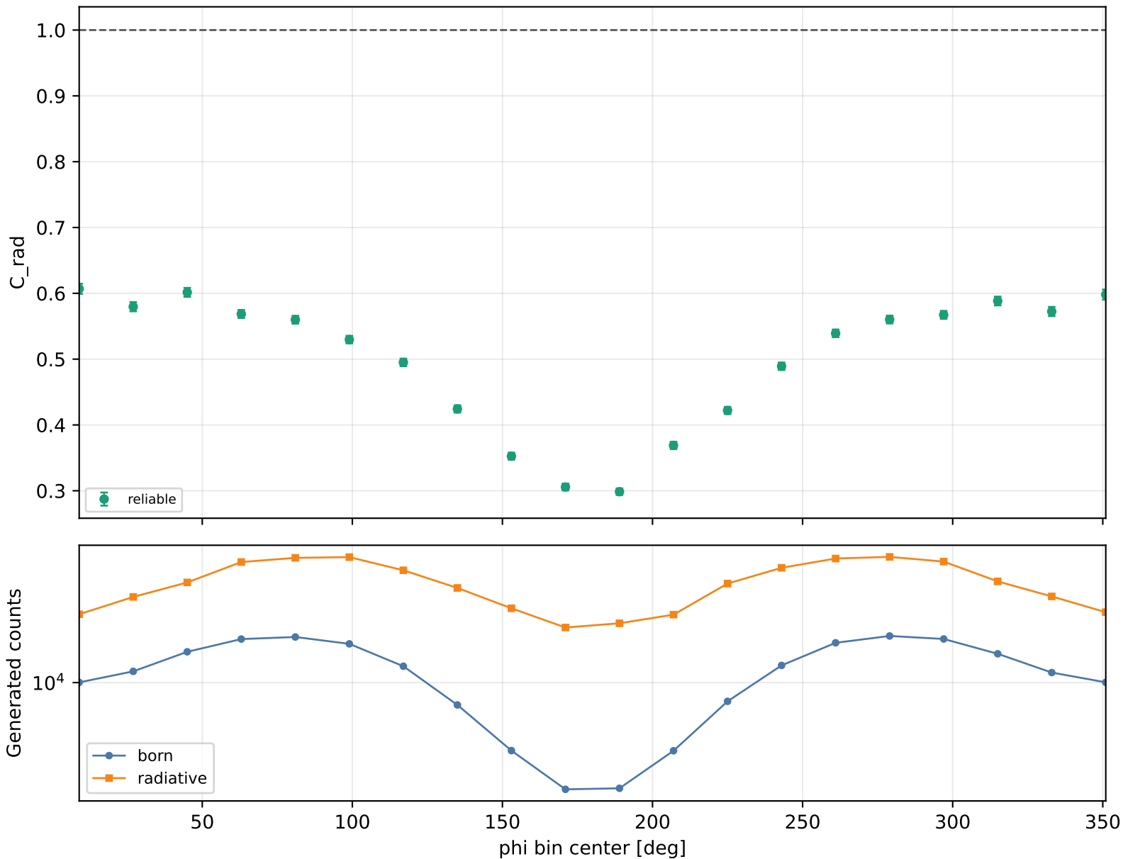
Radiative correction vs phi Q2 1.5-2, xB 0.3-0.38, -t 0.2-0.3
