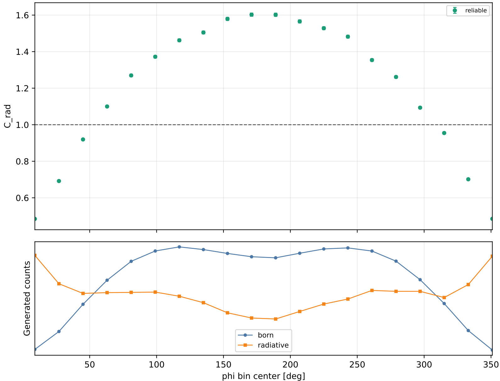
Radiative correction vs phi Q2 1.5-2, xB 0.38-0.48, -t 1.5-2
