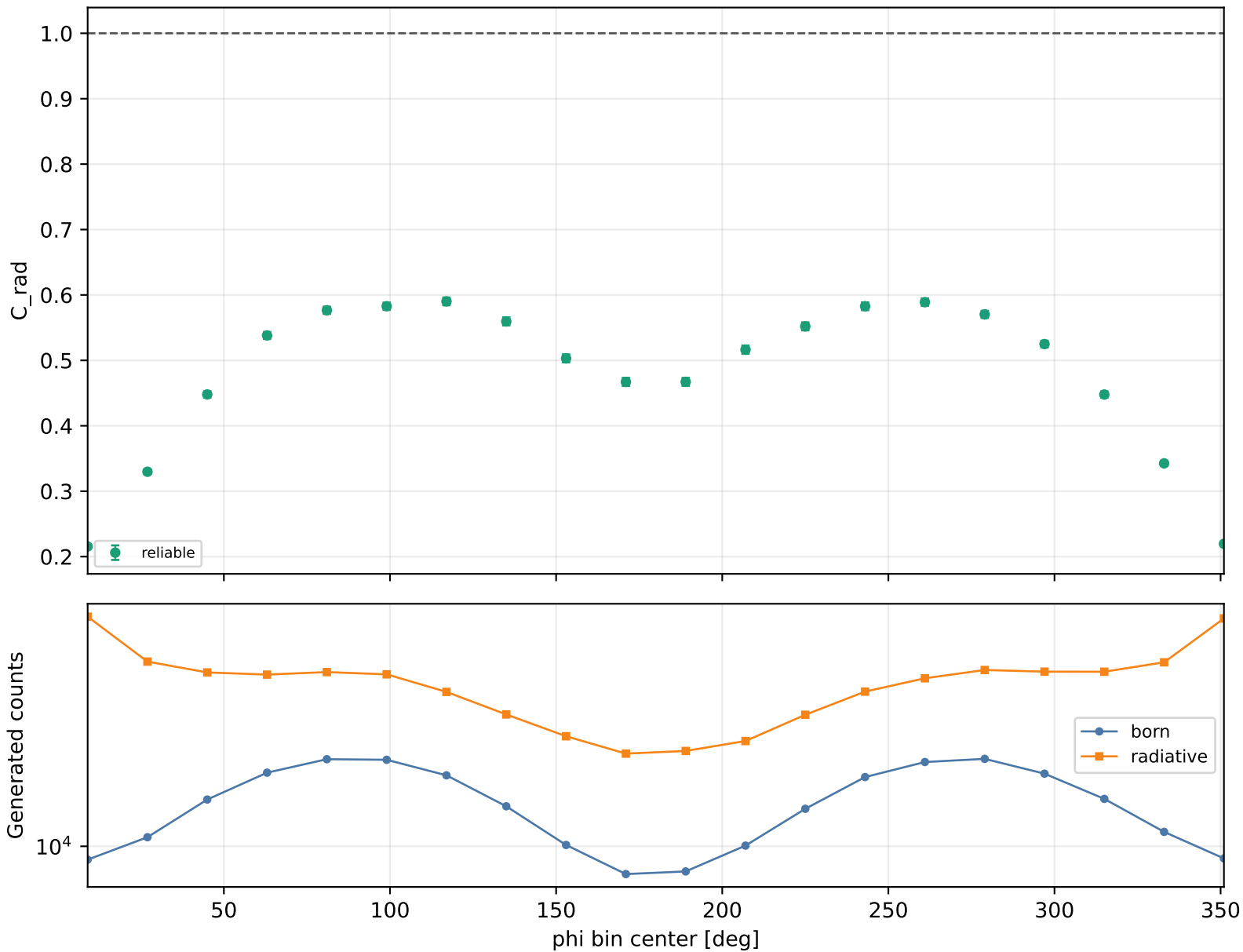
Radiative correction vs phi Q2 2-2.5, xB 0.38-0.48, -t 1-1.5
