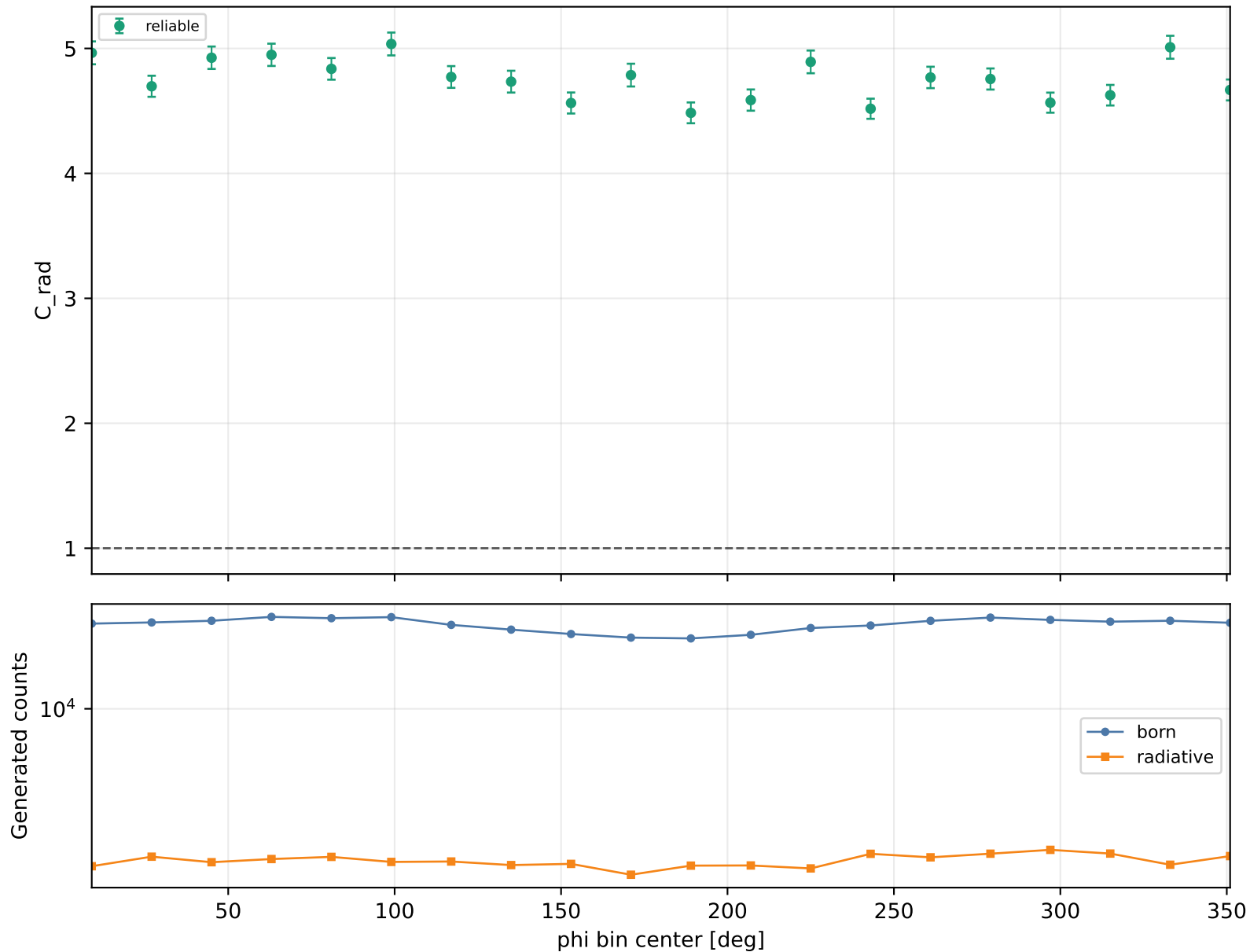
Radiative correction vs phi Q2 2-2.5, xB 0.58-0.7, -t 0.6-1
