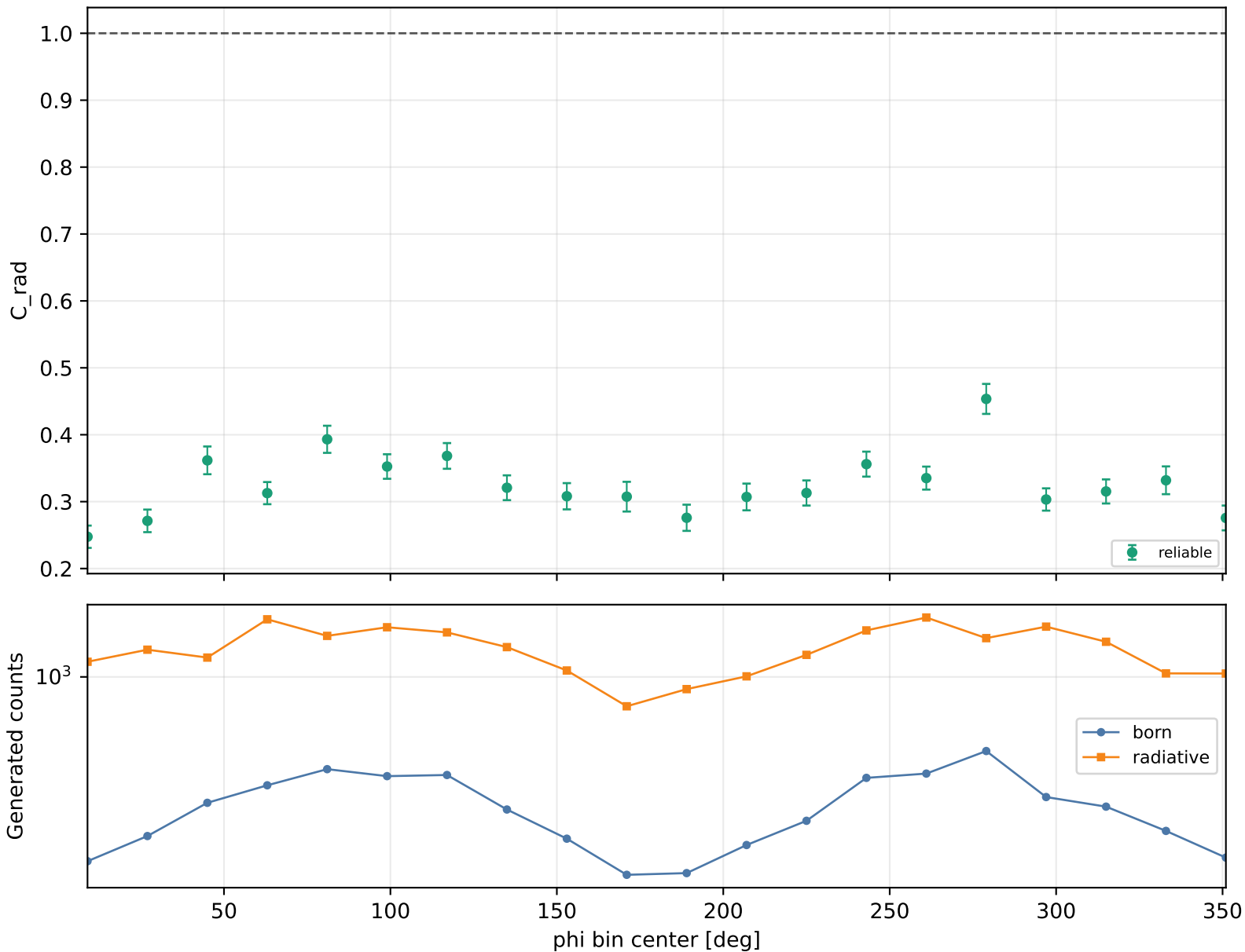
Radiative correction vs phi Q2 4.6-5.5, xB 0.58-0.7, -t 1.5-2
