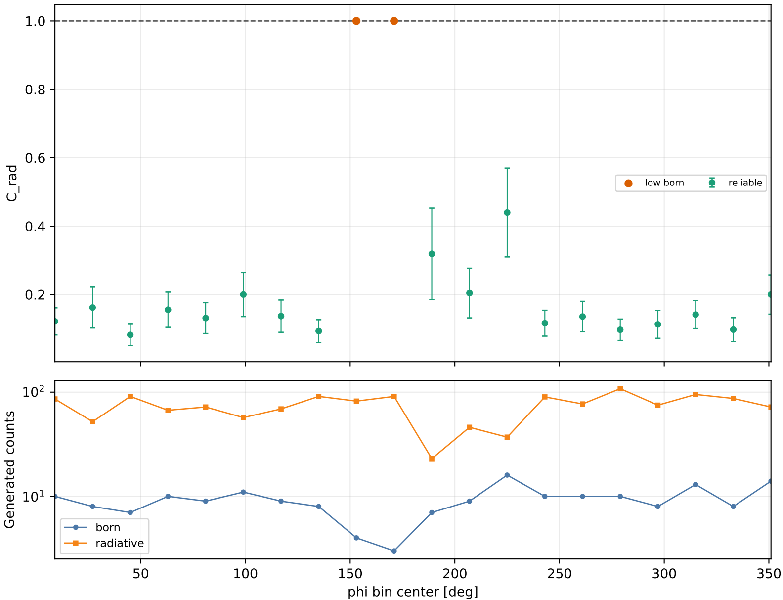
Radiative correction vs phi Q2 1-1.5, xB 0.05-0.1, -t 0.4-0.6
