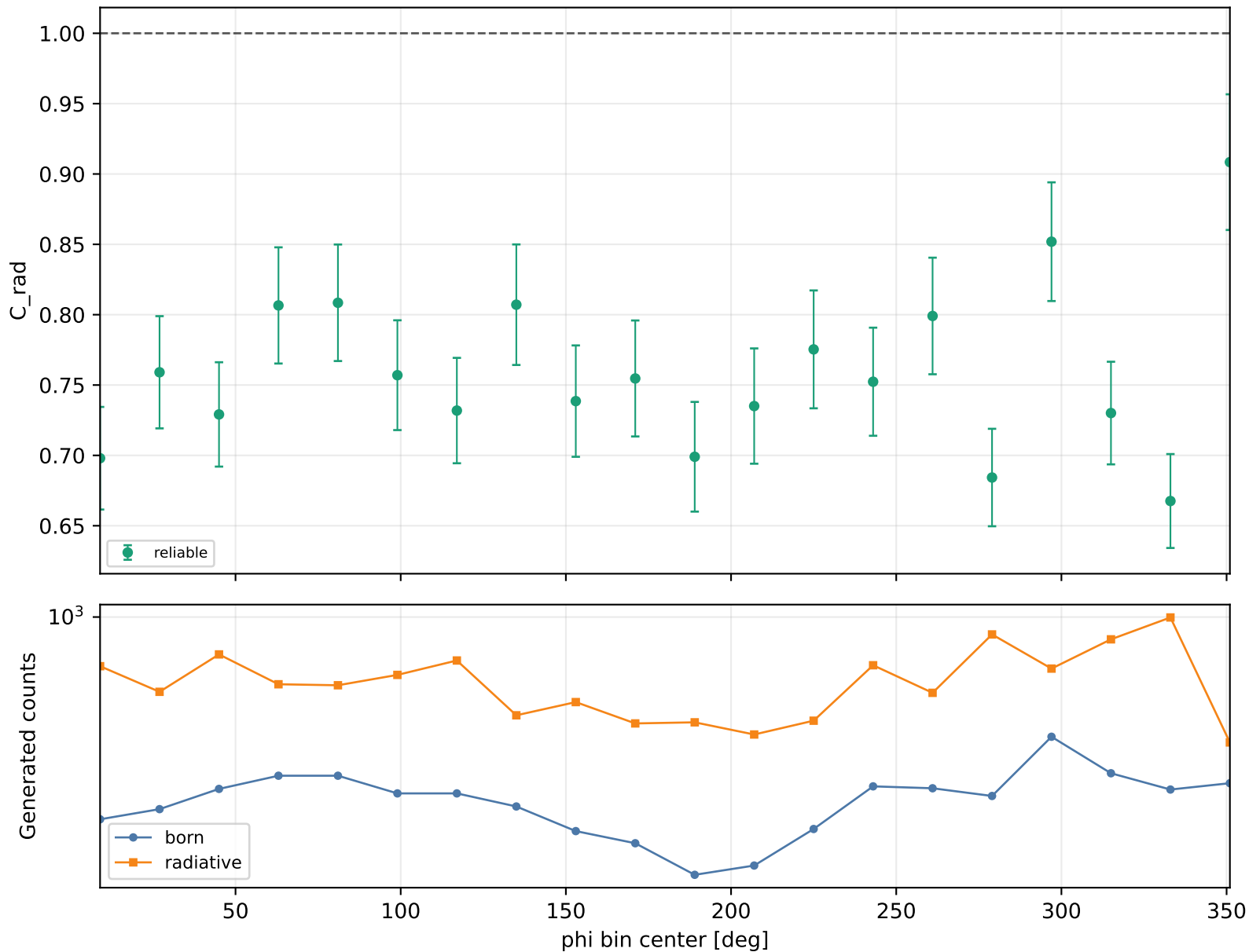
Radiative correction vs phi Q2 4-4.6, xB 0.48-0.58, -t 0.4-0.6
