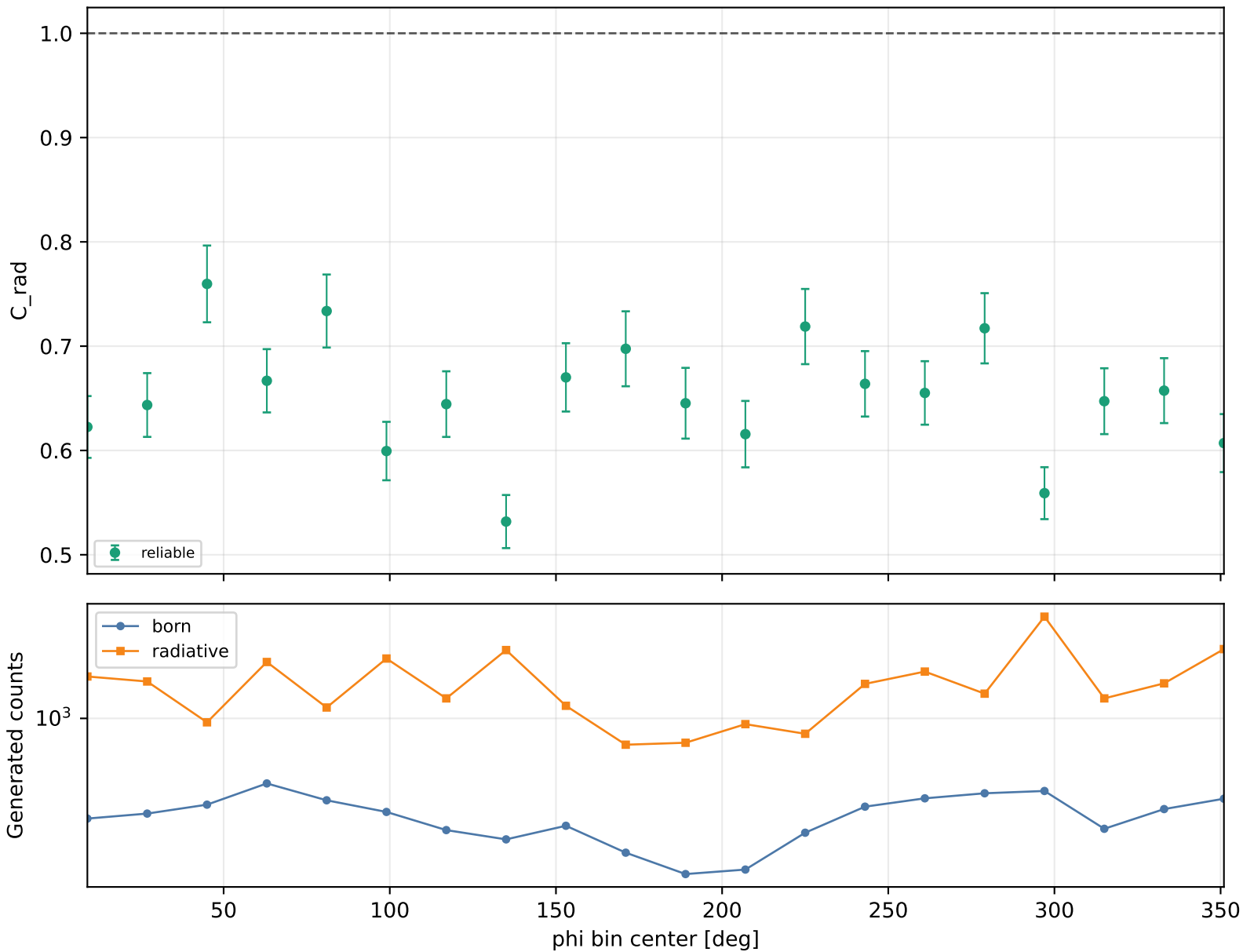
Radiative correction vs phi Q2 3-3.5, xB 0.3-0.38, -t 0.2-0.3
