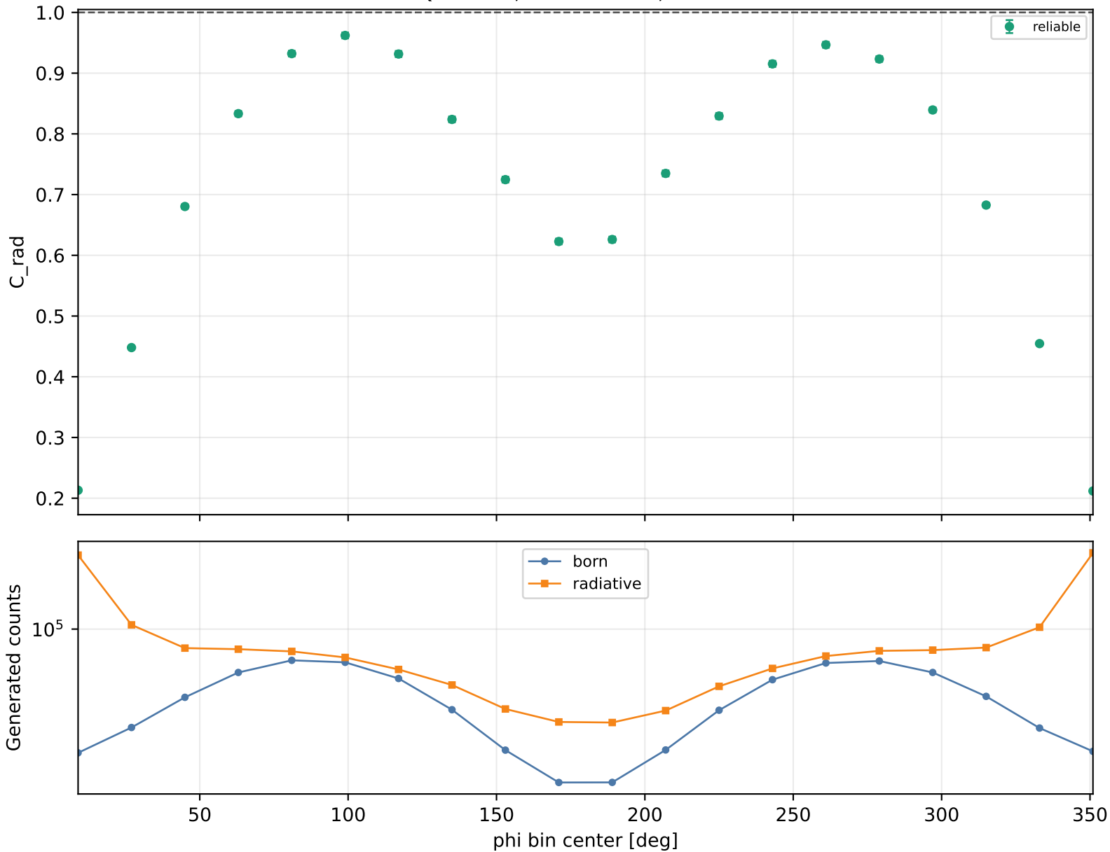
Radiative correction vs phi Q2 1-1.5, xB 0.25-0.3, -t 0.6-1
