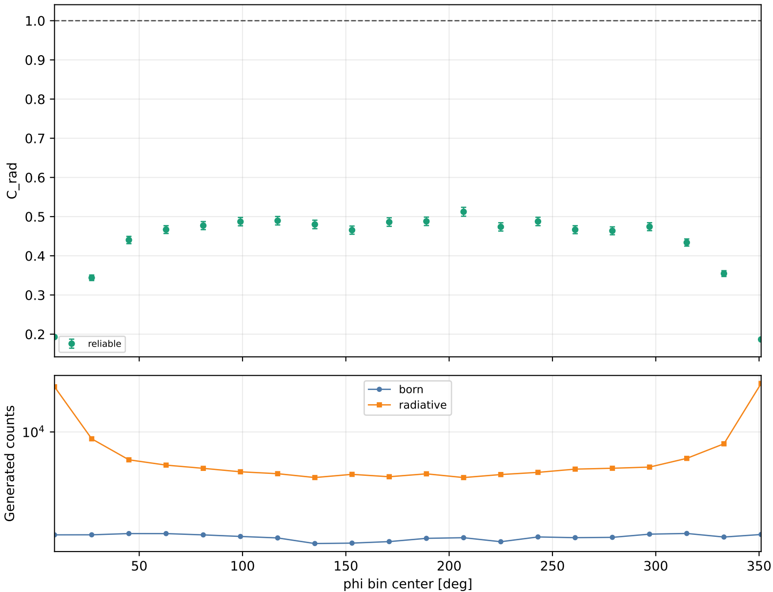
Radiative correction vs phi Q2 1-1.5, xB 0.15-0.2, -t 1.5-2
