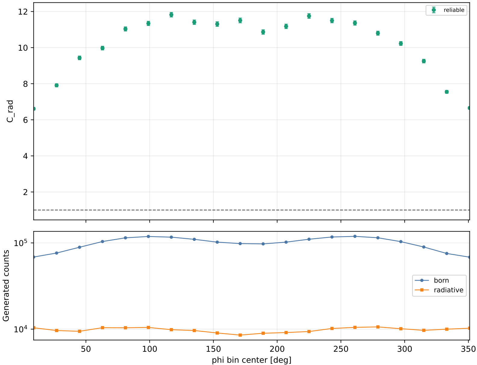
Radiative correction vs phi Q2 1.5-2, xB 0.48-0.58, -t 1-1.5
