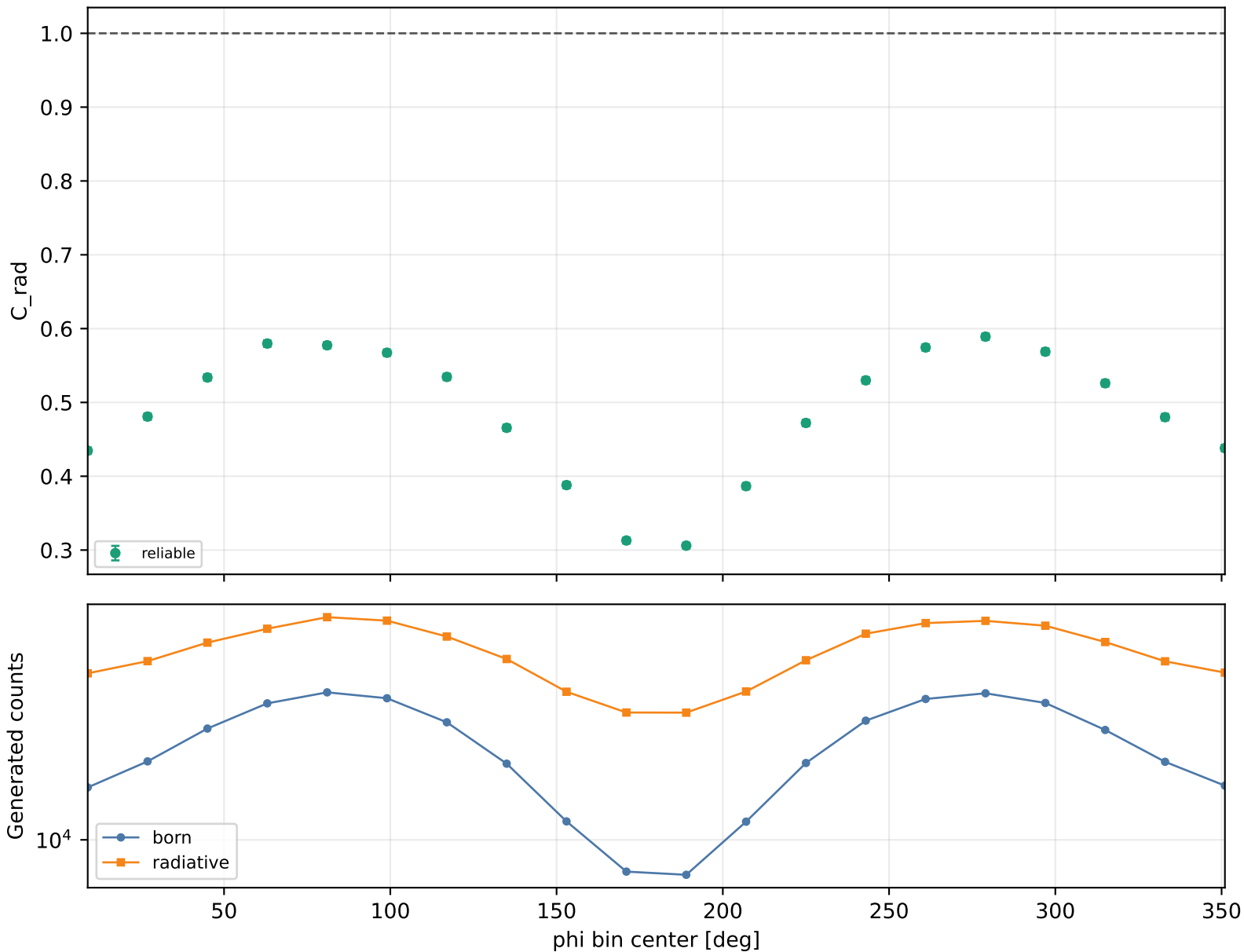
Radiative correction vs phi Q2 1.5-2, xB 0.3-0.38, -t 0.4-0.6
