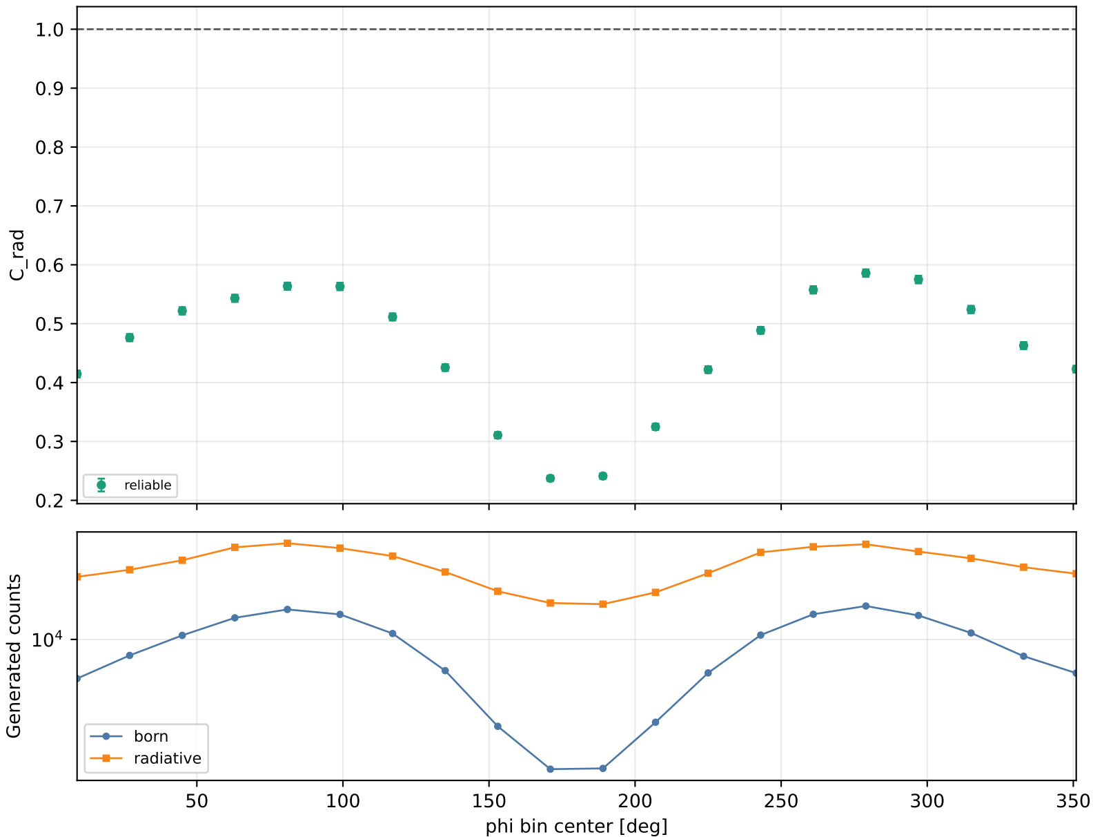
Radiative correction vs phi Q2 1-1.5, xB 0.15-0.2, -t 0.15-0.2
