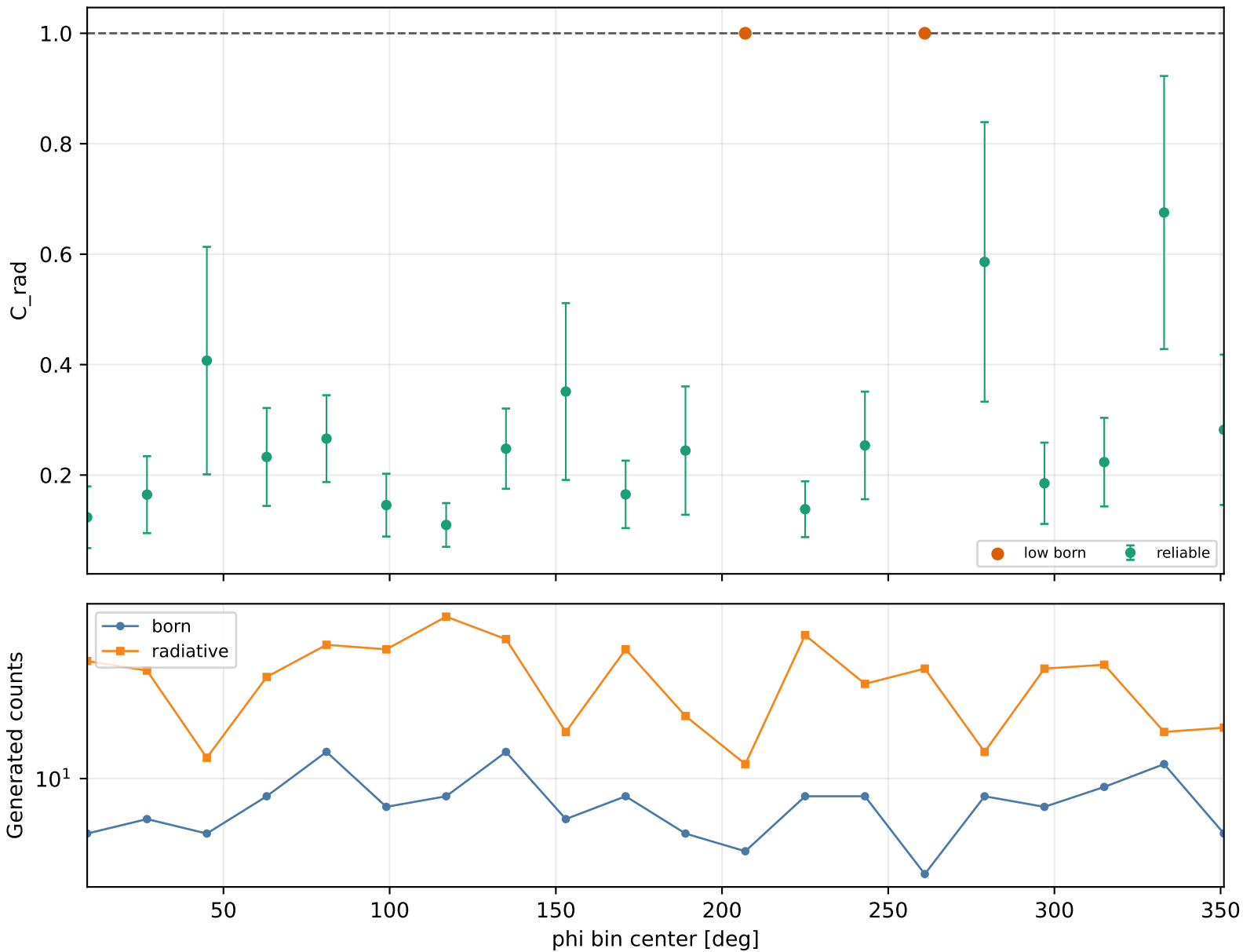
Radiative correction vs phi Q2 1.5-2, xB 0.1-0.15, -t 0.3-0.4
