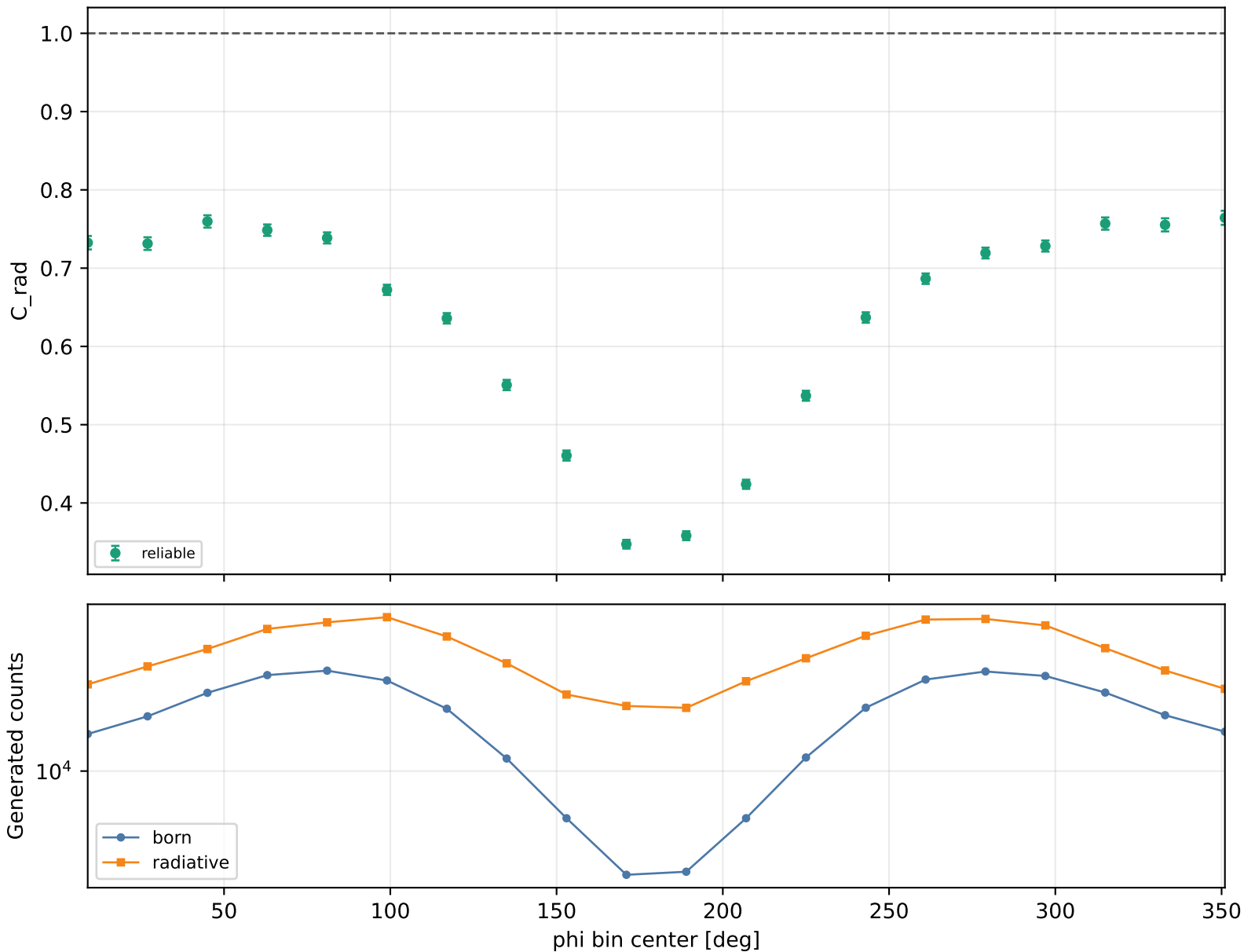
Radiative correction vs phi Q2 1-1.5, xB 0.25-0.3, -t 0.15-0.2
