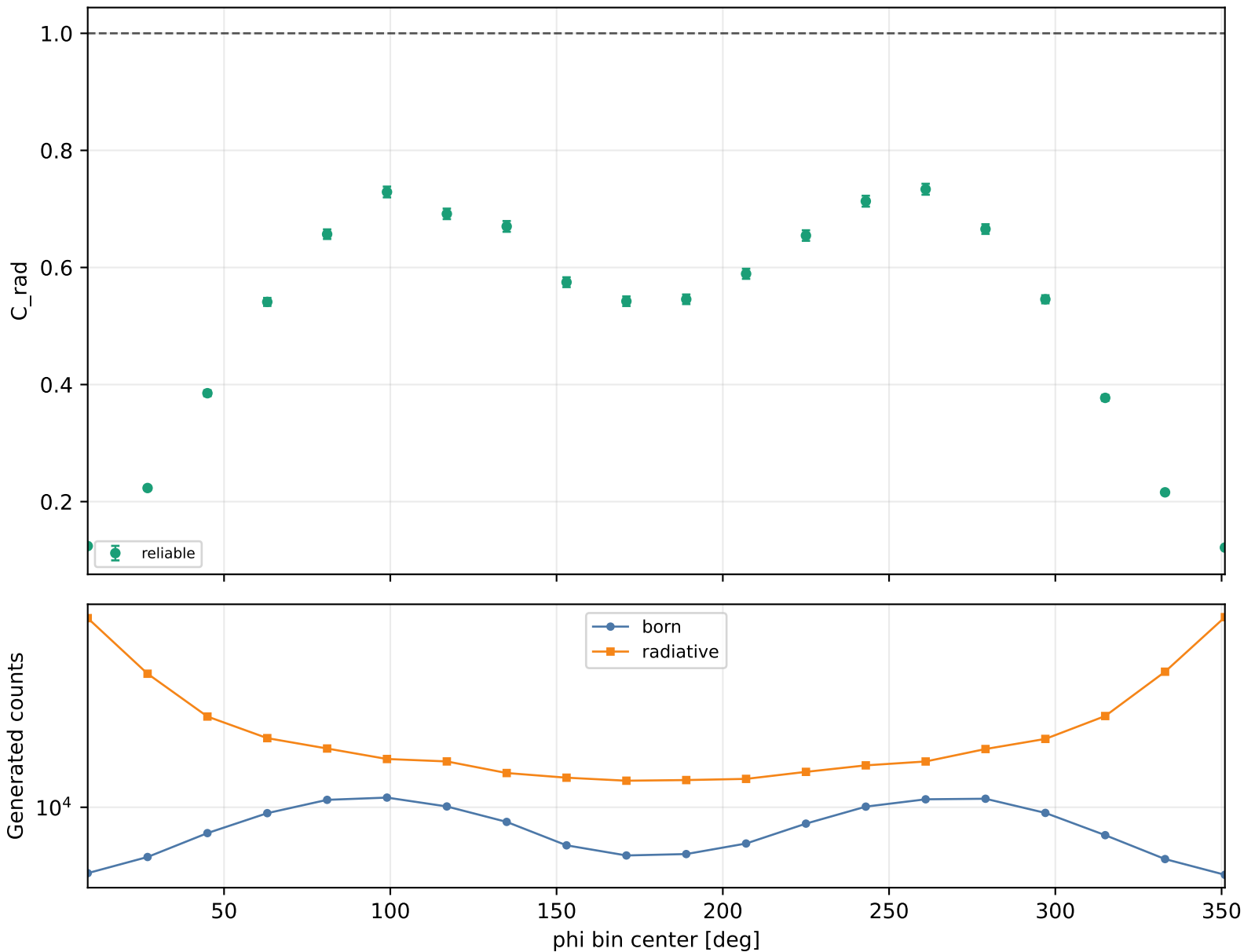
Radiative correction vs phi Q2 1.5-2, xB 0.3-0.38, -t 1.5-2
