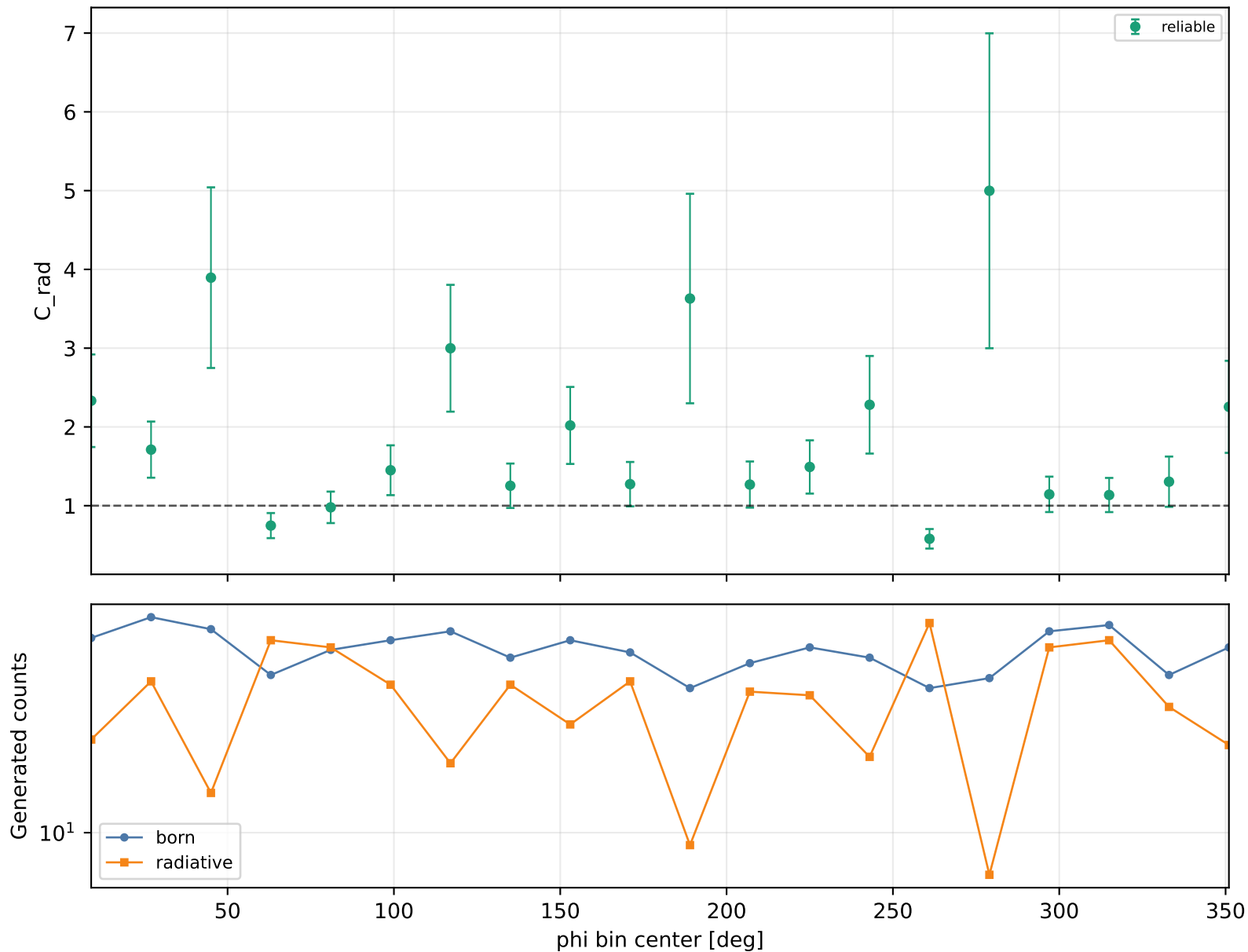
Radiative correction vs phi Q2 2-2.5, xB 0.38-0.48, -t 0.15-0.2
