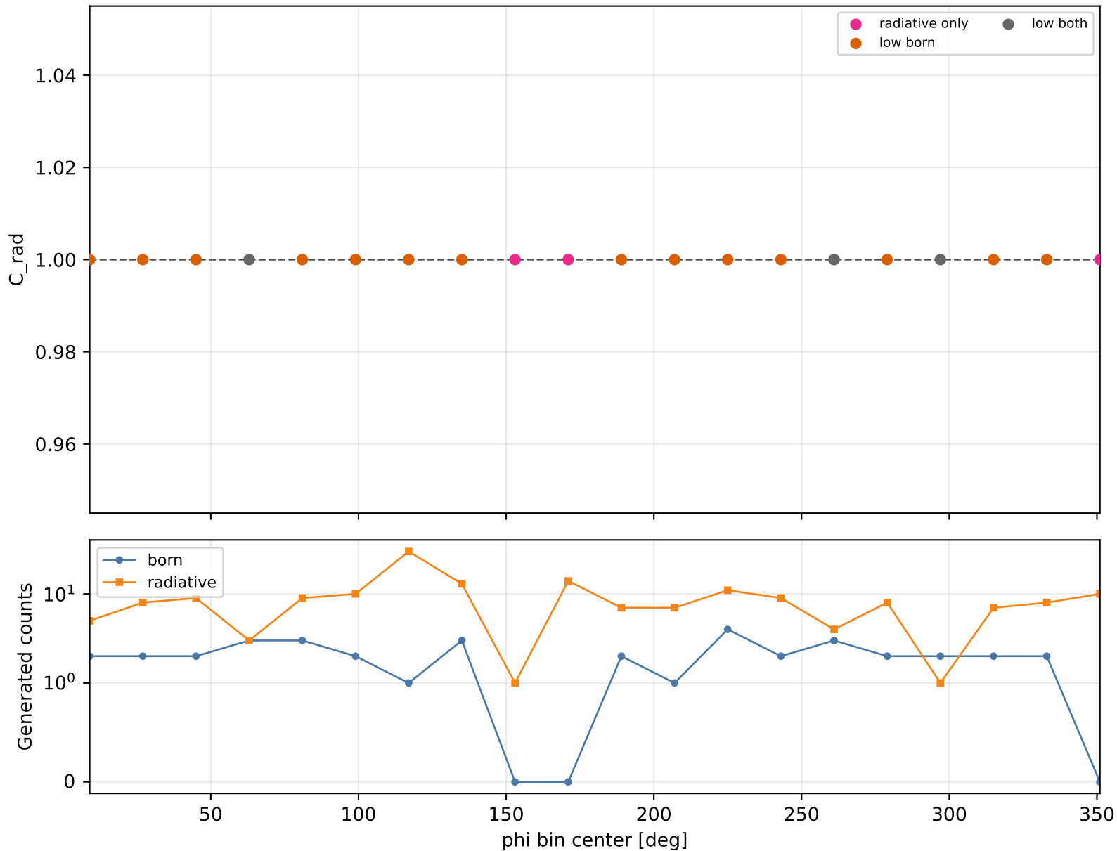
Radiative correction vs phi Q2 3-3.5, xB 0.25-0.3, -t 0.09-0.15
