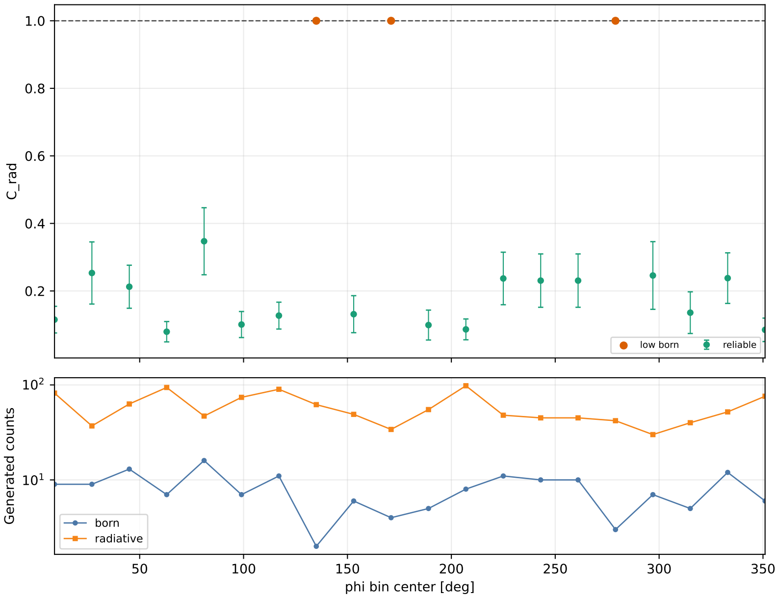
Radiative correction vs phi Q2 1.5-2, xB 0.1-0.15, -t 0.4-0.6
