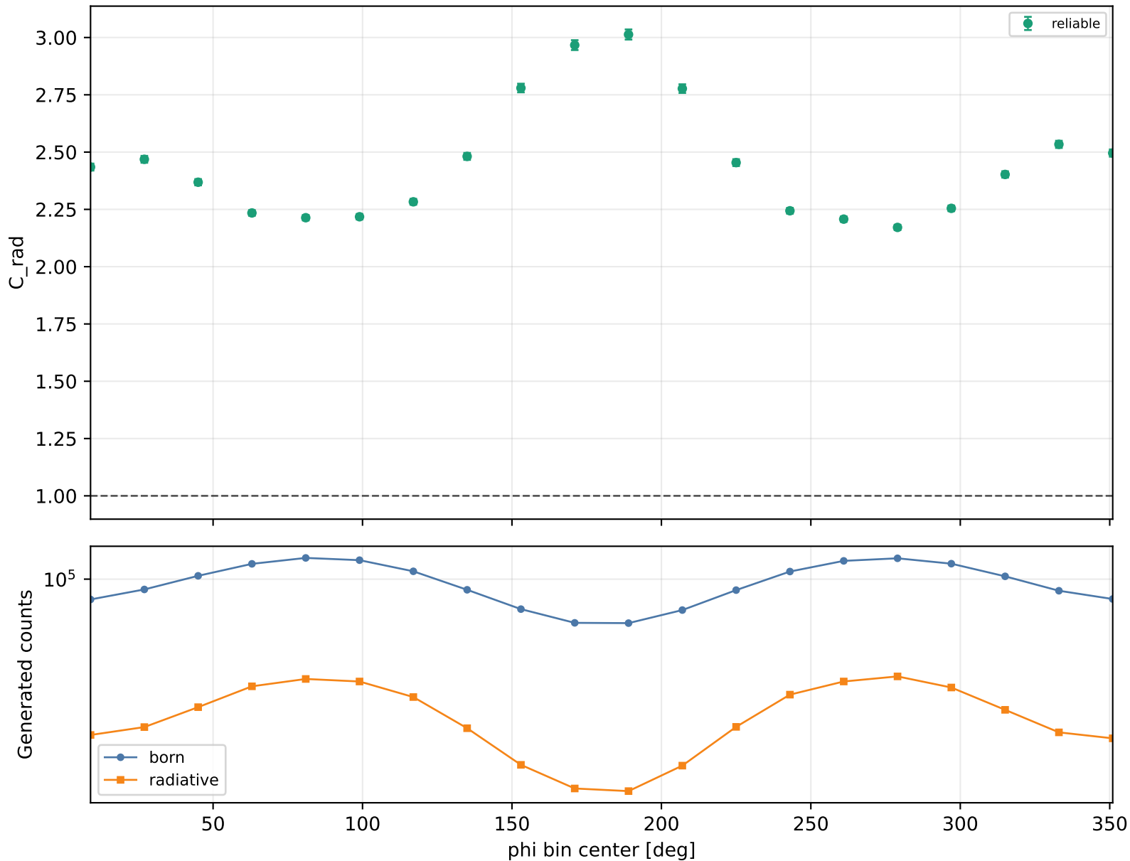
Radiative correction vs phi Q2 1-1.5, xB 0.3-0.38, -t 0.4-0.6
