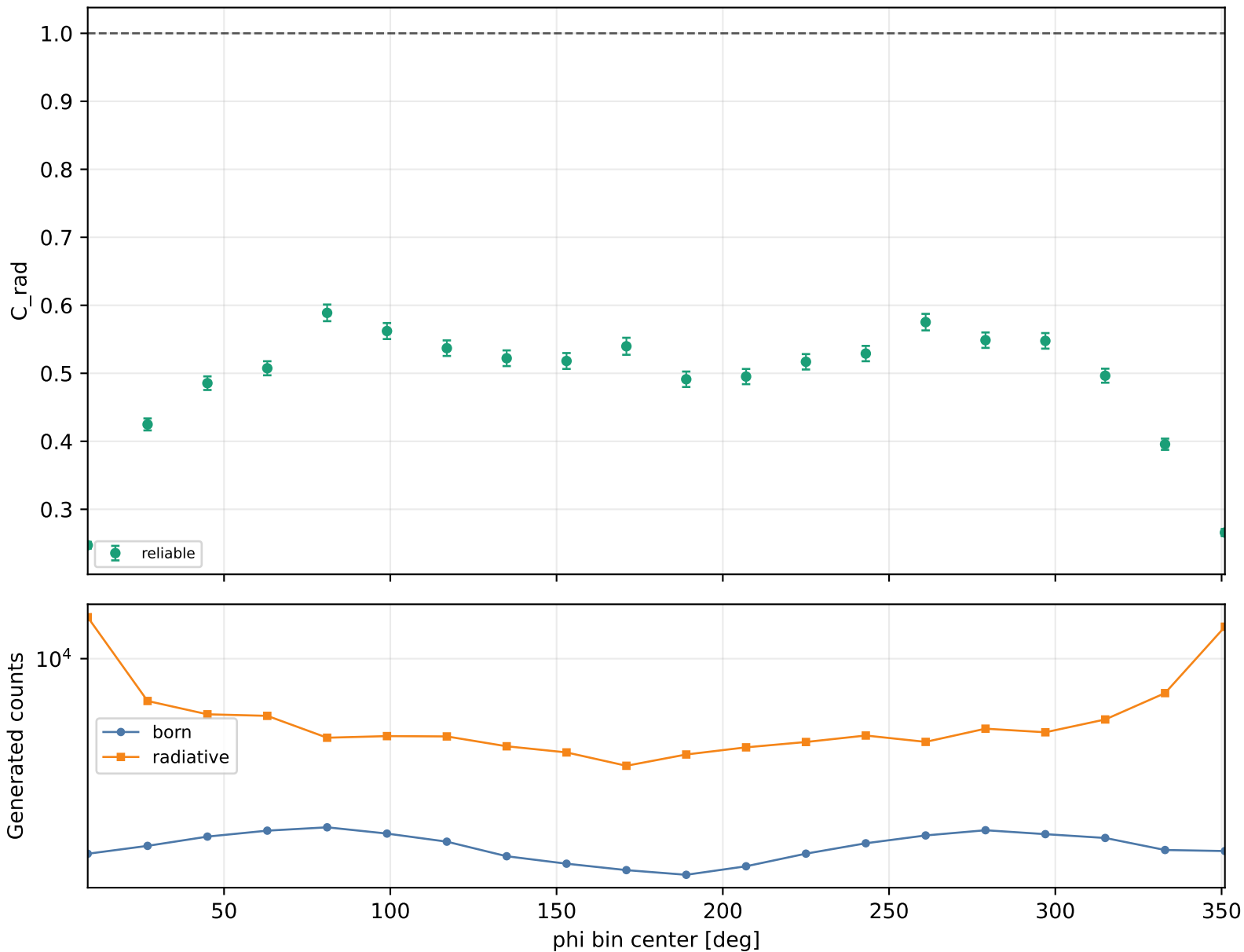
Radiative correction vs phi Q2 1.5-2, xB 0.2-0.25, -t 1-1.5
