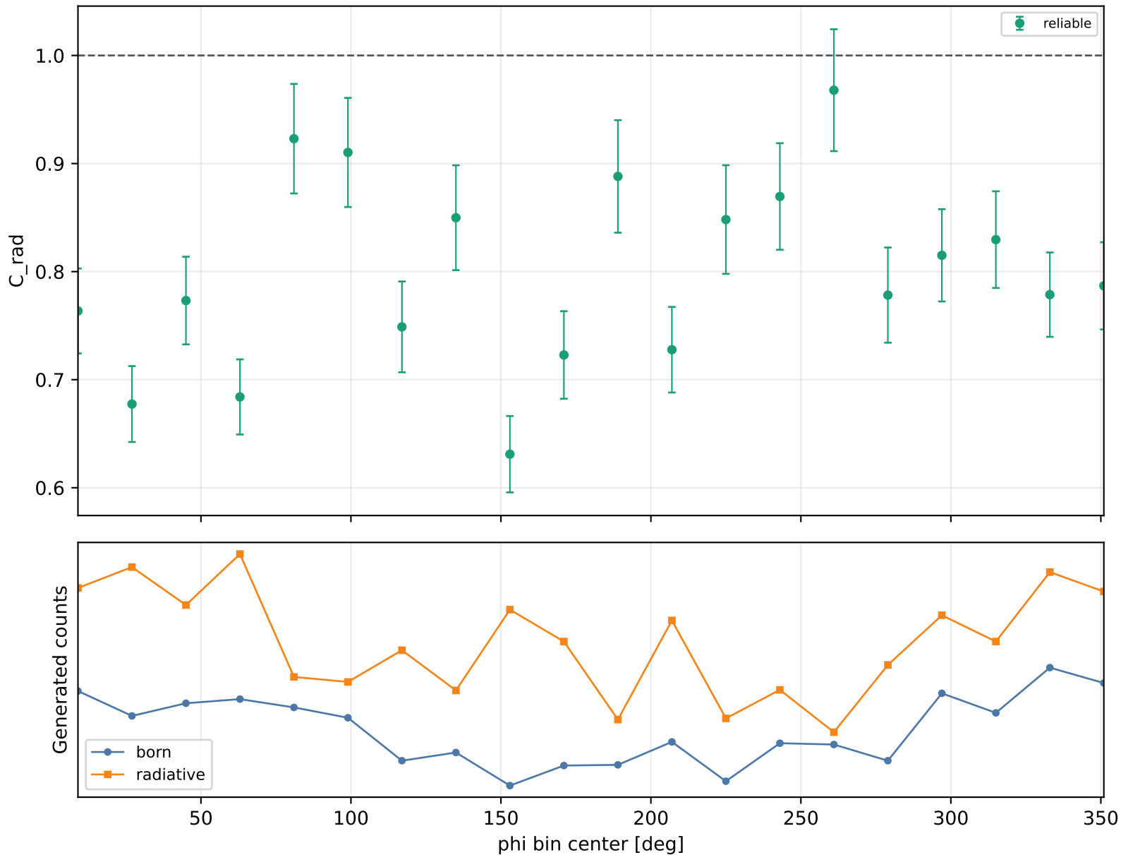
Radiative correction vs phi Q2 2-2.5, xB 0.48-0.58, -t 0.3-0.4
