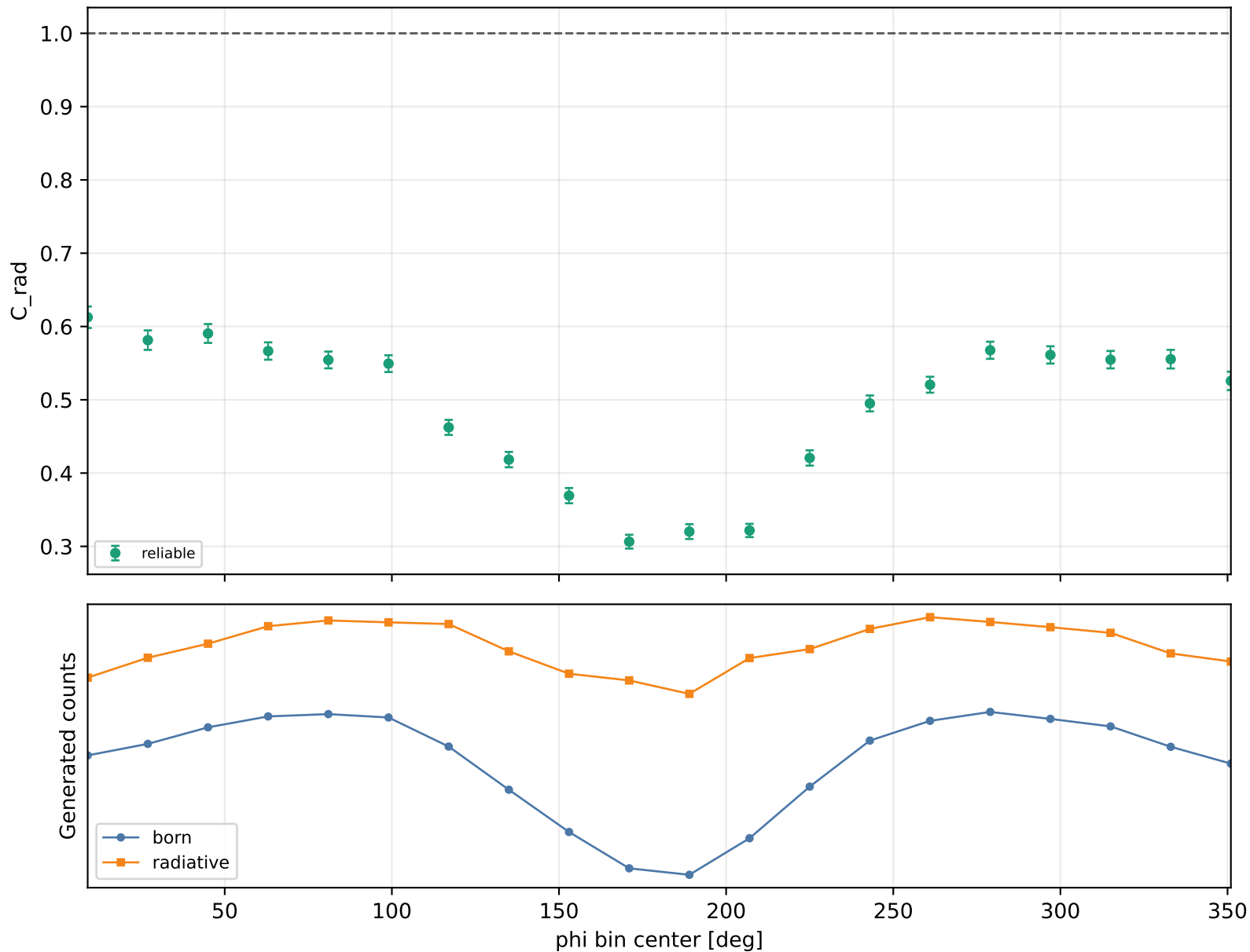
Radiative correction vs phi Q2 1.5-2, xB 0.25-0.3, -t 0.15-0.2
