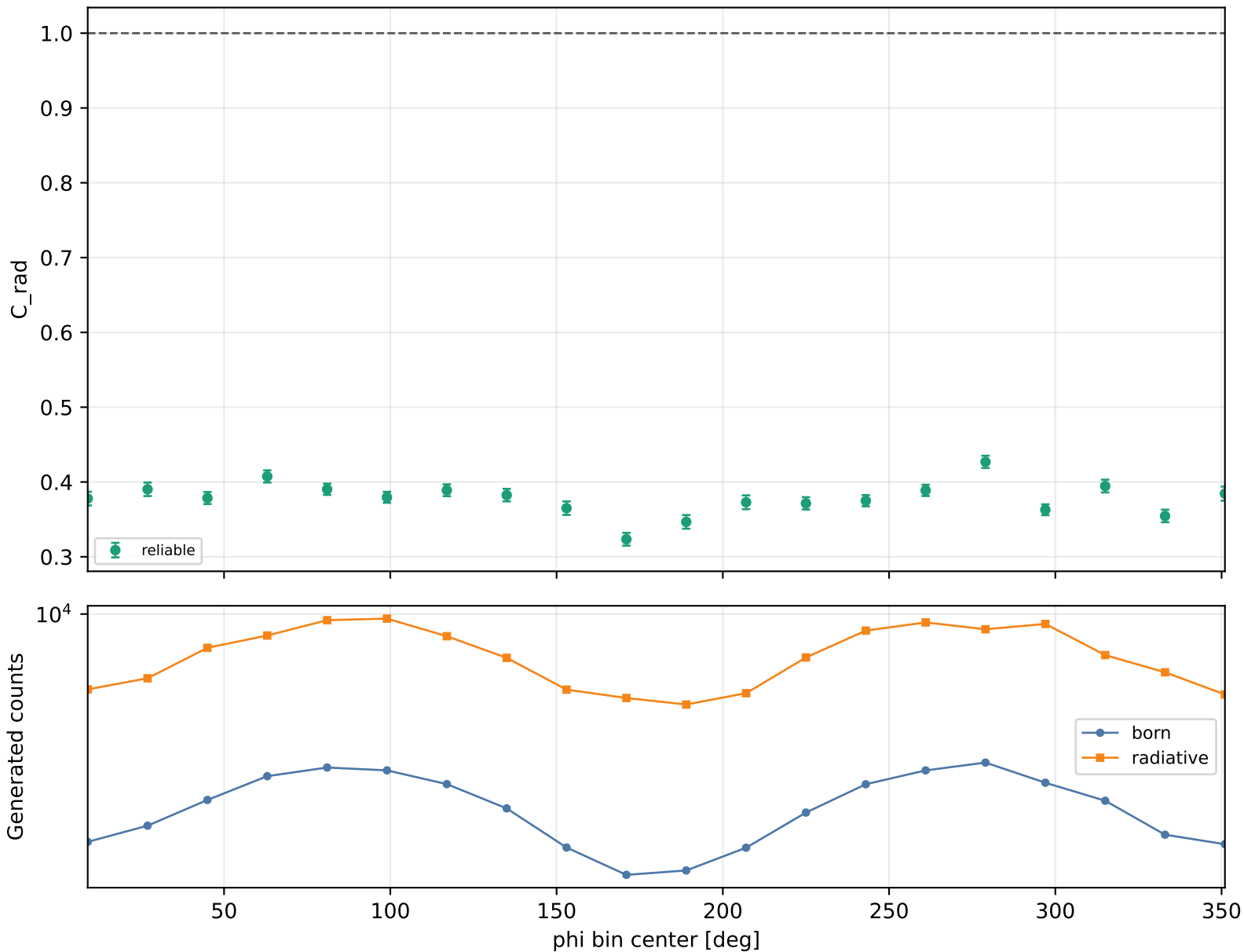
Radiative correction vs phi Q2 3-3.5, xB 0.48-0.58, -t 0.6-1
