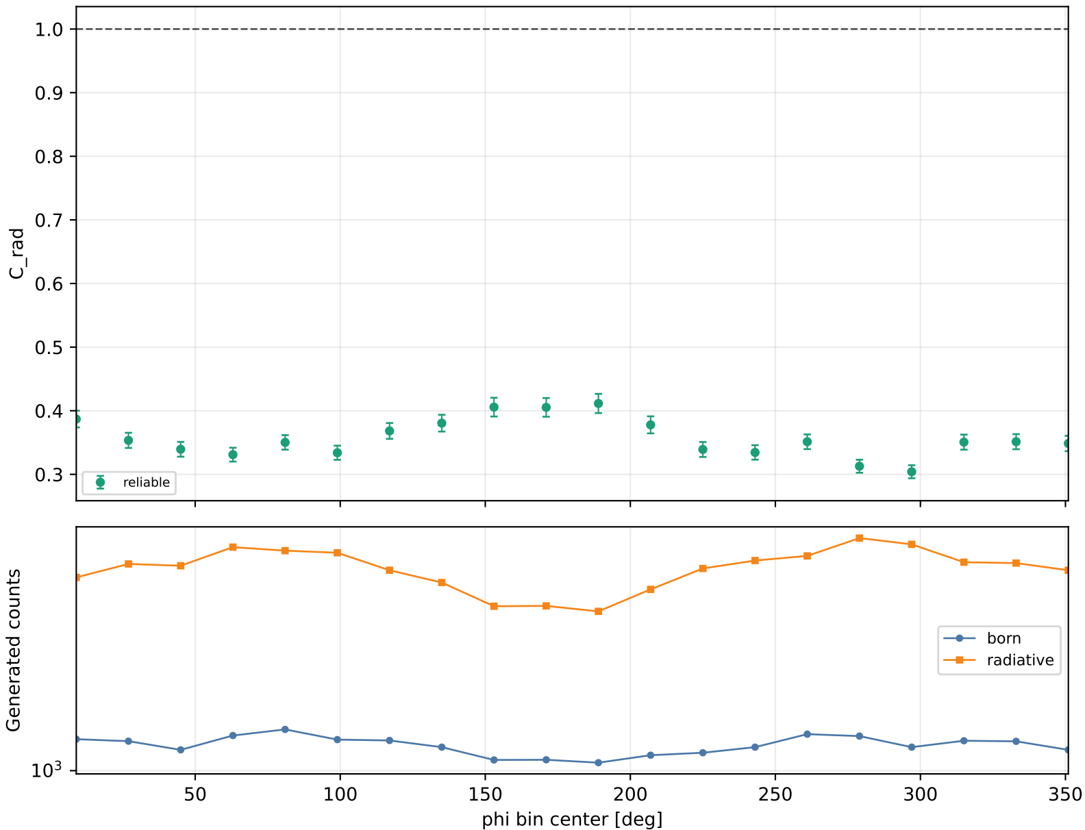
Radiative correction vs phi Q2 3.5-4, xB 0.58-0.7, -t 1-1.5
