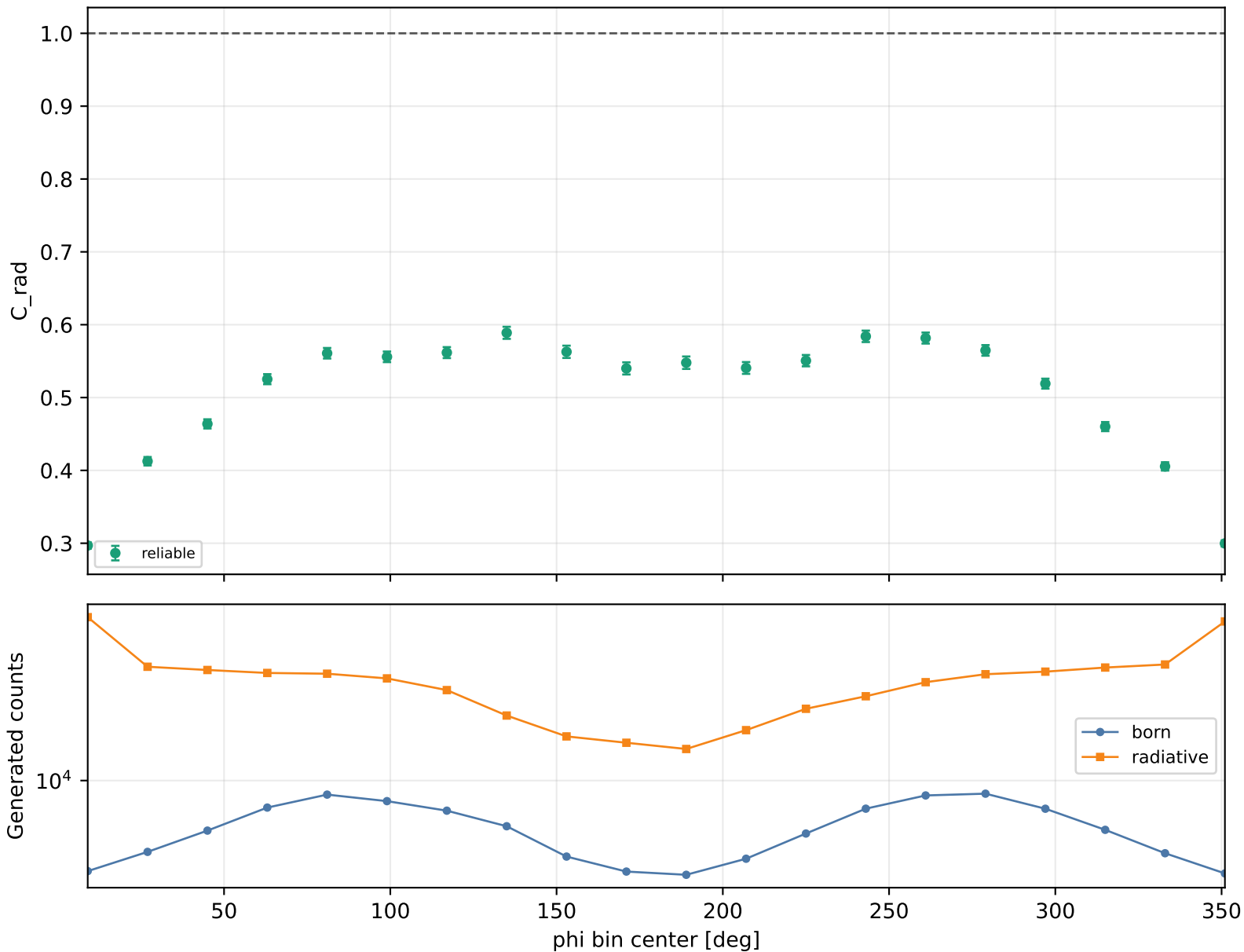
Radiative correction vs phi Q2 2.5-3, xB 0.48-0.58, -t 1.5-2
