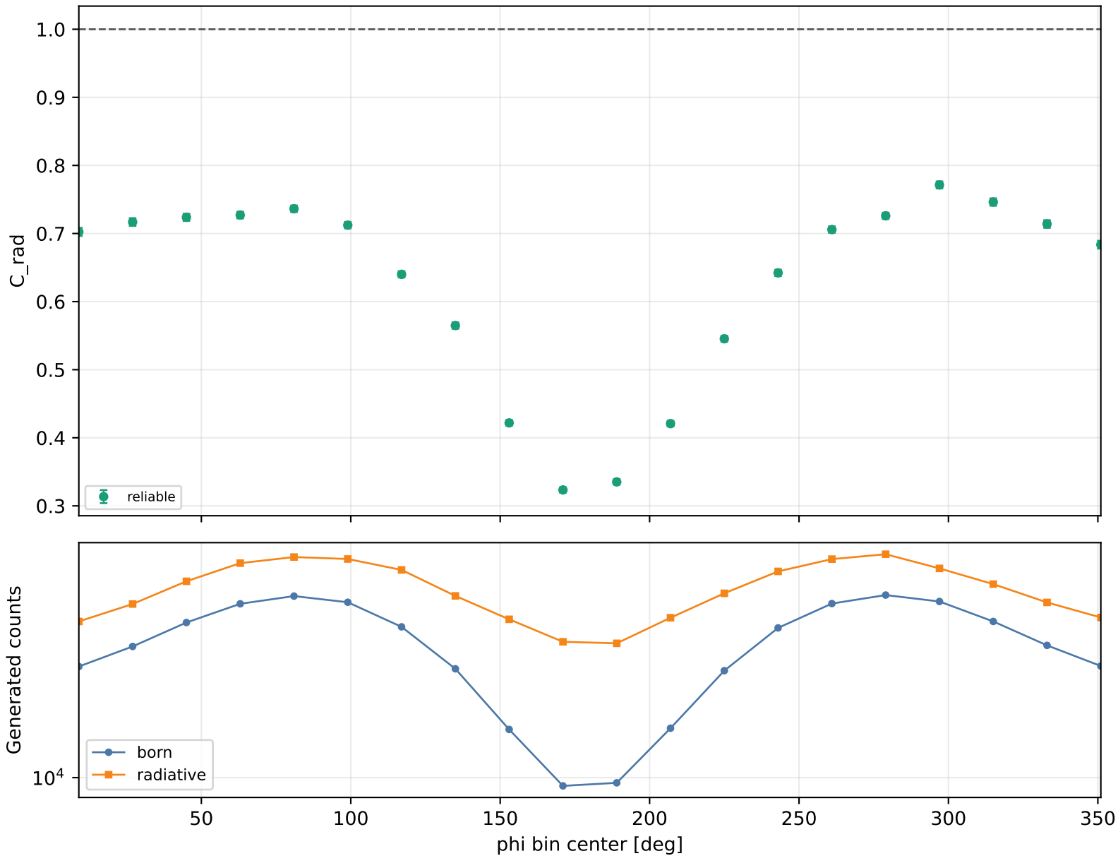
Radiative correction vs phi Q2 1-1.5, xB 0.25-0.3, -t 0.2-0.3
