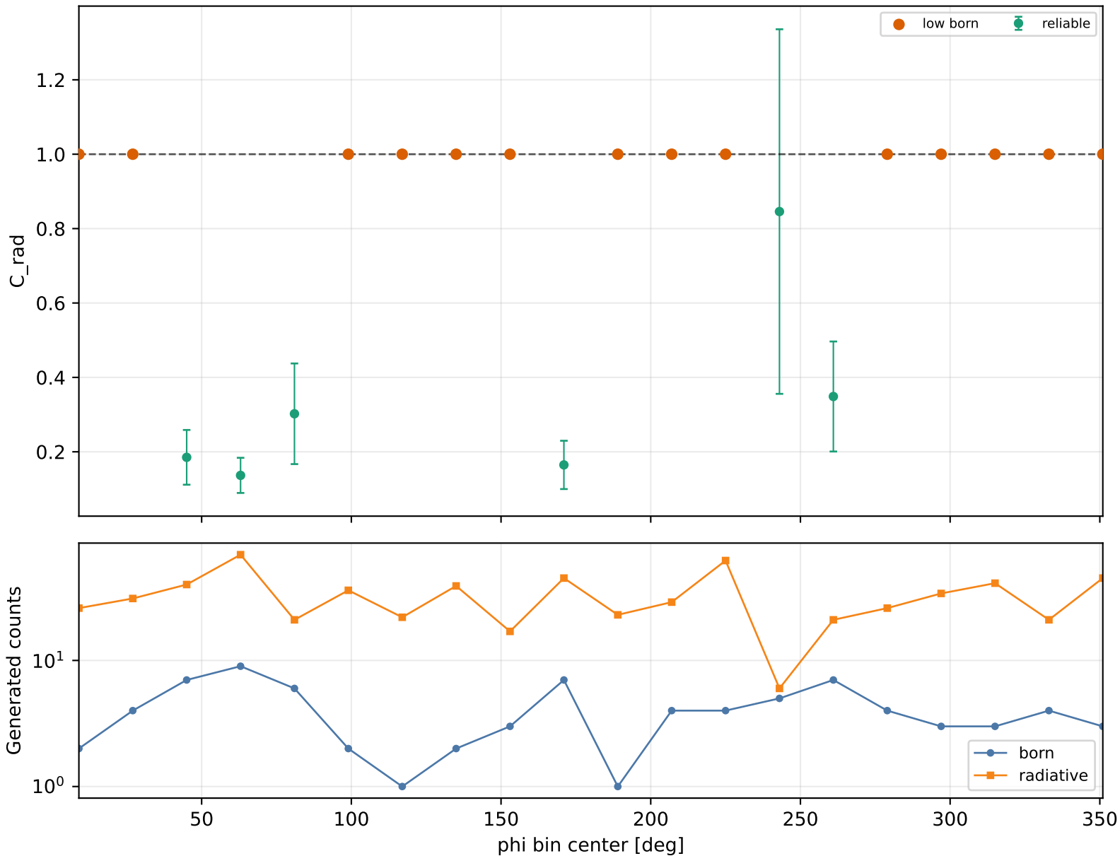
Radiative correction vs phi Q2 1.5-2, xB 0.1-0.15, -t 0.15-0.2
