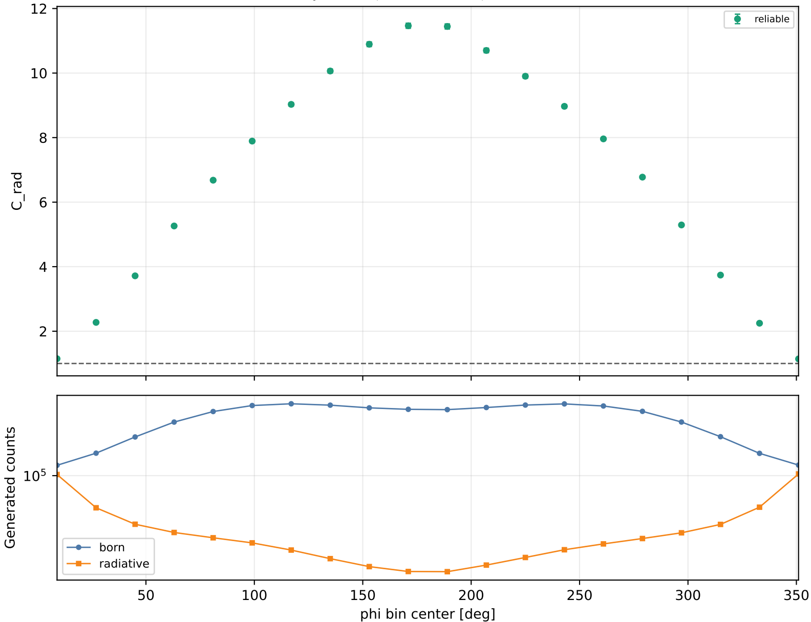
Radiative correction vs phi Q2 1-1.5, xB 0.3-0.38, -t 1-1.5
