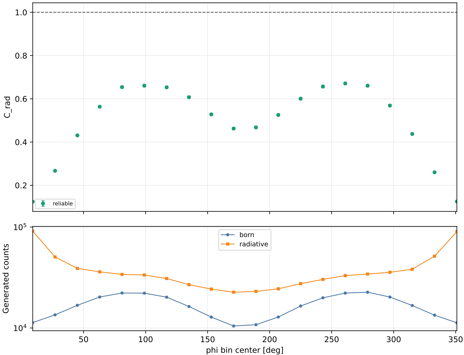
Radiative correction vs phi Q2 1.5-2, xB 0.3-0.38, -t 1-1.5
