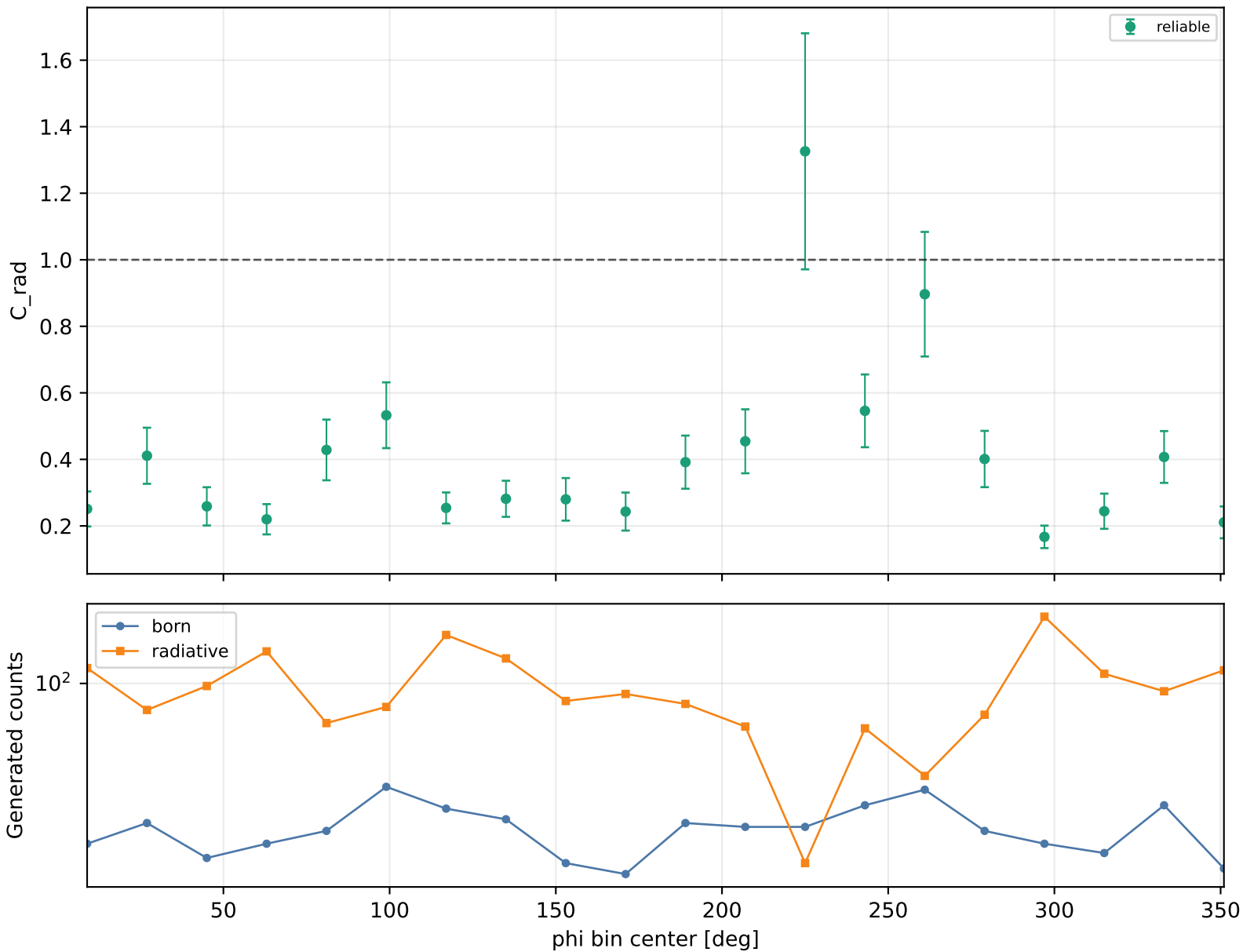
Radiative correction vs phi Q2 4.6-5.5, xB 0.38-0.48, -t 1.5-2
