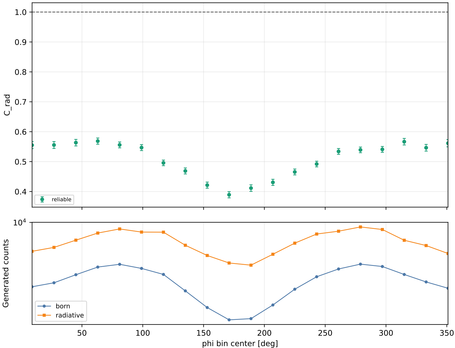
Radiative correction vs phi Q2 2-2.5, xB 0.3-0.38, -t 0.3-0.4
