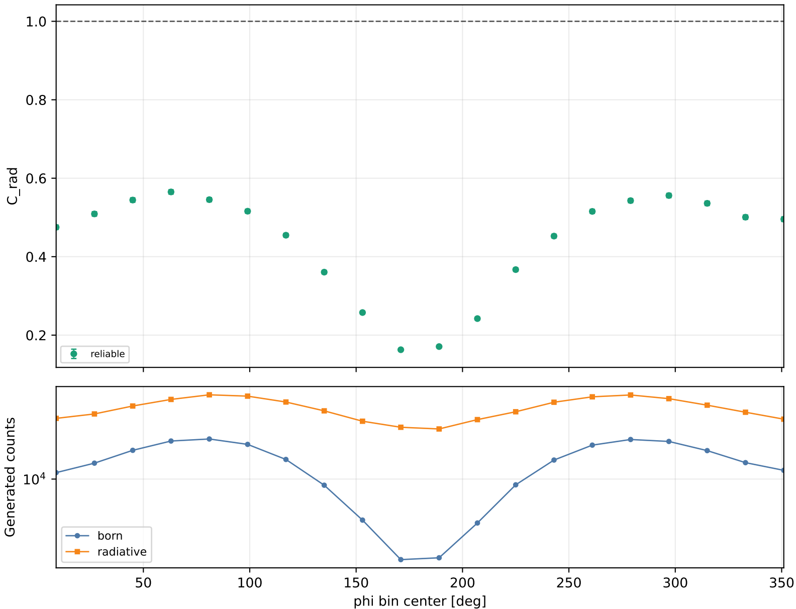
Radiative correction vs phi Q2 1-1.5, xB 0.2-0.25, -t 0.09-0.15
