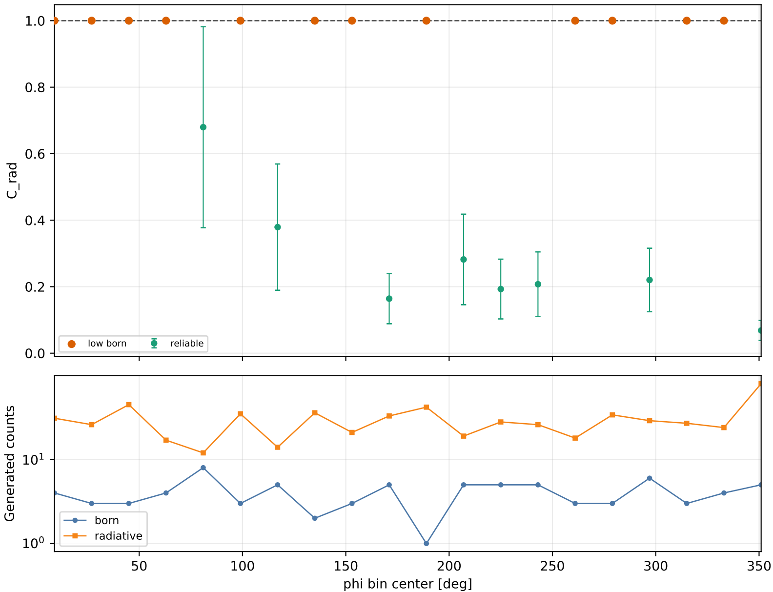
Radiative correction vs phi Q2 2.5-3, xB 0.2-0.25, -t 0.3-0.4
