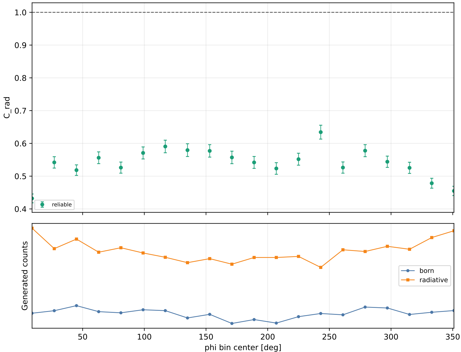
Radiative correction vs phi Q2 1.5-2, xB 0.15-0.2, -t 1-1.5
