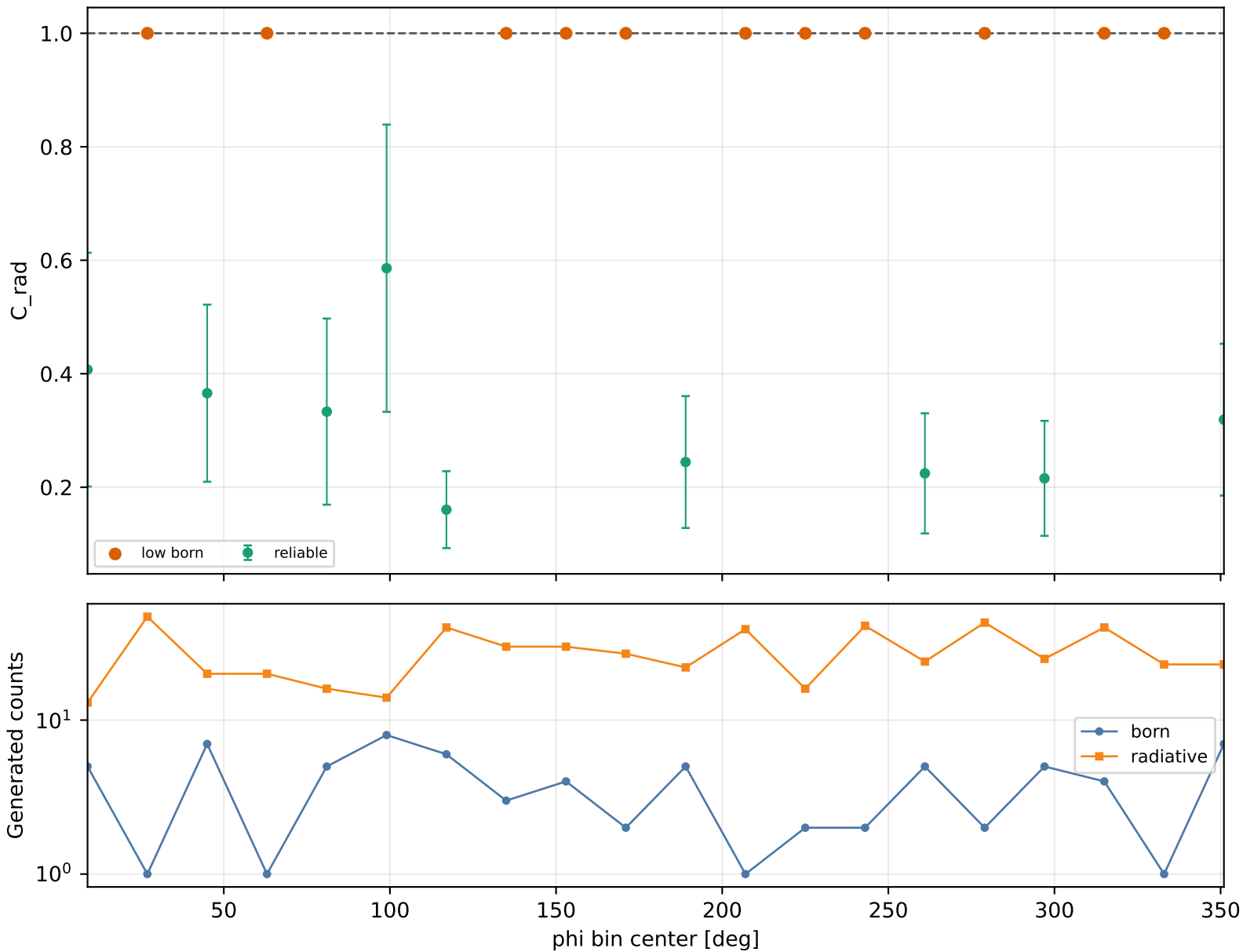
Radiative correction vs phi Q2 1-1.5, xB 0.05-0.1, -t 1-1.5
