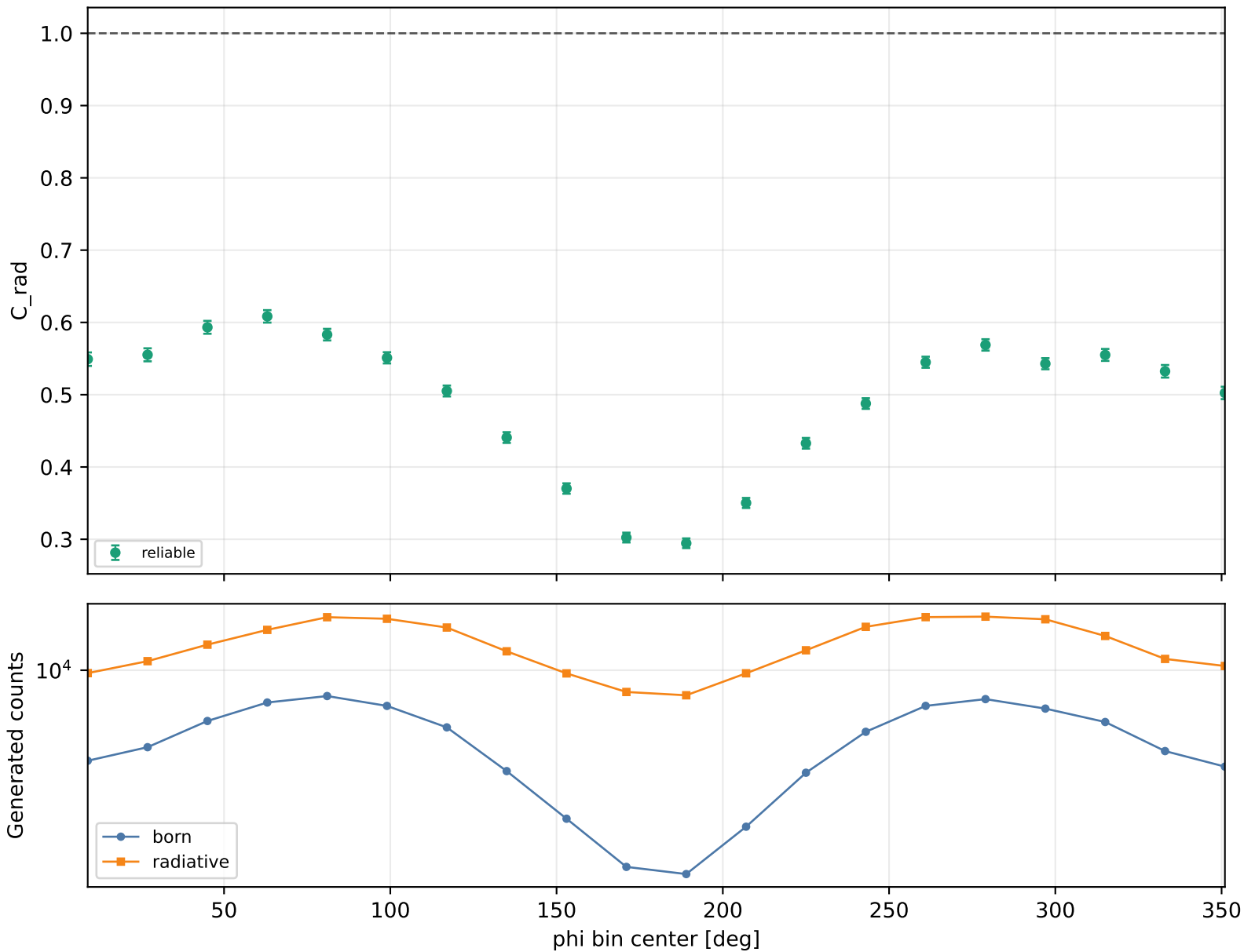
Radiative correction vs phi Q2 1.5-2, xB 0.25-0.3, -t 0.2-0.3
