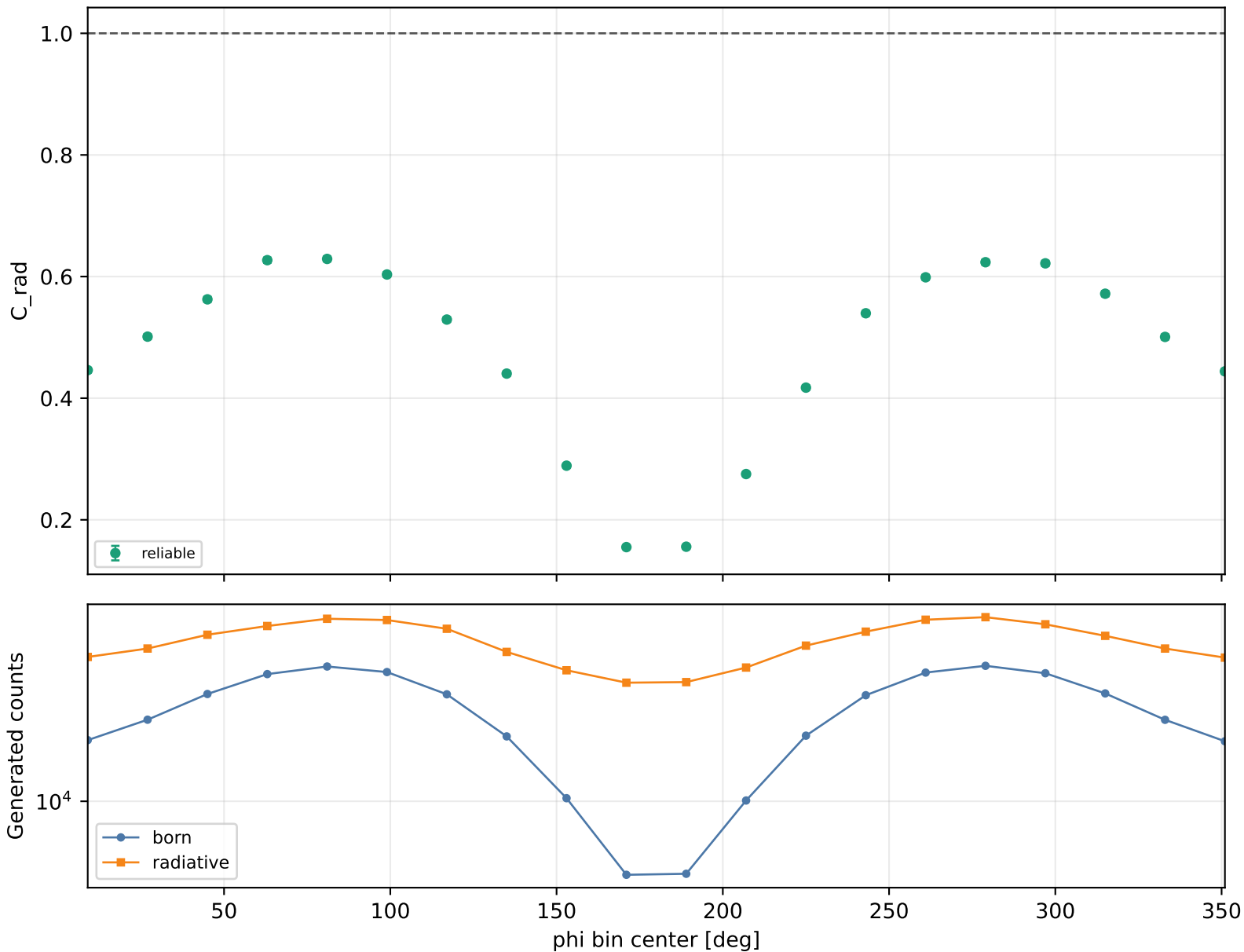
Radiative correction vs phi Q2 1-1.5, xB 0.2-0.25, -t 0.2-0.3
