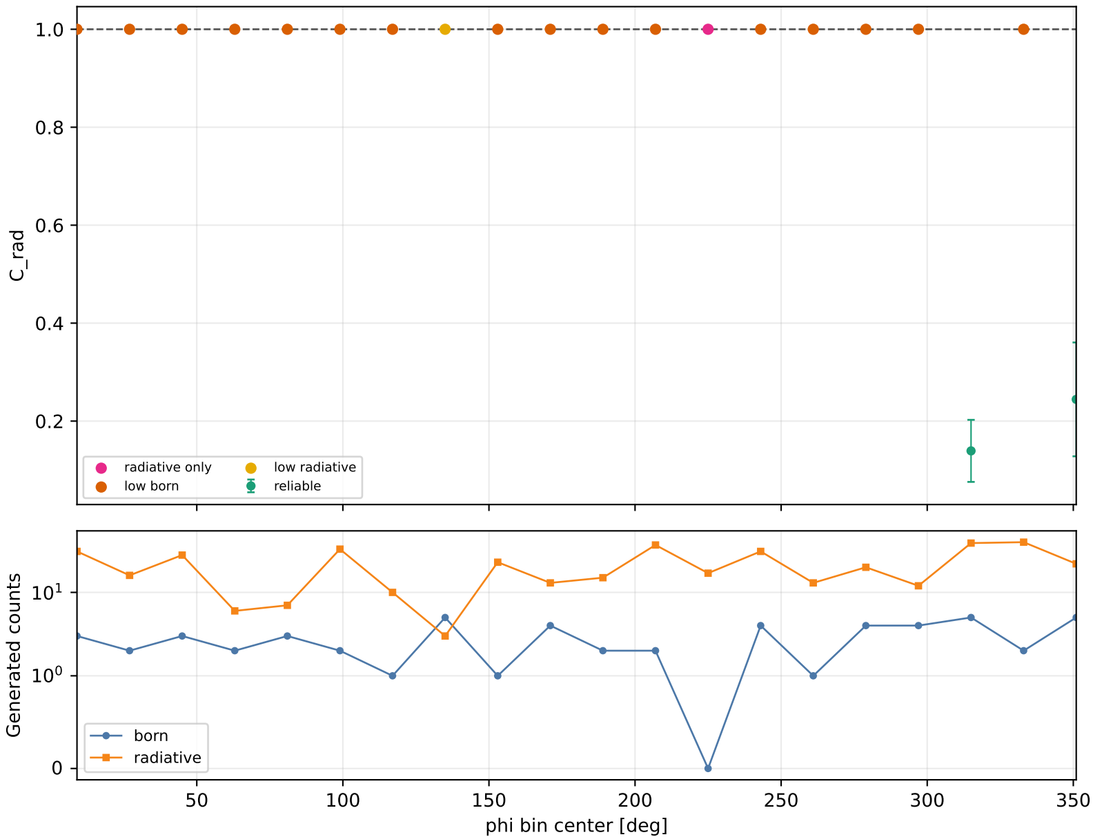
Radiative correction vs phi Q2 2.5-3, xB 0.2-0.25, -t 0.15-0.2
