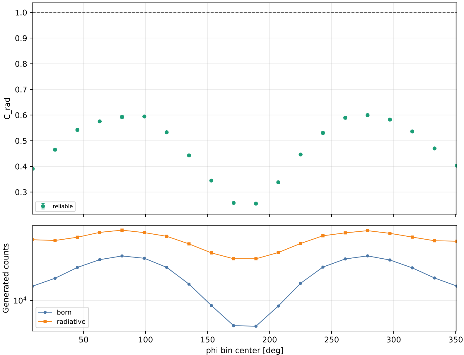
Radiative correction vs phi Q2 1-1.5, xB 0.15-0.2, -t 0.2-0.3
