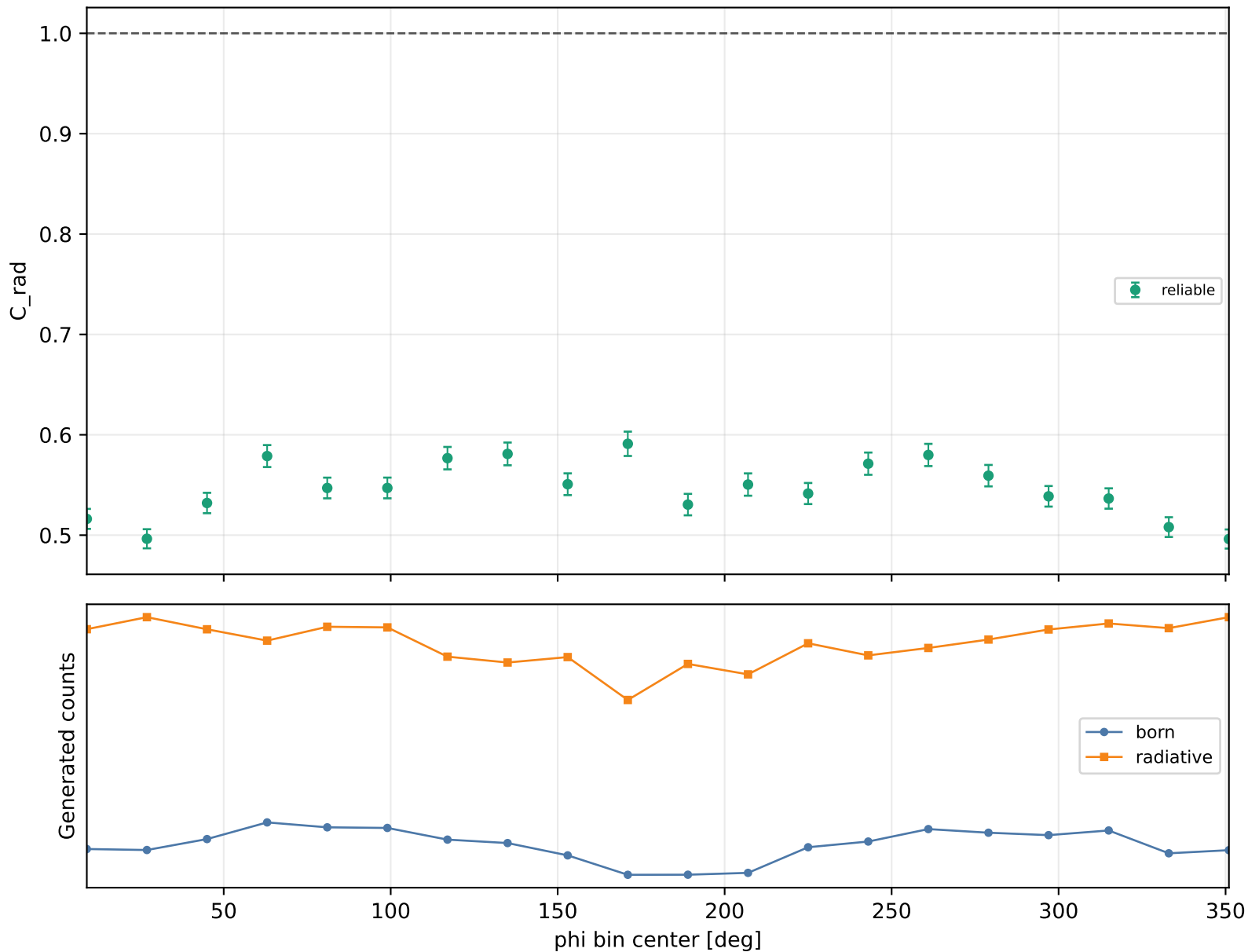
Radiative correction vs phi Q2 3-3.5, xB 0.58-0.7, -t 1-1.5
