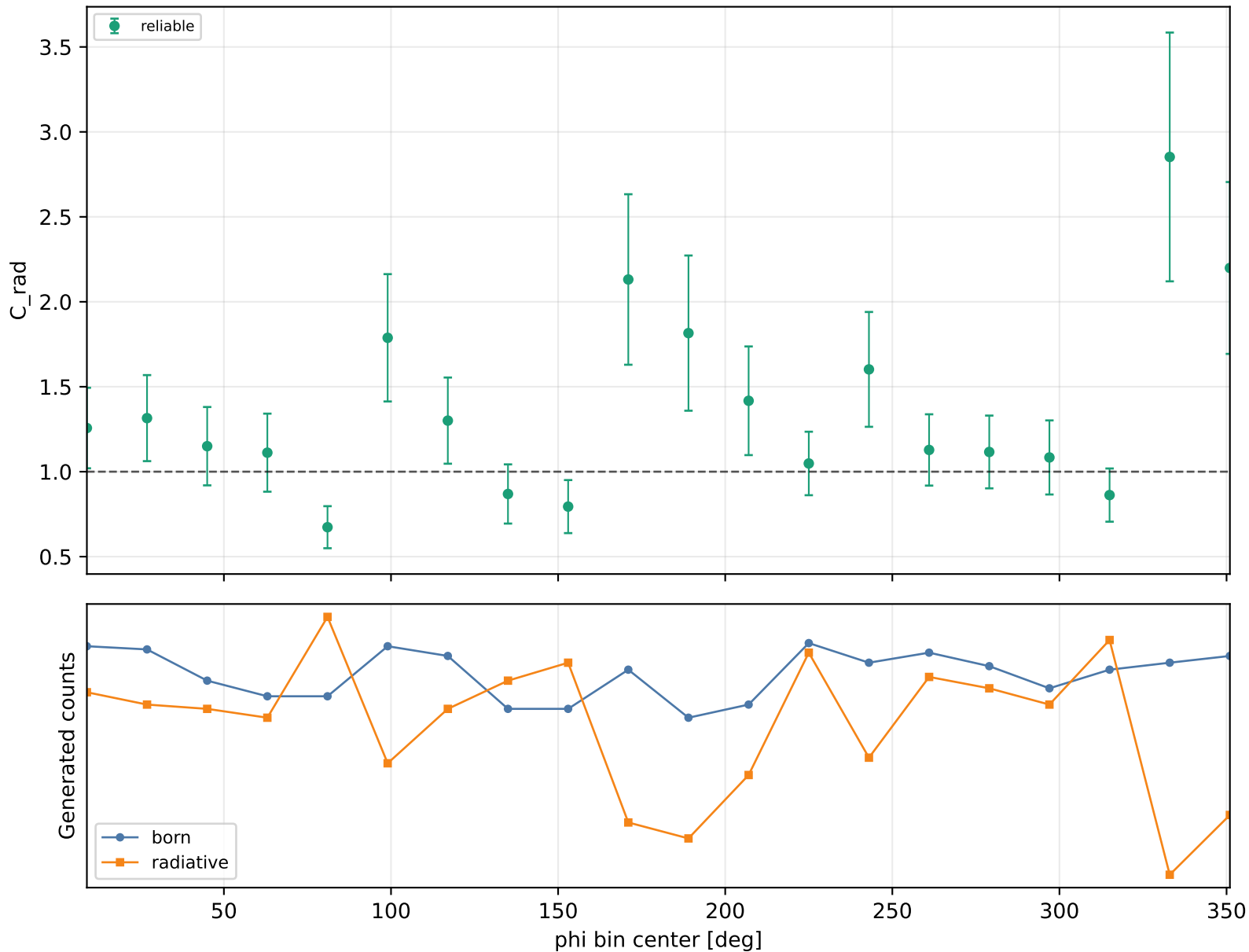
Radiative correction vs phi Q2 3.5-4, xB 0.48-0.58, -t 0.3-0.4
