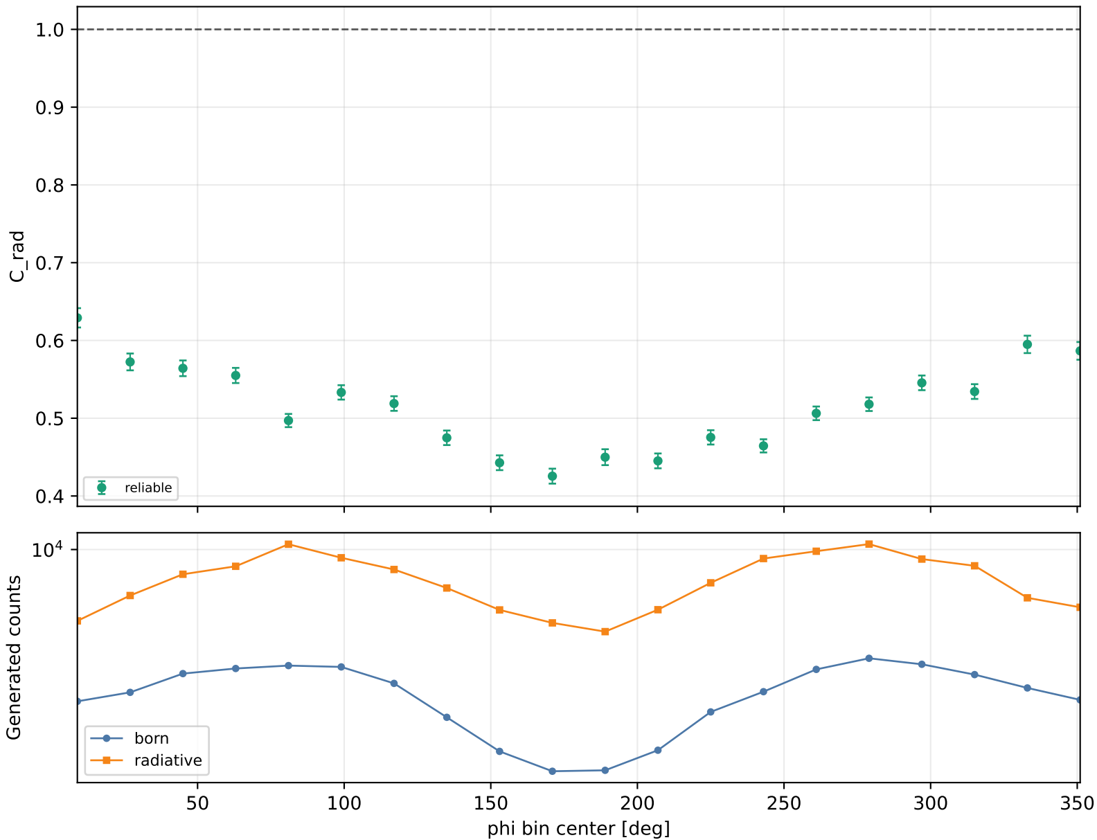
Radiative correction vs phi Q2 2-2.5, xB 0.38-0.48, -t 0.3-0.4
