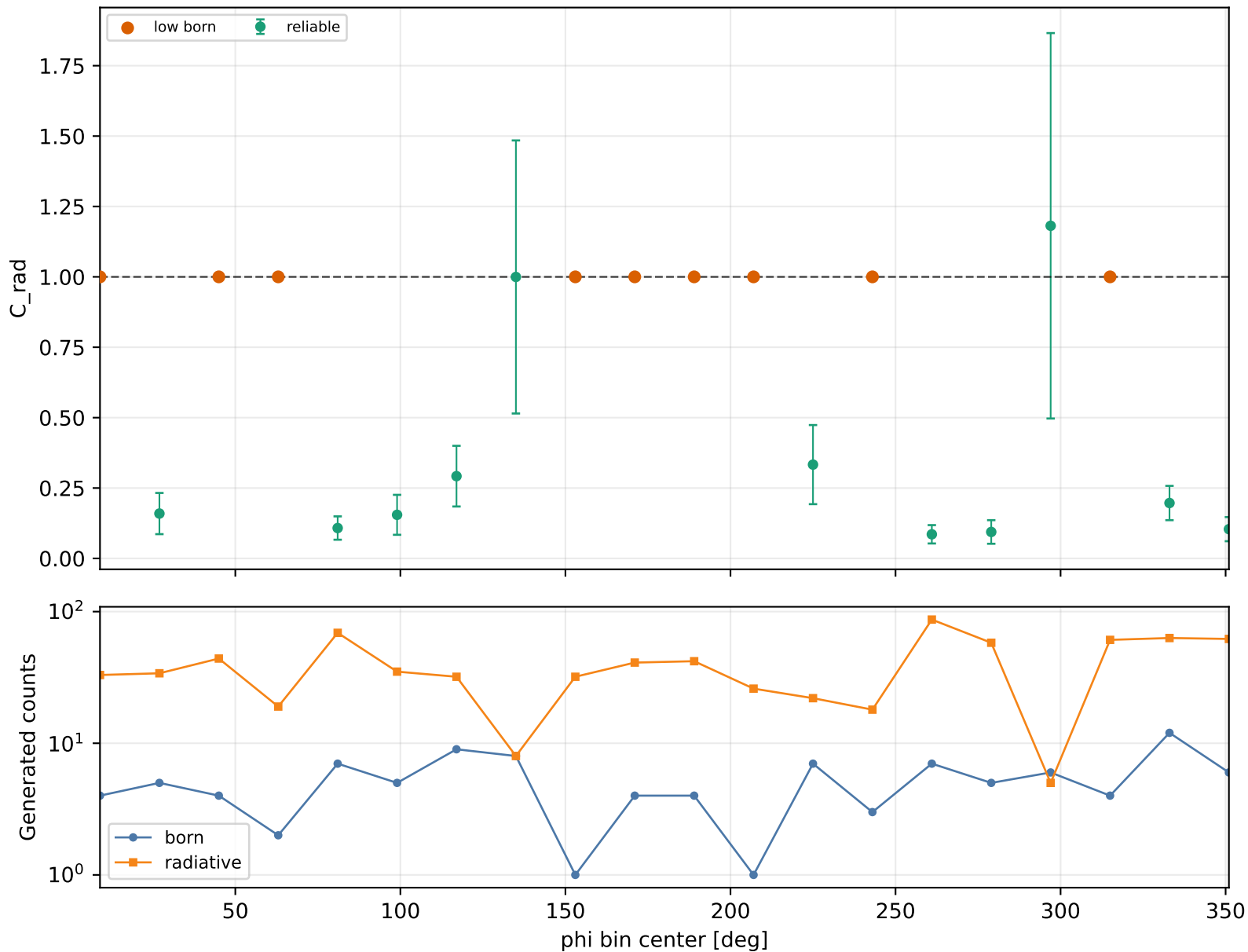
Radiative correction vs phi Q2 1.5-2, xB 0.1-0.15, -t 0.09-0.15
