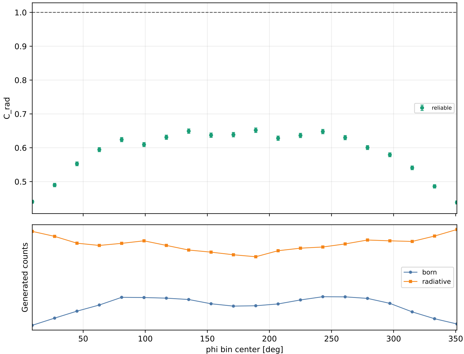
Radiative correction vs phi Q2 2.5-3, xB 0.58-0.7, -t 1.5-2
