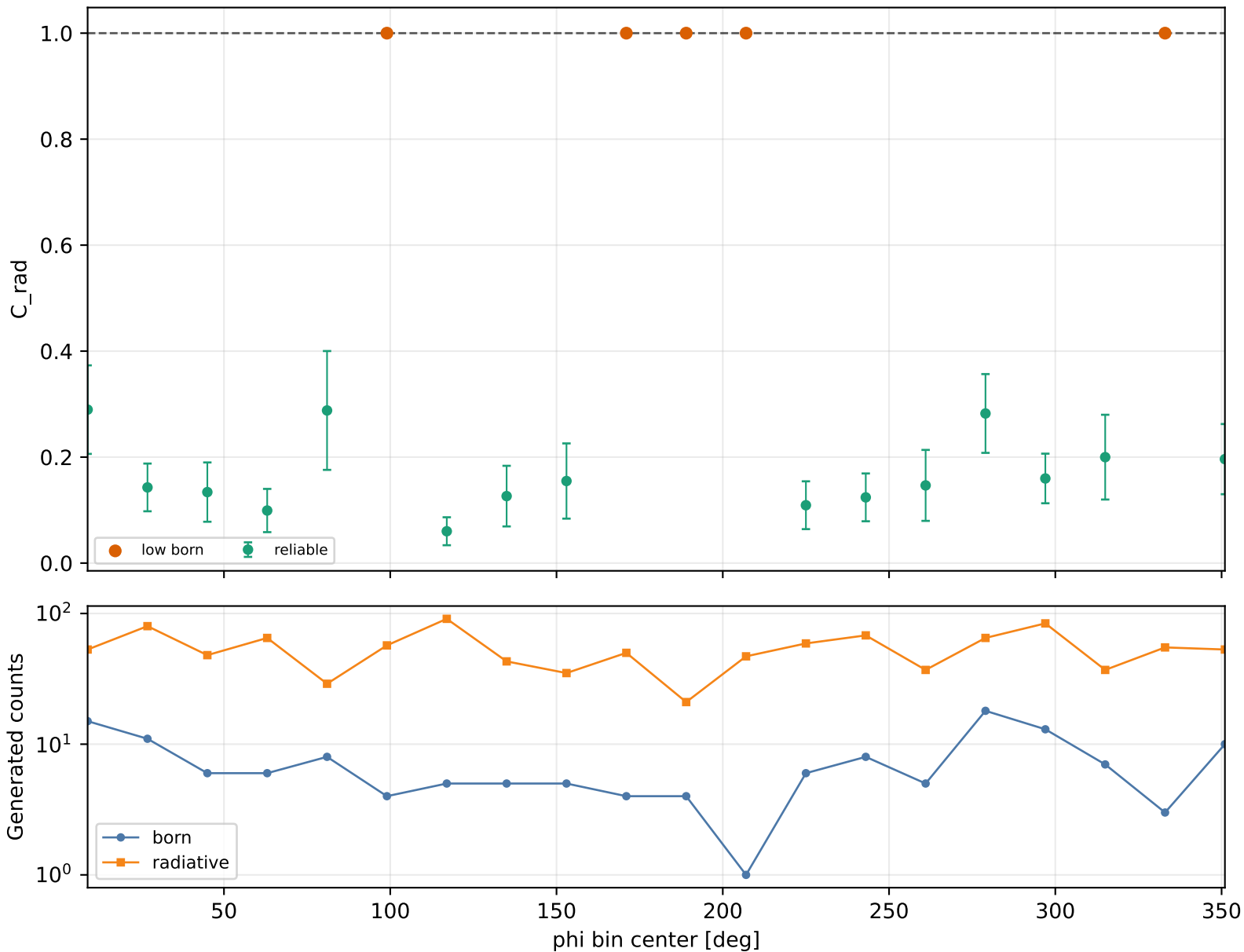
Radiative correction vs phi Q2 2-2.5, xB 0.15-0.2, -t 0.2-0.3
