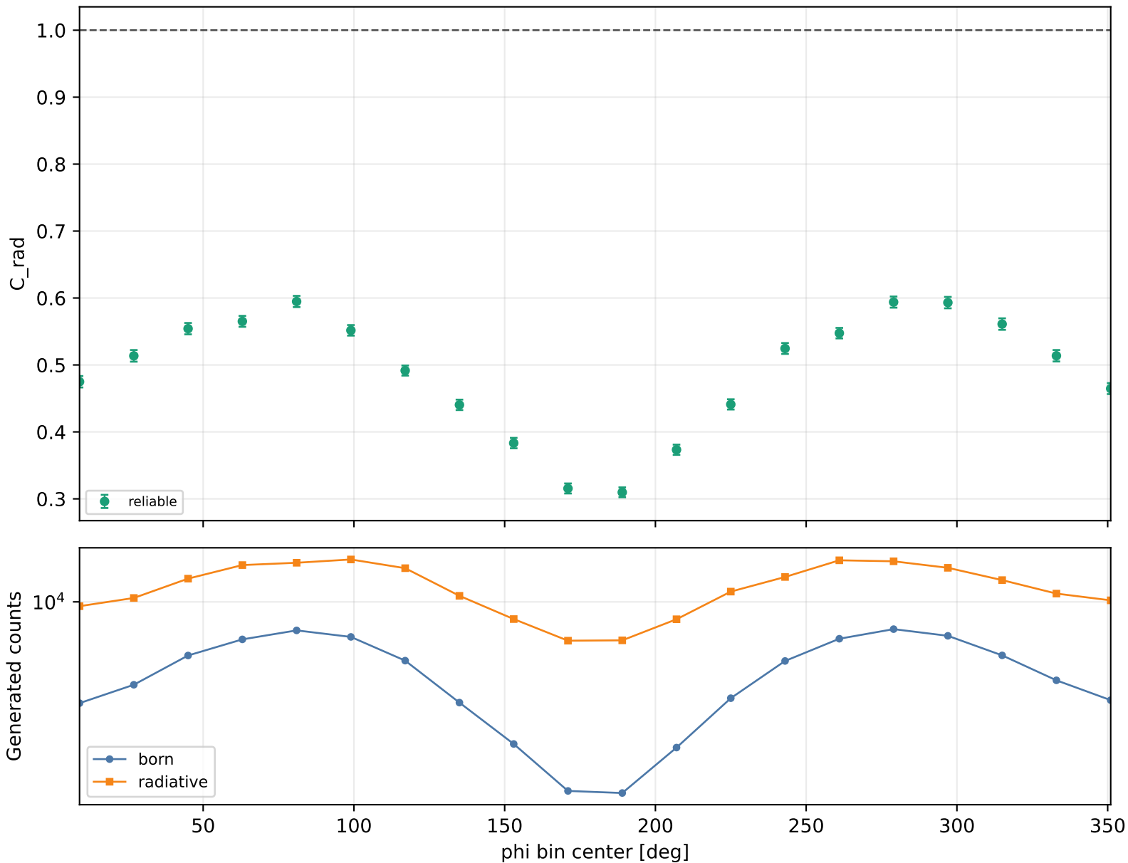
Radiative correction vs phi Q2 1.5-2, xB 0.25-0.3, -t 0.3-0.4
