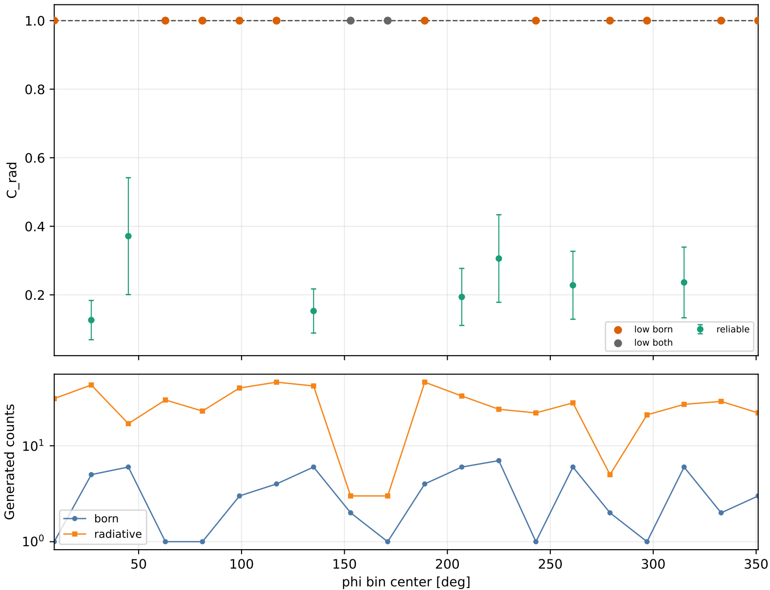
Radiative correction vs phi Q2 2-2.5, xB 0.15-0.2, -t 0.15-0.2
