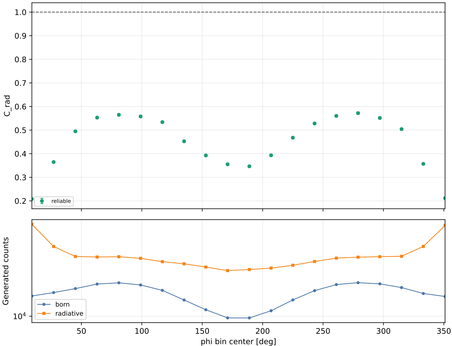
Radiative correction vs phi Q2 1-1.5, xB 0.15-0.2, -t 0.6-1
