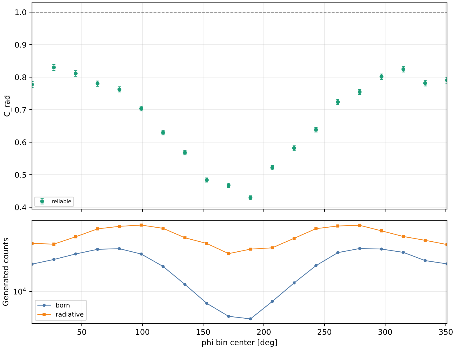
Radiative correction vs phi Q2 1-1.5, xB 0.25-0.3, -t 0.09-0.15
