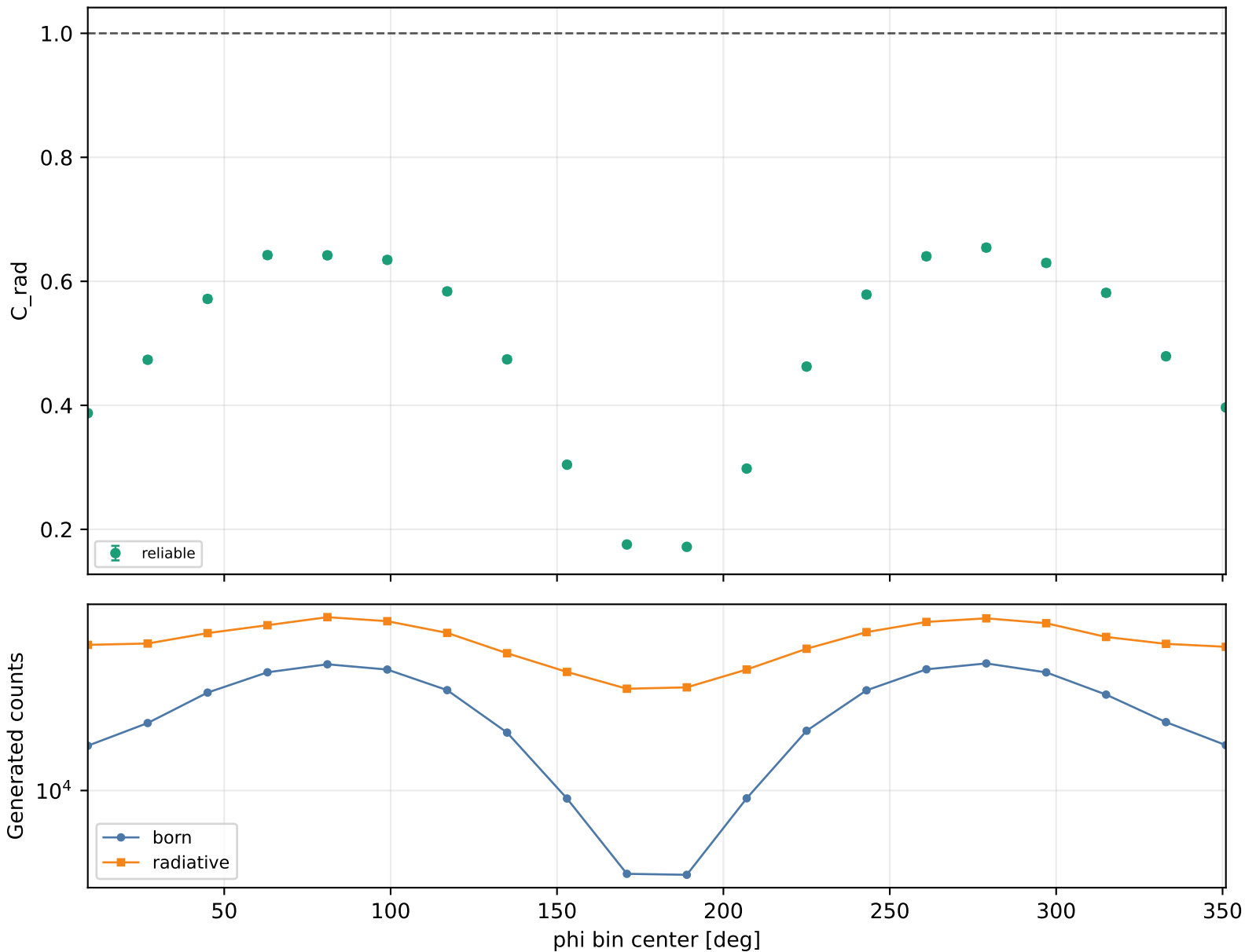
Radiative correction vs phi Q2 1-1.5, xB 0.2-0.25, -t 0.3-0.4
