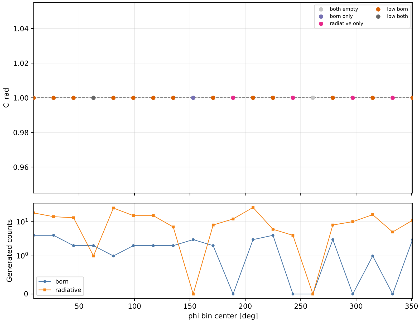
Radiative correction vs phi Q2 2-2.5, xB 0.15-0.2, -t 1.5-2
