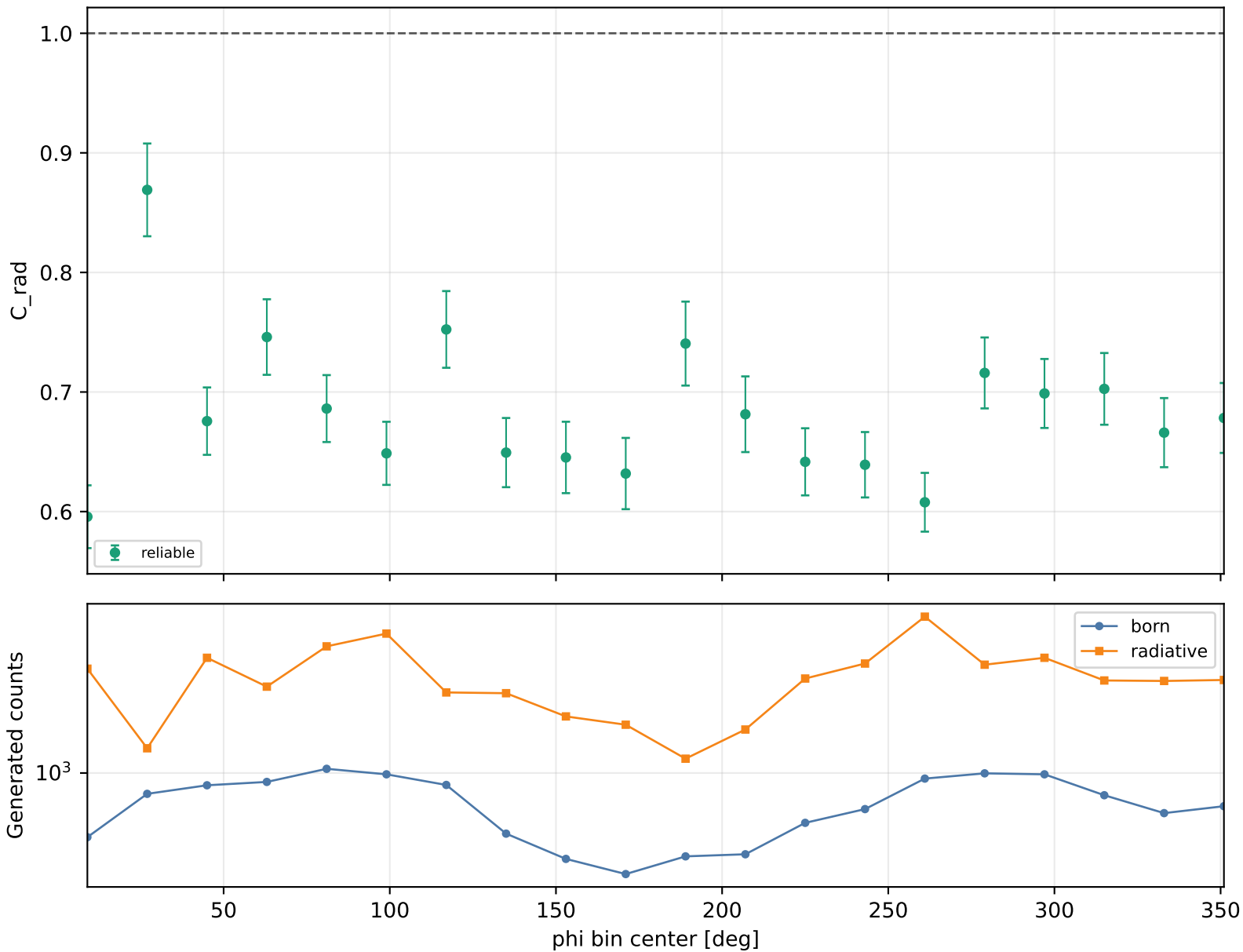
Radiative correction vs phi Q2 3.5-4, xB 0.48-0.58, -t 0.4-0.6
