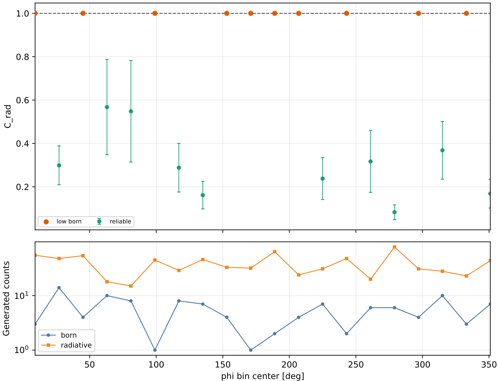
Radiative correction vs phi Q2 2.5-3, xB 0.2-0.25, -t 0.2-0.3
