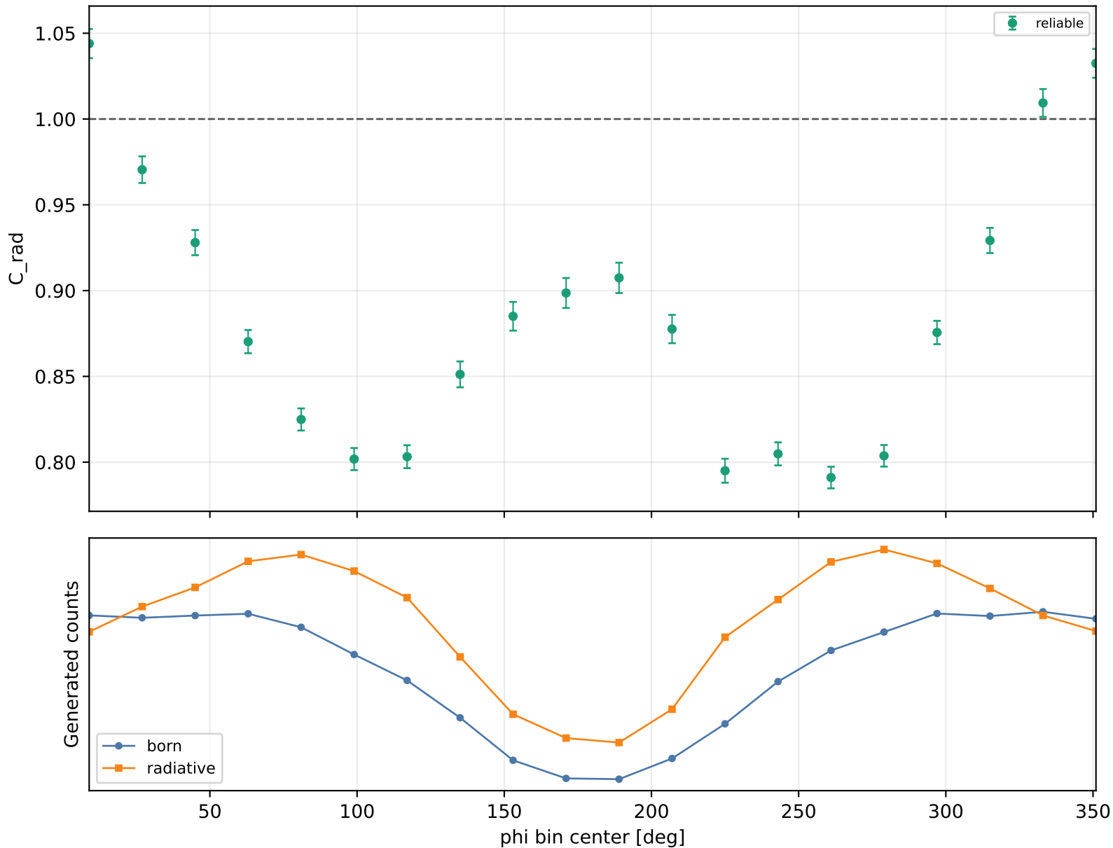
Radiative correction vs phi Q2 1.5-2, xB 0.38-0.48, -t 0.4-0.6
