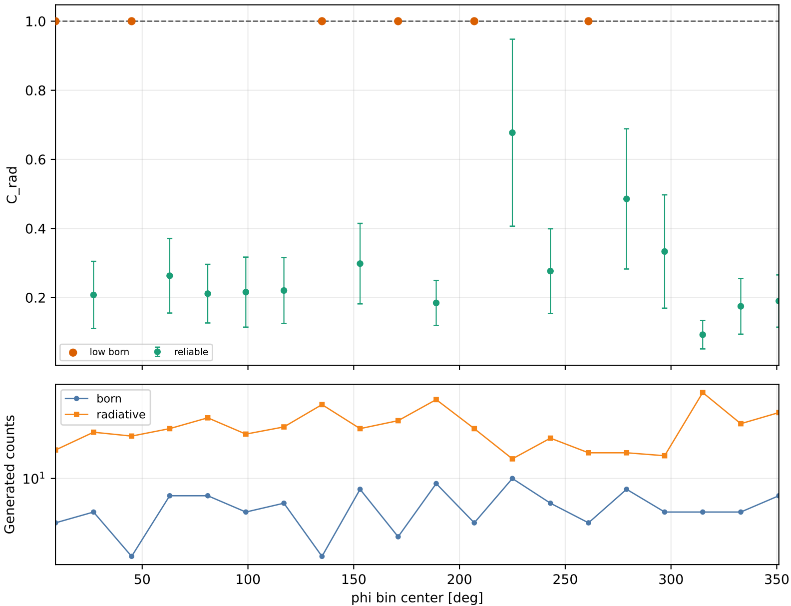
Radiative correction vs phi Q2 3-3.5, xB 0.25-0.3, -t 1-1.5
