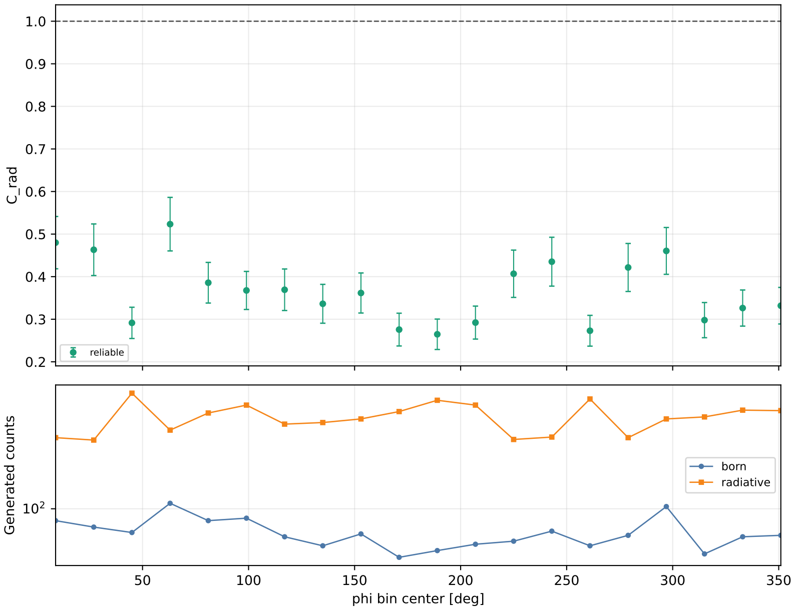
Radiative correction vs phi Q2 4.6-5.5, xB 0.38-0.48, -t 0.6-1
