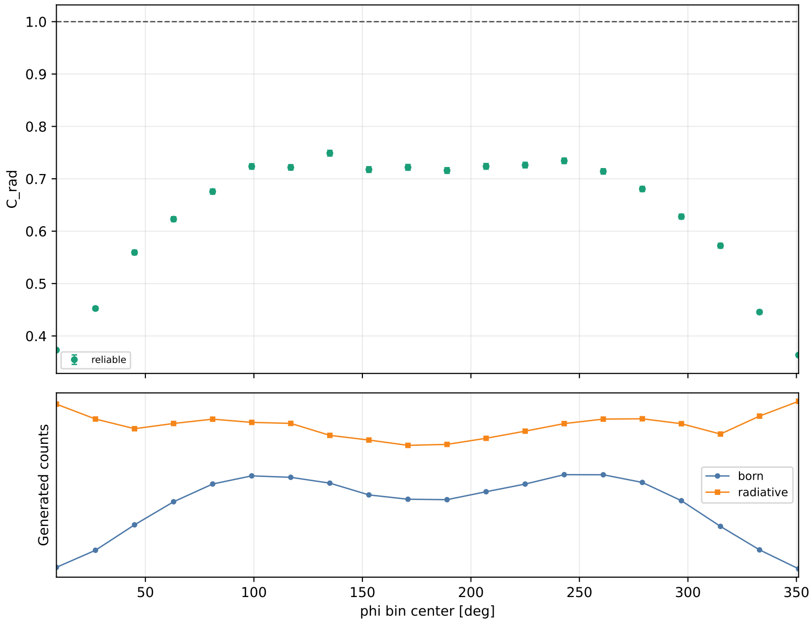
Radiative correction vs phi Q2 2-2.5, xB 0.48-0.58, -t 1.5-2
