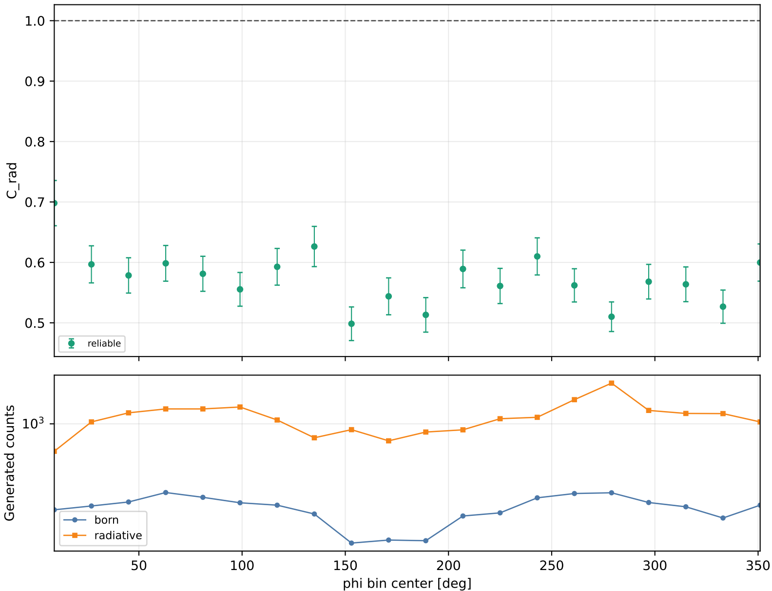
Radiative correction vs phi Q2 4-4.6, xB 0.38-0.48, -t 0.4-0.6
