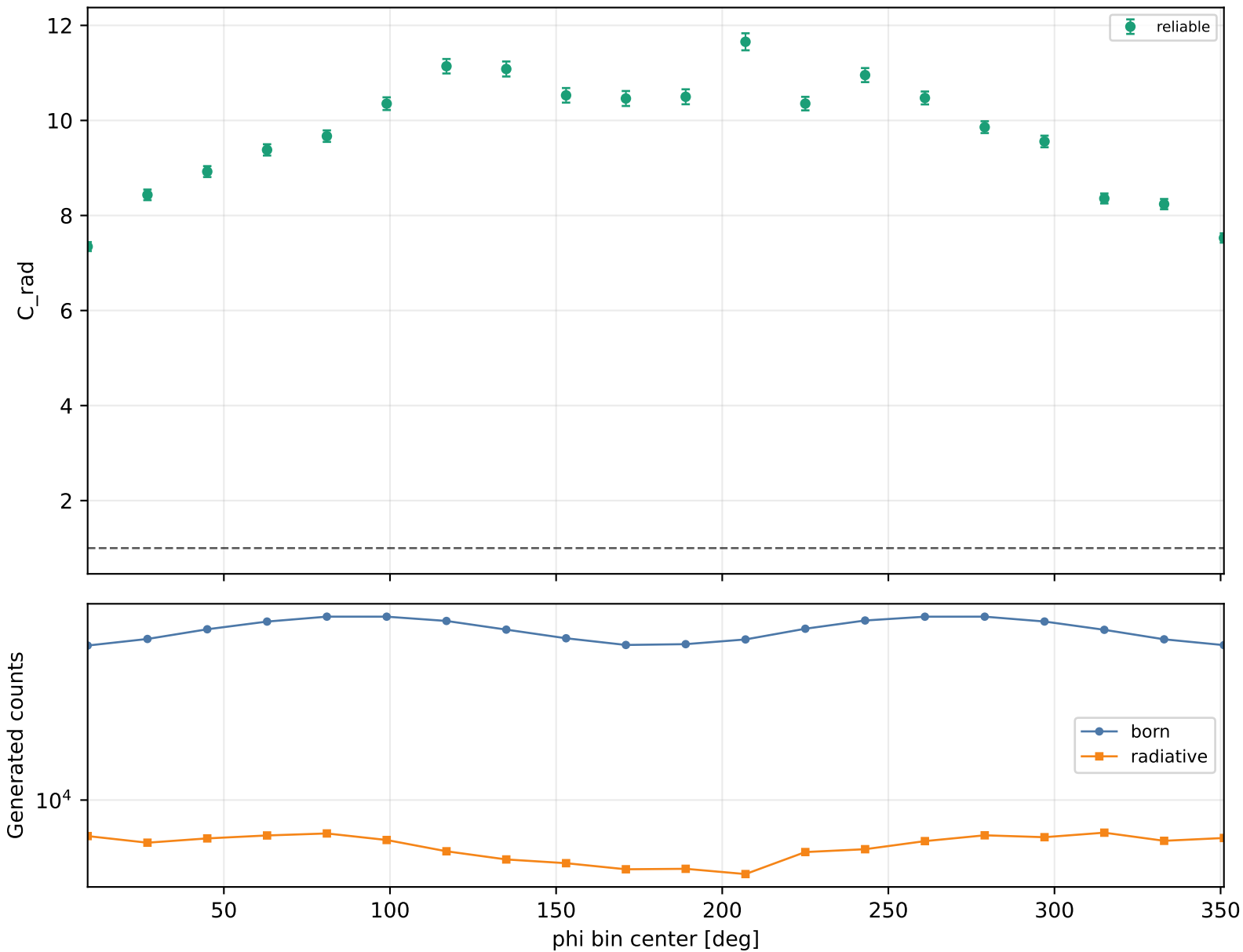
Radiative correction vs phi Q2 1.5-2, xB 0.48-0.58, -t 0.6-1
