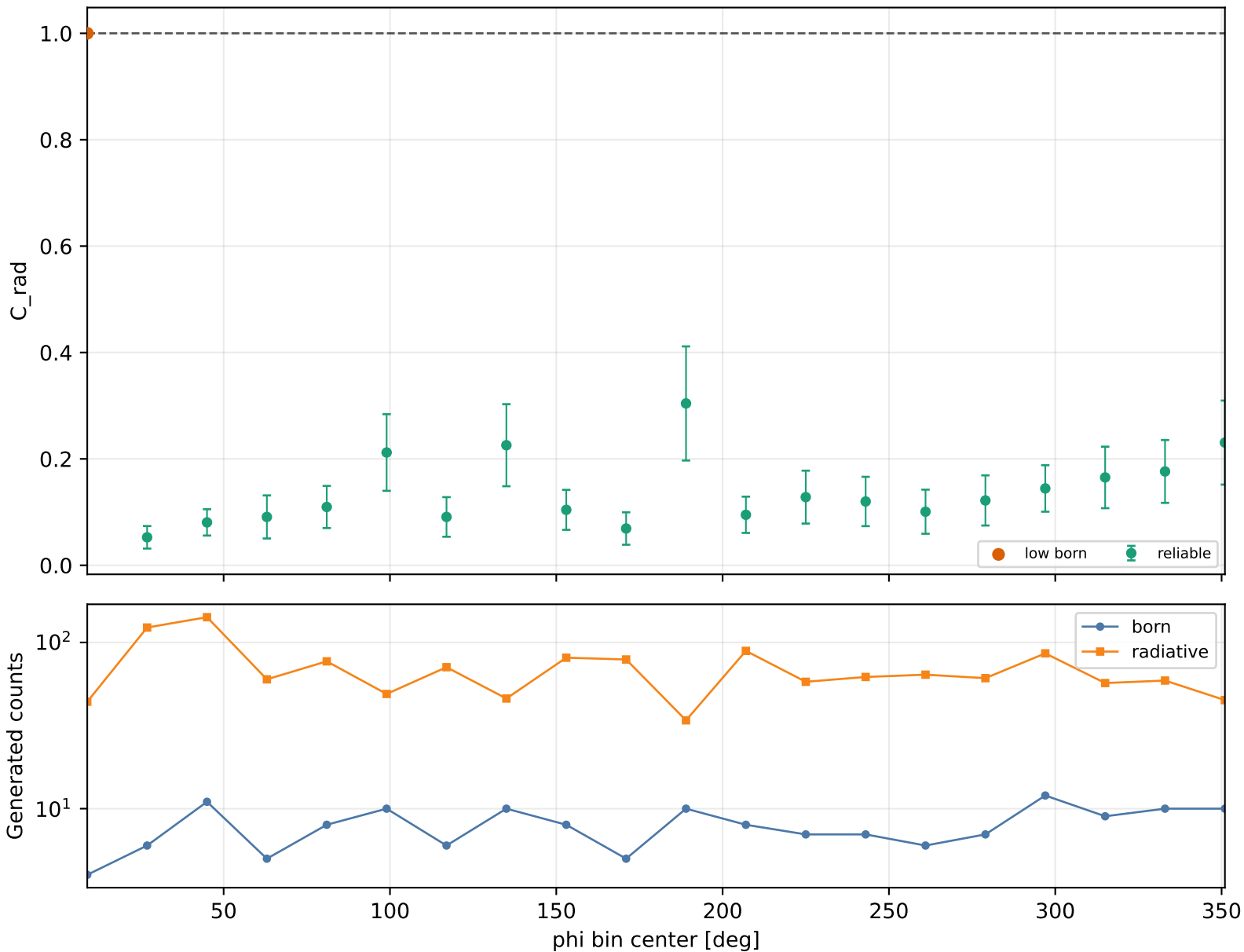
Radiative correction vs phi Q2 1.5-2, xB 0.1-0.15, -t 0.2-0.3
