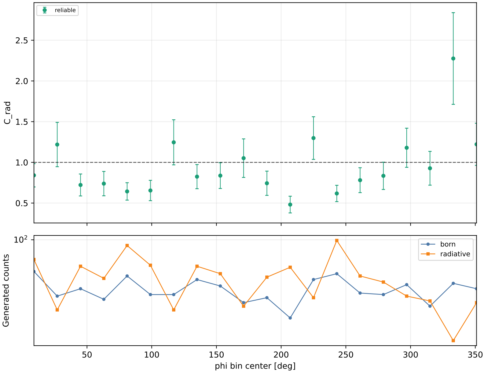
Radiative correction vs phi Q2 3-3.5, xB 0.3-0.38, -t 0.09-0.15
