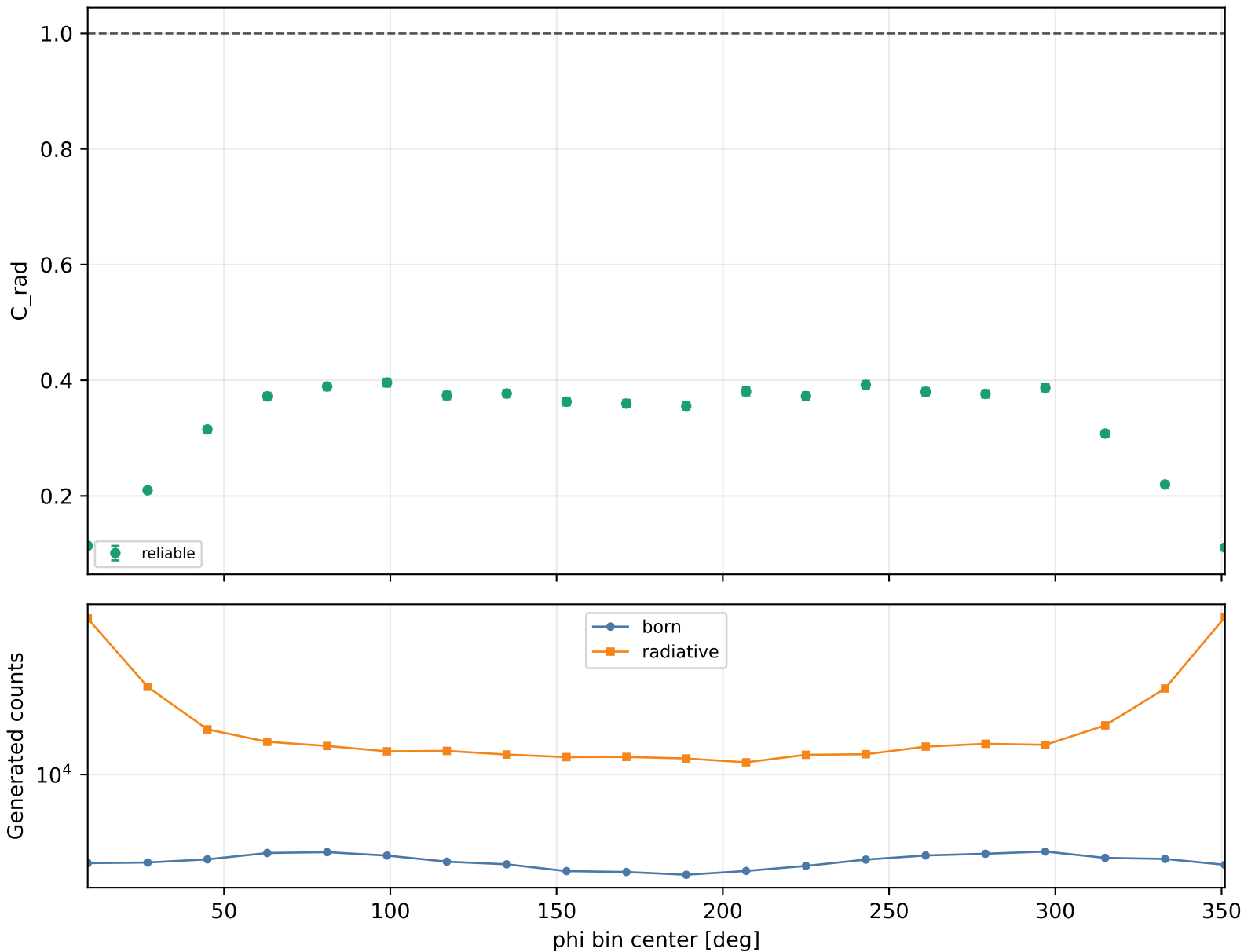
Radiative correction vs phi Q2 1-1.5, xB 0.2-0.25, -t 1.5-2
