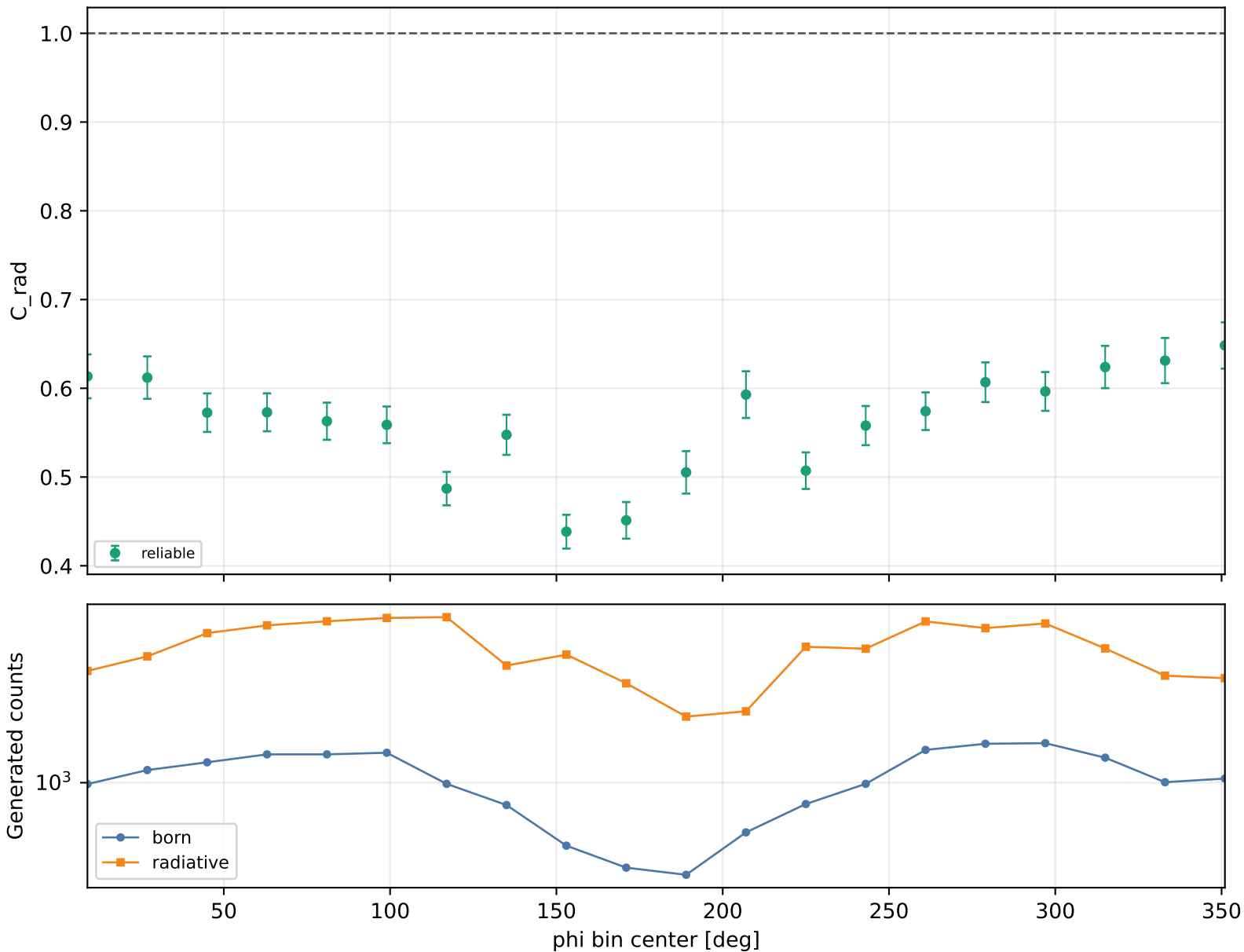
Radiative correction vs phi Q2 2-2.5, xB 0.25-0.3, -t 0.15-0.2
