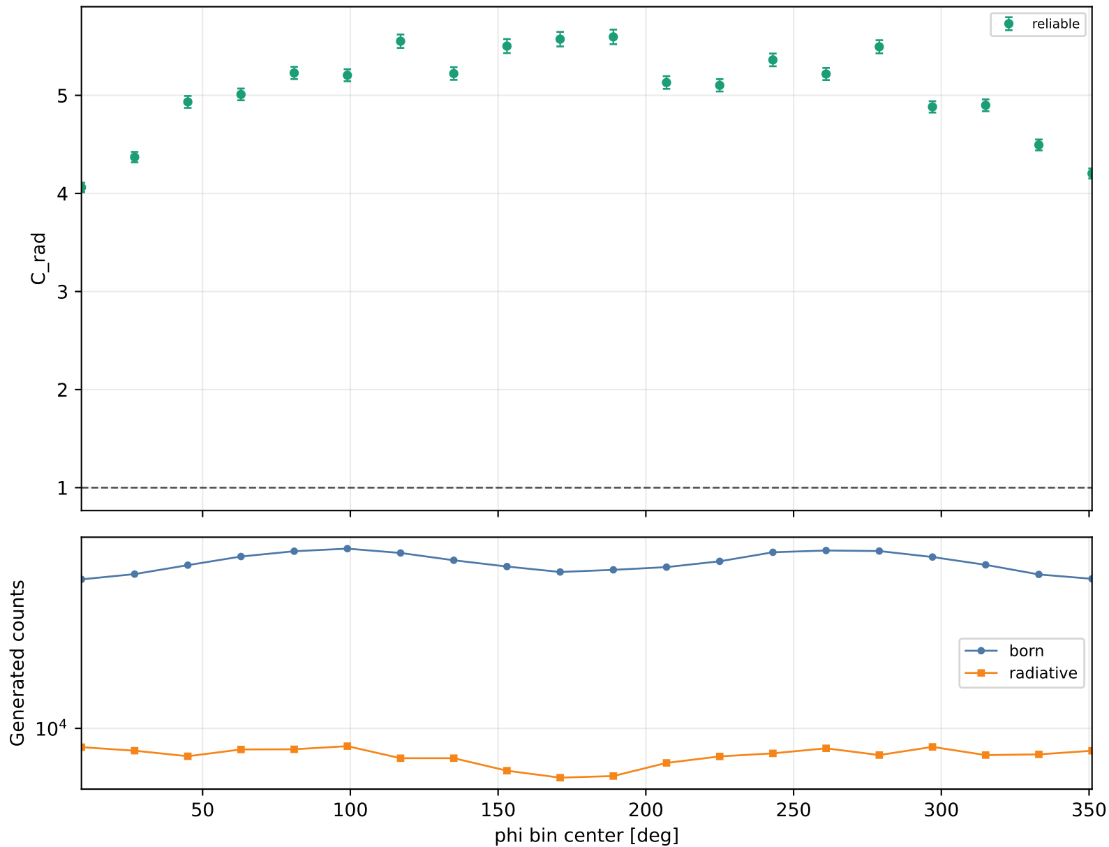
Radiative correction vs phi Q2 2-2.5, xB 0.58-0.7, -t 1-1.5
