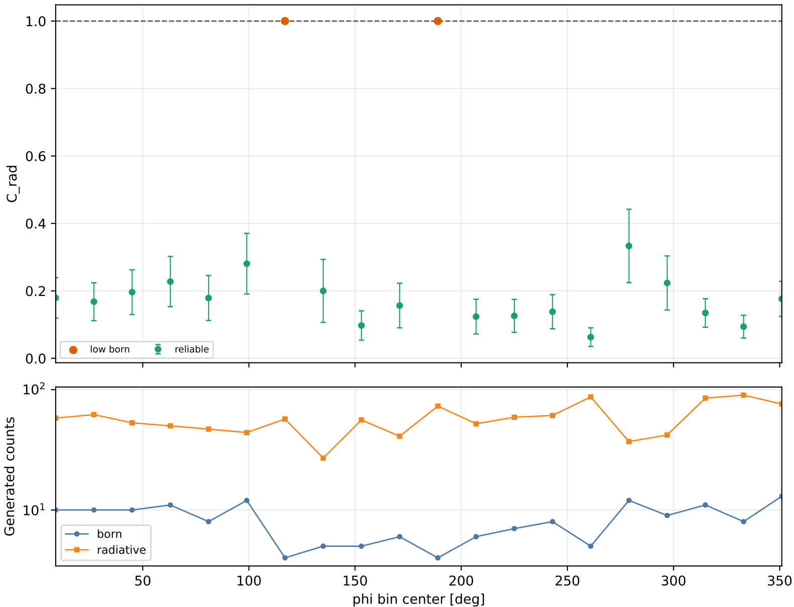
Radiative correction vs phi Q2 1-1.5, xB 0.05-0.1, -t 0.3-0.4
