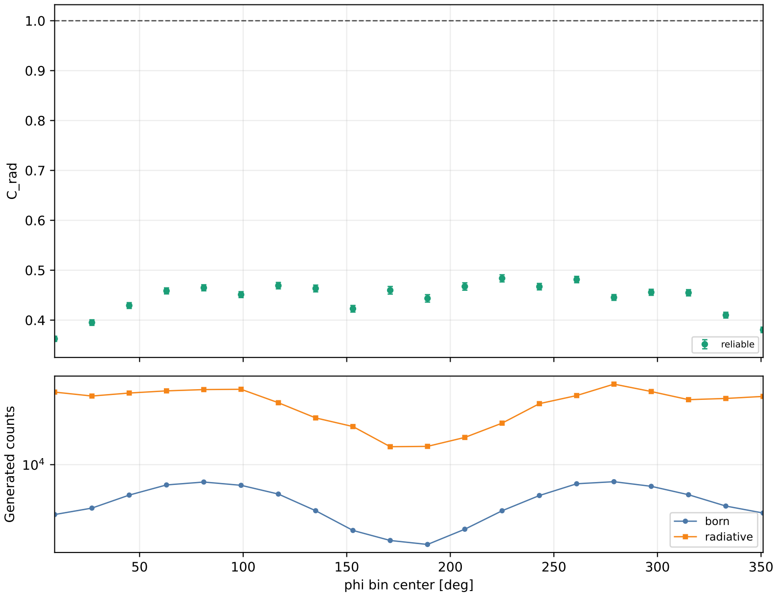
Radiative correction vs phi Q2 2.5-3, xB 0.48-0.58, -t 1-1.5
