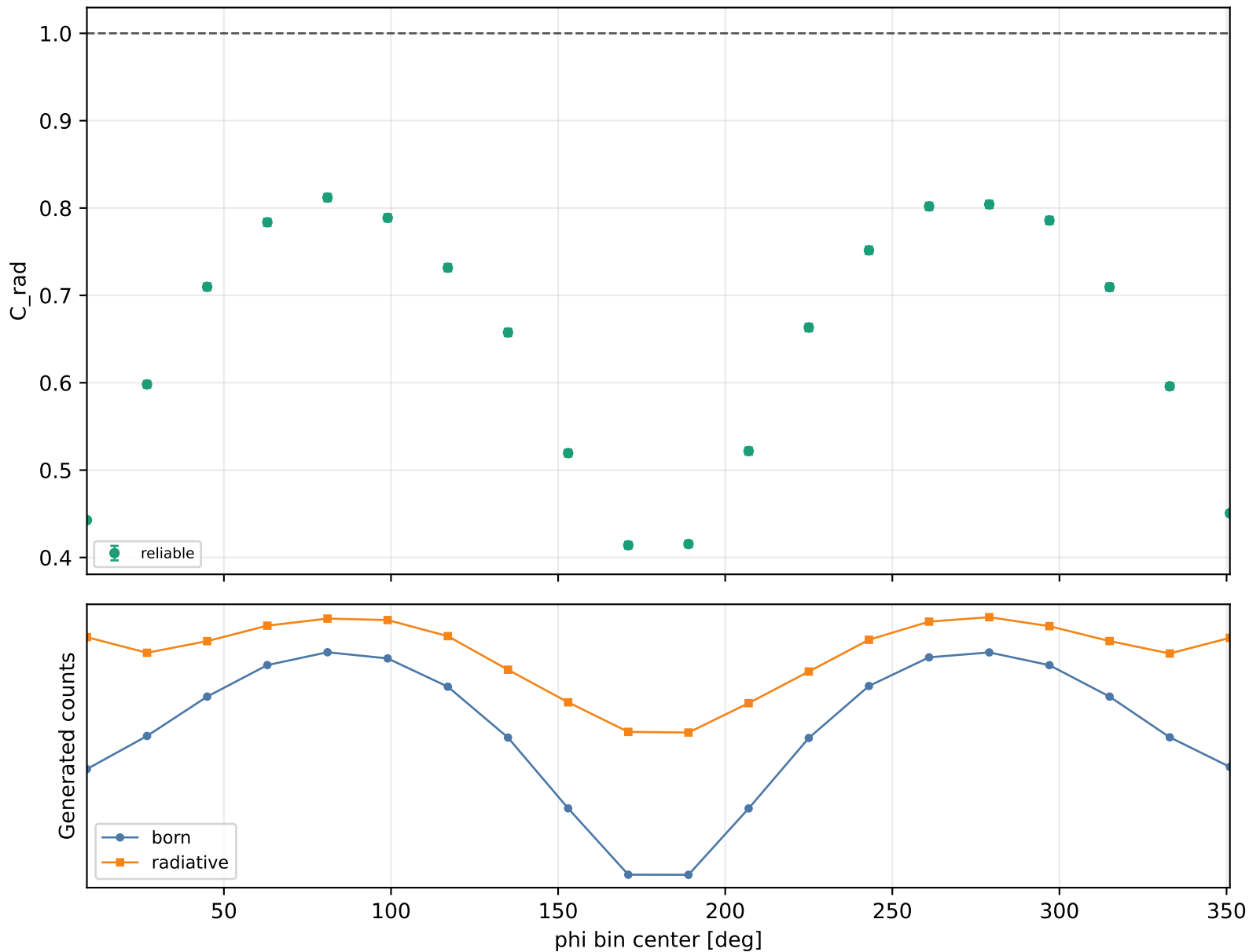
Radiative correction vs phi Q2 1-1.5, xB 0.25-0.3, -t 0.4-0.6
