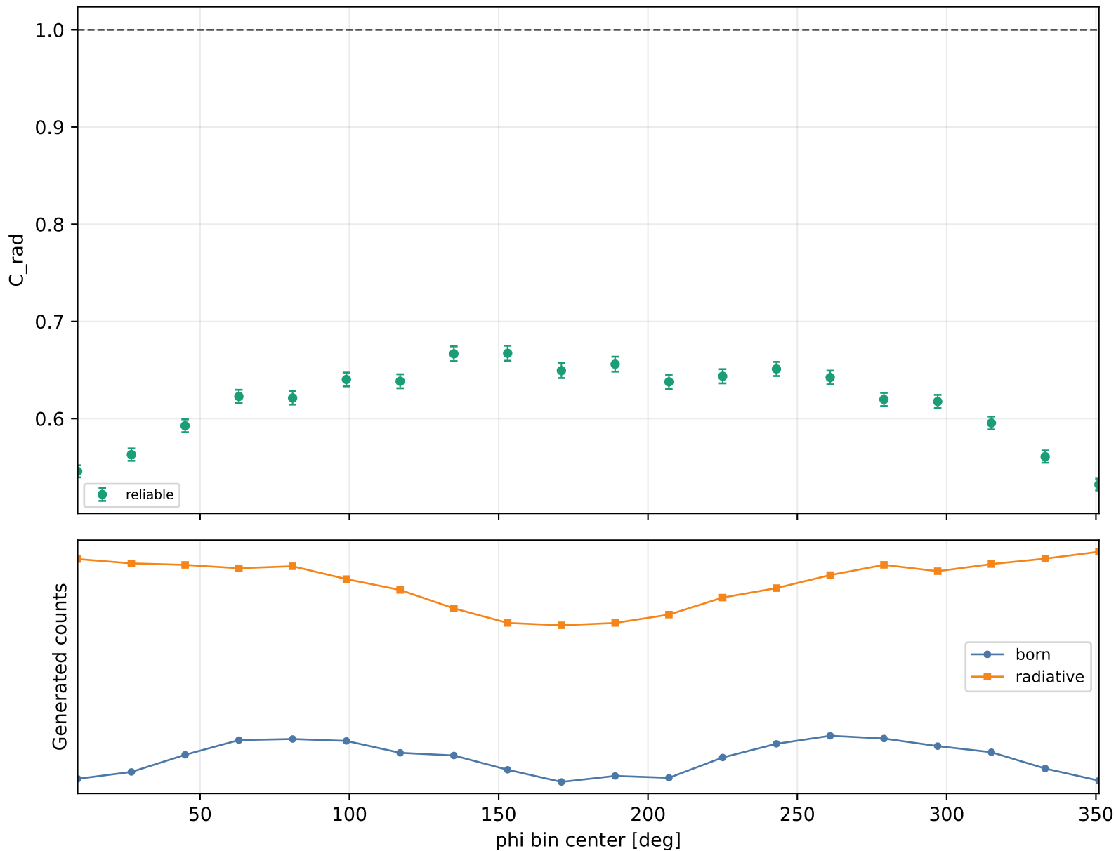
Radiative correction vs phi Q2 2.5-3, xB 0.58-0.7, -t 1-1.5
