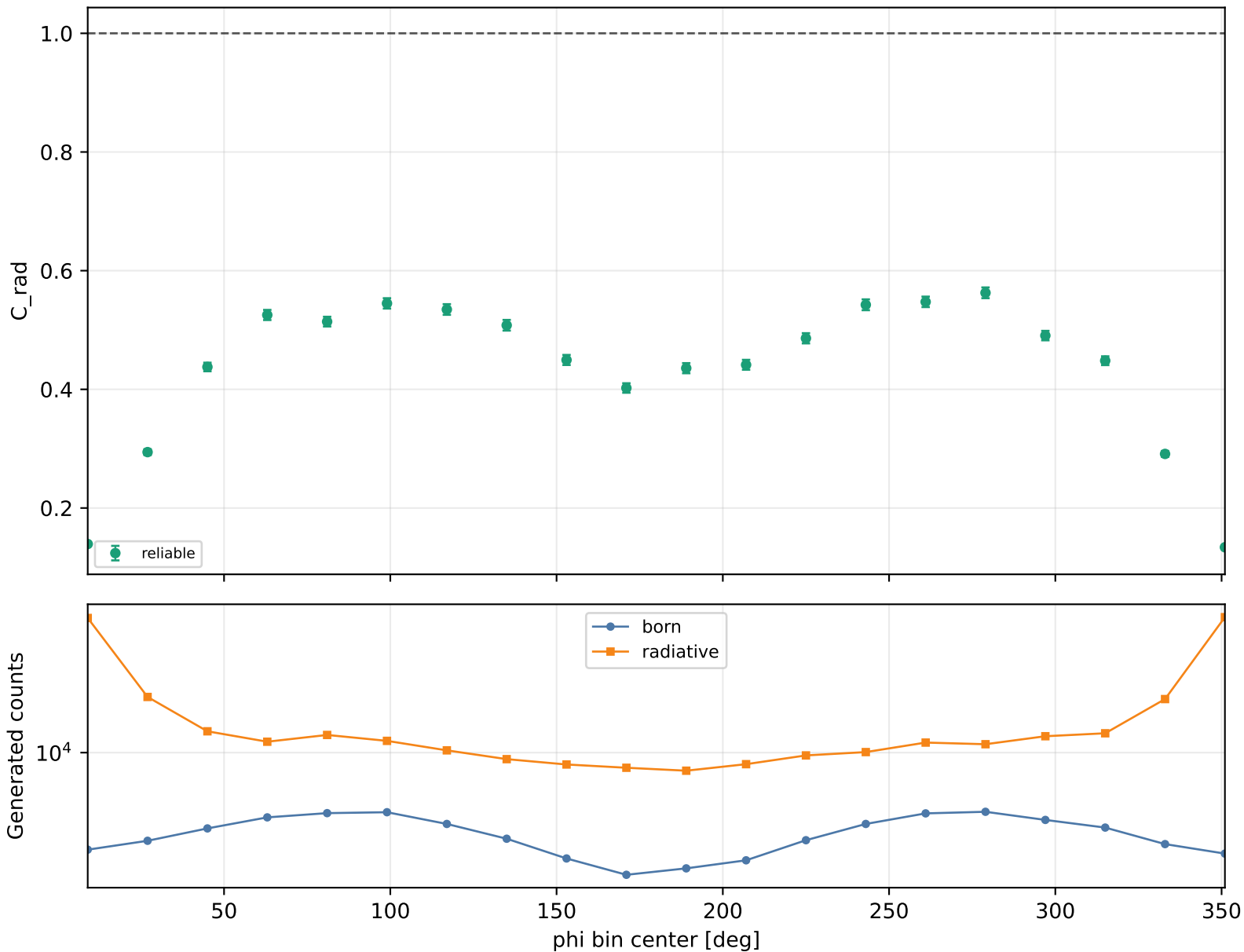
Radiative correction vs phi Q2 1.5-2, xB 0.25-0.3, -t 1-1.5
