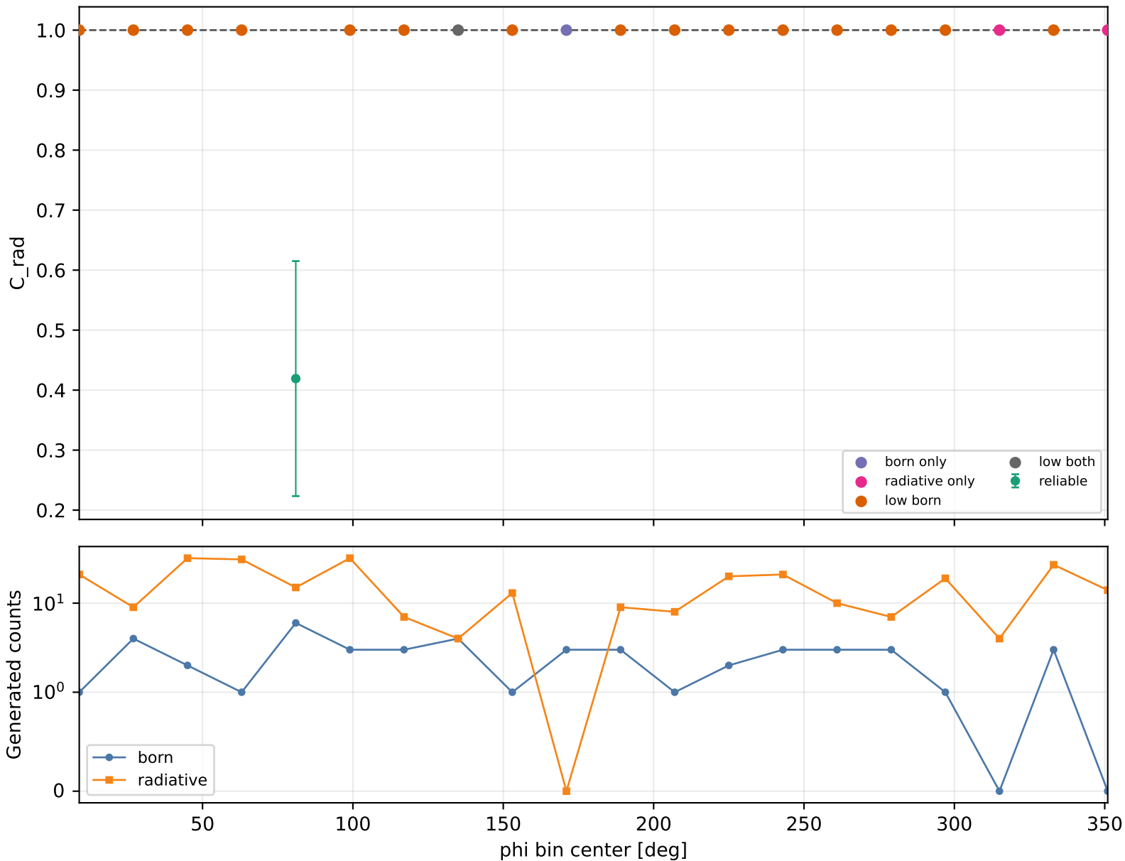
Radiative correction vs phi Q2 3-3.5, xB 0.25-0.3, -t 1.5-2
