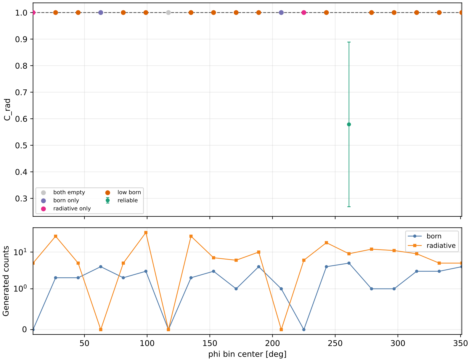
Radiative correction vs phi Q2 1-1.5, xB 0.05-0.1, -t 1.5-2
