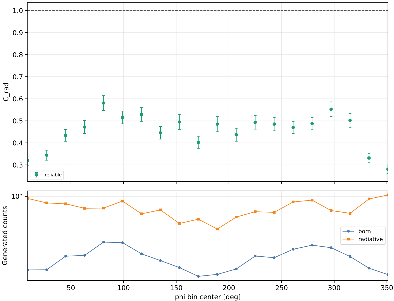
Radiative correction vs phi Q2 4.6-5.5, xB 0.48-0.58, -t 1.5-2
