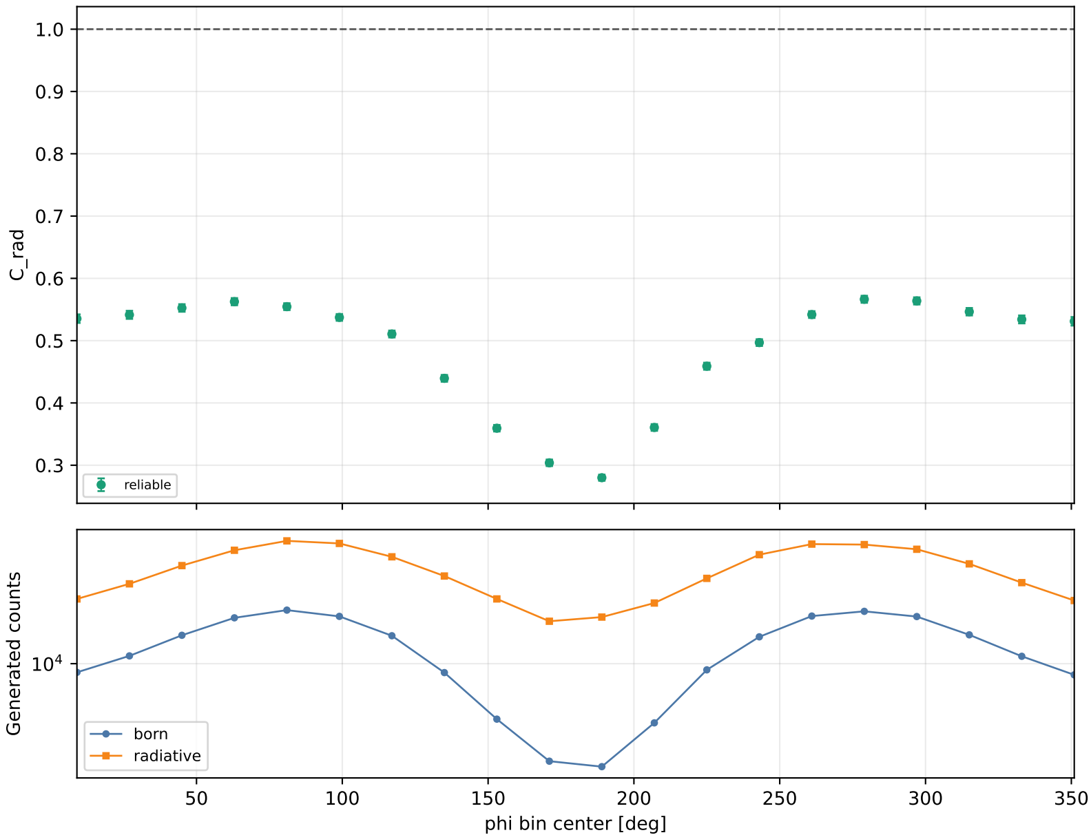
Radiative correction vs phi Q2 1.5-2, xB 0.3-0.38, -t 0.3-0.4
