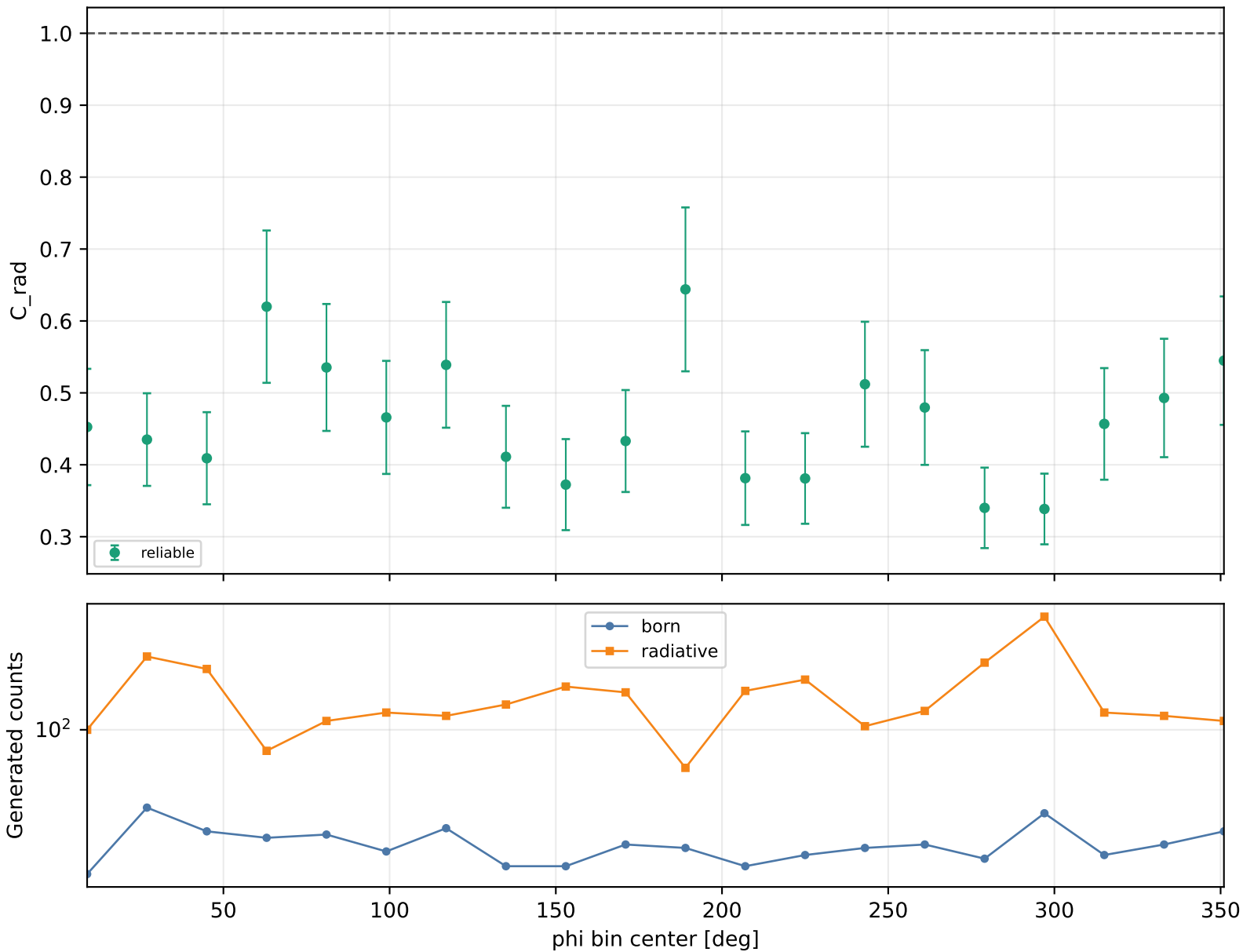
Radiative correction vs phi Q2 4.6-5.5, xB 0.38-0.48, -t 0.4-0.6
