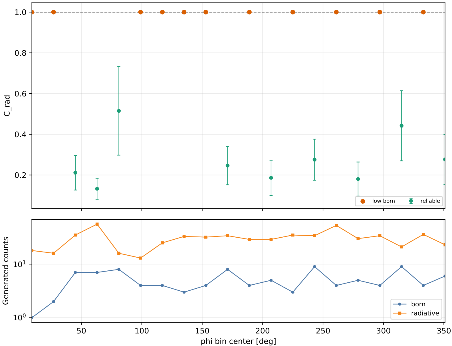
Radiative correction vs phi Q2 3-3.5, xB 0.25-0.3, -t 0.2-0.3
