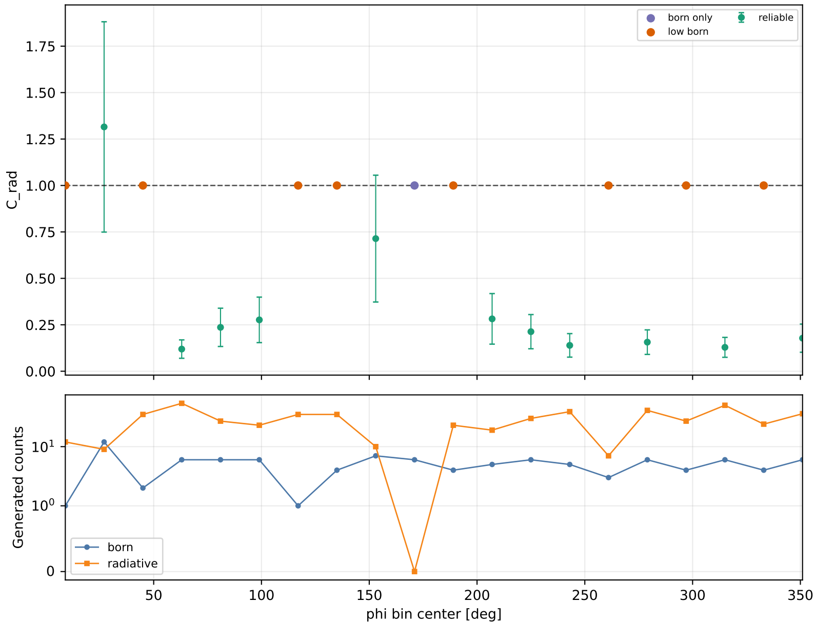
Radiative correction vs phi Q2 1.5-2, xB 0.1-0.15, -t 1-1.5
