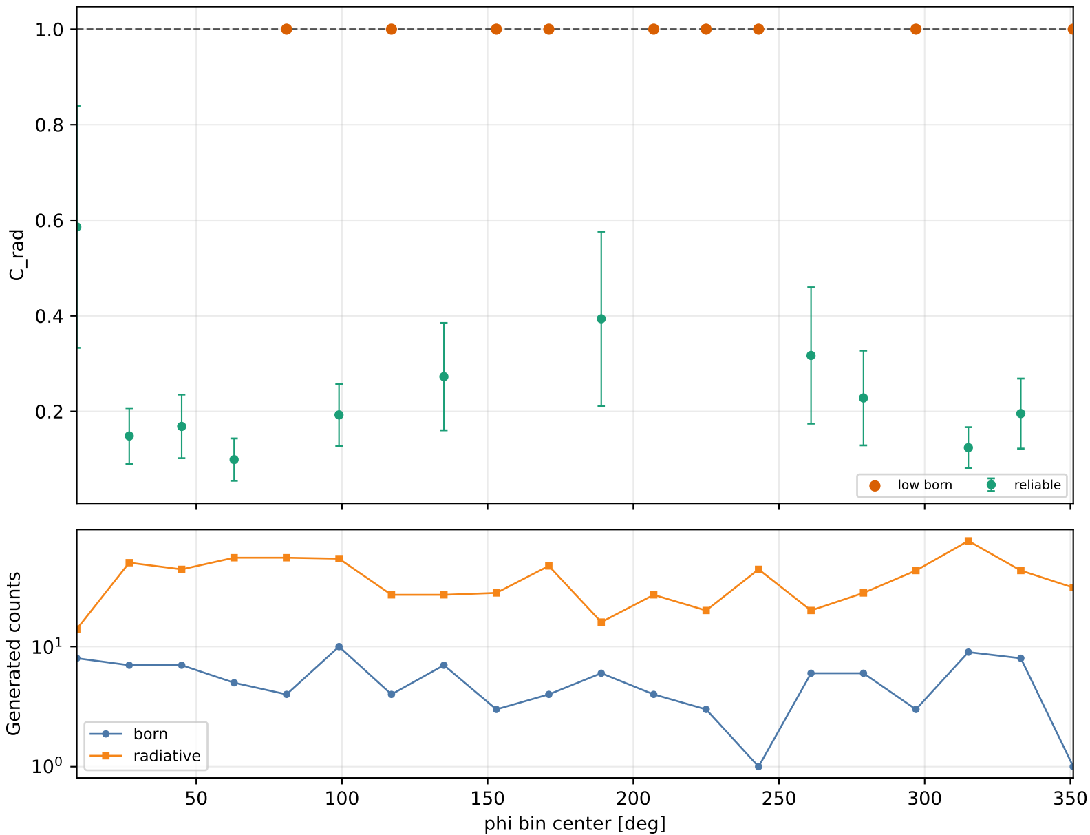
Radiative correction vs phi Q2 2-2.5, xB 0.15-0.2, -t 0.3-0.4
