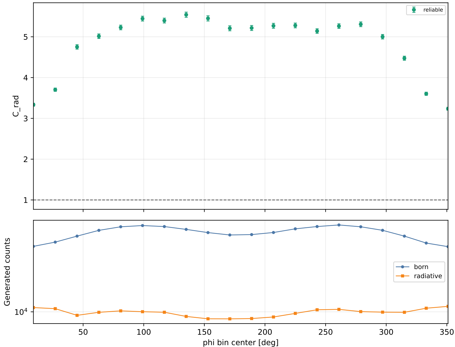
Radiative correction vs phi Q2 2-2.5, xB 0.58-0.7, -t 1.5-2
