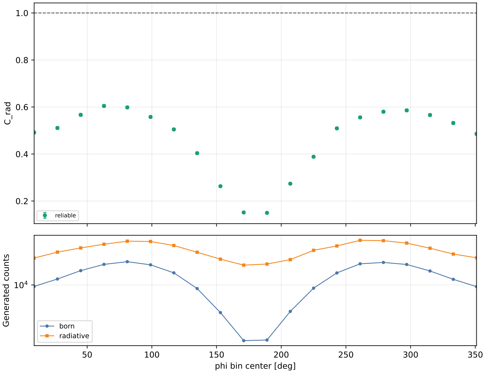
Radiative correction vs phi Q2 1-1.5, xB 0.2-0.25, -t 0.15-0.2
