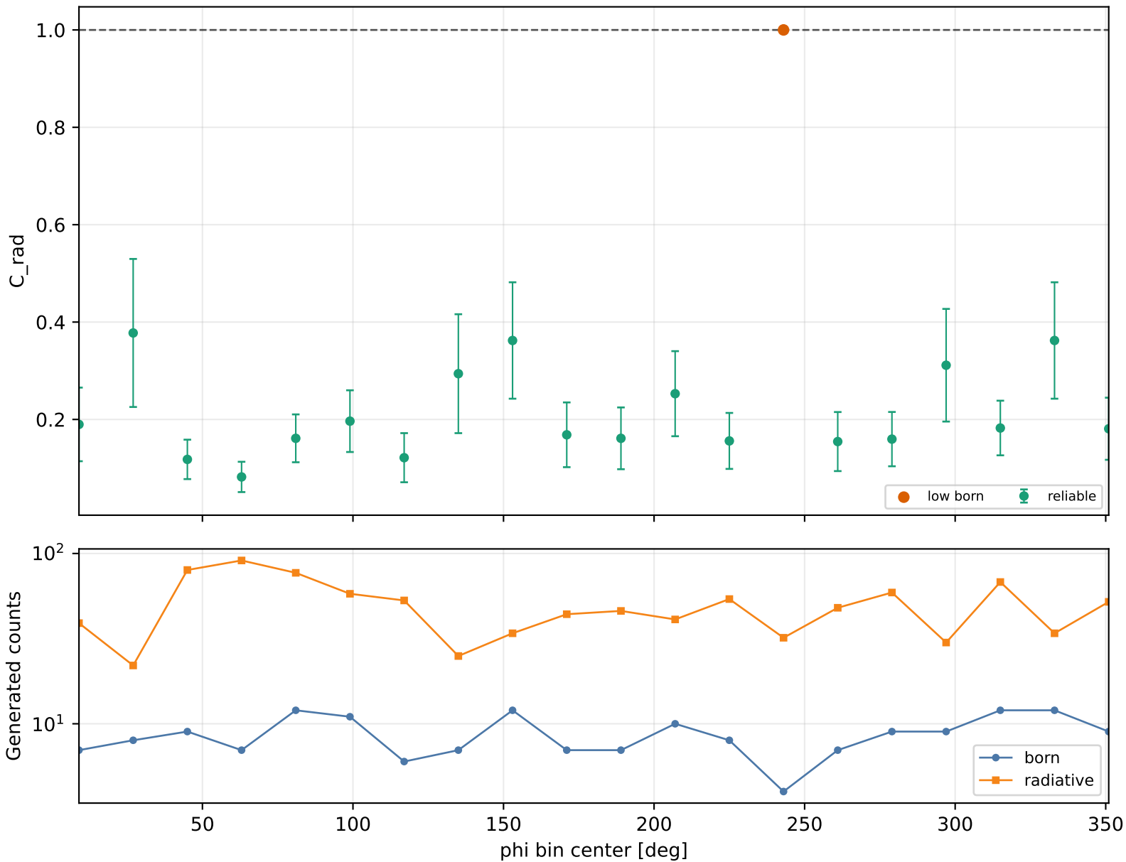
Radiative correction vs phi Q2 3-3.5, xB 0.25-0.3, -t 0.6-1
