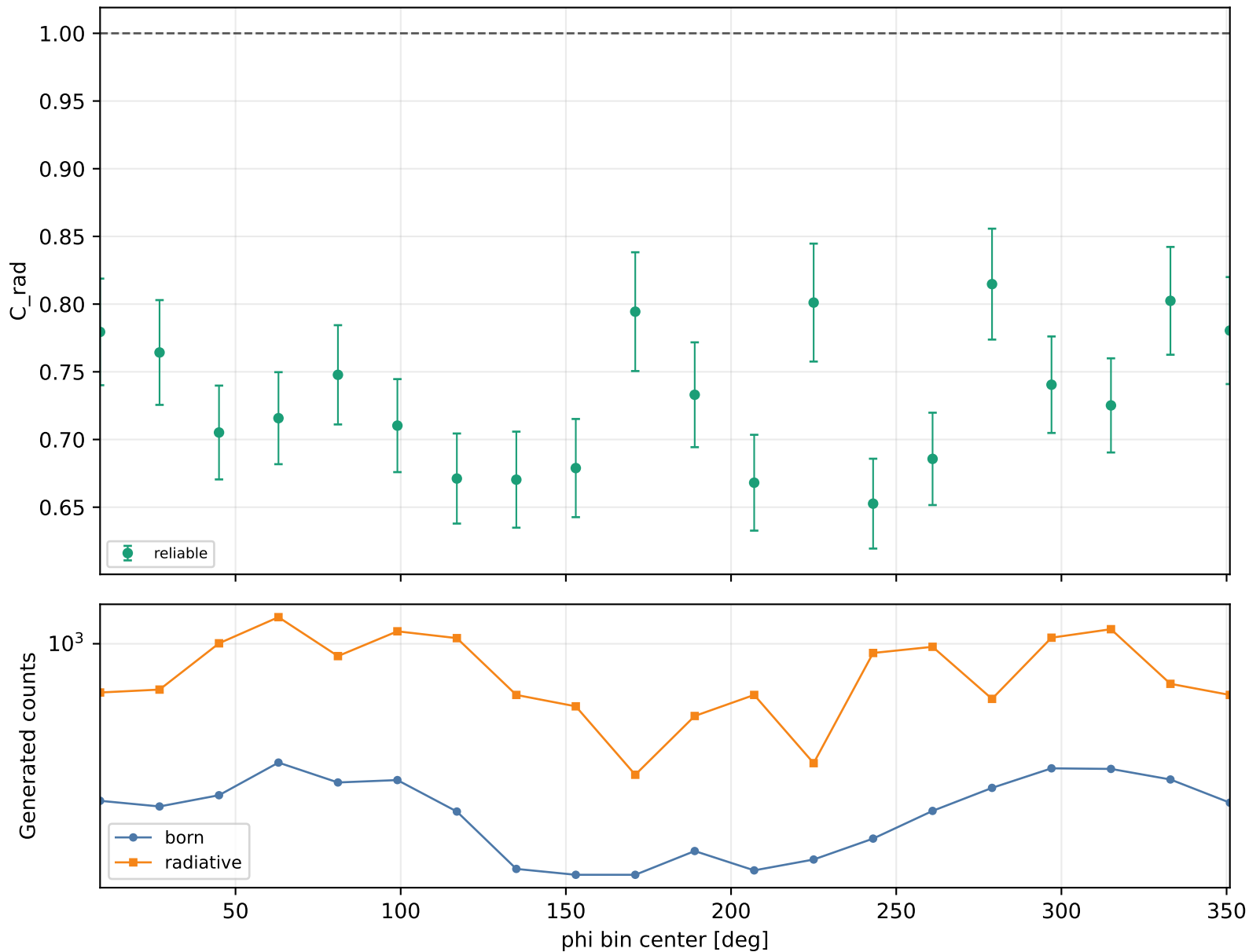
Radiative correction vs phi Q2 2.5-3, xB 0.3-0.38, -t 0.15-0.2
