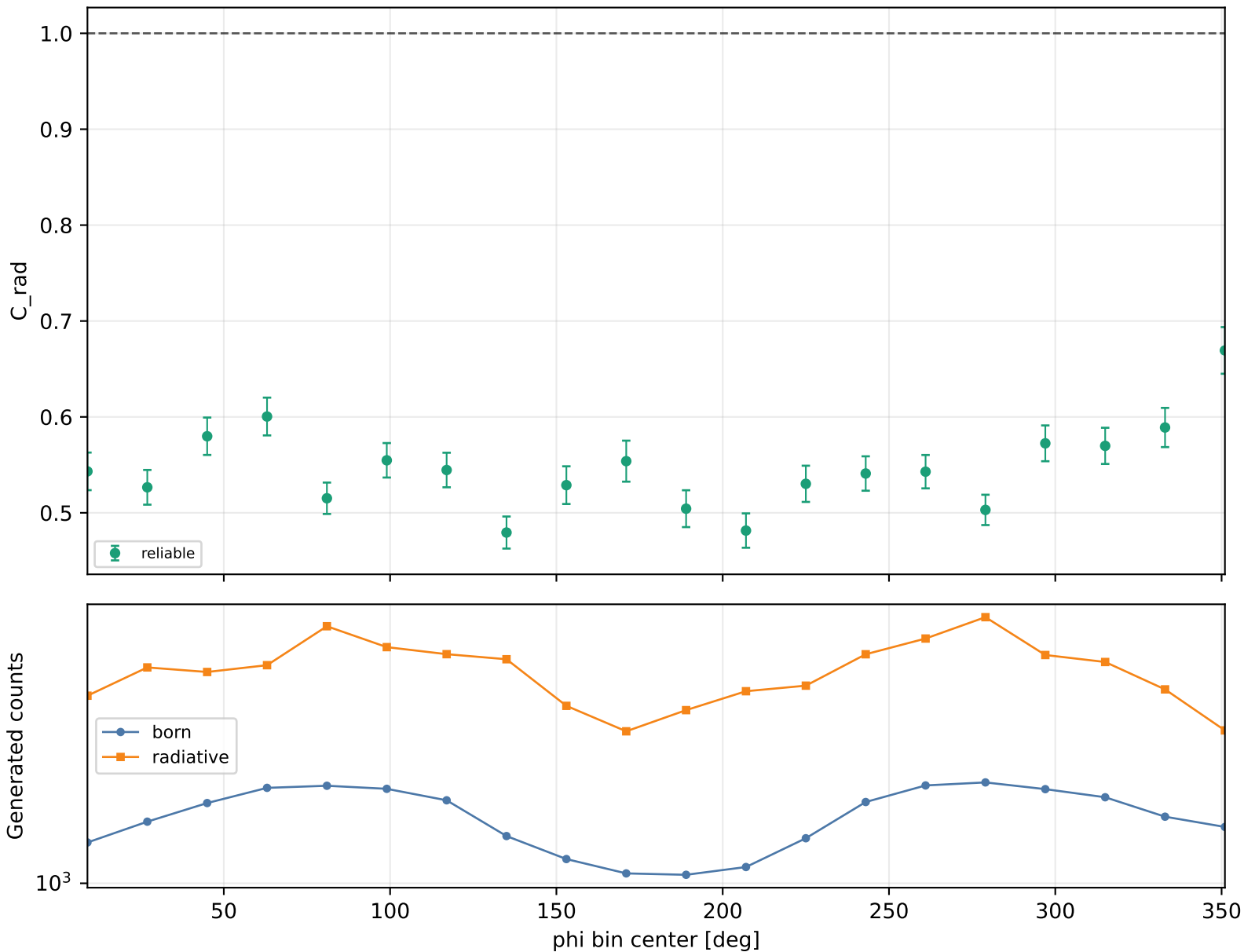
Radiative correction vs phi Q2 3-3.5, xB 0.48-0.58, -t 0.4-0.6
