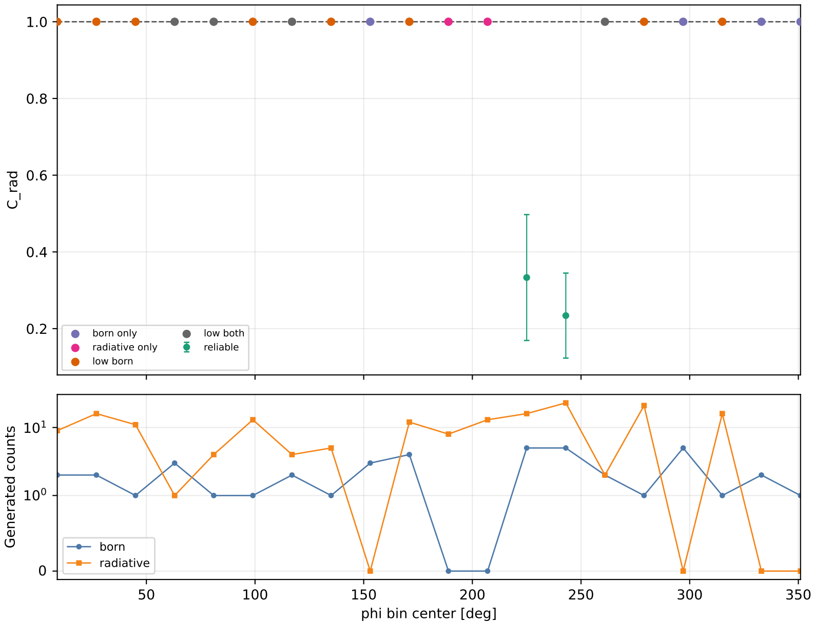
Radiative correction vs phi Q2 2.5-3, xB 0.2-0.25, -t 1.5-2
