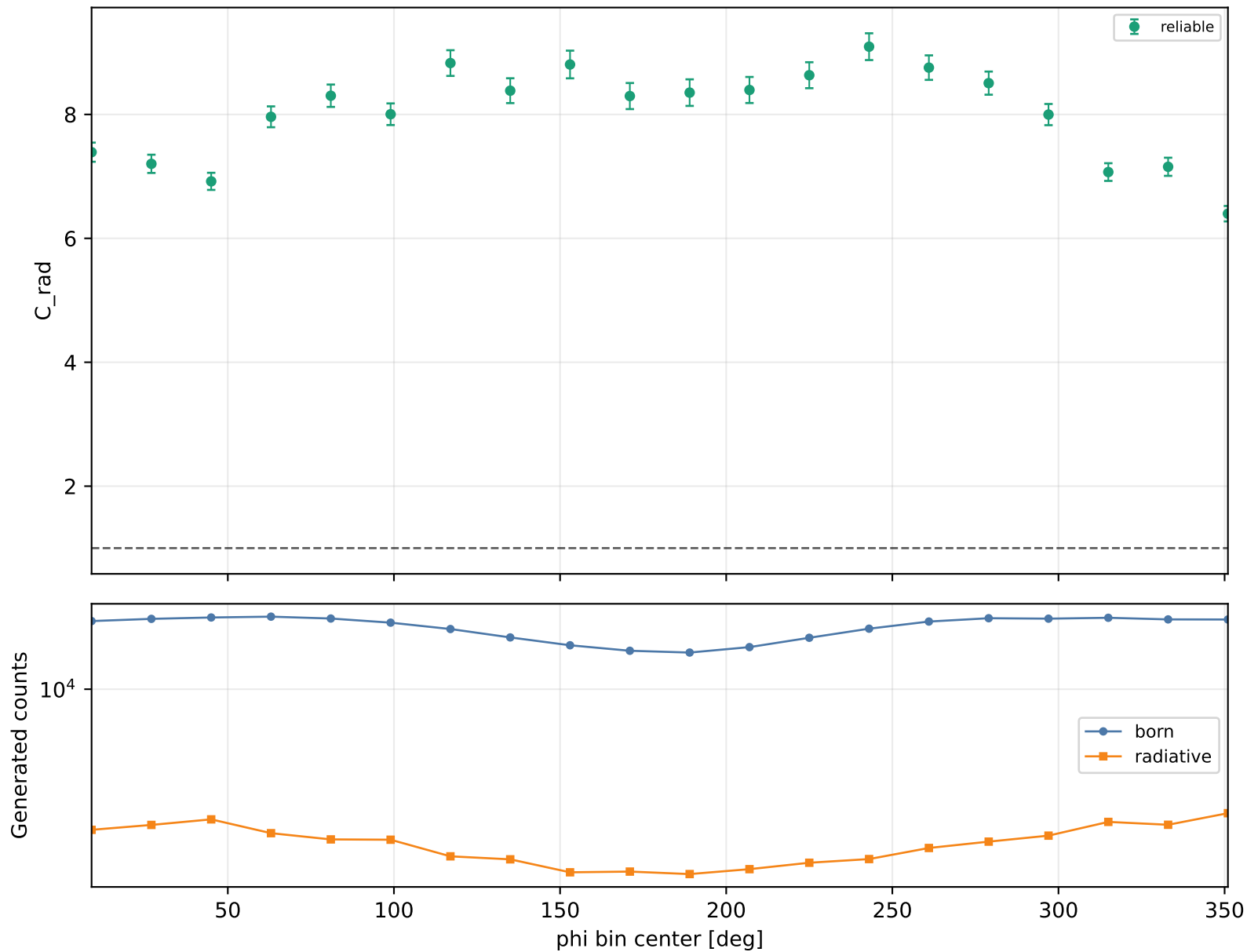
Radiative correction vs phi Q2 1.5-2, xB 0.48-0.58, -t 0.4-0.6
