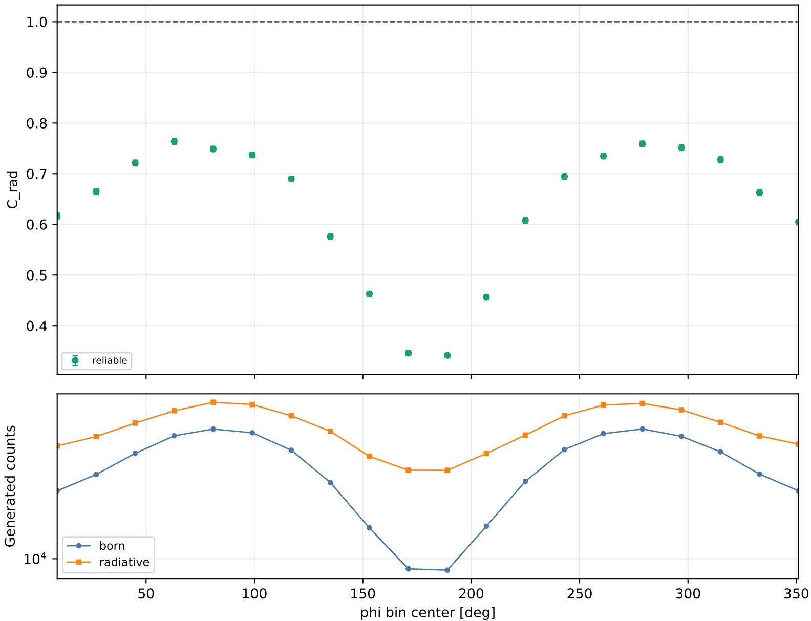
Radiative correction vs phi Q2 1-1.5, xB 0.25-0.3, -t 0.3-0.4
