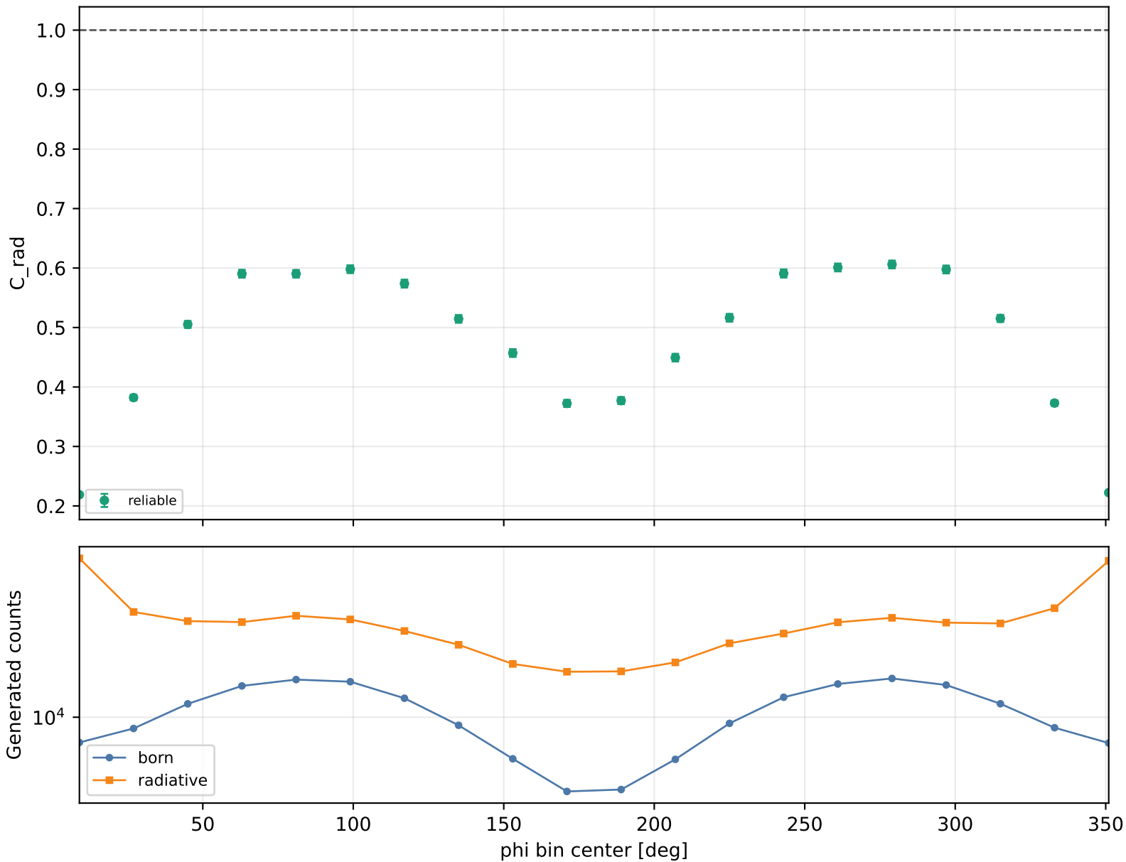
Radiative correction vs phi Q2 1.5-2, xB 0.25-0.3, -t 0.6-1
