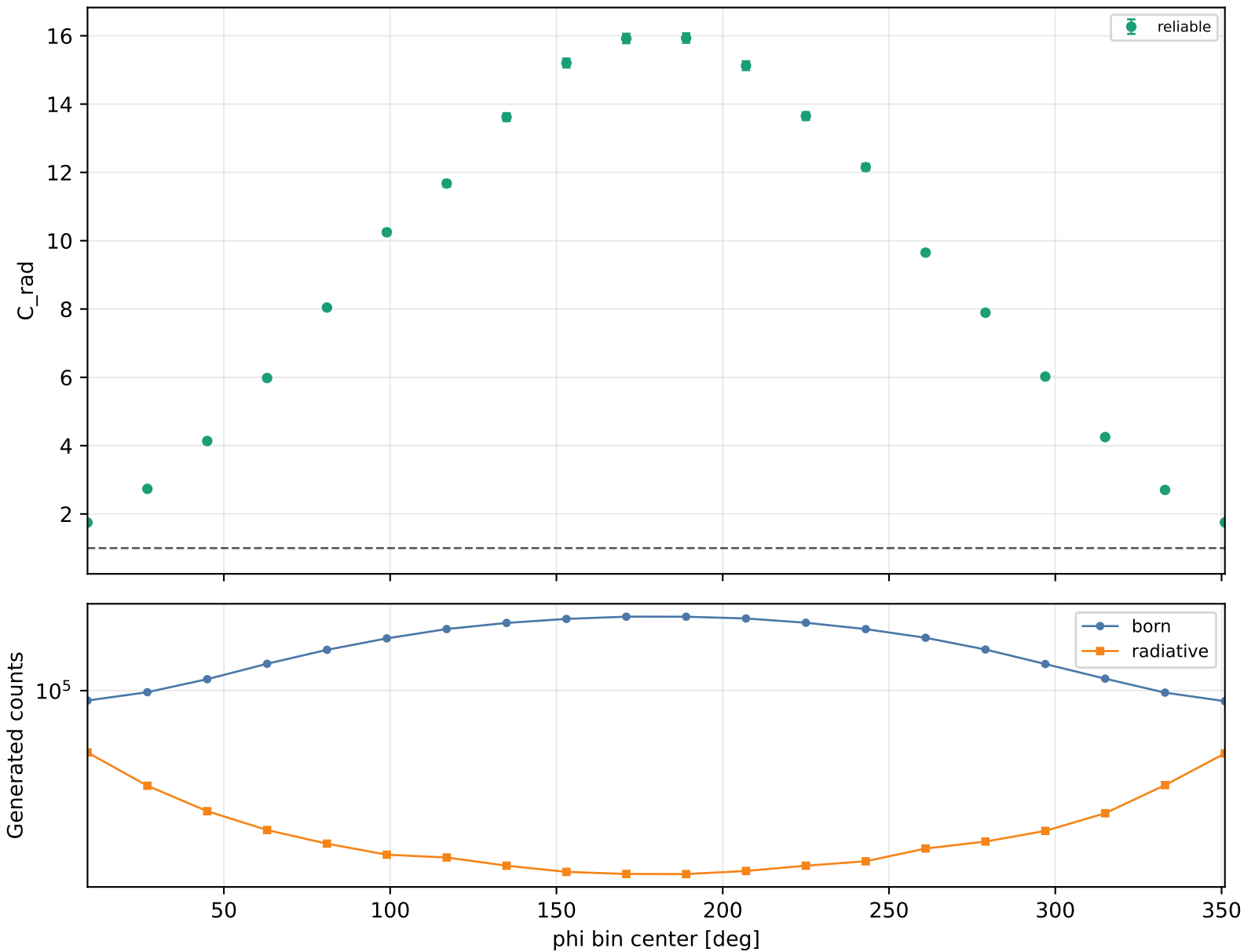
Radiative correction vs phi Q2 1-1.5, xB 0.3-0.38, -t 1.5-2
