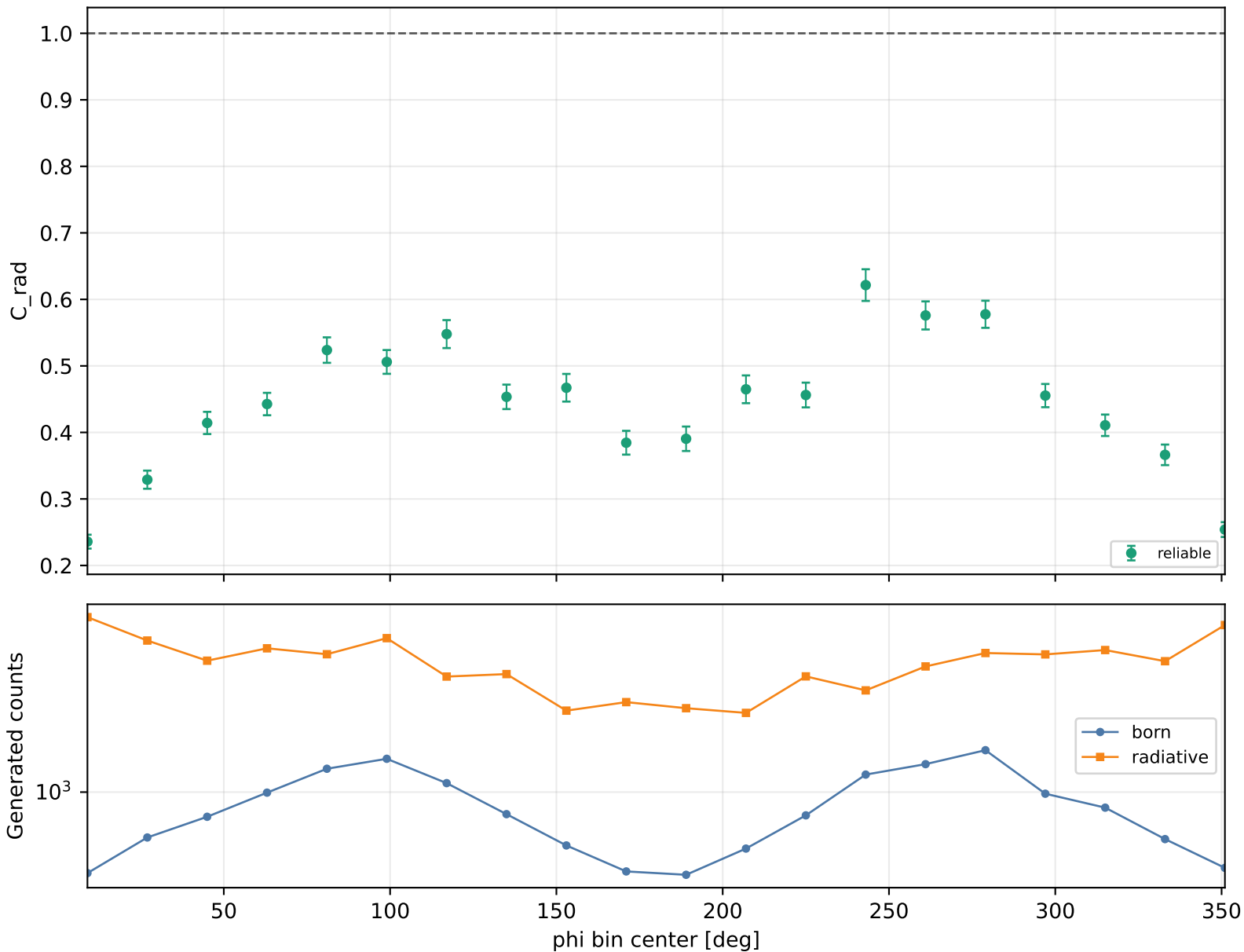
Radiative correction vs phi Q2 4-4.6, xB 0.48-0.58, -t 1.5-2
