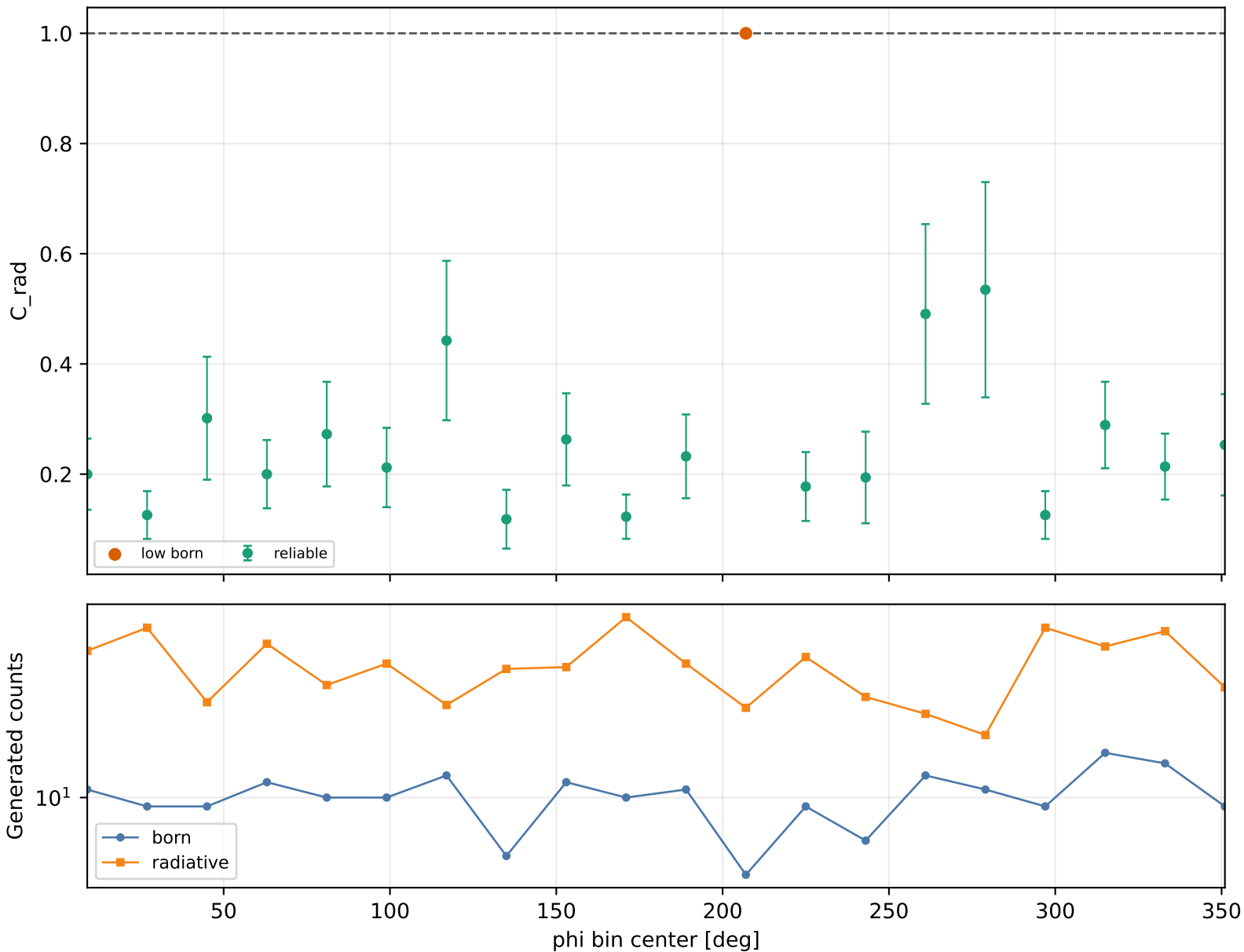
Radiative correction vs phi Q2 2.5-3, xB 0.2-0.25, -t 0.6-1
