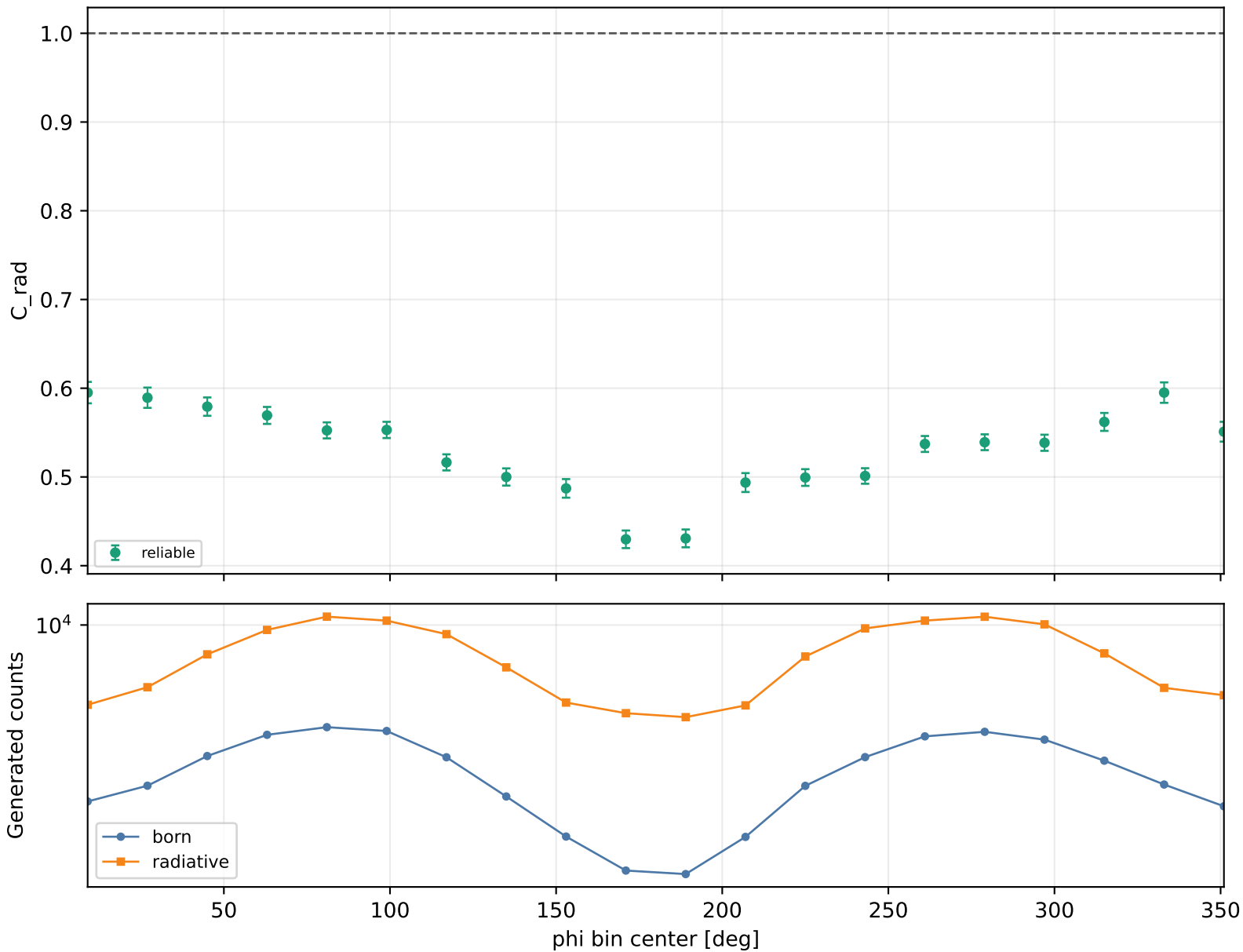
Radiative correction vs phi Q2 2.5-3, xB 0.38-0.48, -t 0.4-0.6
