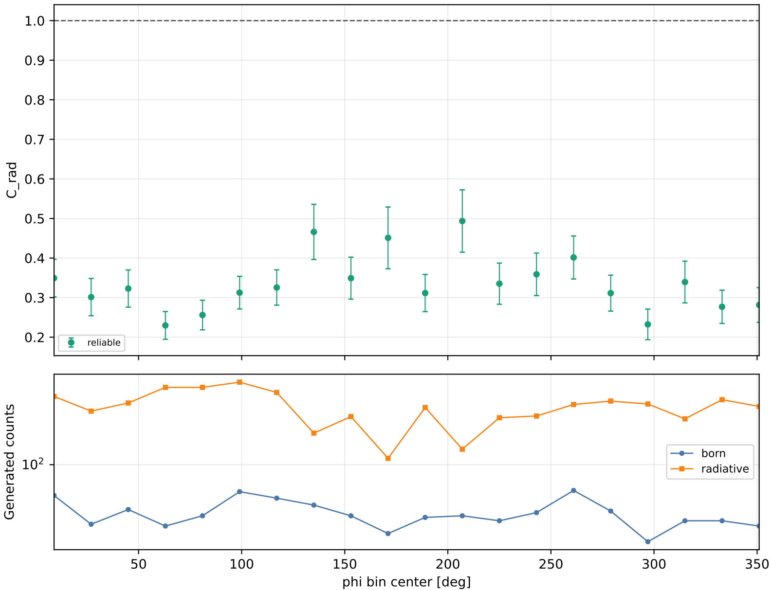
Radiative correction vs phi Q2 4.6-5.5, xB 0.38-0.48, -t 1-1.5
