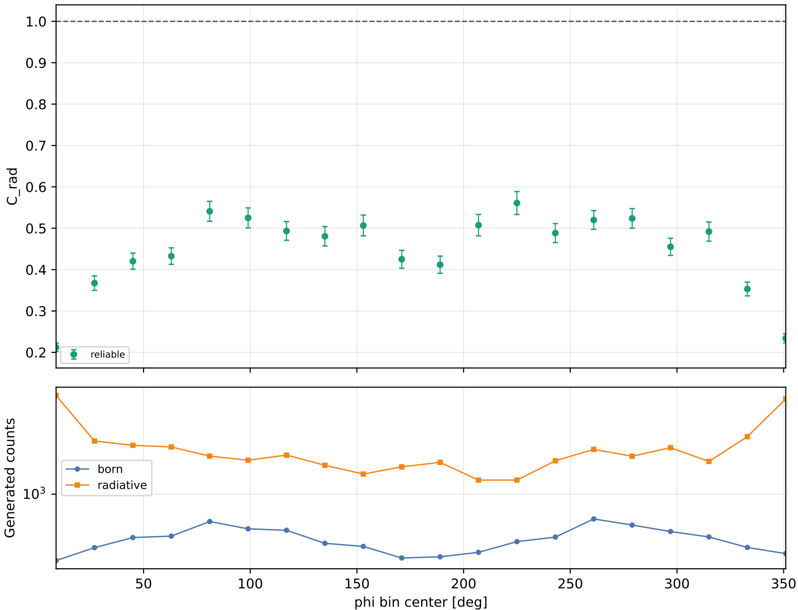
Radiative correction vs phi Q2 3.5-4, xB 0.38-0.48, -t 1.5-2
