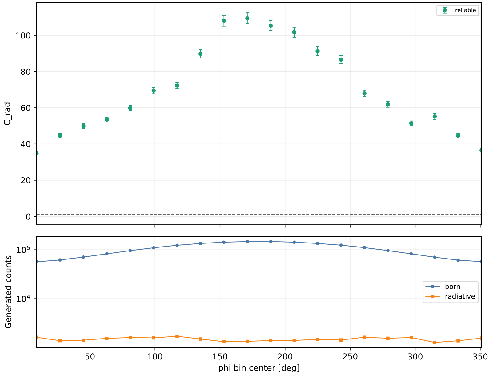
Radiative correction vs phi Q2 1-1.5, xB 0.38-0.48, -t 1.5-2
