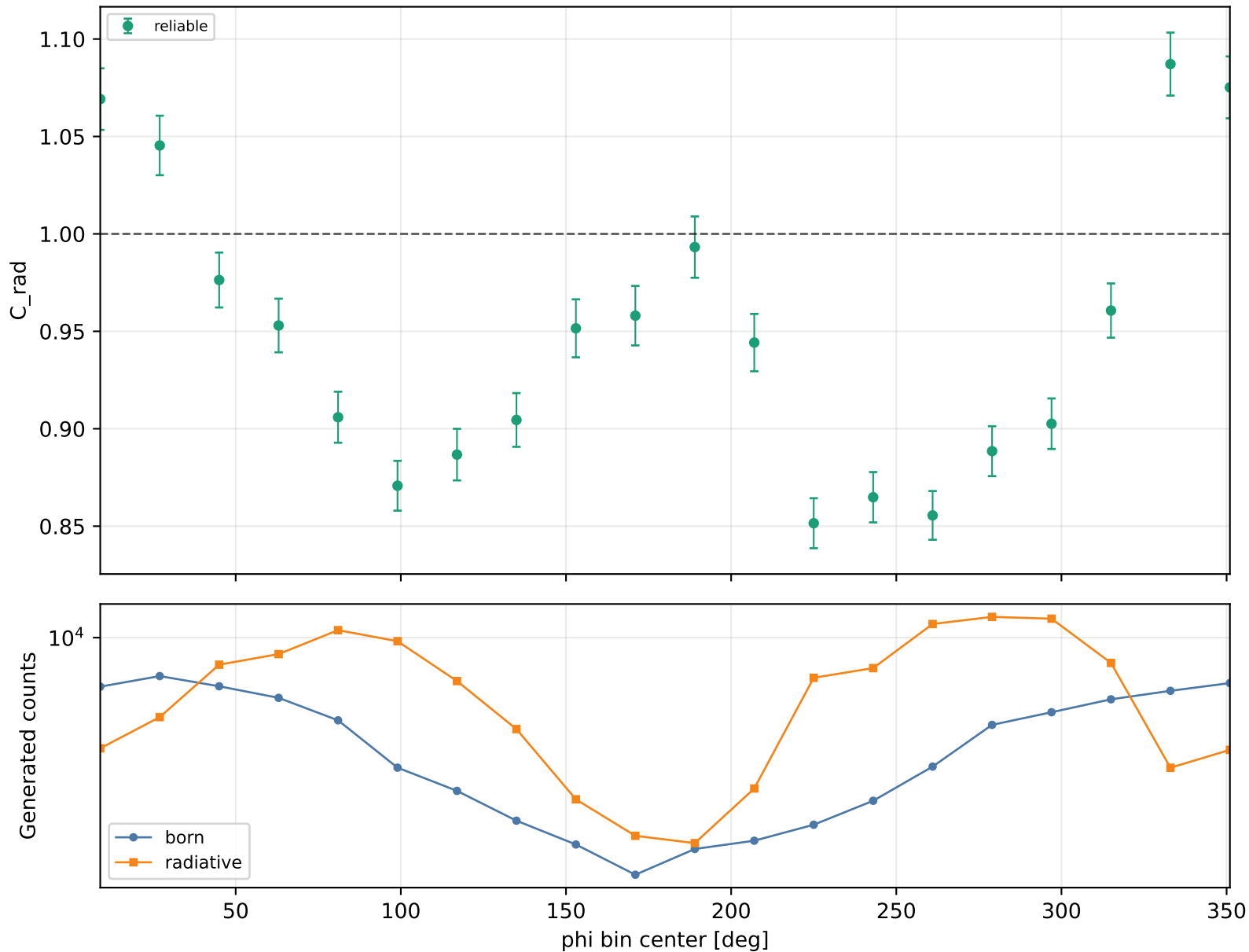
Radiative correction vs phi Q2 1.5-2, xB 0.38-0.48, -t 0.2-0.3
