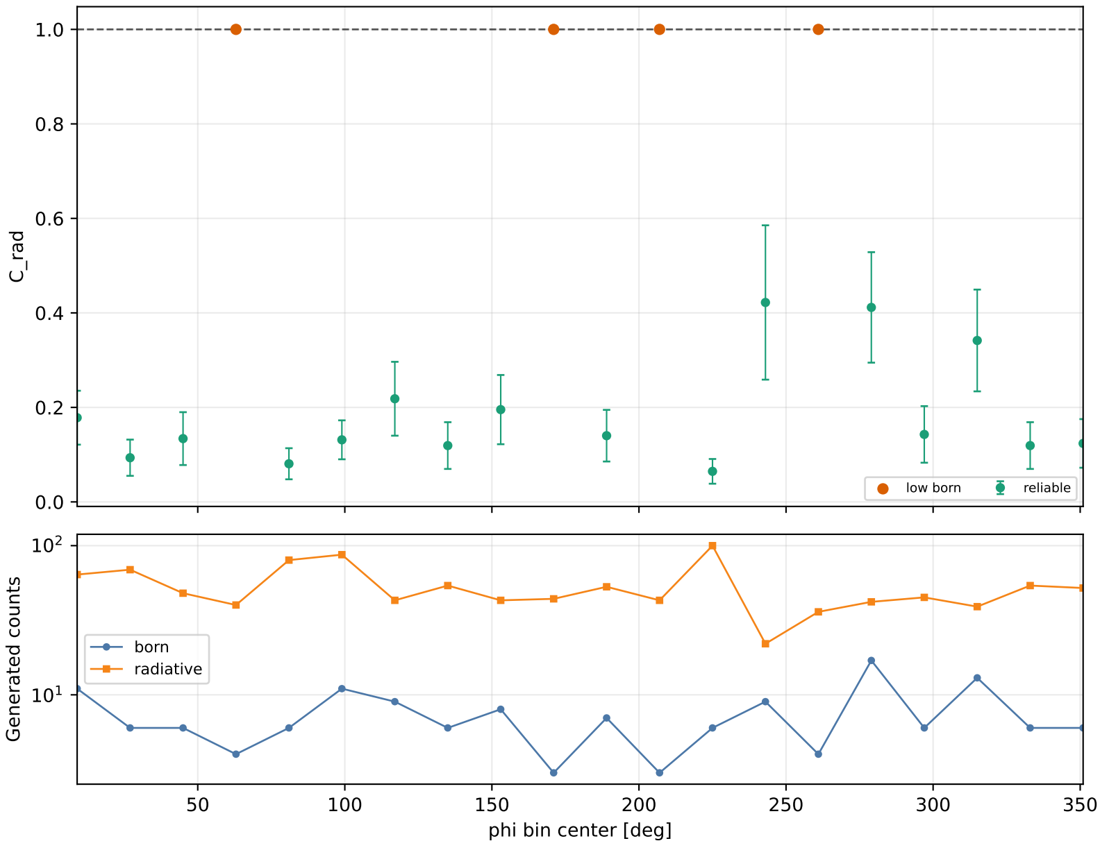
Radiative correction vs phi Q2 1-1.5, xB 0.05-0.1, -t 0.15-0.2
