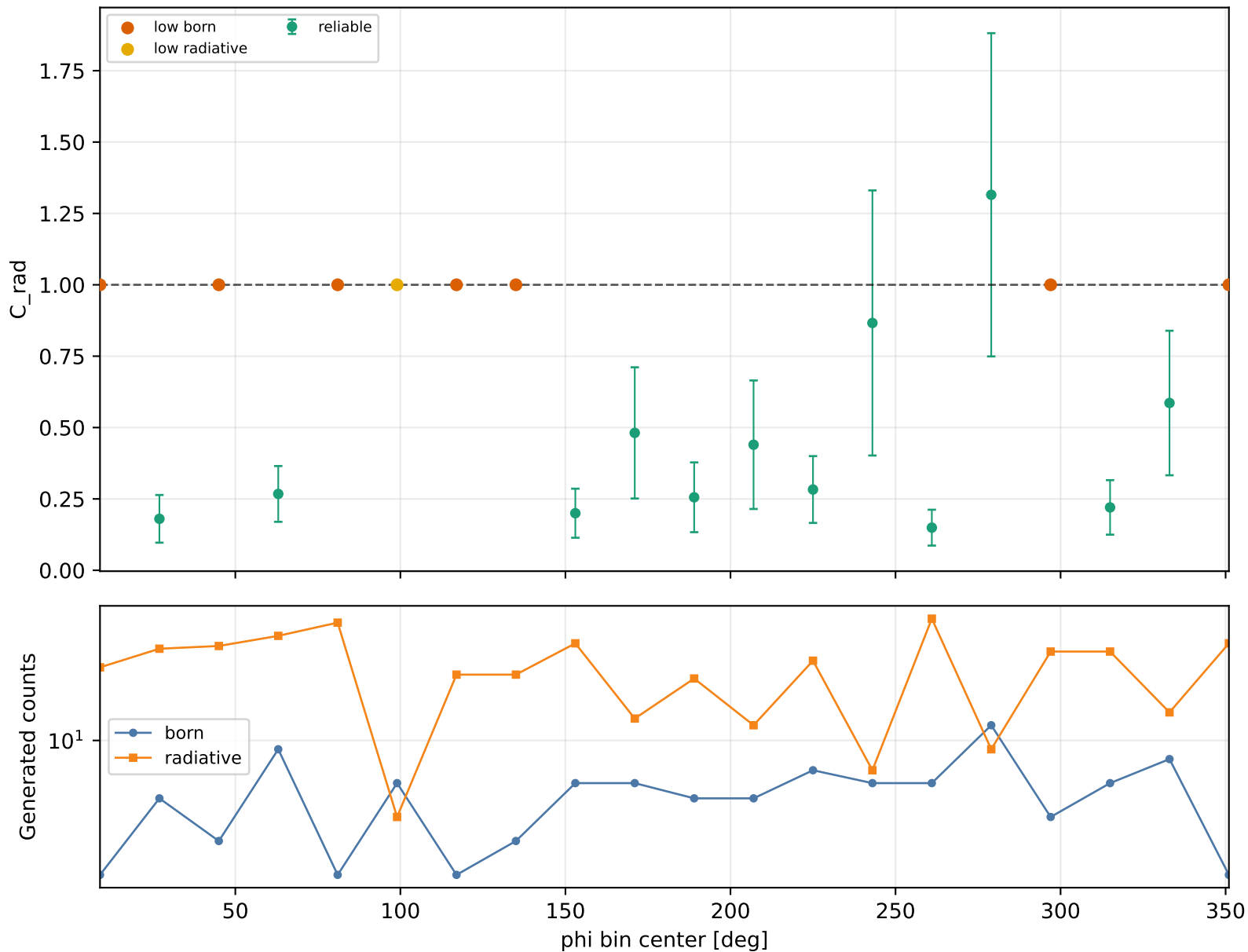
Radiative correction vs phi Q2 2-2.5, xB 0.15-0.2, -t 1-1.5
