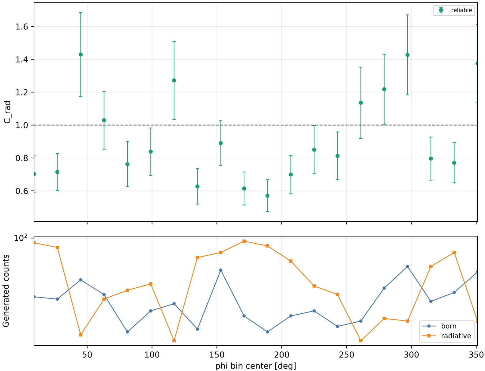
Radiative correction vs phi Q2 4-4.6, xB 0.38-0.48, -t 0.2-0.3
