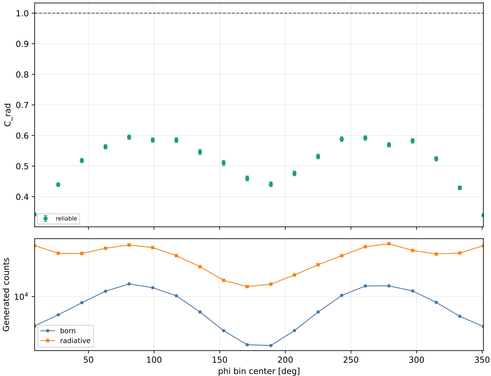
Radiative correction vs phi Q2 2-2.5, xB 0.3-0.38, -t 0.6-1
