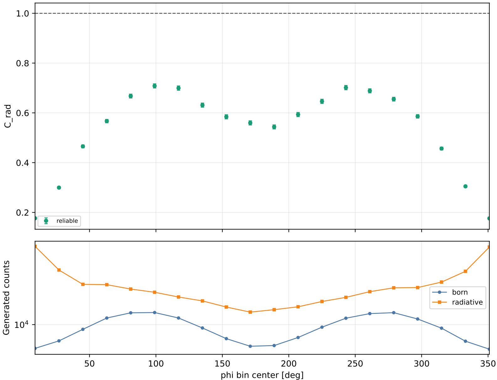
Radiative correction vs phi Q2 2-2.5, xB 0.38-0.48, -t 1.5-2
