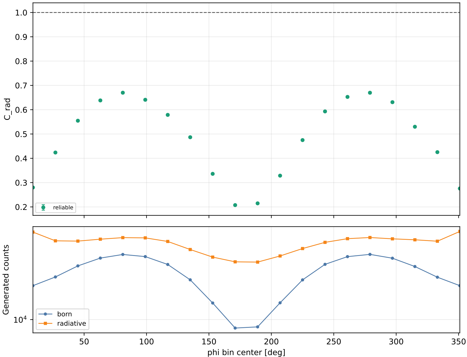
Radiative correction vs phi Q2 1-1.5, xB 0.2-0.25, -t 0.4-0.6
