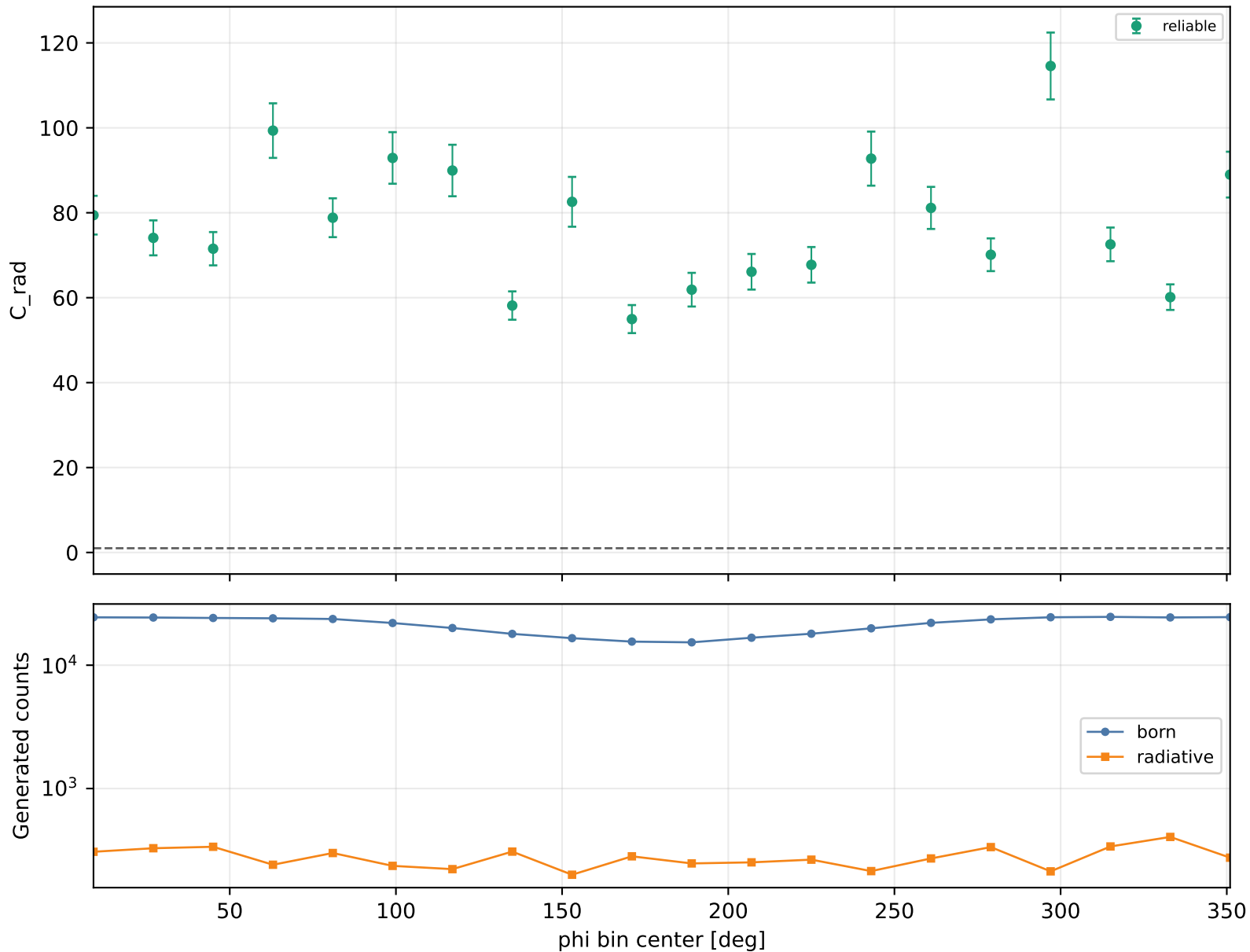
Radiative correction vs phi Q2 1-1.5, xB 0.38-0.48, -t 0.3-0.4
