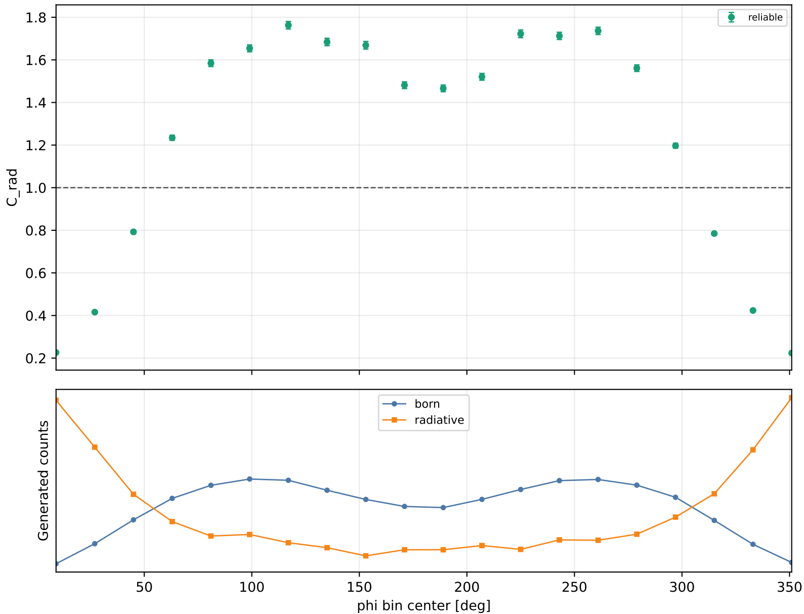
Radiative correction vs phi Q2 1-1.5, xB 0.25-0.3, -t 1.5-2
