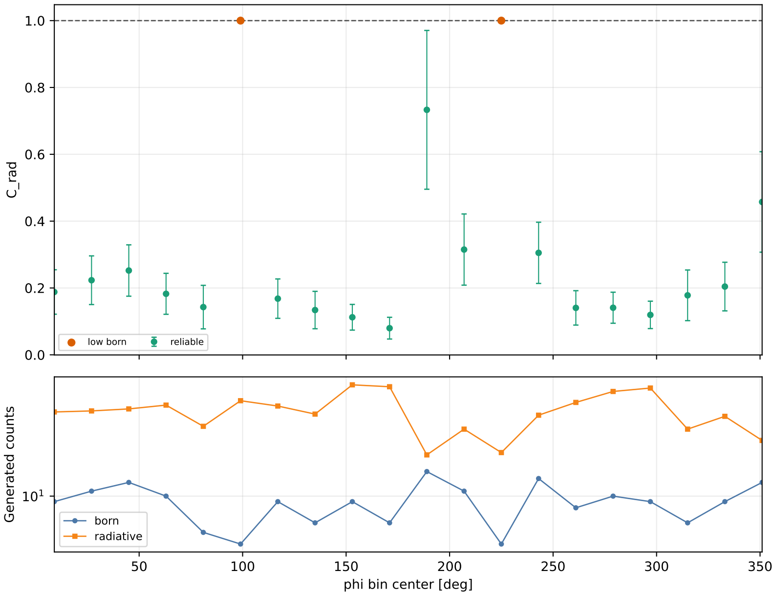
Radiative correction vs phi Q2 2-2.5, xB 0.15-0.2, -t 0.4-0.6
