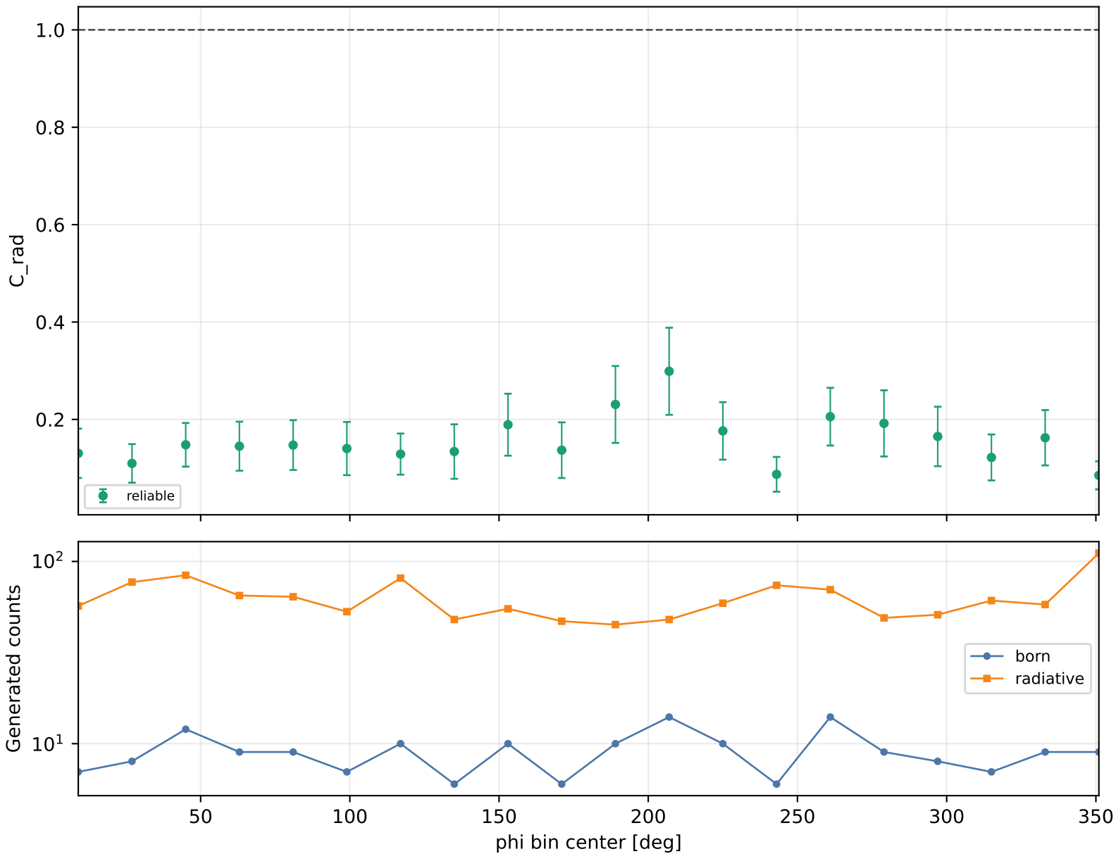
Radiative correction vs phi Q2 1.5-2, xB 0.1-0.15, -t 0.6-1
