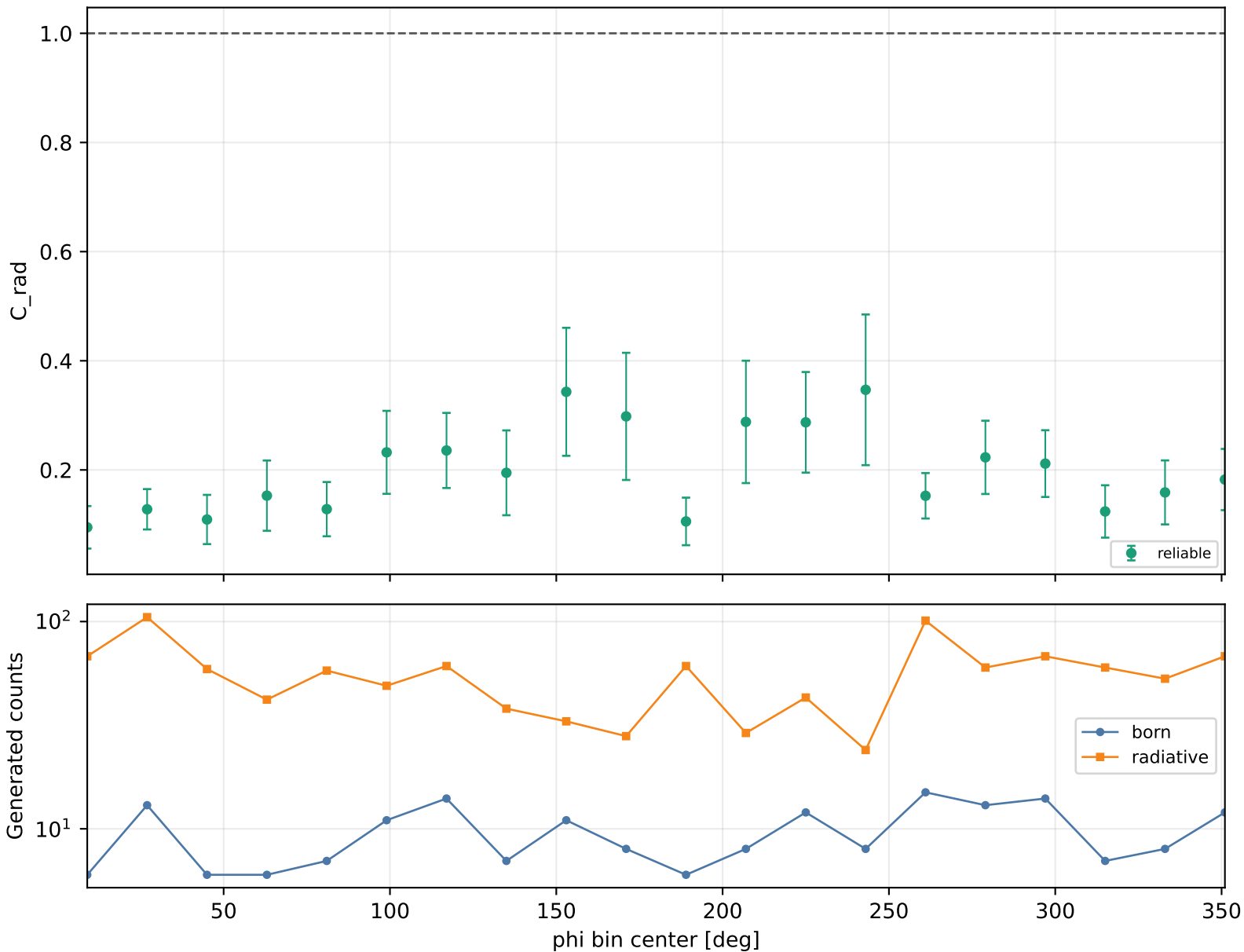
Radiative correction vs phi Q2 2-2.5, xB 0.15-0.2, -t 0.6-1
