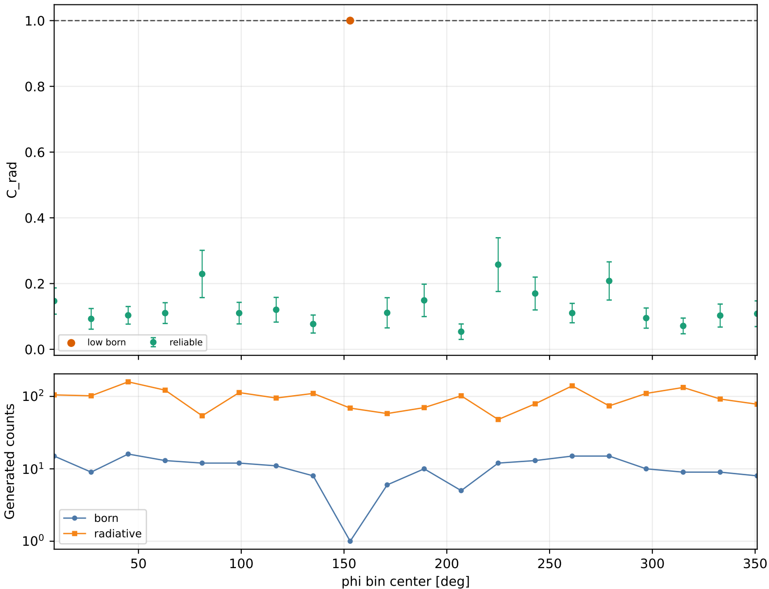
Radiative correction vs phi Q2 1-1.5, xB 0.05-0.1, -t 0.2-0.3
