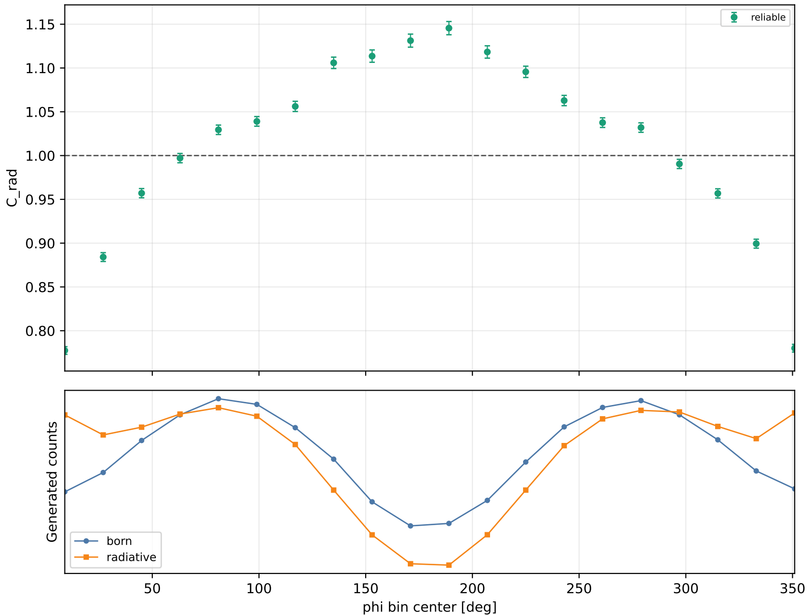
Radiative correction vs phi Q2 1.5-2, xB 0.38-0.48, -t 0.6-1
