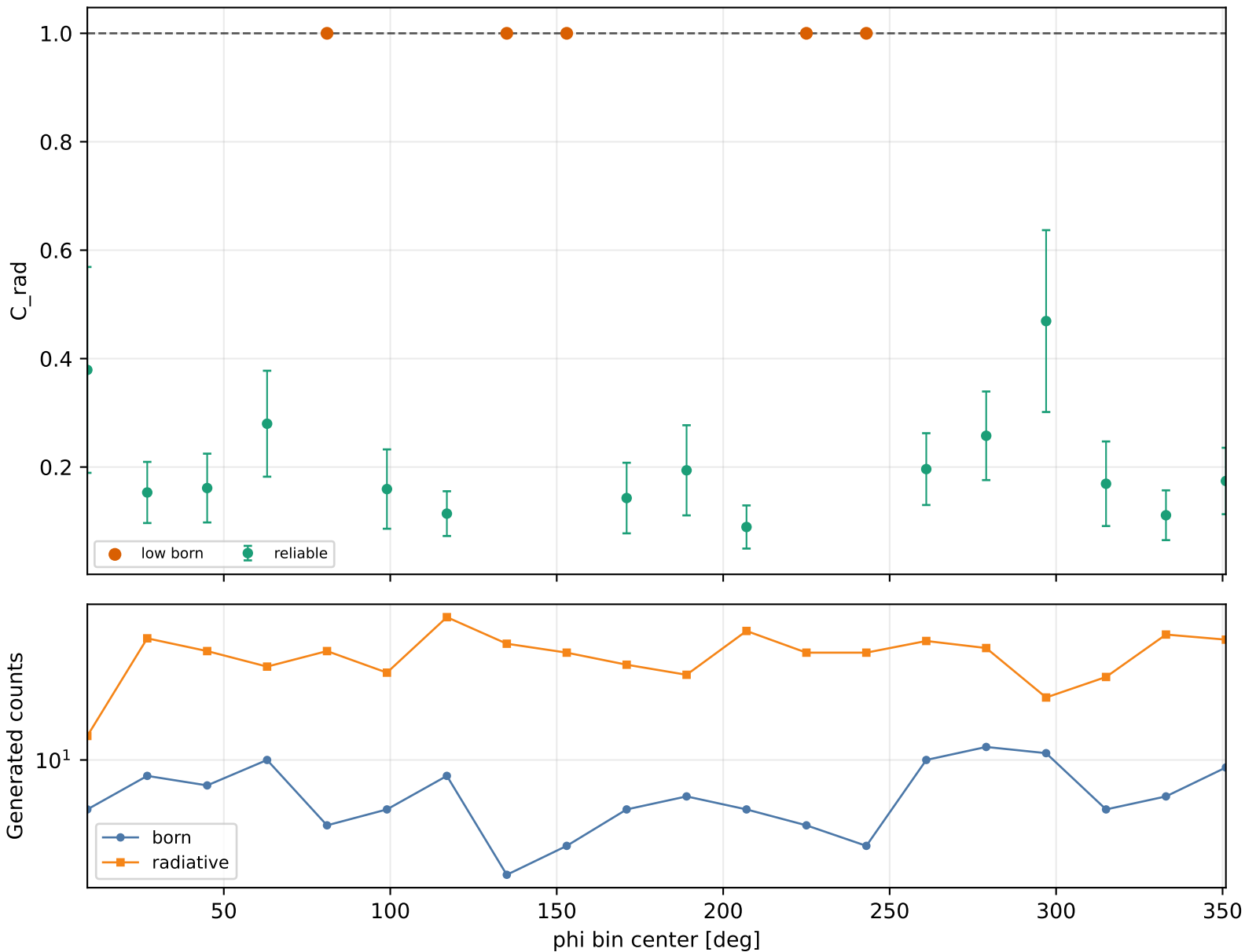
Radiative correction vs phi Q2 3-3.5, xB 0.25-0.3, -t 0.4-0.6
