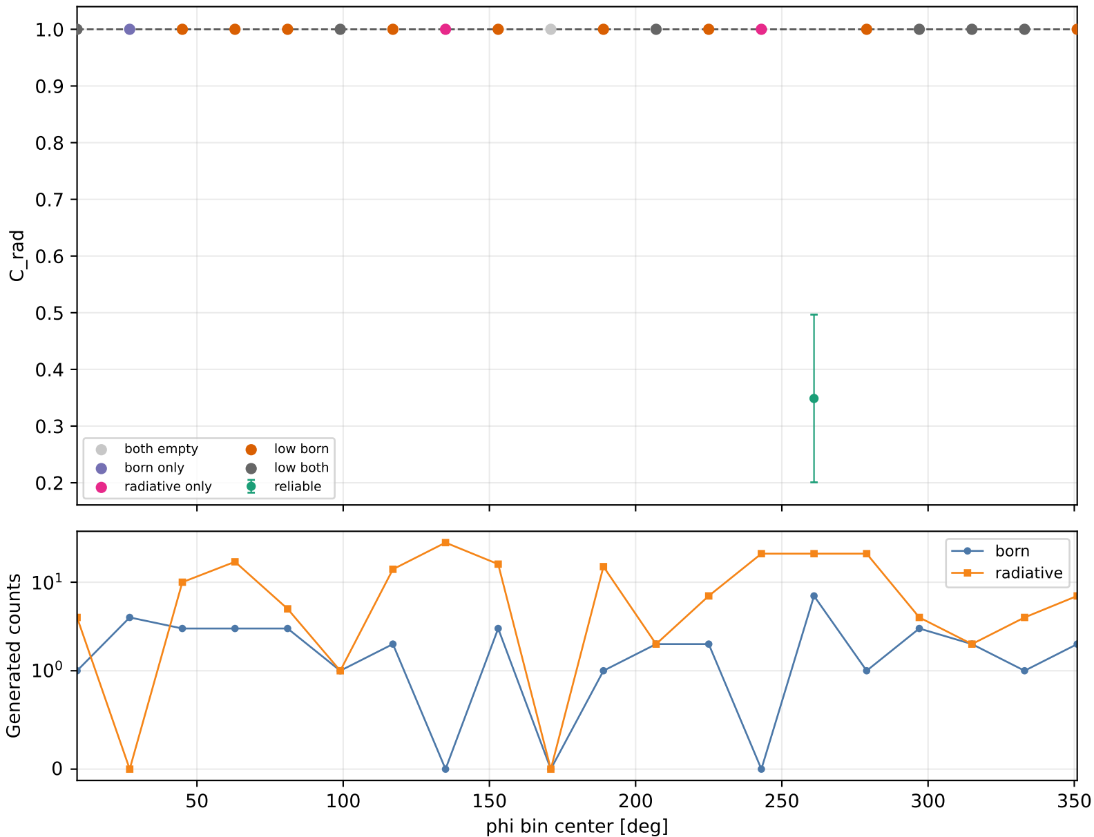
Radiative correction vs phi Q2 3-3.5, xB 0.25-0.3, -t 0.15-0.2
