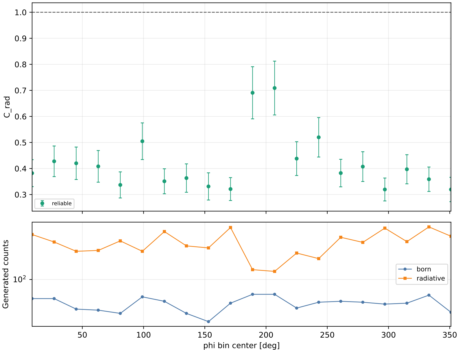
Radiative correction vs phi Q2 3.5-4, xB 0.3-0.38, -t 1.5-2
