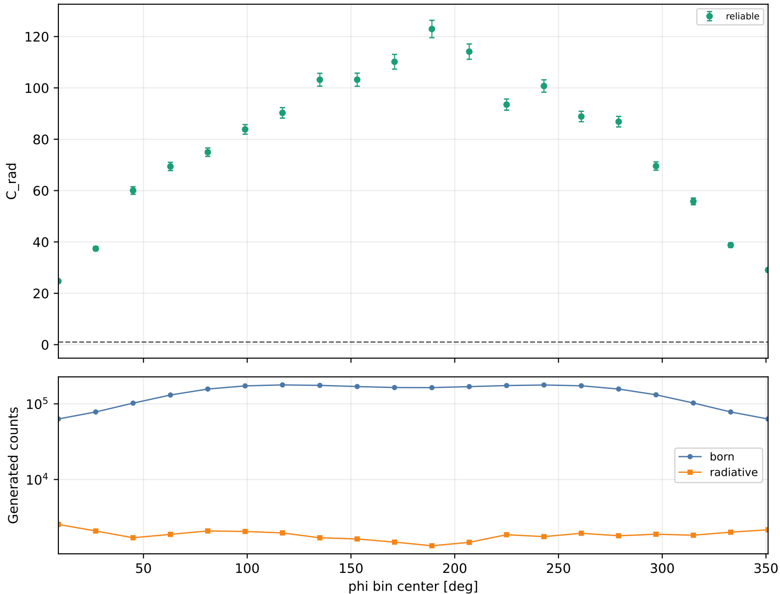
Radiative correction vs phi Q2 1-1.5, xB 0.38-0.48, -t 1-1.5
