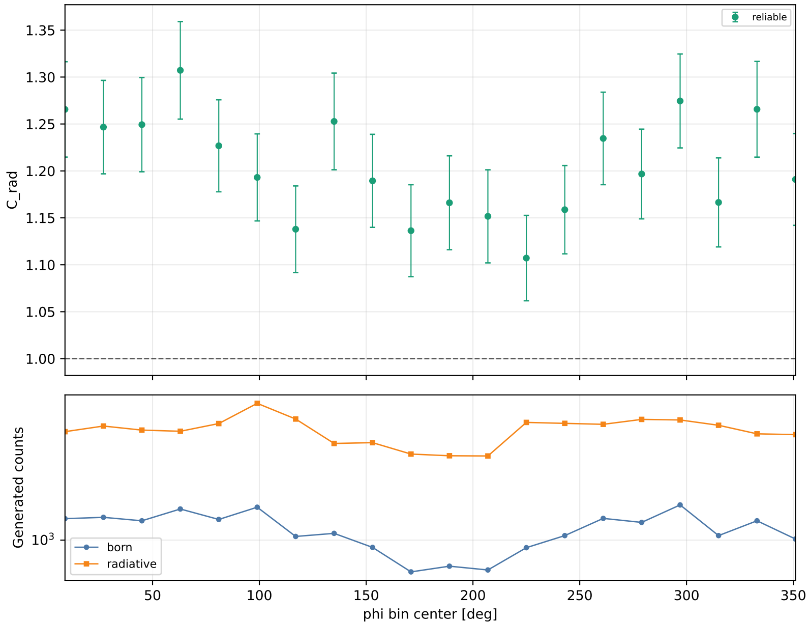
Radiative correction vs phi Q2 3.5-4, xB 0.38-0.48, -t 0.3-0.4
