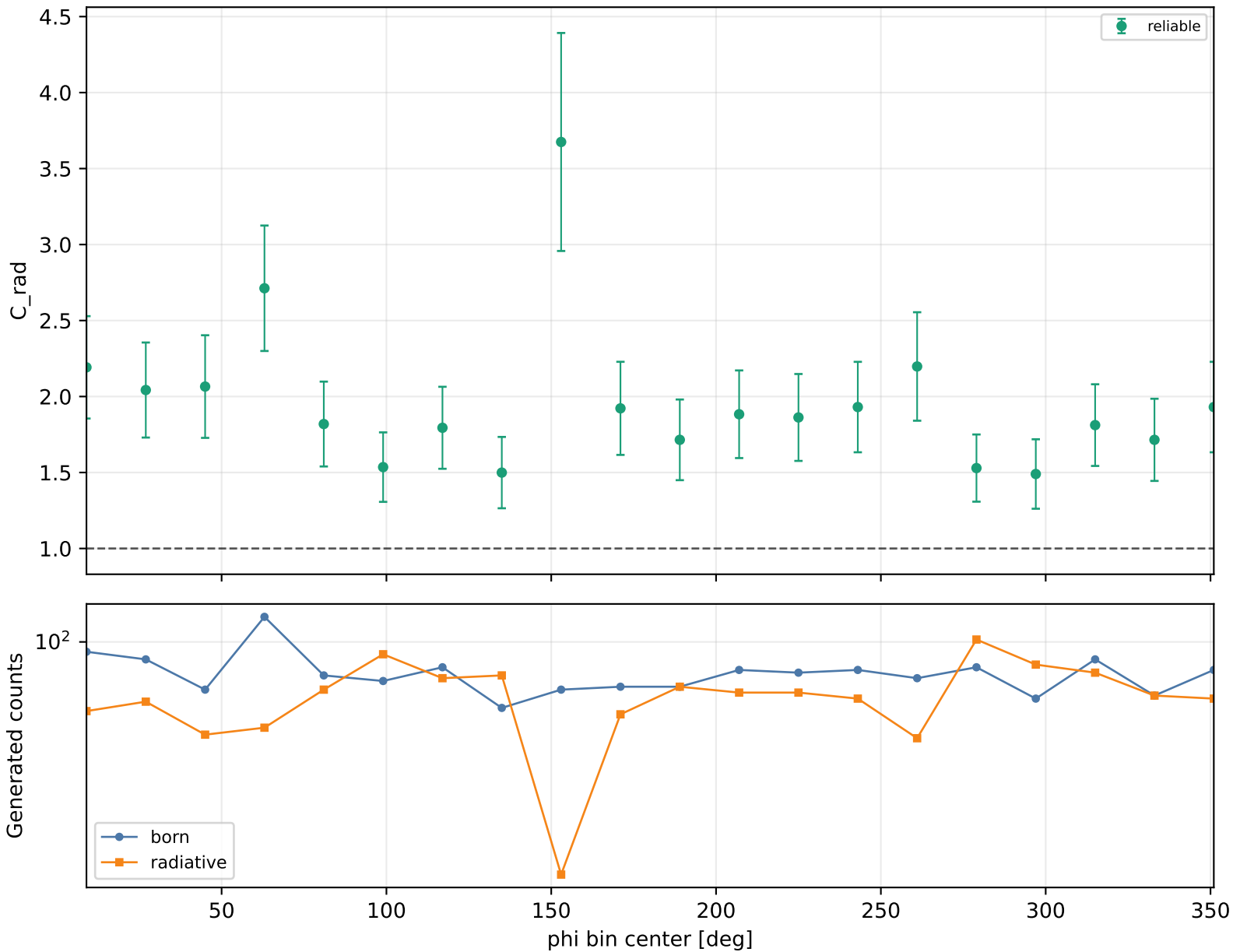
Radiative correction vs phi Q2 3.5-4, xB 0.48-0.58, -t 0.3-0.4
