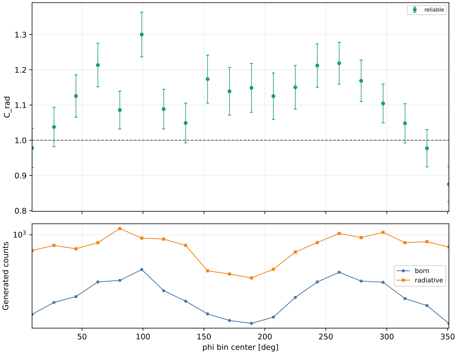
Radiative correction vs phi Q2 4.6-5.5, xB 0.48-0.58, -t 1.5-2
