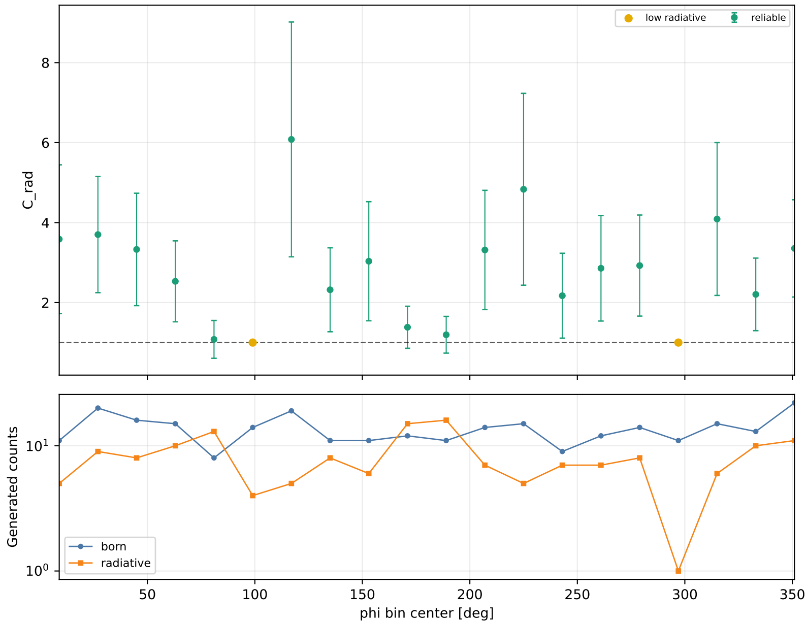
Radiative correction vs phi Q2 3.5-4, xB 0.58-0.7, -t 0.4-0.6
