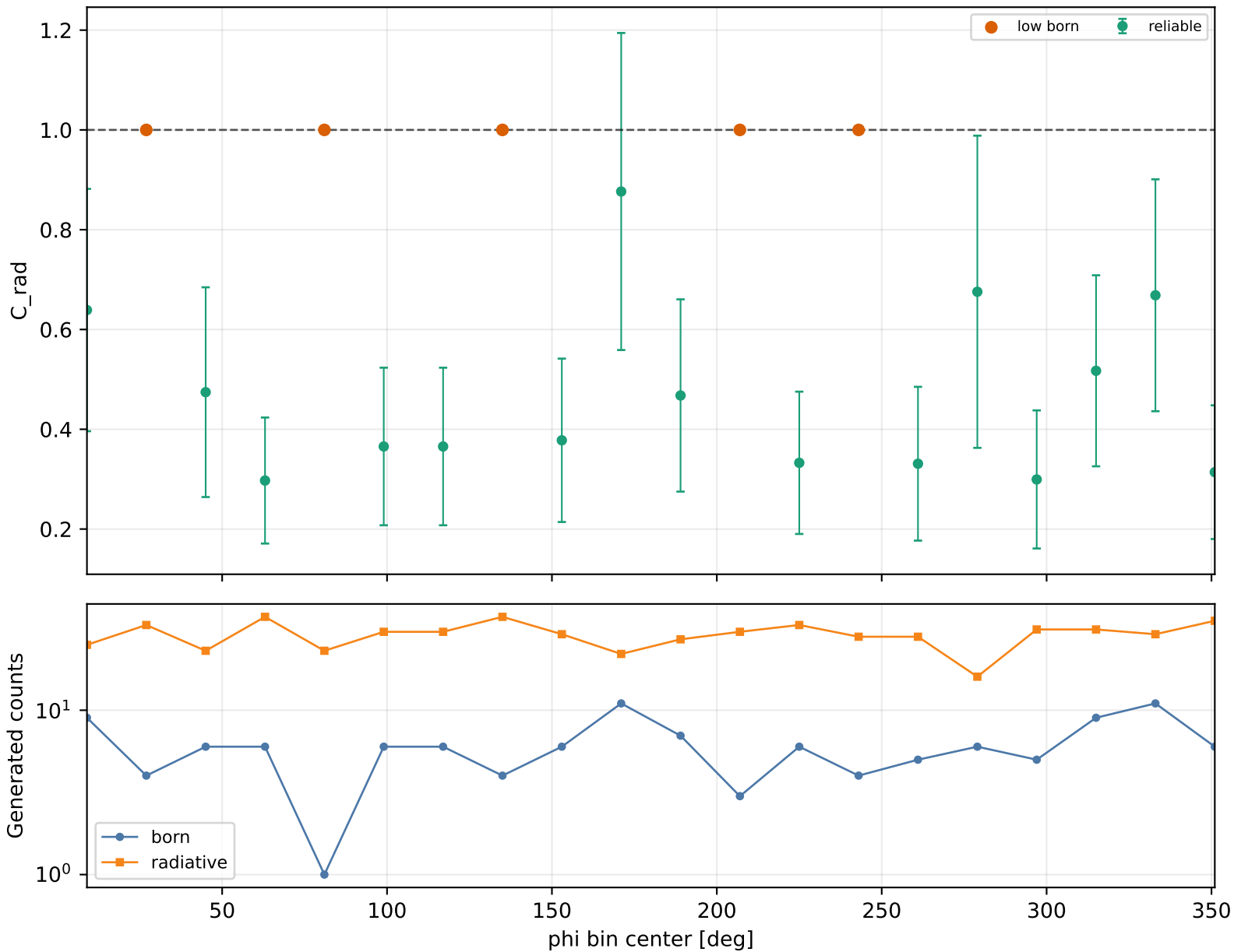
Radiative correction vs phi Q2 2.5-3, xB 0.2-0.25, -t 0.09-0.15
