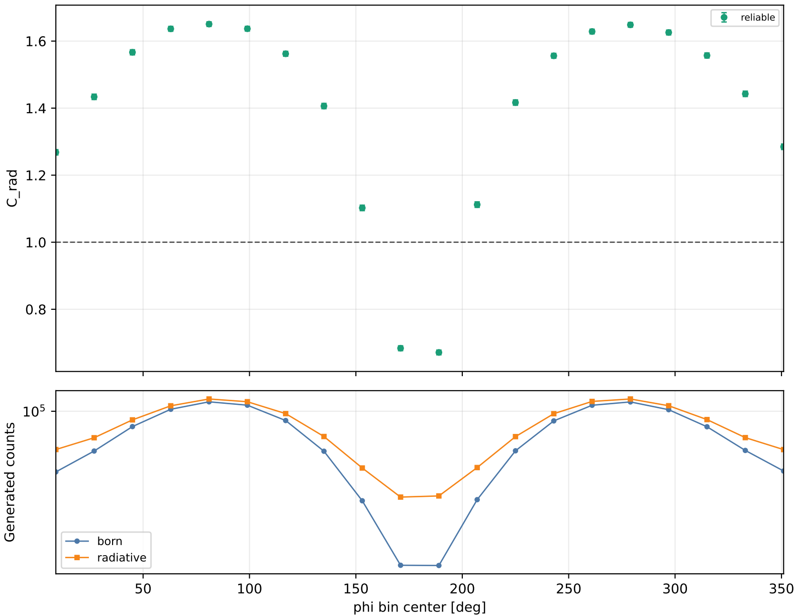
Radiative correction vs phi Q2 1-1.5, xB 0.25-0.3, -t 0.4-0.6
