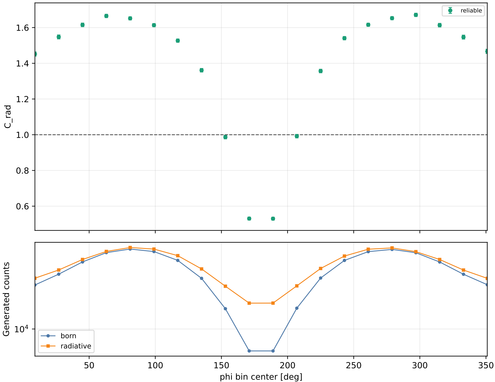
Radiative correction vs phi Q2 1-1.5, xB 0.25-0.3, -t 0.3-0.4
