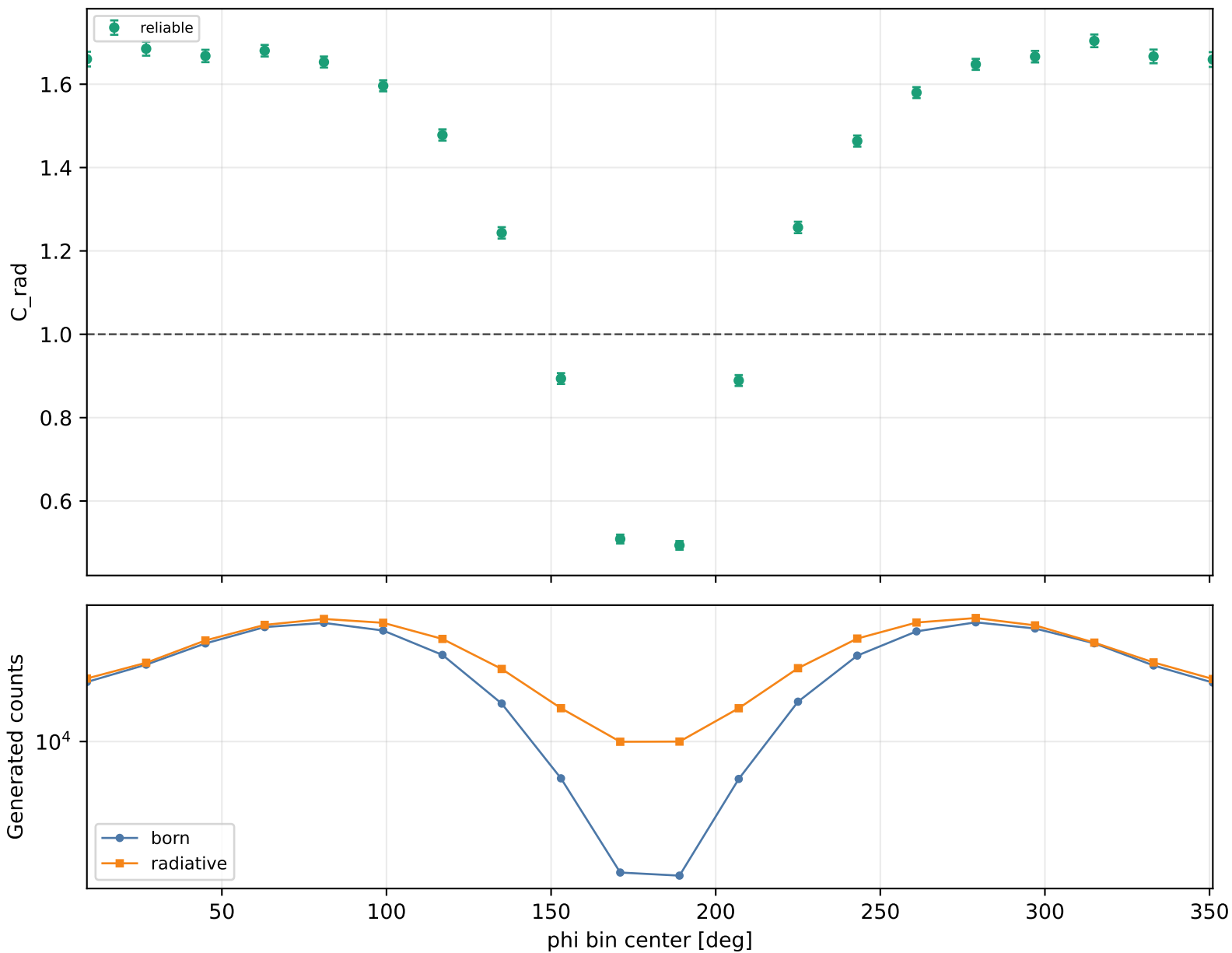
Radiative correction vs phi Q2 1-1.5, xB 0.25-0.3, -t 0.15-0.2
