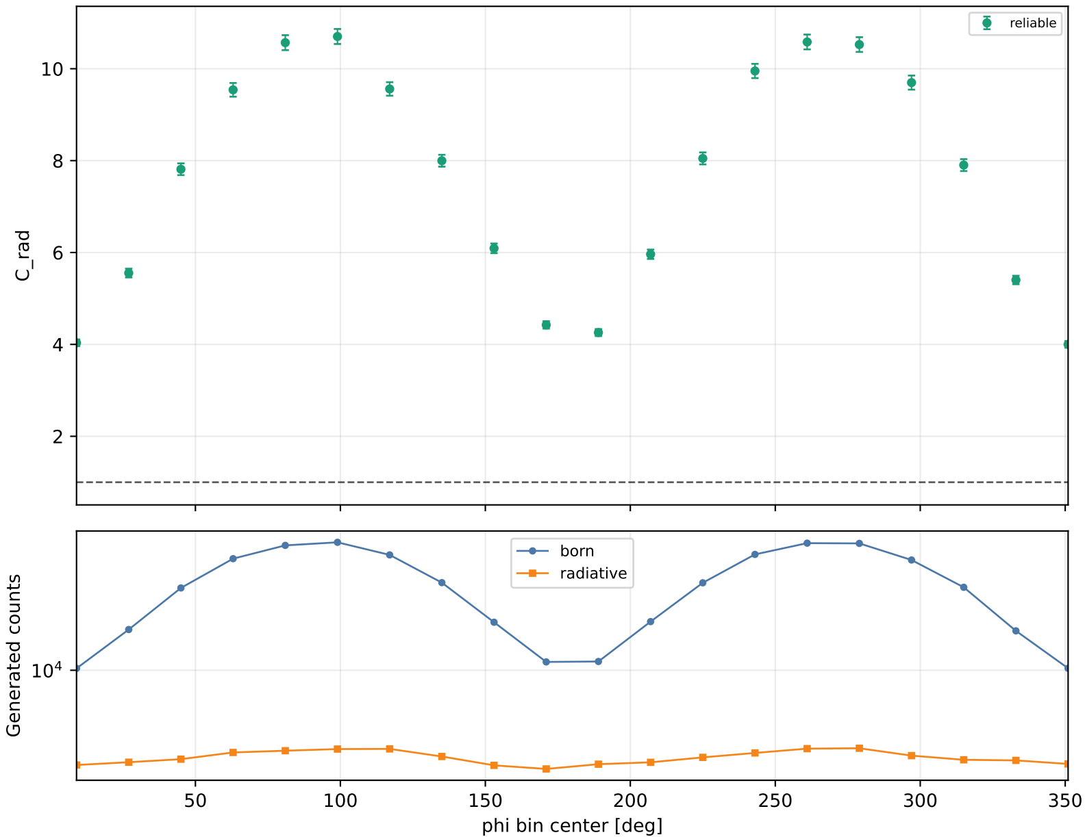
Radiative correction vs phi Q2 2-2.5, xB 0.58-0.7, -t 1.5-2
