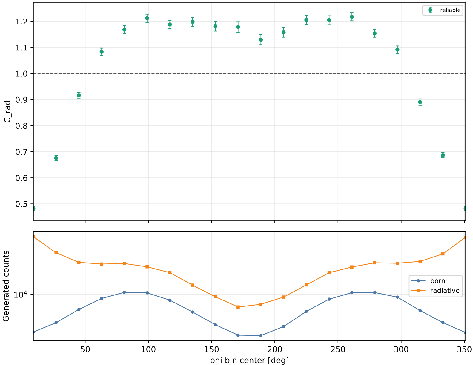
Radiative correction vs phi Q2 1.5-2, xB 0.3-0.38, -t 1.5-2
