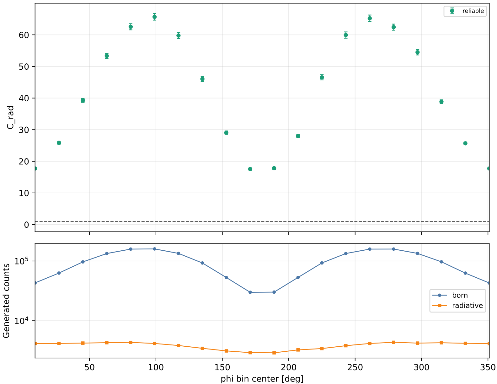
Radiative correction vs phi Q2 1.5-2, xB 0.48-0.58, -t 0.6-1
