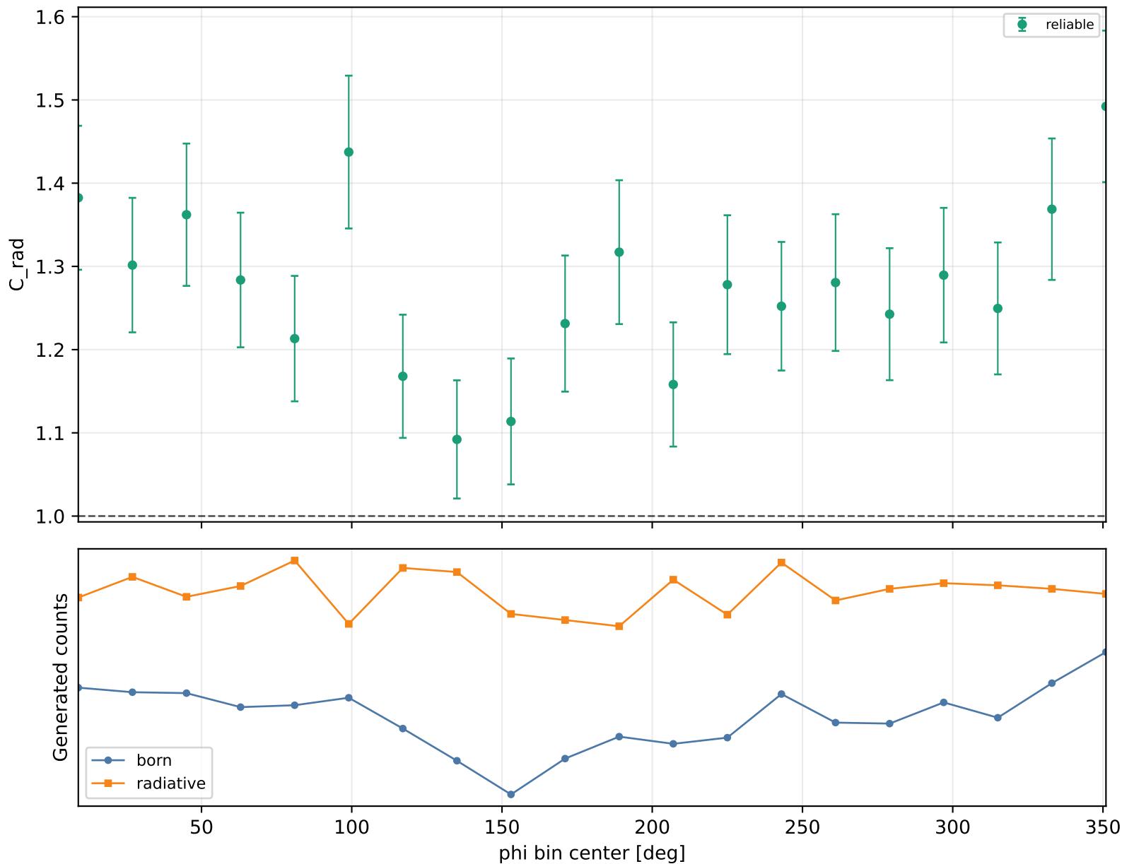
Radiative correction vs phi Q2 4.6-5.5, xB 0.48-0.58, -t 0.4-0.6
