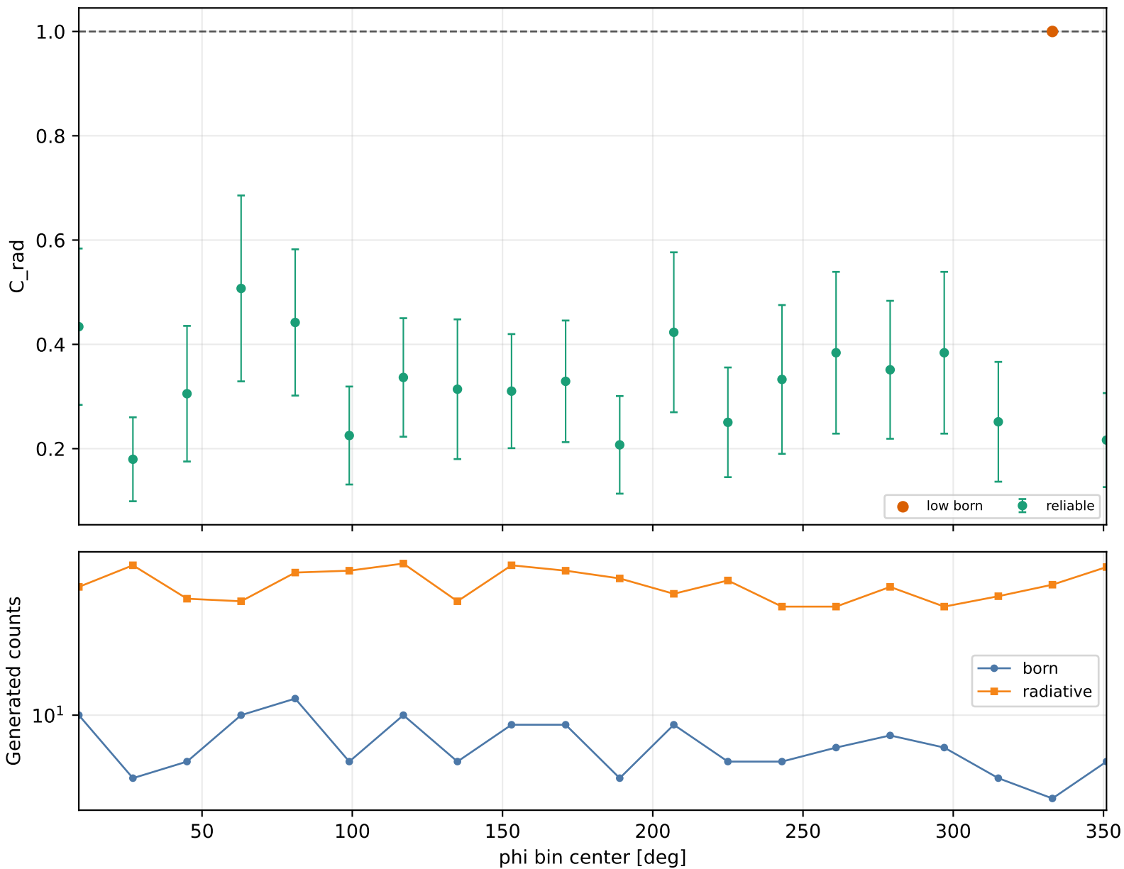
Radiative correction vs phi Q2 2-2.5, xB 0.15-0.2, -t 1-1.5
