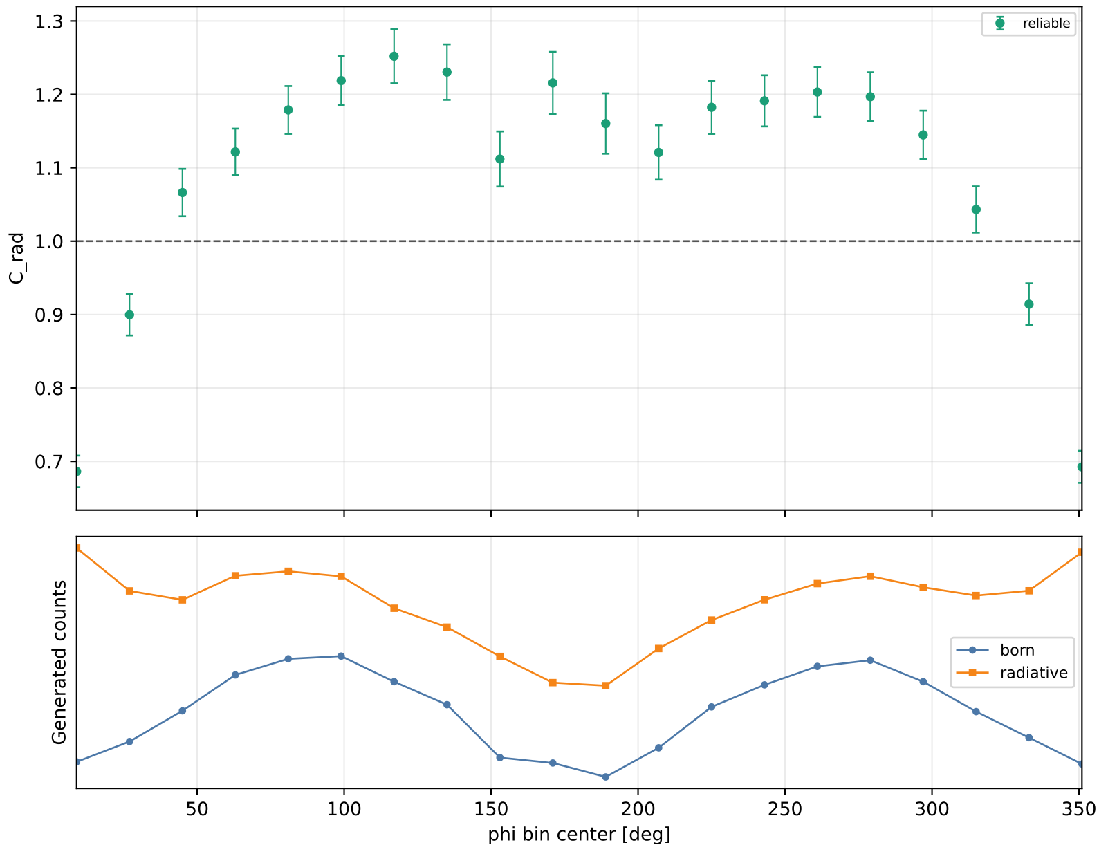
Radiative correction vs phi Q2 3-3.5, xB 0.38-0.48, -t 1.5-2
