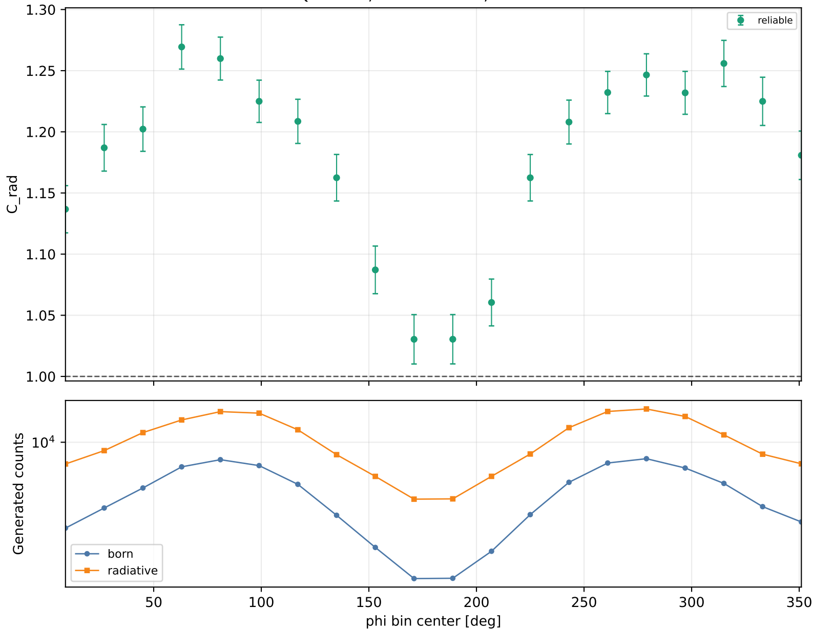
Radiative correction vs phi Q2 2.5-3, xB 0.38-0.48, -t 0.4-0.6
