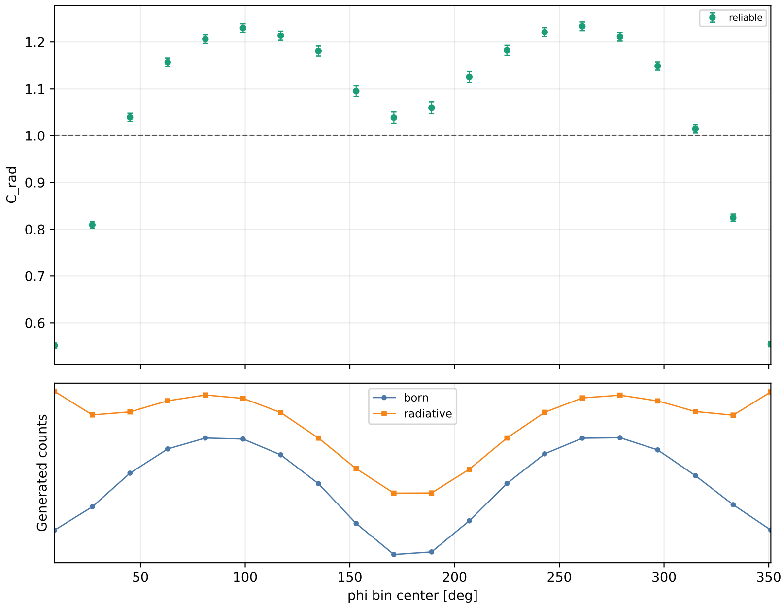
Radiative correction vs phi Q2 1.5-2, xB 0.3-0.38, -t 1-1.5
