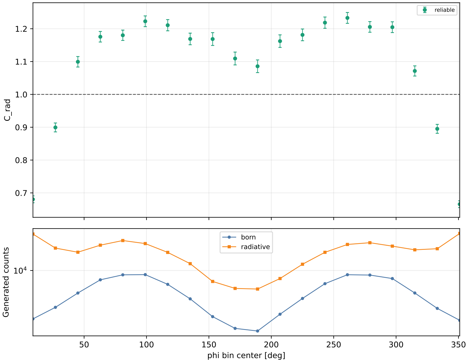
Radiative correction vs phi Q2 2-2.5, xB 0.3-0.38, -t 1-1.5
