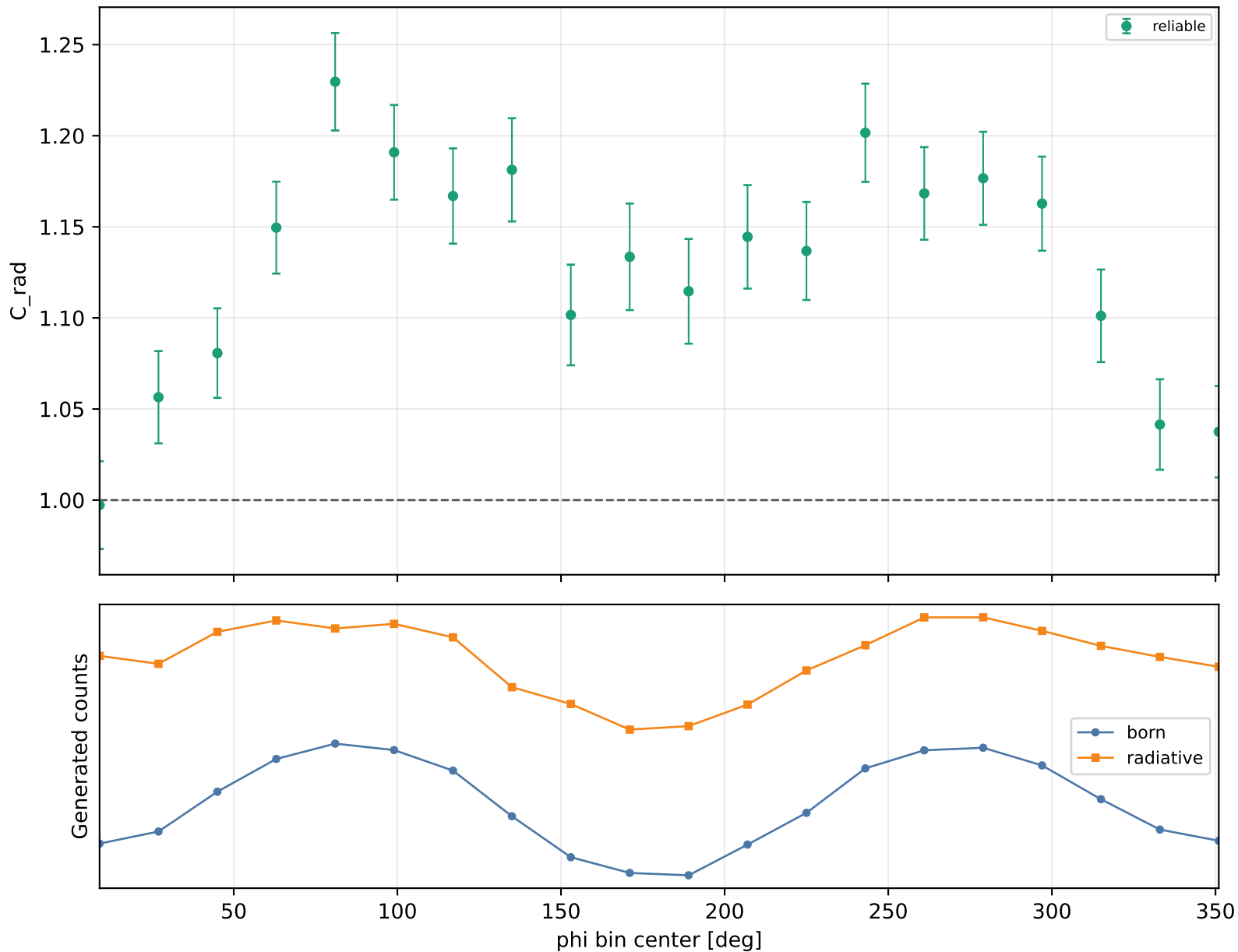
Radiative correction vs phi Q2 3.5-4, xB 0.38-0.48, -t 0.6-1
