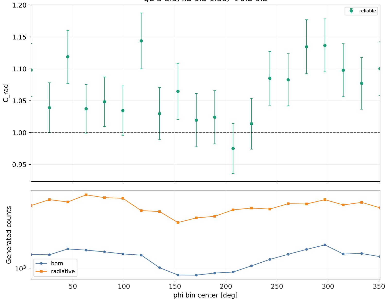
Radiative correction vs phi Q2 3-3.5, xB 0.3-0.38, -t 0.2-0.3
