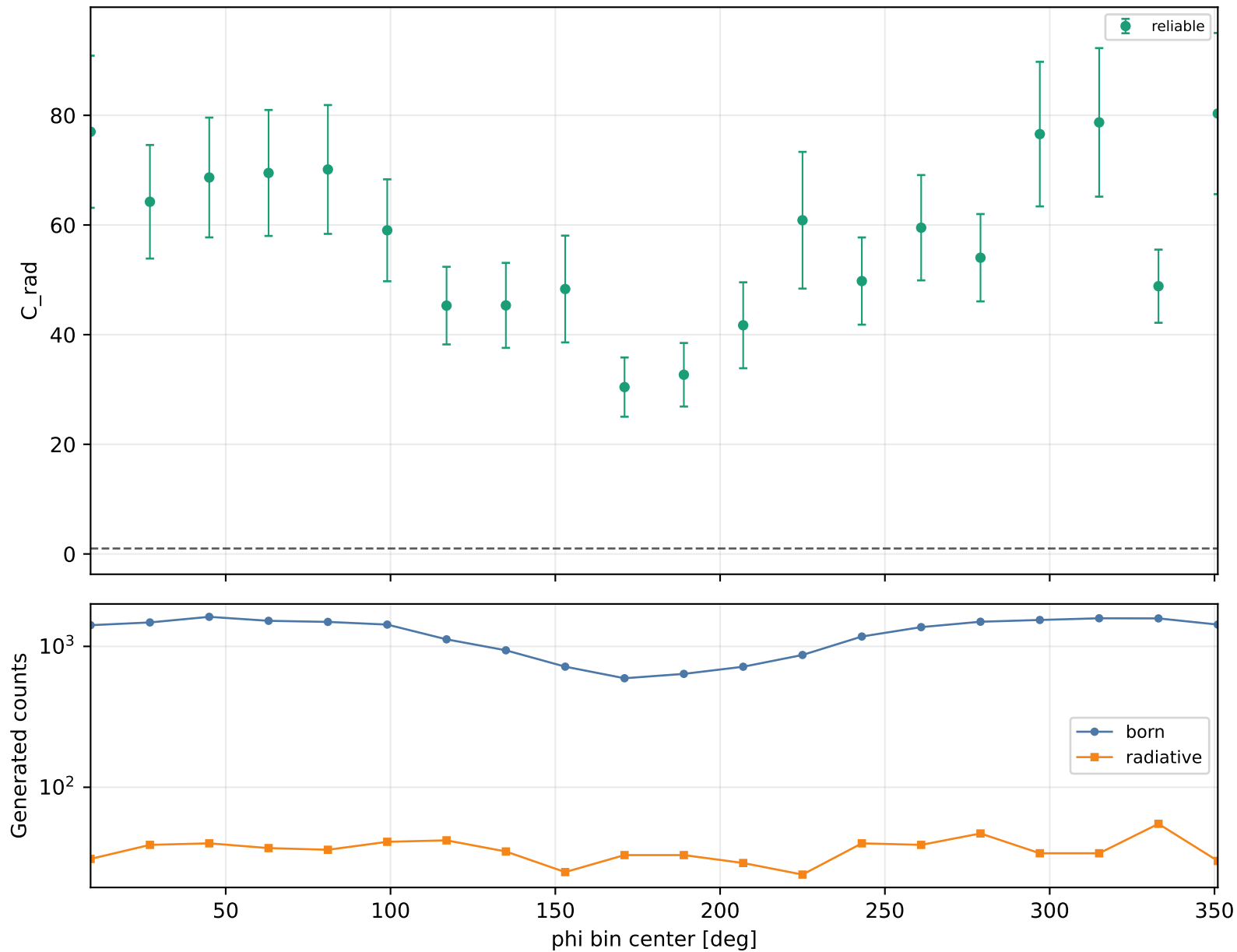
Radiative correction vs phi Q2 1-1.5, xB 0.38-0.48, -t 0.15-0.2
