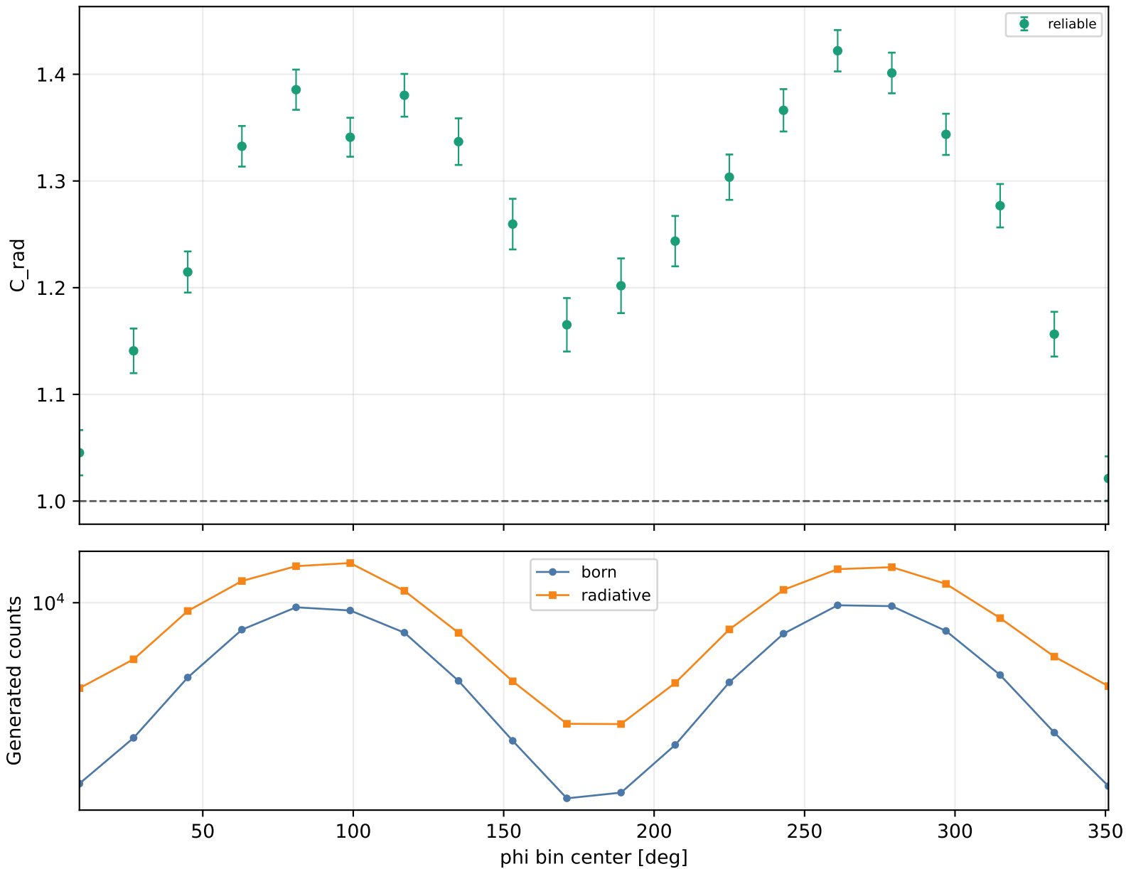
Radiative correction vs phi Q2 3-3.5, xB 0.48-0.58, -t 1-1.5
