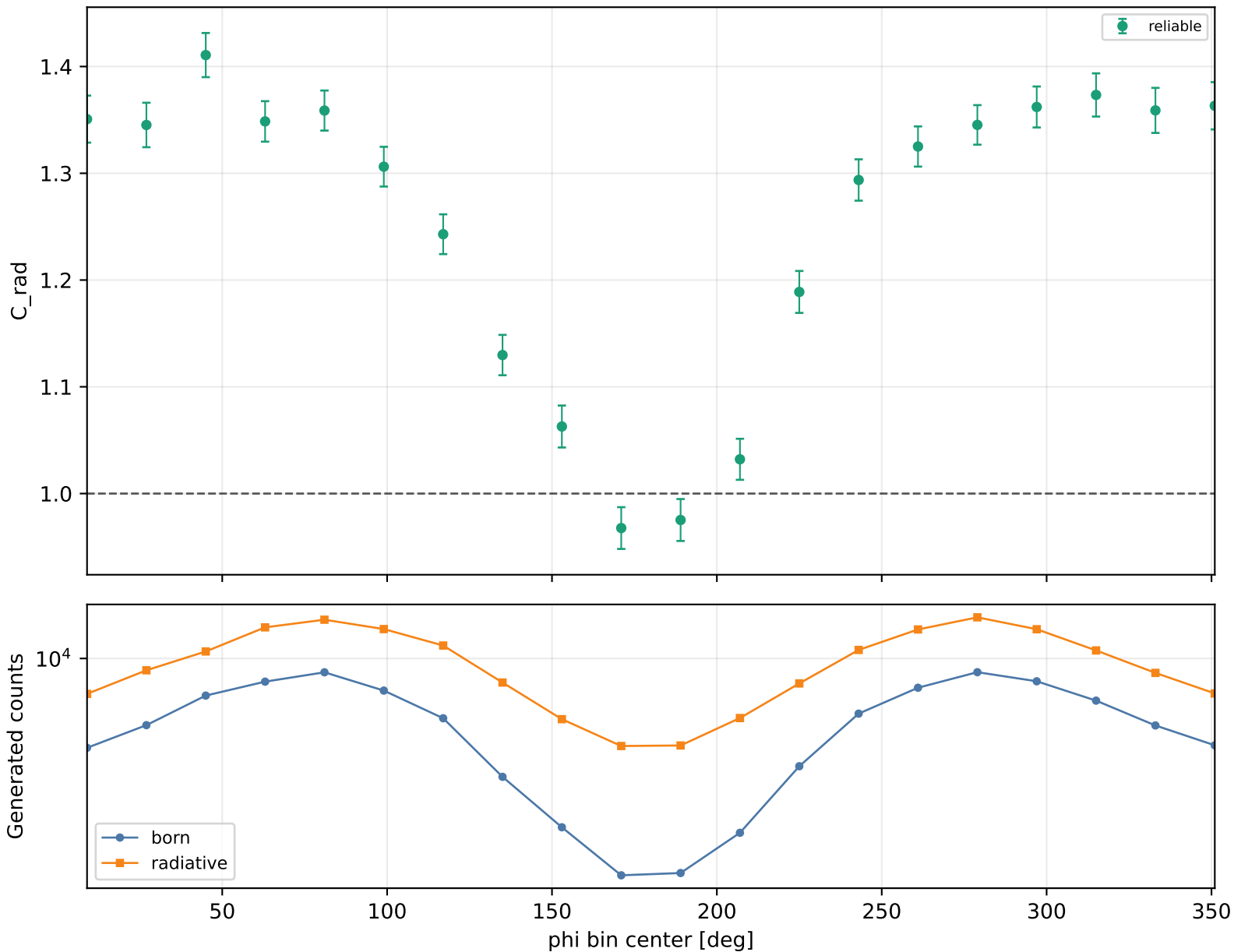
Radiative correction vs phi Q2 2-2.5, xB 0.38-0.48, -t 0.3-0.4
