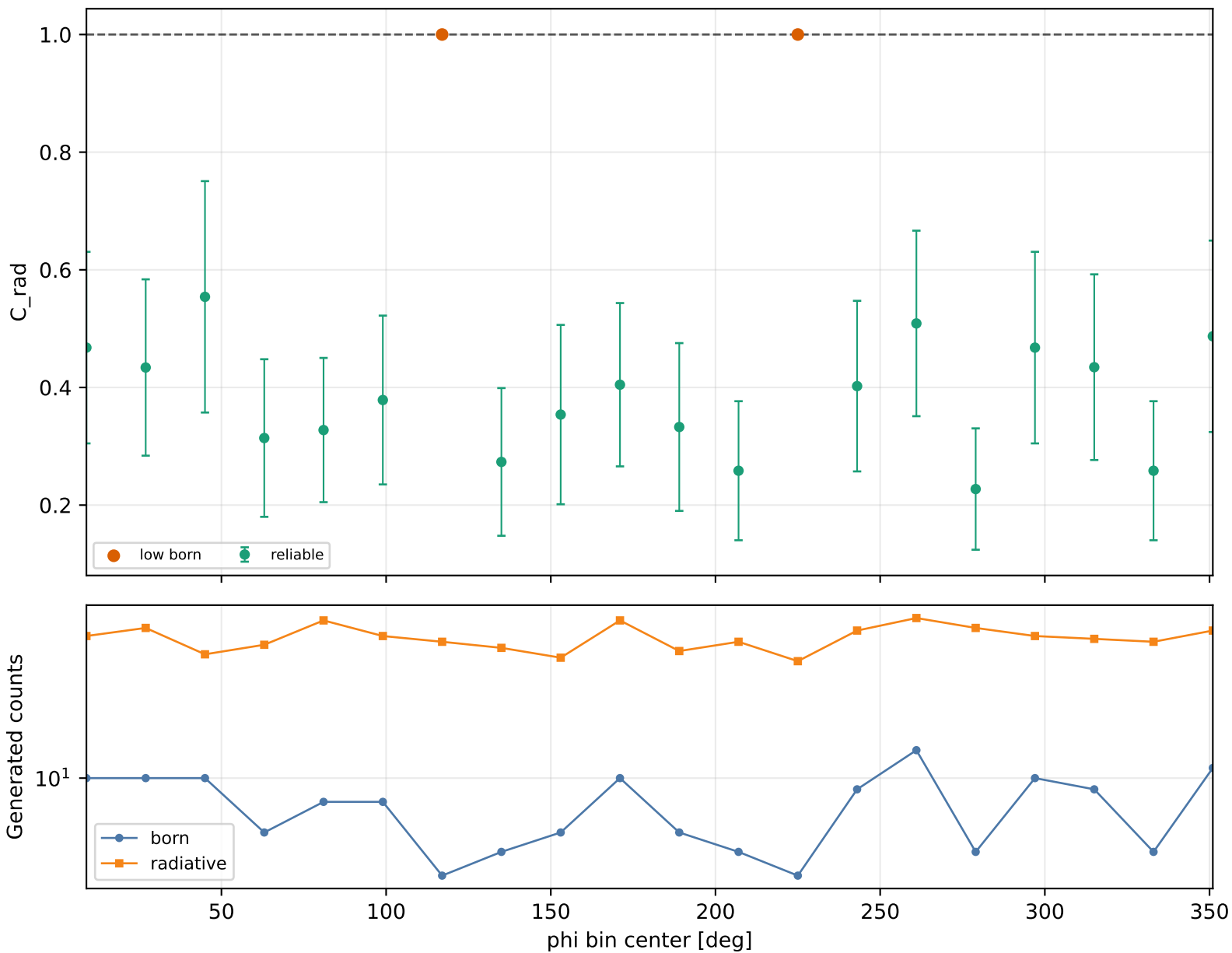
Radiative correction vs phi Q2 3-3.5, xB 0.25-0.3, -t 0.3-0.4
