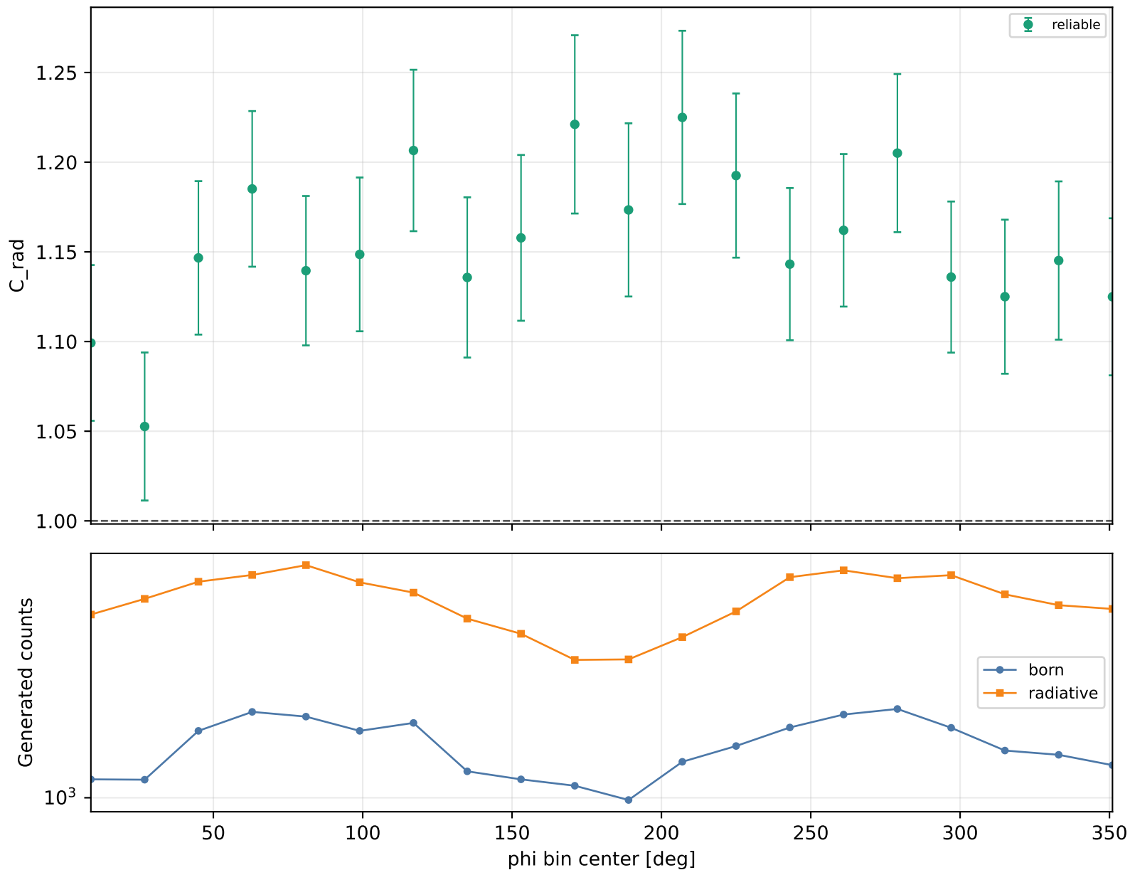
Radiative correction vs phi Q2 4.6-5.5, xB 0.48-0.58, -t 0.6-1
