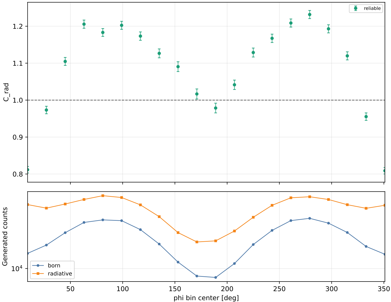
Radiative correction vs phi Q2 1.5-2, xB 0.25-0.3, -t 0.6-1
