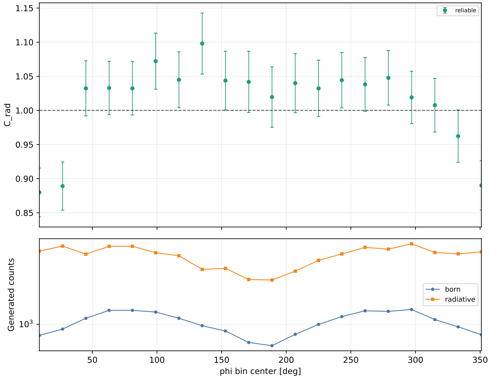
Radiative correction vs phi Q2 4-4.6, xB 0.38-0.48, -t 1-1.5
