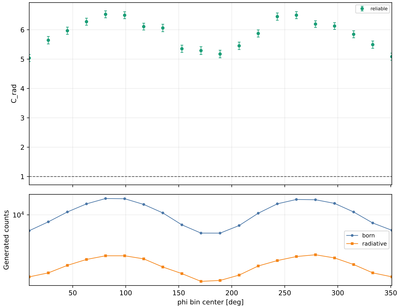
Radiative correction vs phi Q2 4-4.6, xB 0.58-0.7, -t 1-1.5
