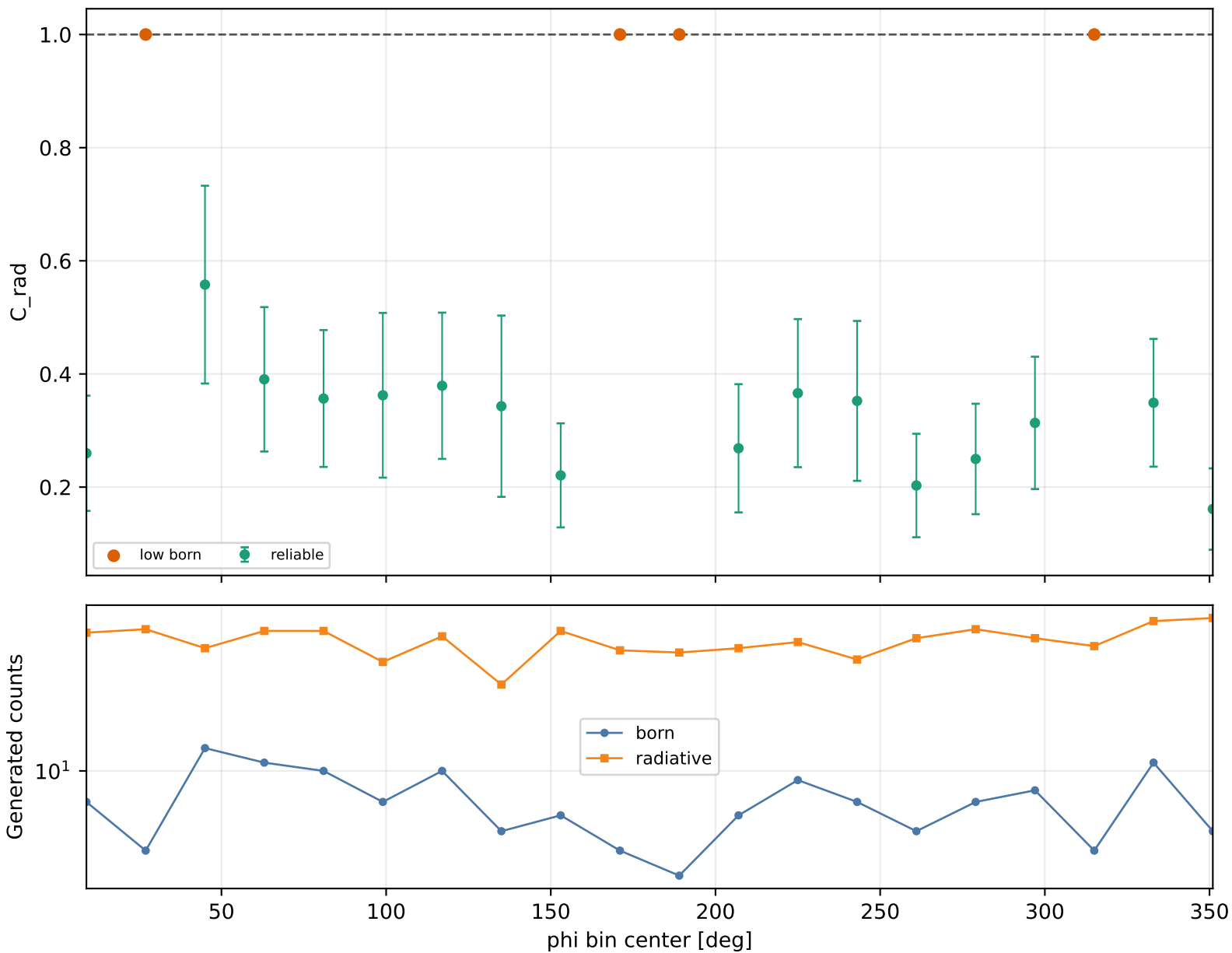
Radiative correction vs phi Q2 3-3.5, xB 0.25-0.3, -t 1-1.5
