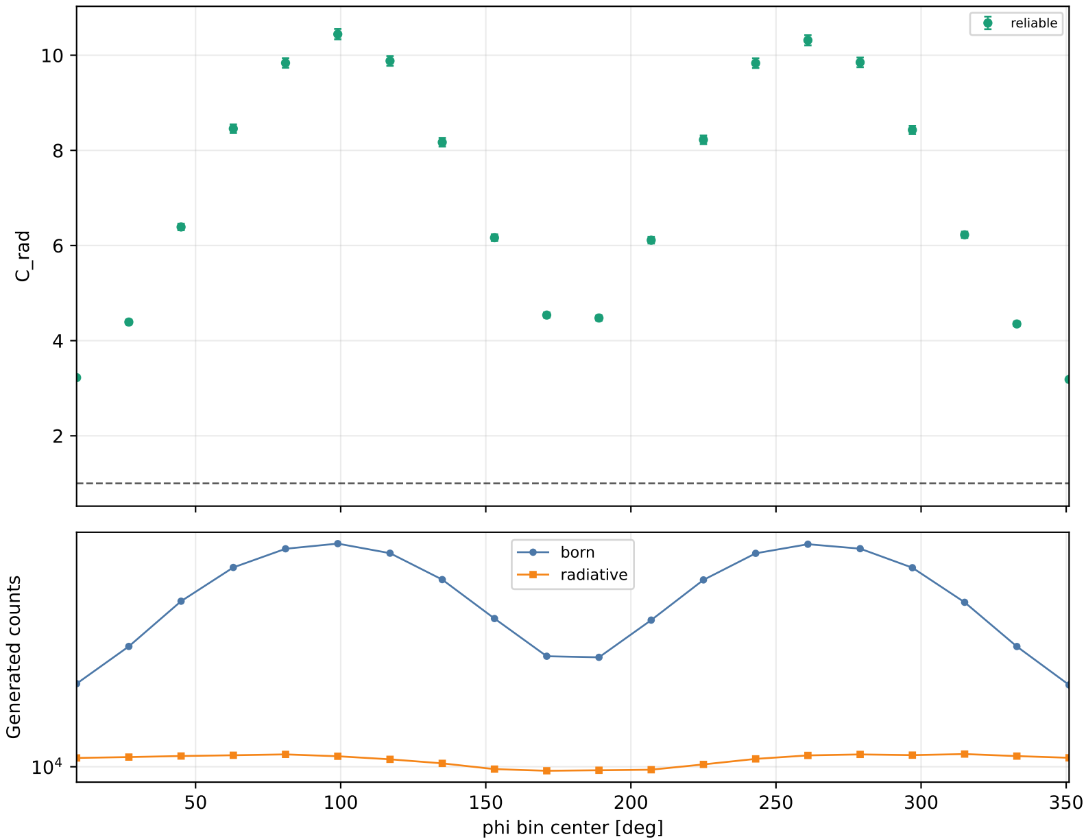
Radiative correction vs phi Q2 2.5-3, xB 0.58-0.7, -t 1-1.5
