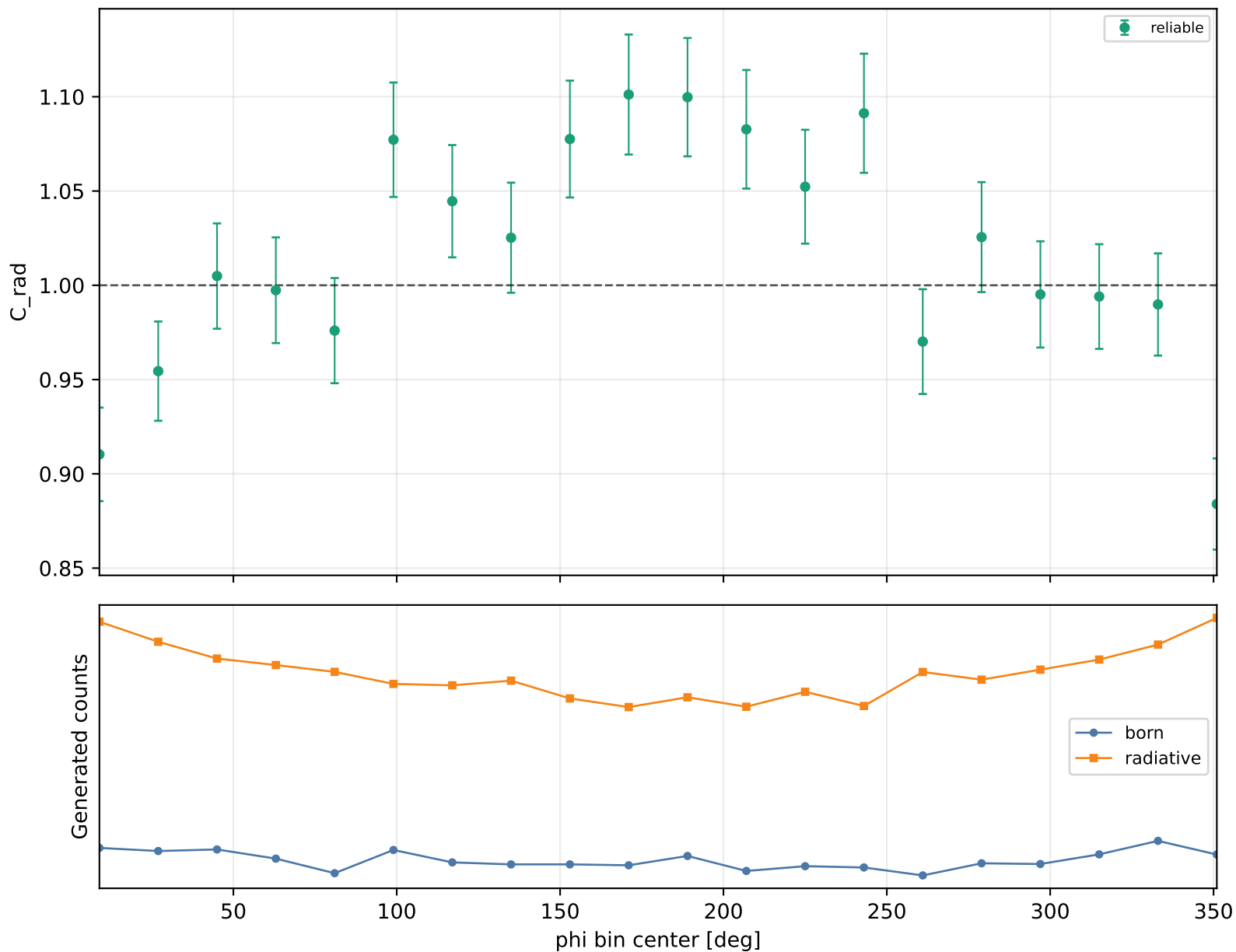
Radiative correction vs phi Q2 1-1.5, xB 0.1-0.15, -t 1.5-2
