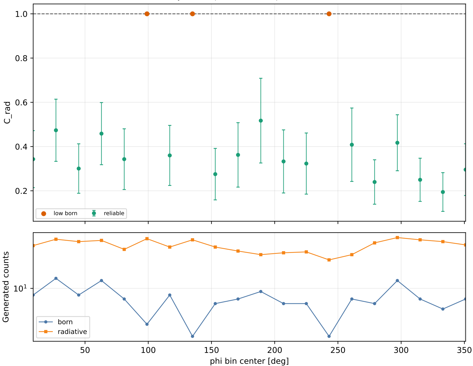
Radiative correction vs phi Q2 3-3.5, xB 0.25-0.3, -t 0.2-0.3
