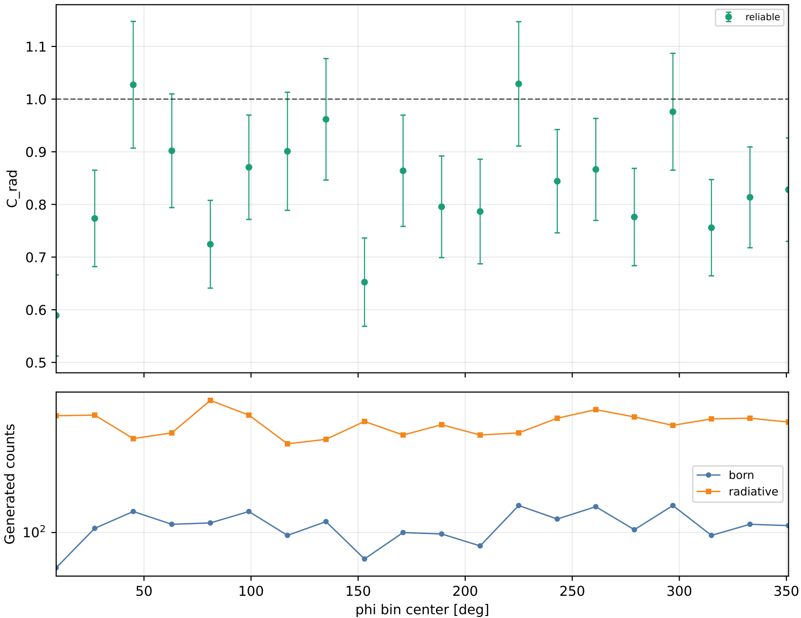
Radiative correction vs phi Q2 3.5-4, xB 0.3-0.38, -t 1.5-2
