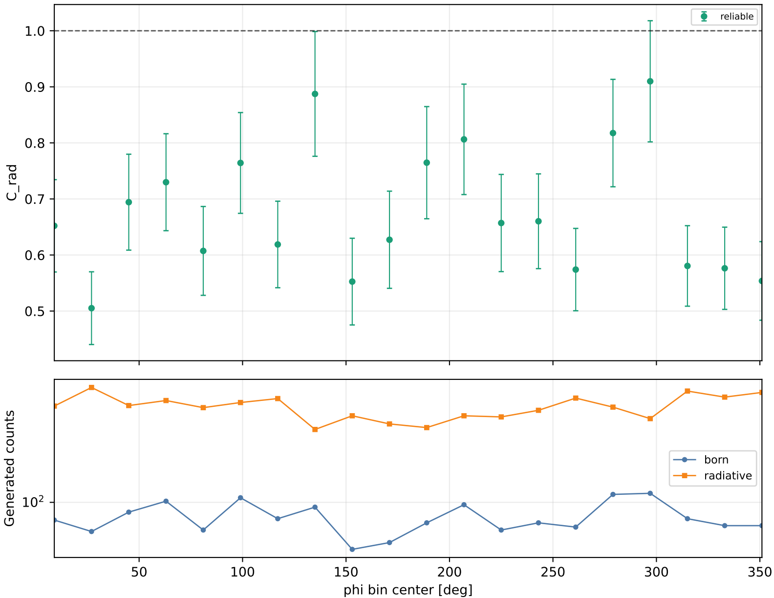
Radiative correction vs phi Q2 4.6-5.5, xB 0.38-0.48, -t 1-1.5
