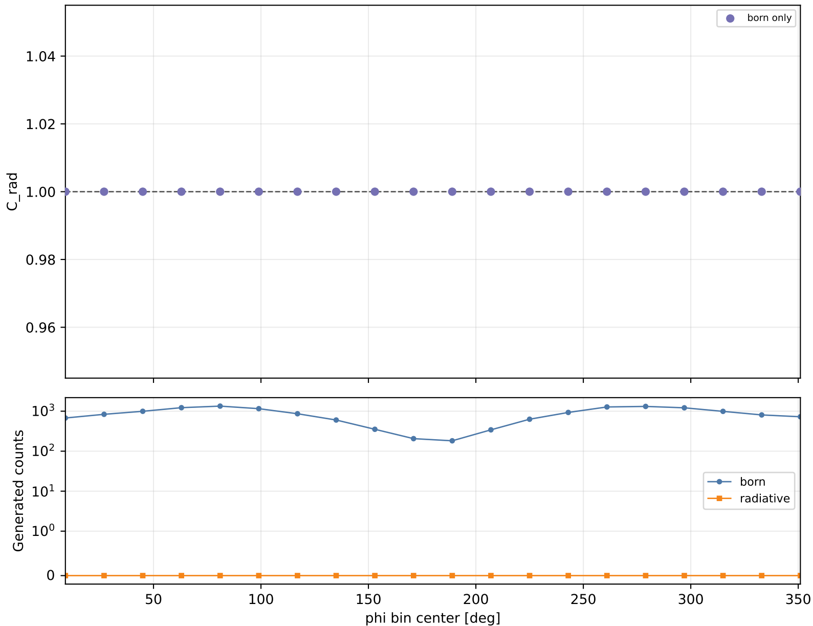
Radiative correction vs phi Q2 1-1.5, xB 0.48-0.58, -t 0.3-0.4
