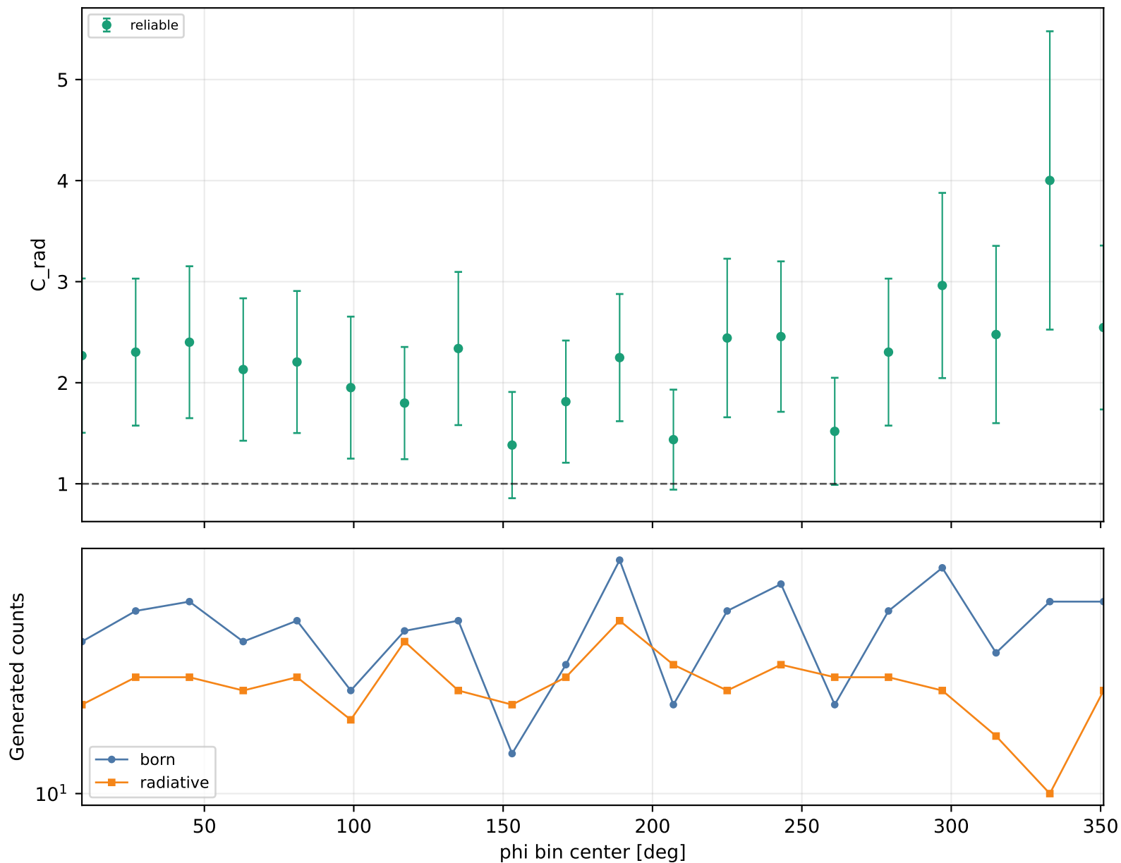
Radiative correction vs phi Q2 4.6-5.5, xB 0.48-0.58, -t 0.3-0.4
