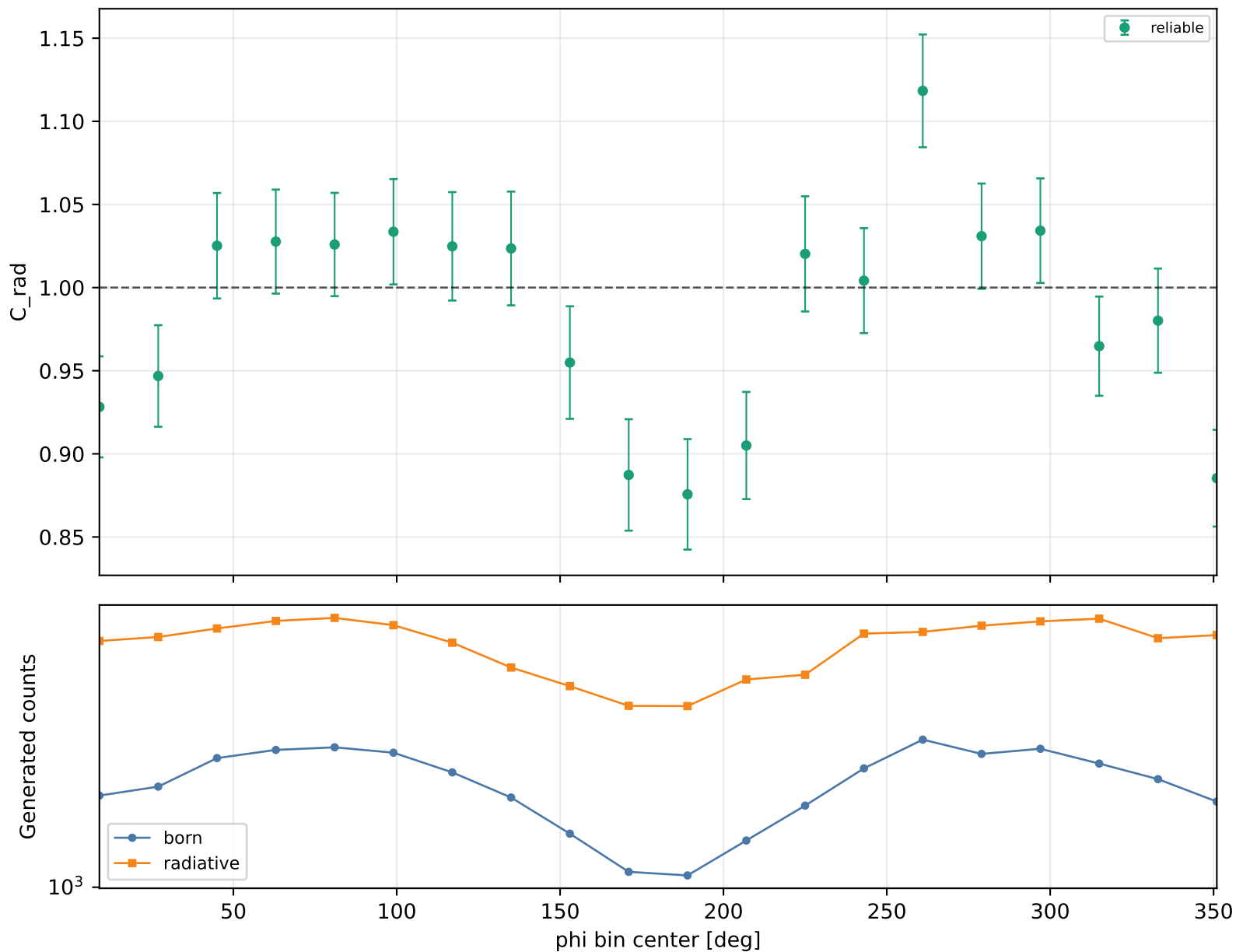
Radiative correction vs phi Q2 2-2.5, xB 0.2-0.25, -t 0.3-0.4
