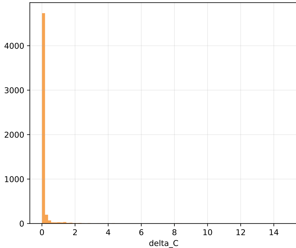
Correction uncertainty distribution
