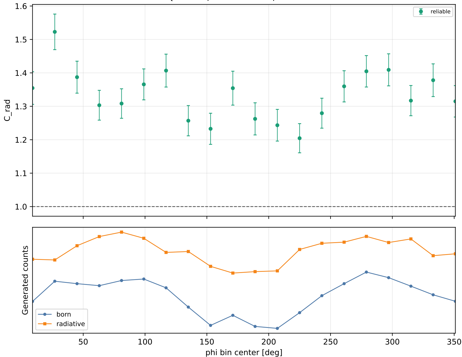
Radiative correction vs phi Q2 3.5-4, xB 0.48-0.58, -t 0.4-0.6
