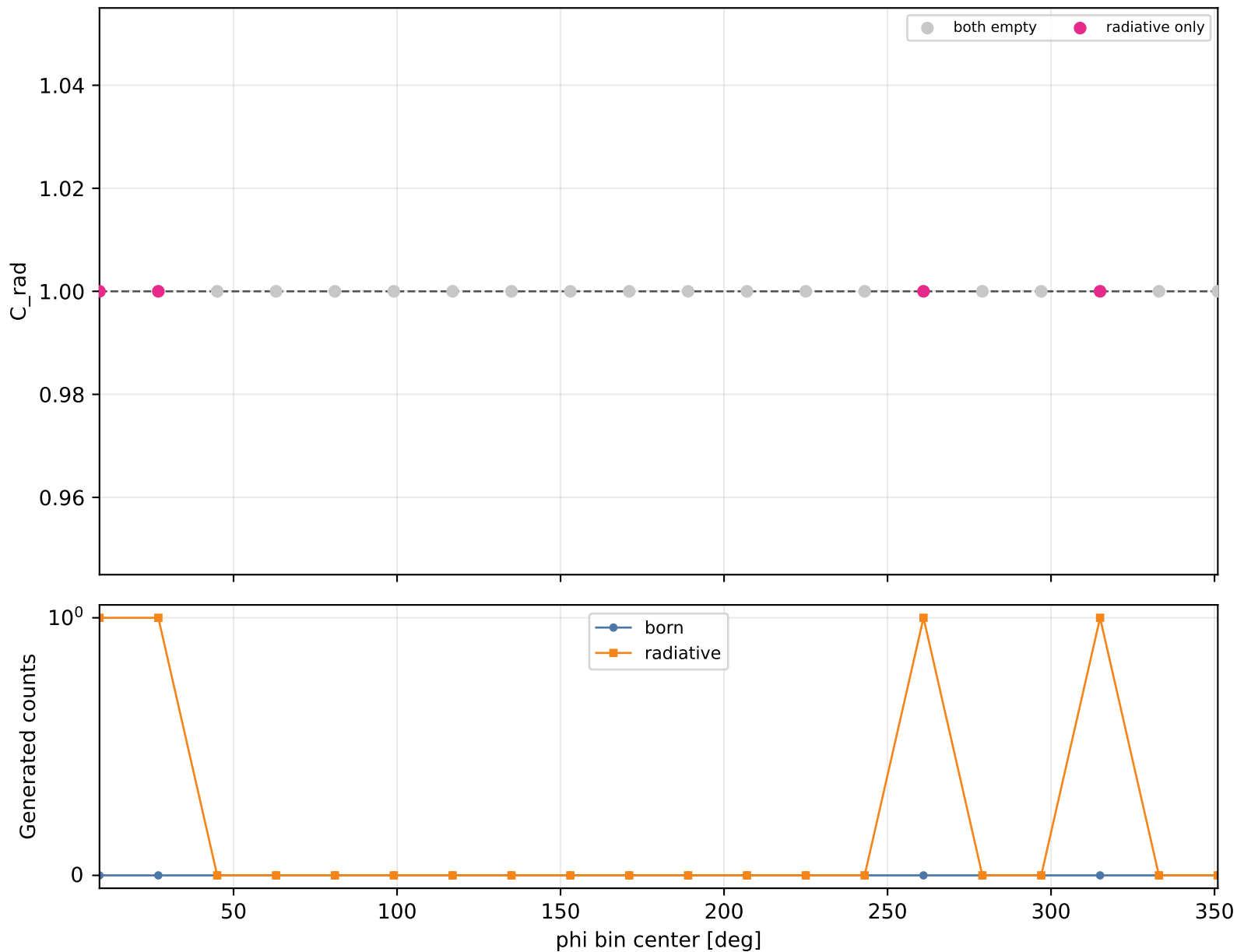
Radiative correction vs phi Q2 5.5-6.535, xB 0.58-0.7, -t 0.6-1
