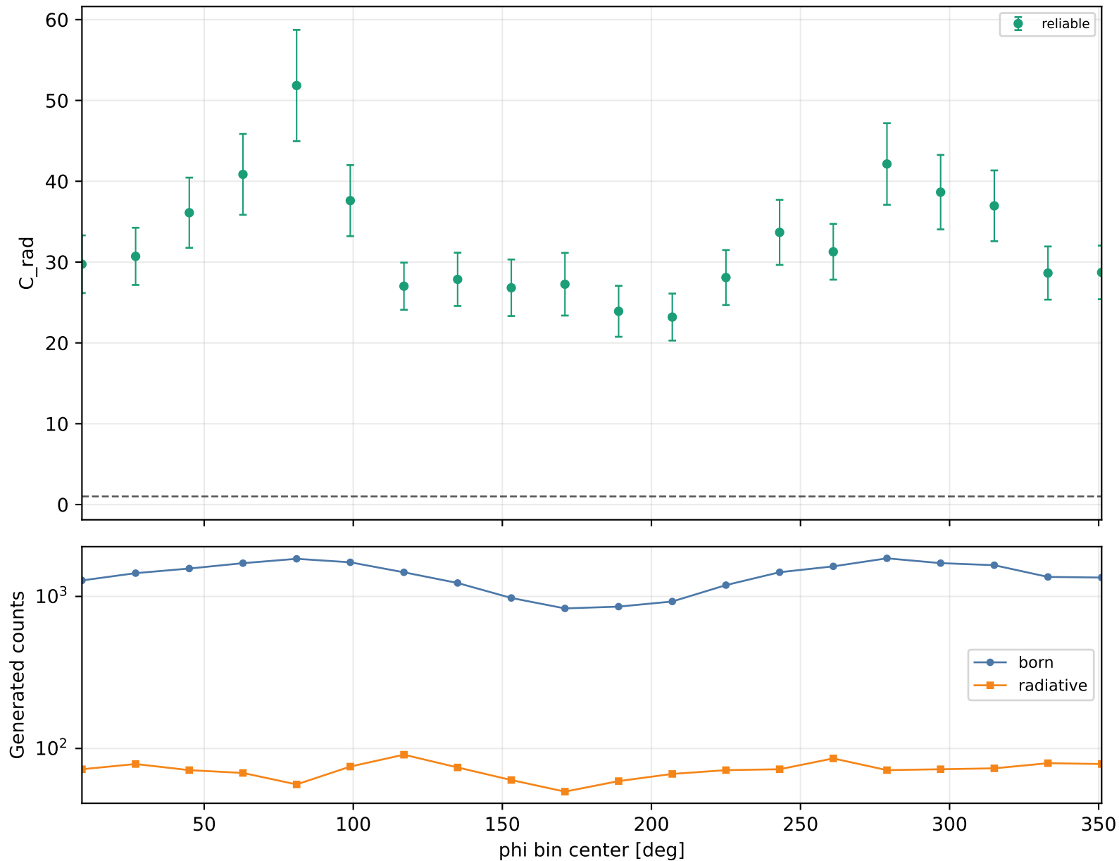
Radiative correction vs phi Q2 2-2.5, xB 0.58-0.7, -t 0.4-0.6
