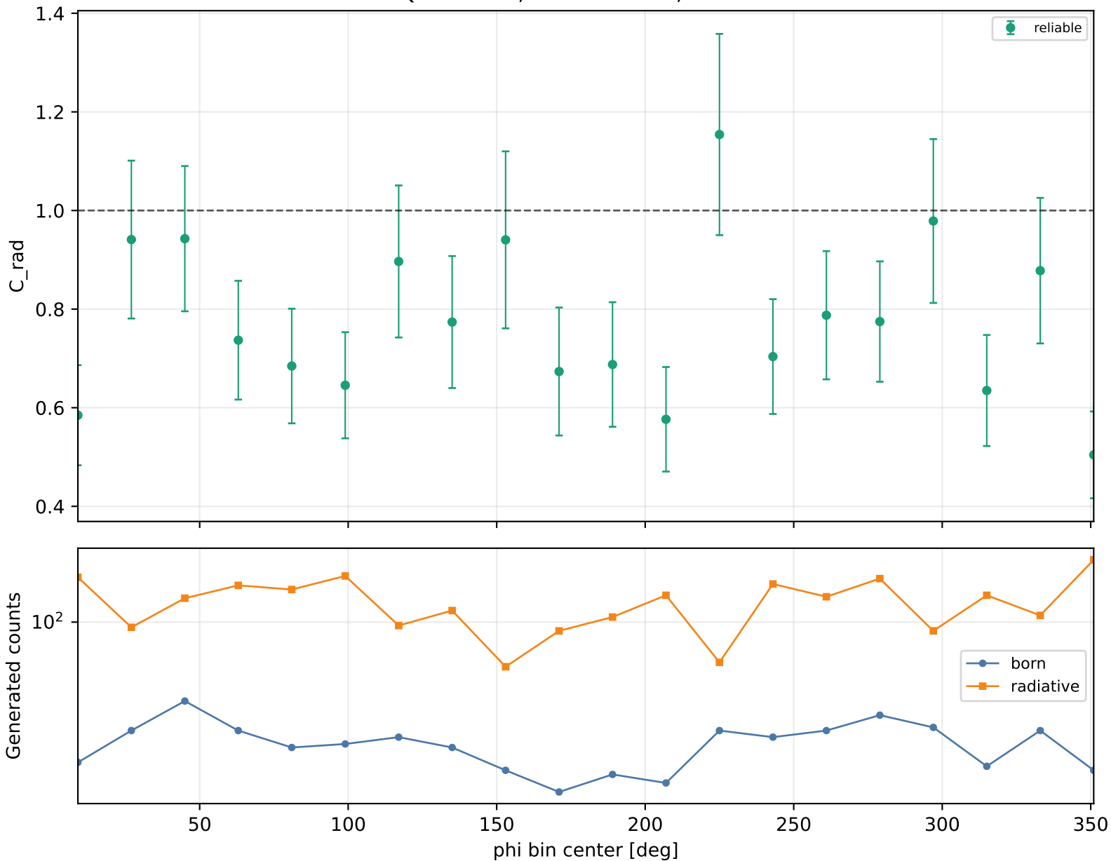
Radiative correction vs phi Q2 4.6-5.5, xB 0.38-0.48, -t 1.5-2
