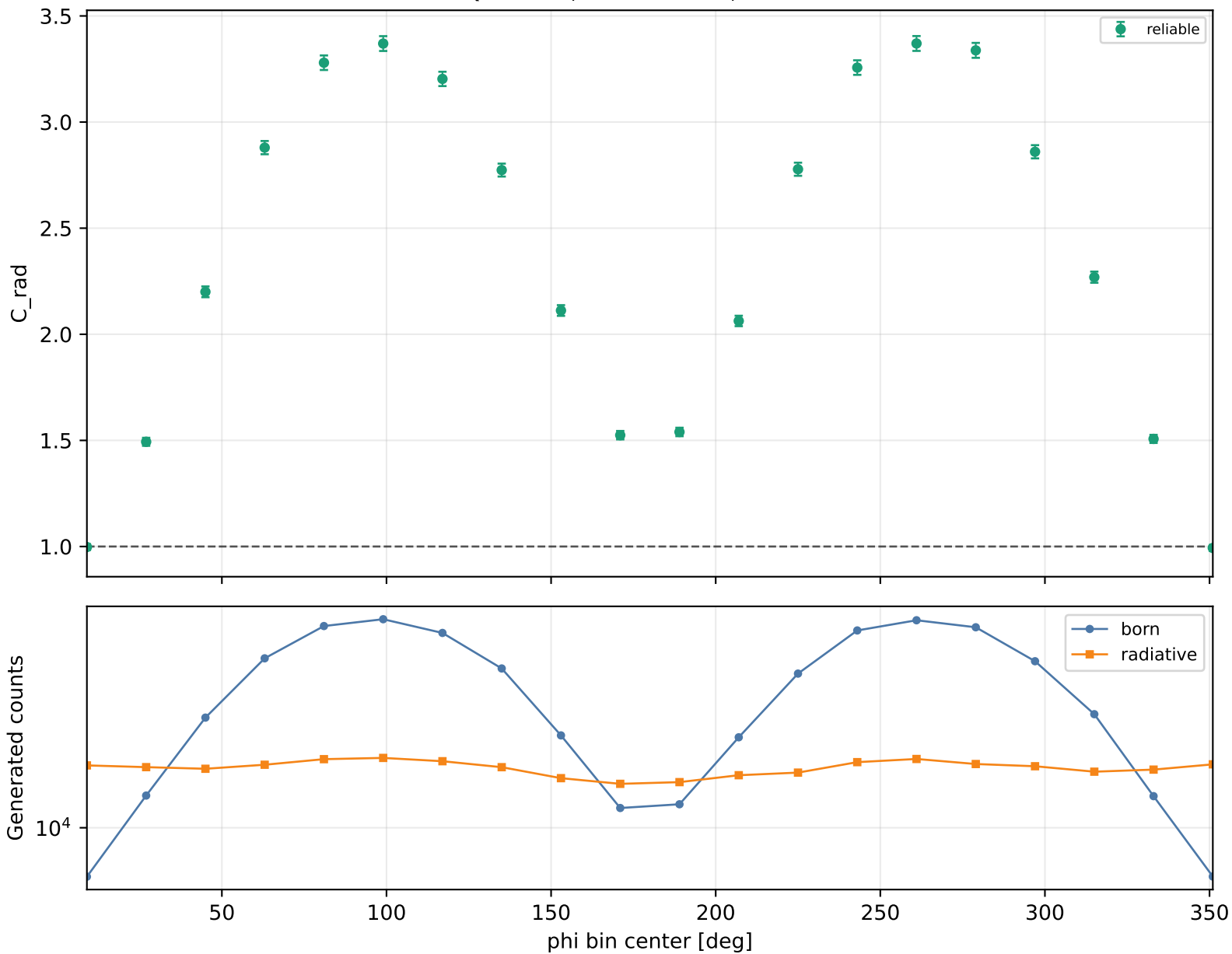
Radiative correction vs phi Q2 2.5-3, xB 0.58-0.7, -t 1.5-2
