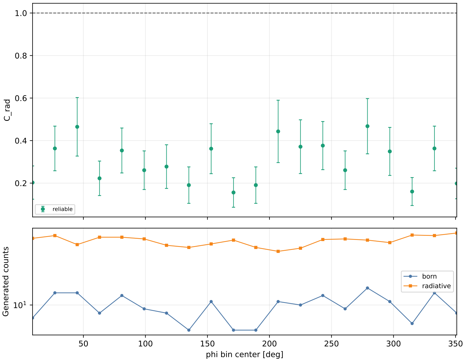
Radiative correction vs phi Q2 2-2.5, xB 0.15-0.2, -t 0.2-0.3
