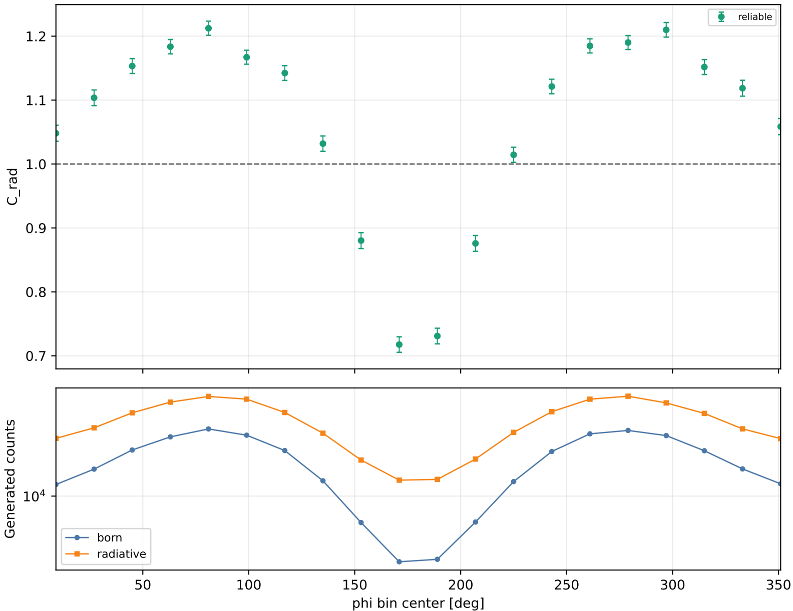
Radiative correction vs phi Q2 1-1.5, xB 0.15-0.2, -t 0.15-0.2
