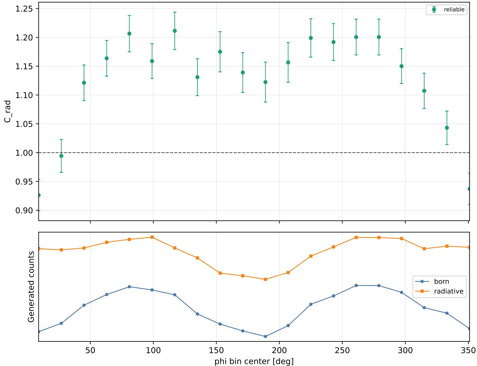
Radiative correction vs phi Q2 3.5-4, xB 0.38-0.48, -t 1-1.5
