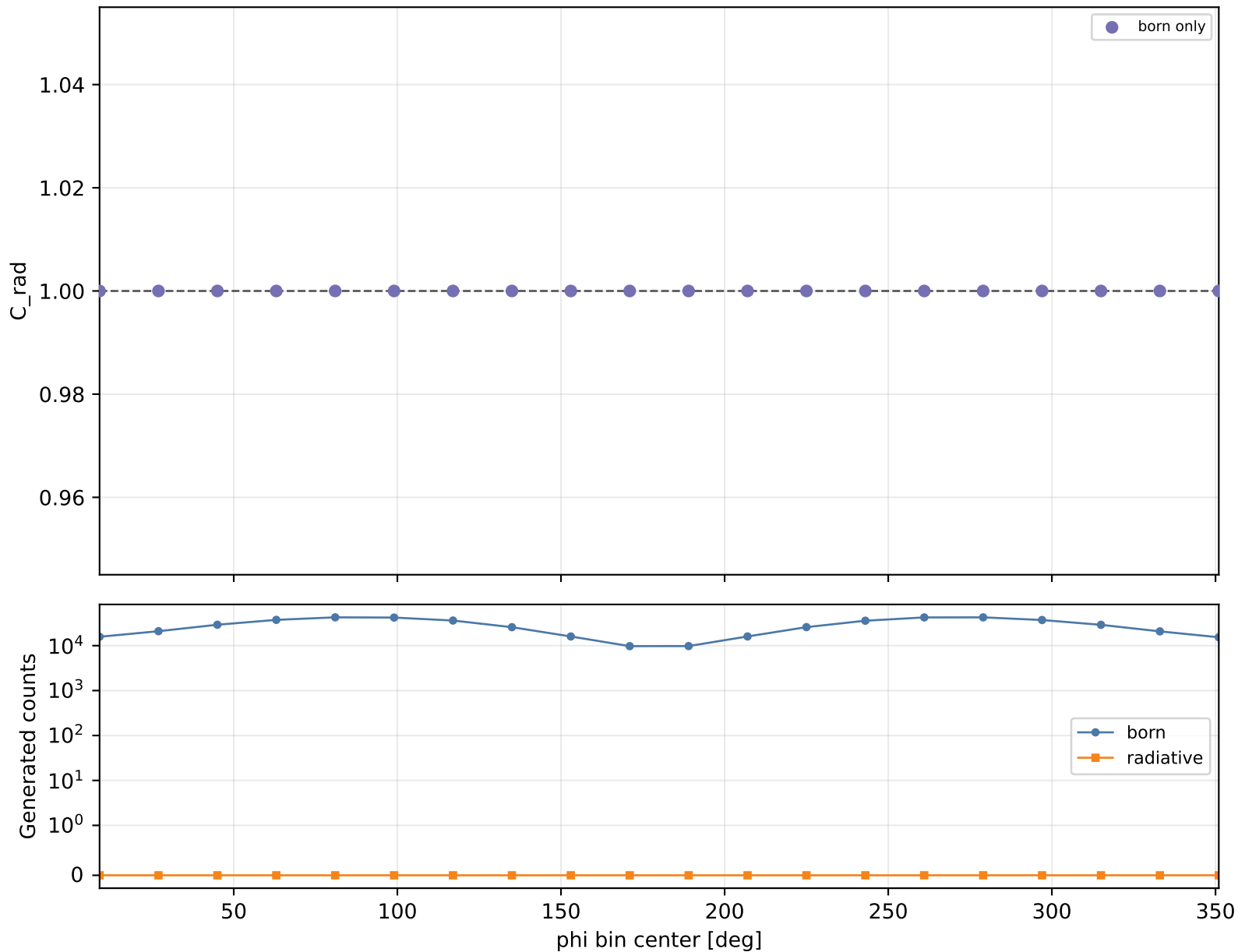
Radiative correction vs phi Q2 1.5-2, xB 0.58-0.7, -t 0.6-1
