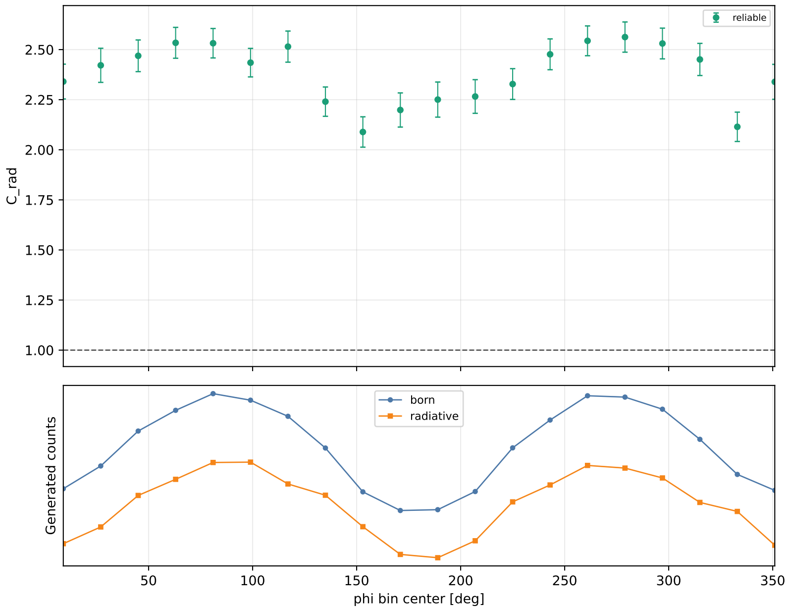
Radiative correction vs phi Q2 4.6-5.5, xB 0.58-0.7, -t 1-1.5
