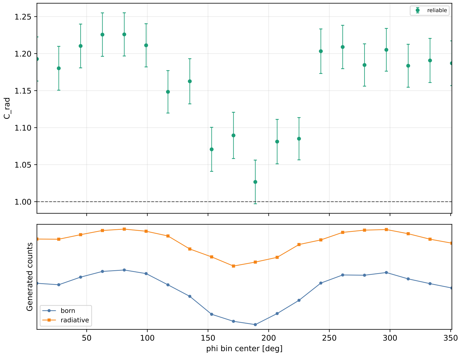
Radiative correction vs phi Q2 2.5-3, xB 0.3-0.38, -t 0.2-0.3
