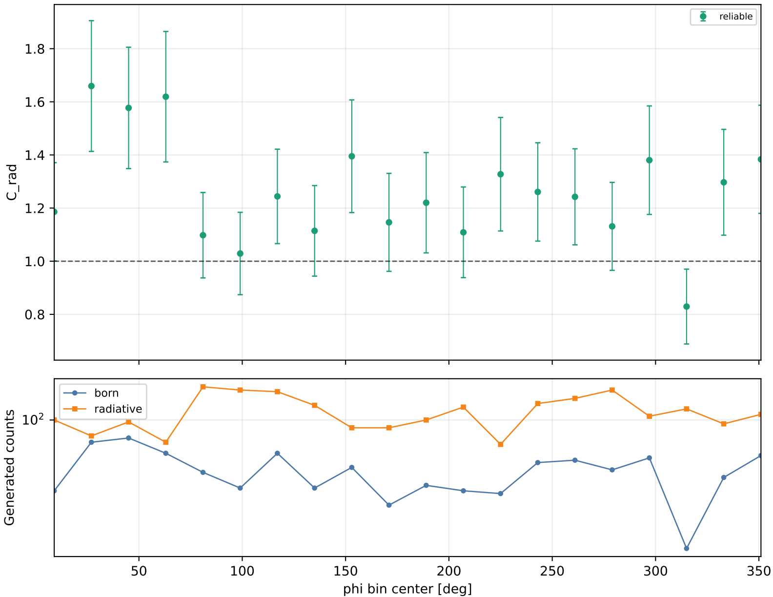
Radiative correction vs phi Q2 3-3.5, xB 0.3-0.38, -t 0.09-0.15
