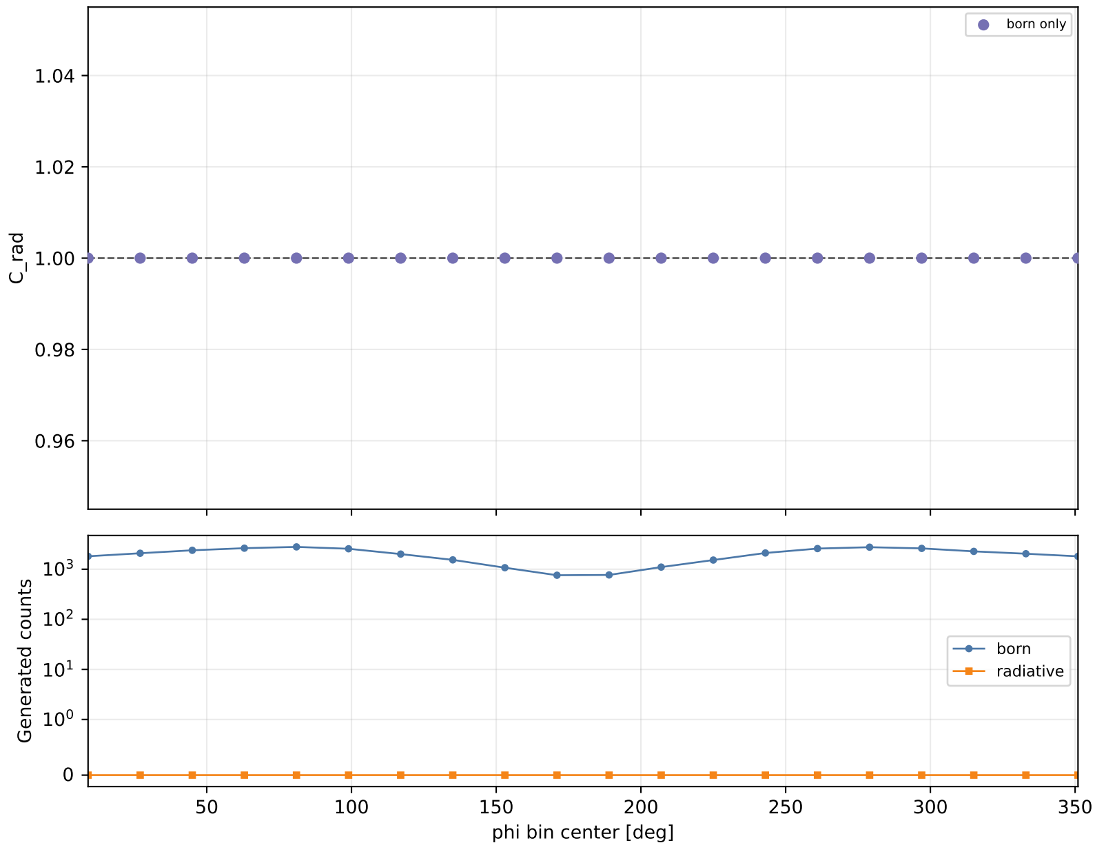
Radiative correction vs phi Q2 1.5-2, xB 0.58-0.7, -t 0.4-0.6
