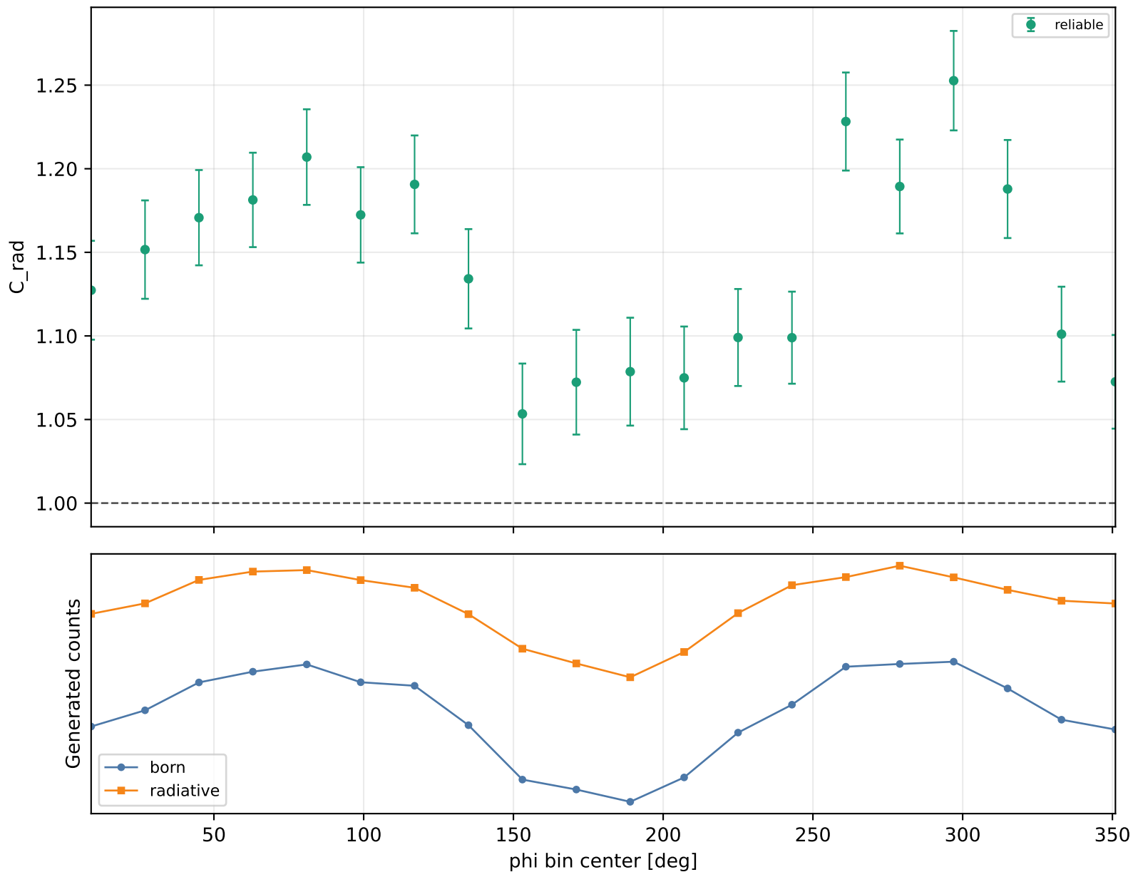
Radiative correction vs phi Q2 2.5-3, xB 0.3-0.38, -t 0.3-0.4
