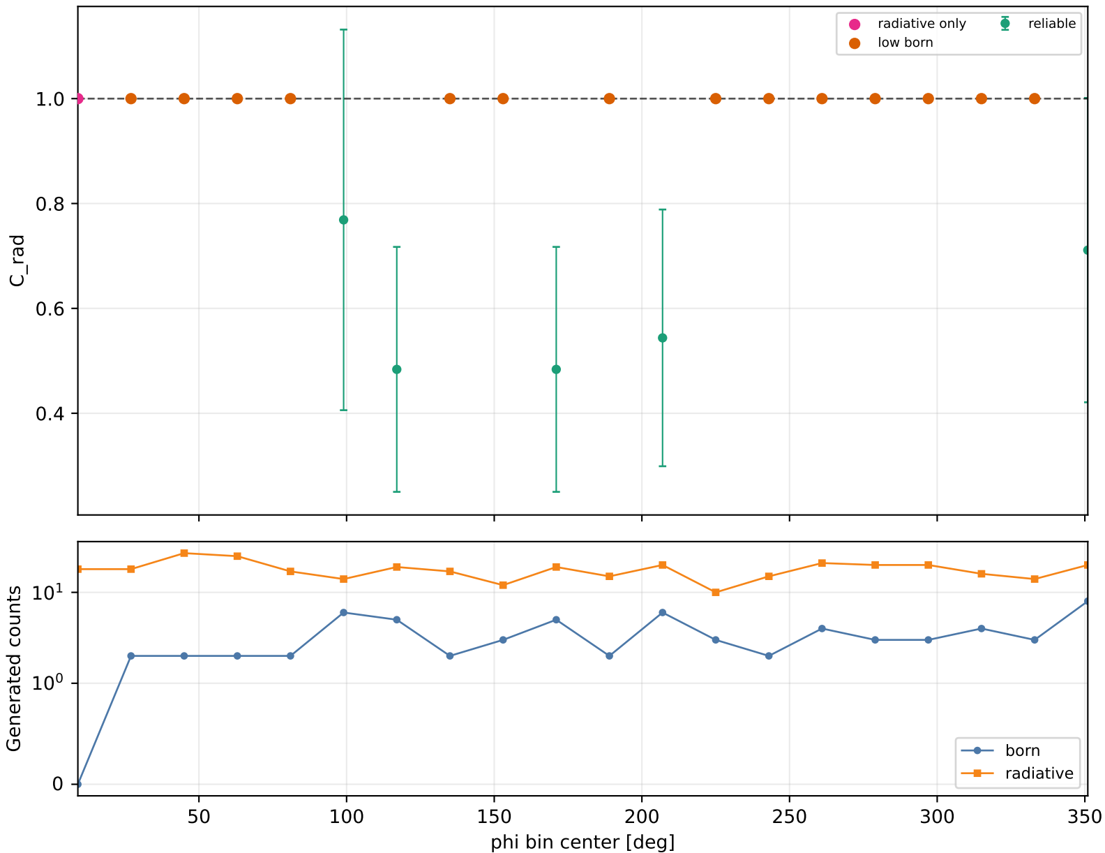
Radiative correction vs phi Q2 2.5-3, xB 0.2-0.25, -t 1.5-2
