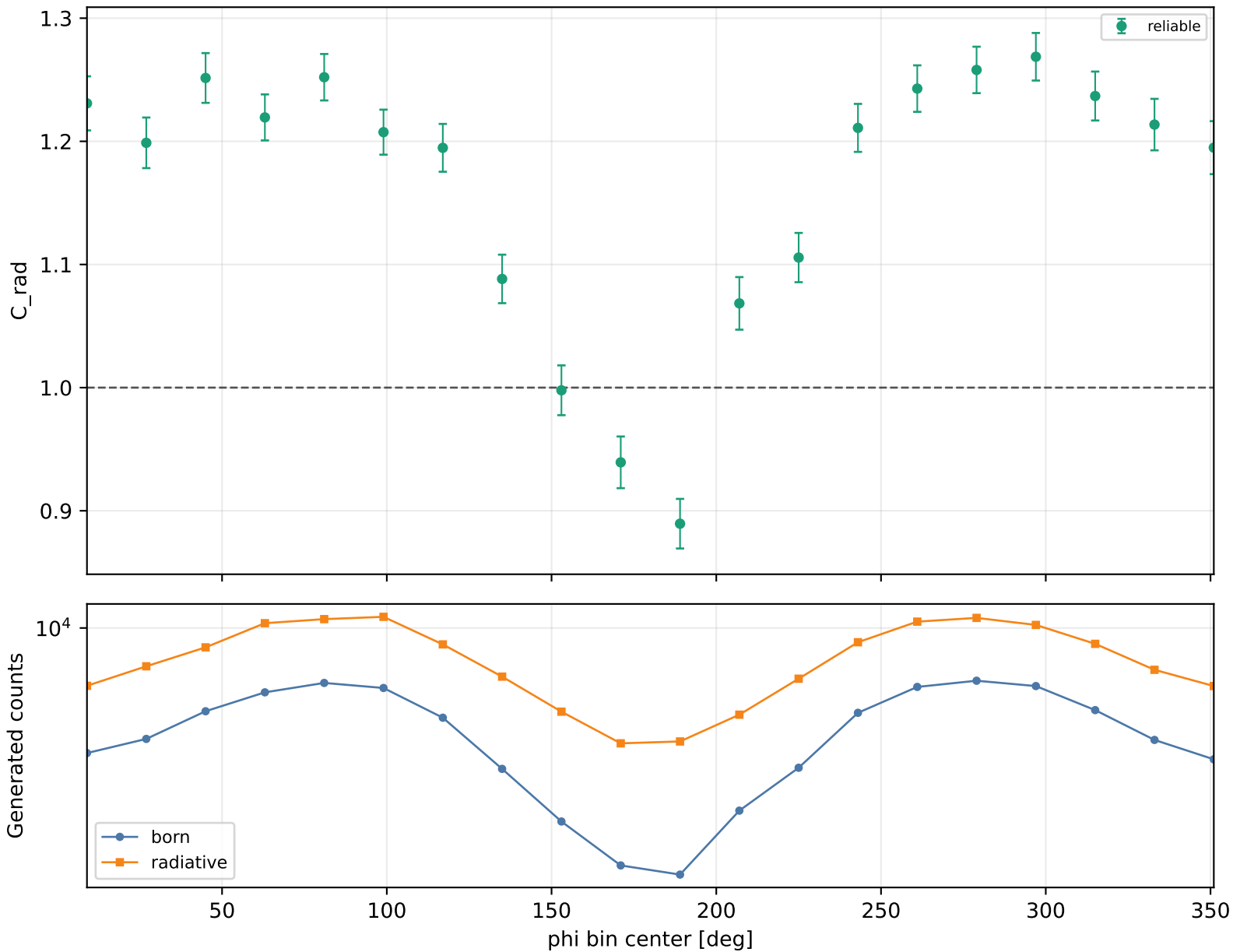
Radiative correction vs phi Q2 2-2.5, xB 0.3-0.38, -t 0.3-0.4
