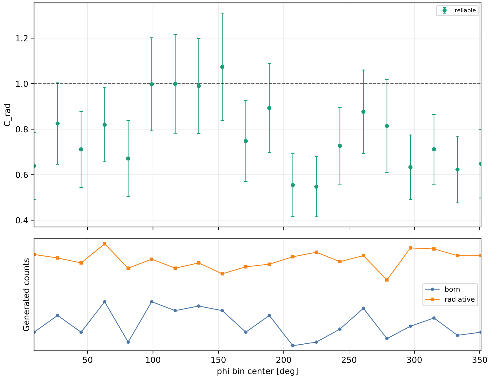
Radiative correction vs phi Q2 4.6-5.5, xB 0.38-0.48, -t 0.3-0.4
