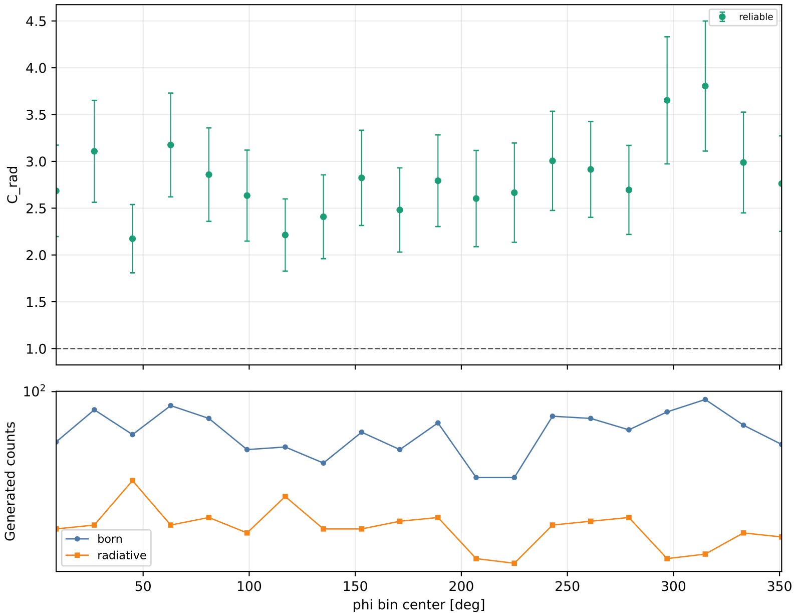
Radiative correction vs phi Q2 2-2.5, xB 0.38-0.48, -t 0.15-0.2
