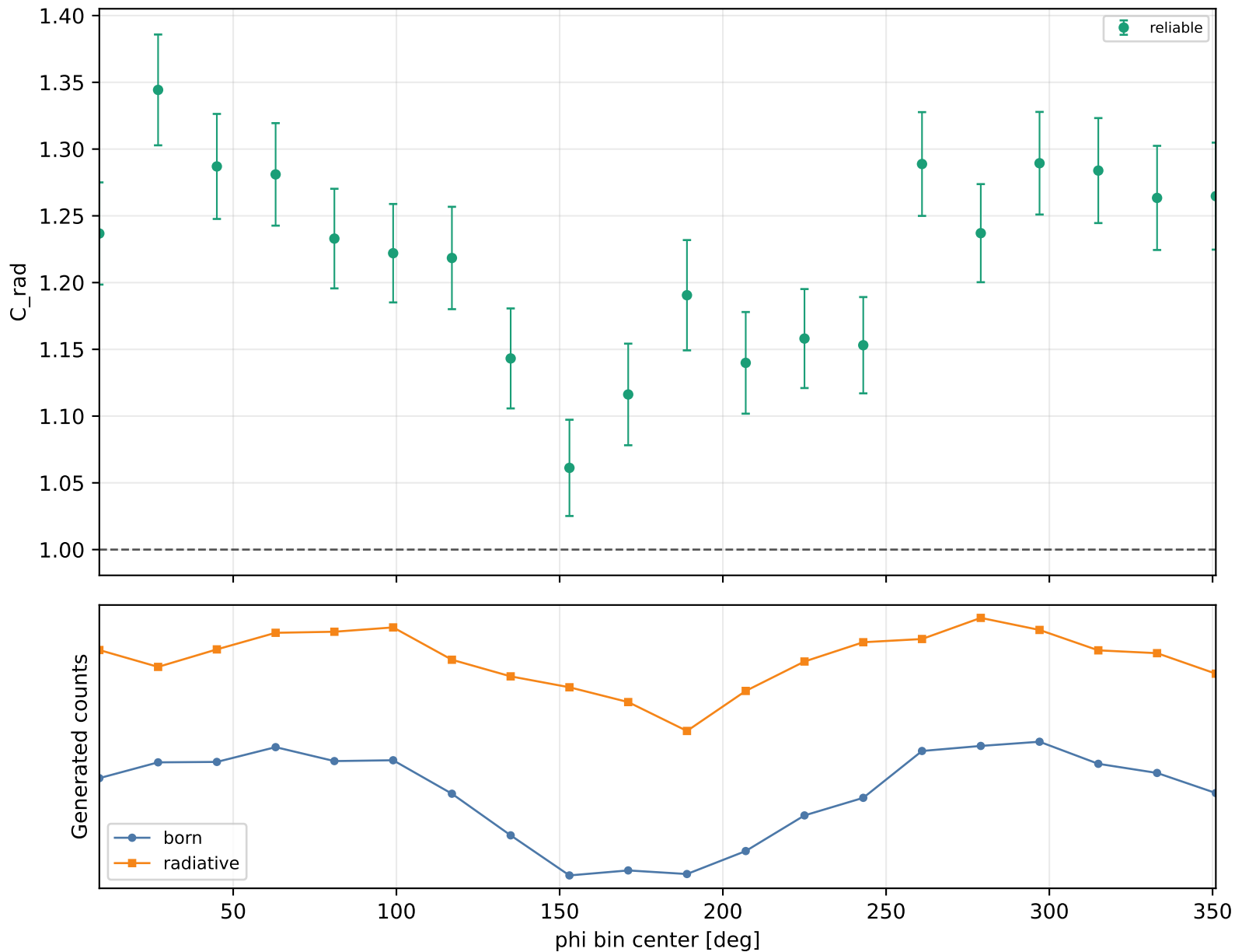
Radiative correction vs phi Q2 3-3.5, xB 0.38-0.48, -t 0.3-0.4
