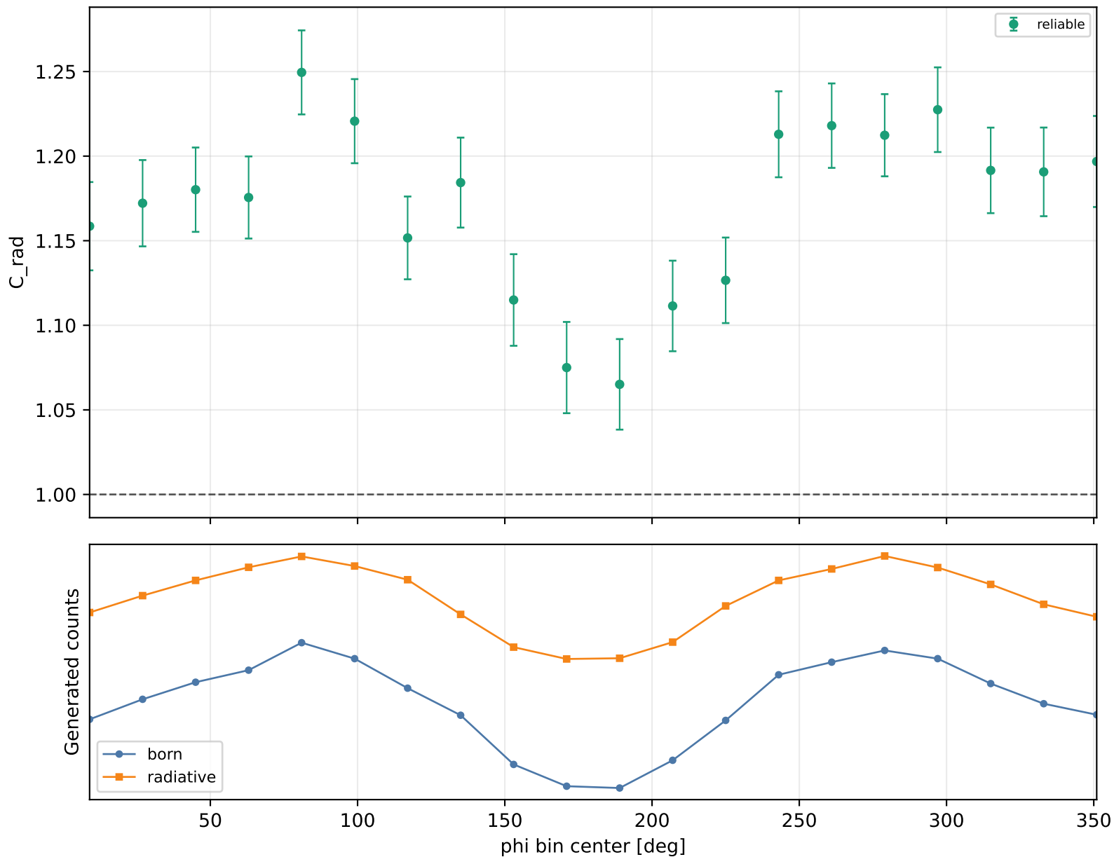
Radiative correction vs phi Q2 3-3.5, xB 0.38-0.48, -t 0.4-0.6
