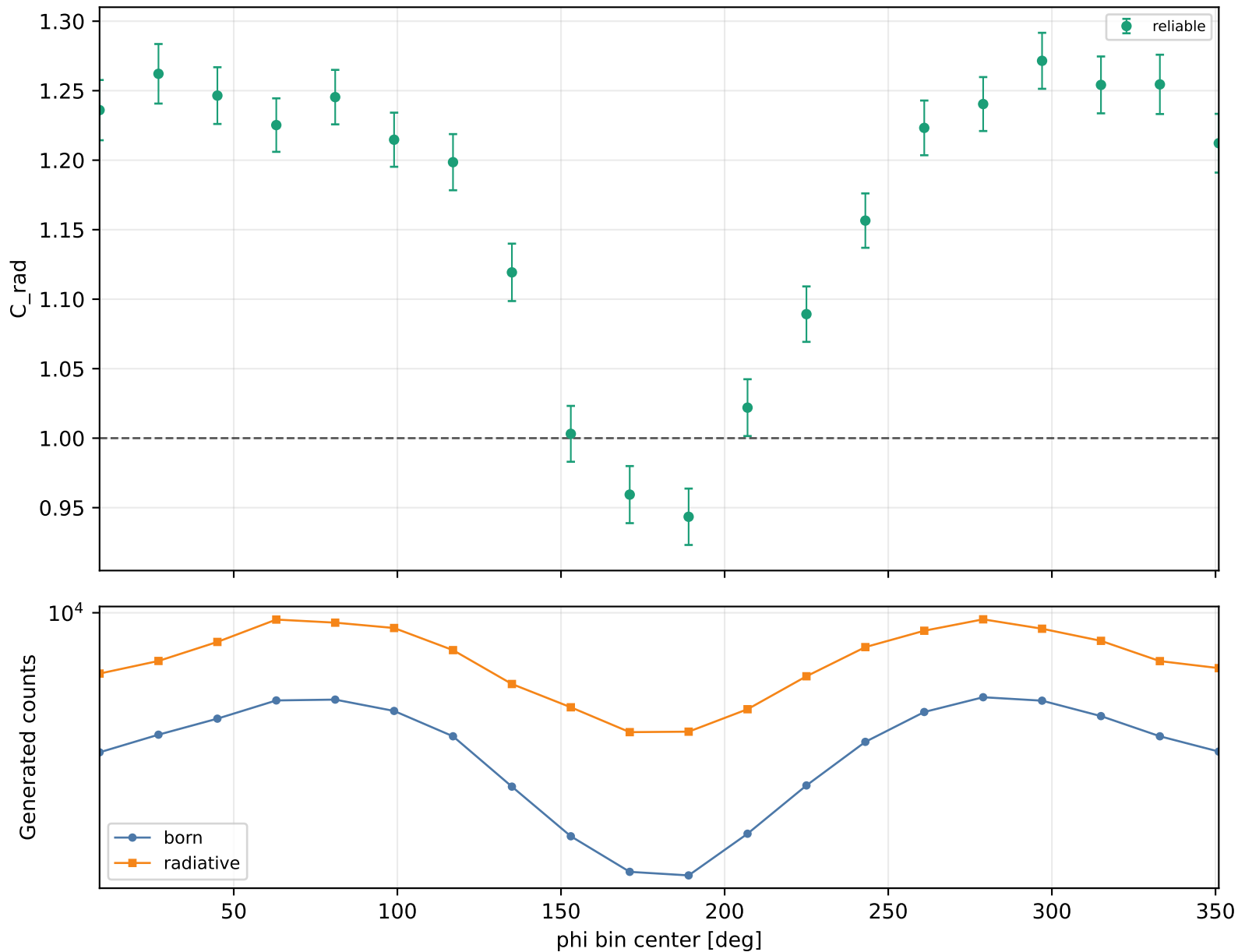
Radiative correction vs phi Q2 2-2.5, xB 0.3-0.38, -t 0.2-0.3
