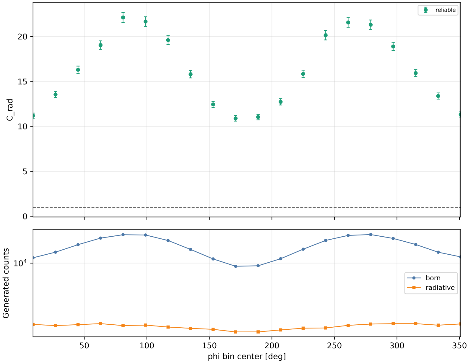
Radiative correction vs phi Q2 3-3.5, xB 0.58-0.7, -t 0.6-1
