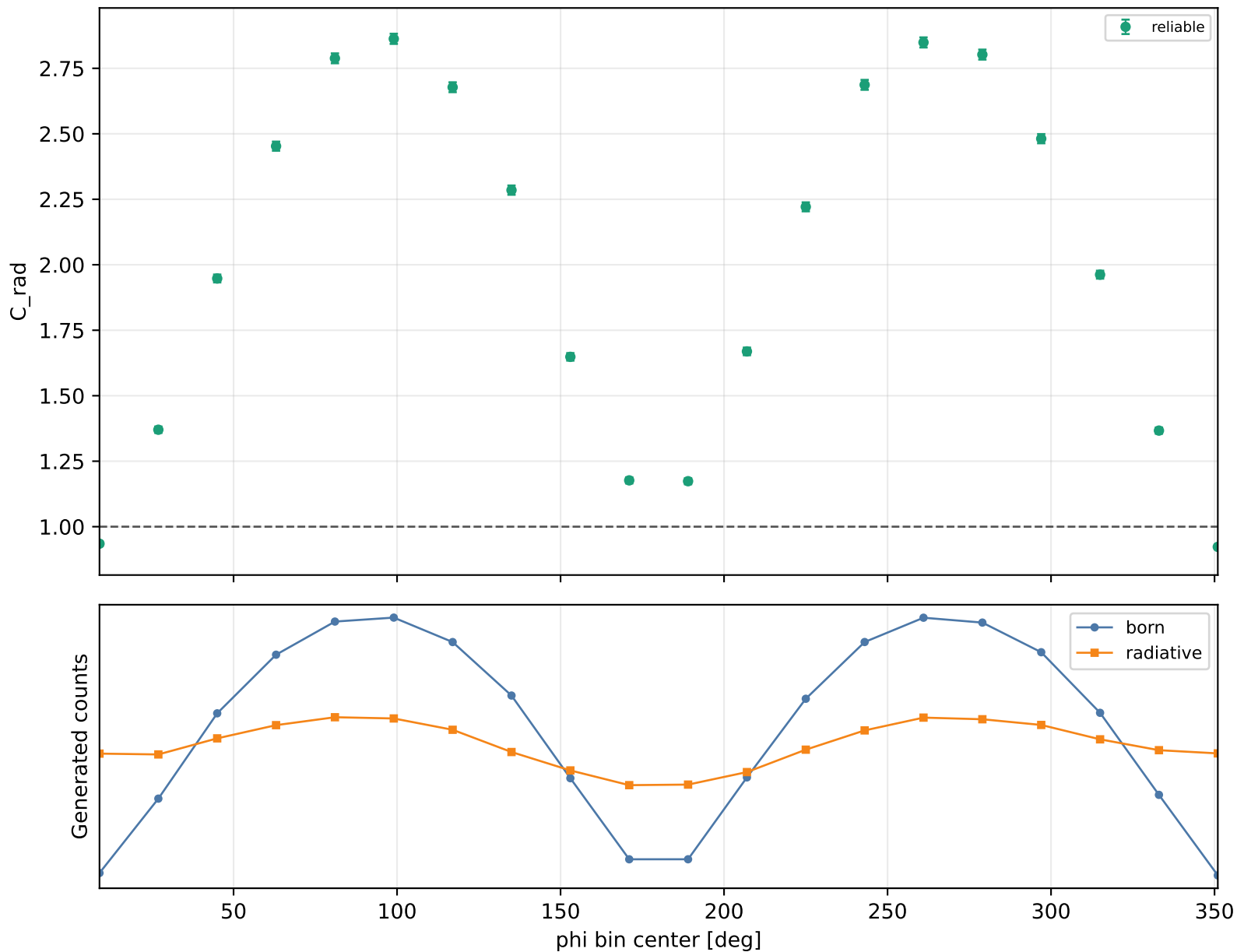
Radiative correction vs phi Q2 2-2.5, xB 0.48-0.58, -t 1-1.5
