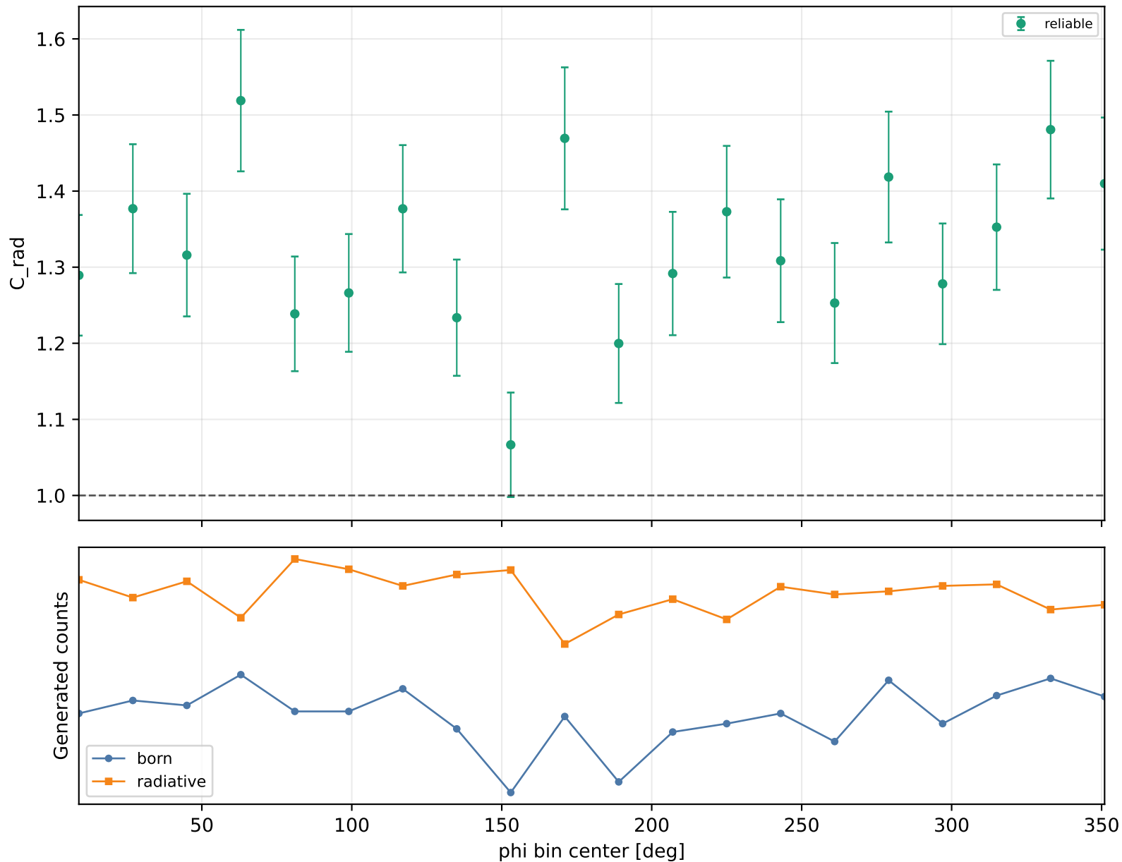
Radiative correction vs phi Q2 3.5-4, xB 0.38-0.48, -t 0.2-0.3
