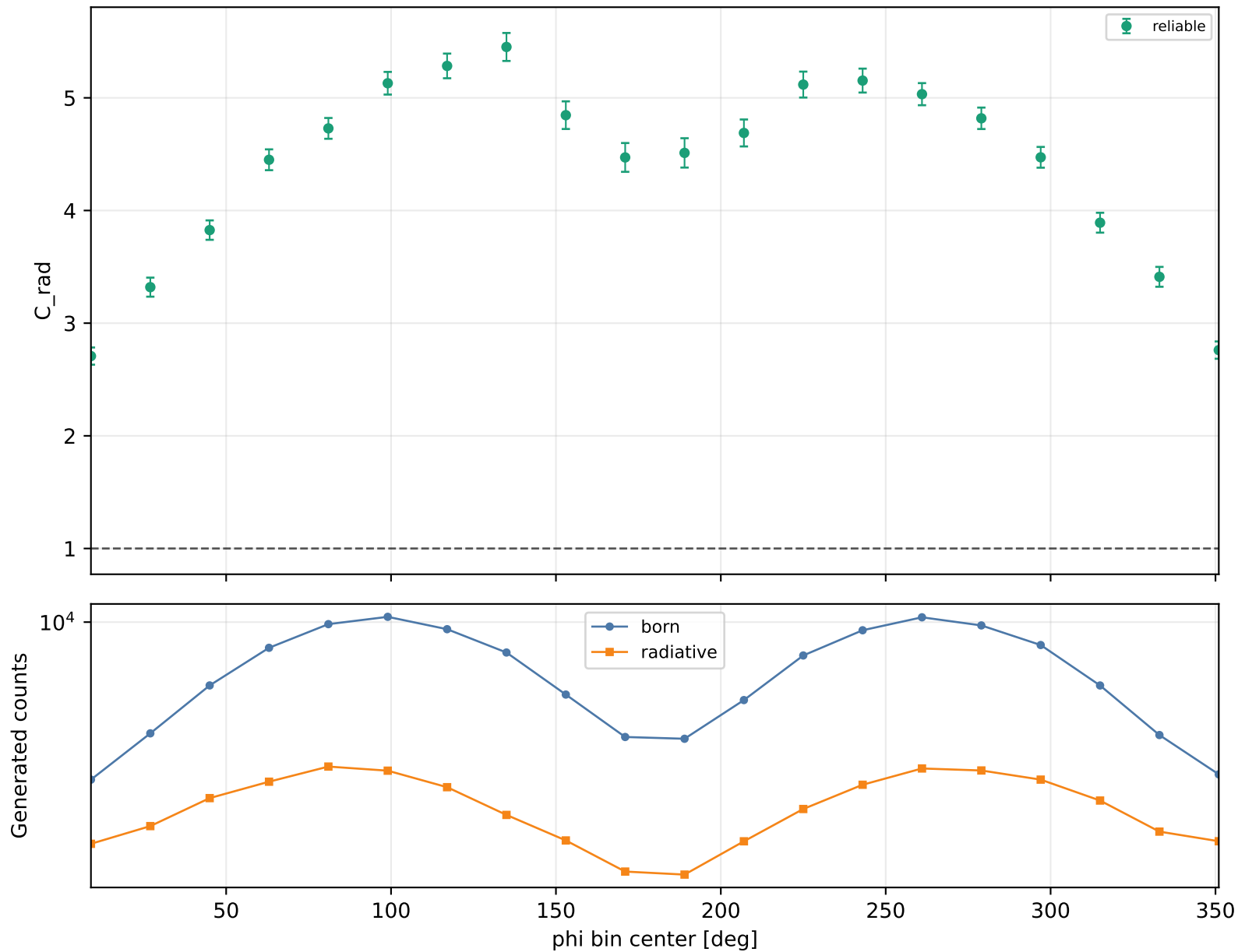
Radiative correction vs phi Q2 4-4.6, xB 0.58-0.7, -t 1.5-2
