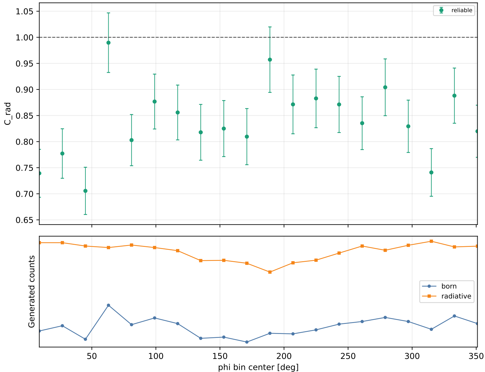
Radiative correction vs phi Q2 3.5-4, xB 0.3-0.38, -t 0.6-1
