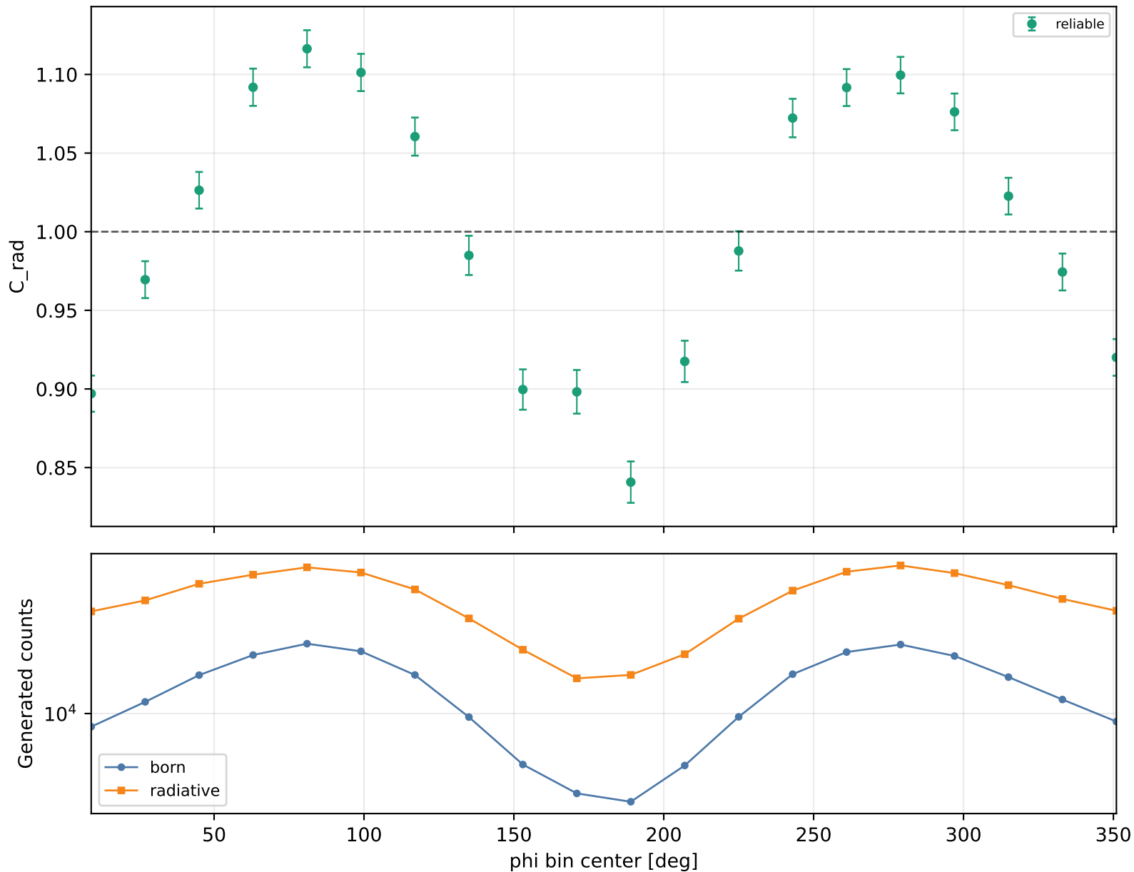
Radiative correction vs phi Q2 1-1.5, xB 0.1-0.15, -t 0.2-0.3
