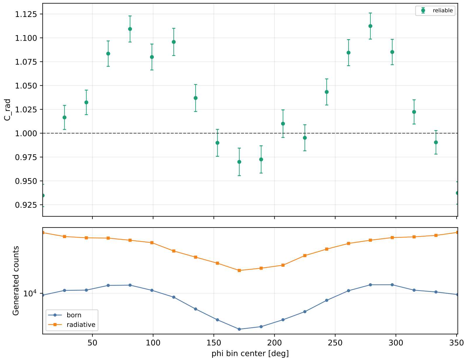
Radiative correction vs phi Q2 1-1.5, xB 0.1-0.15, -t 0.6-1
