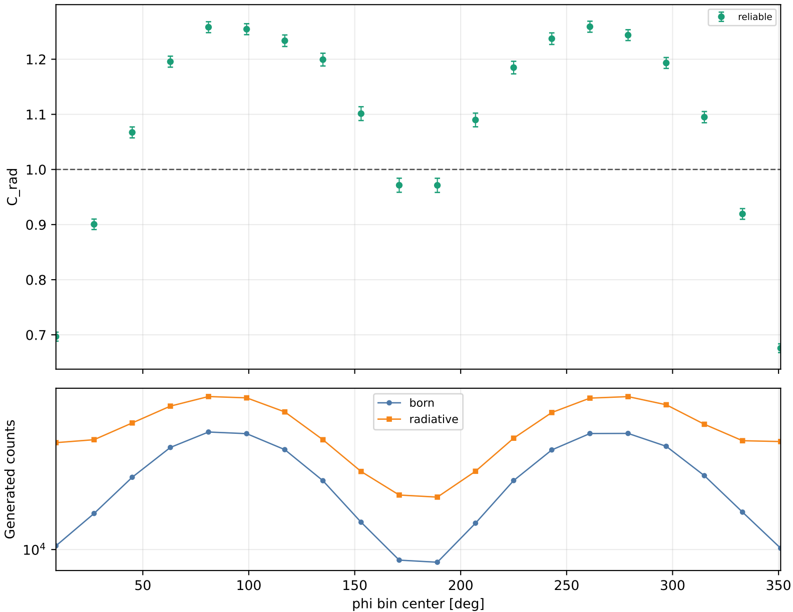
Radiative correction vs phi Q2 2-2.5, xB 0.38-0.48, -t 1-1.5
