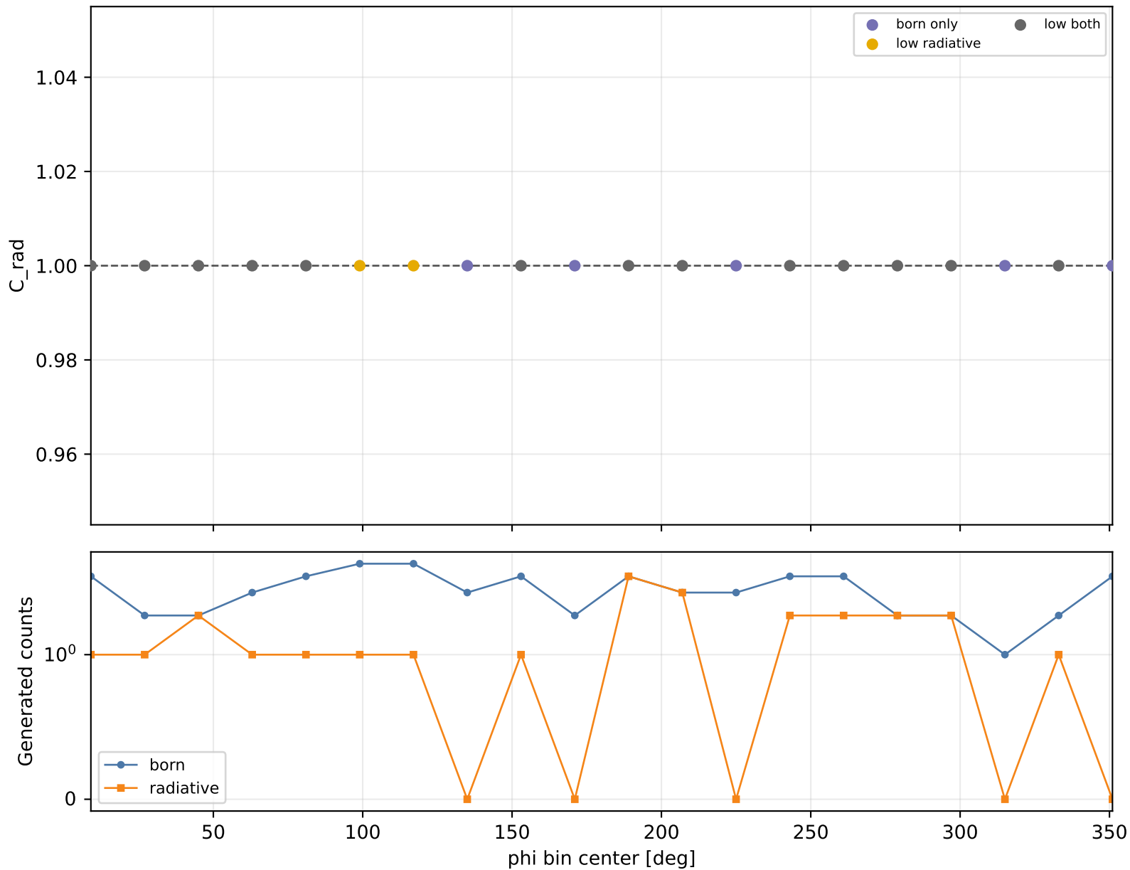
Radiative correction vs phi Q2 4-4.6, xB 0.58-0.7, -t 0.4-0.6
