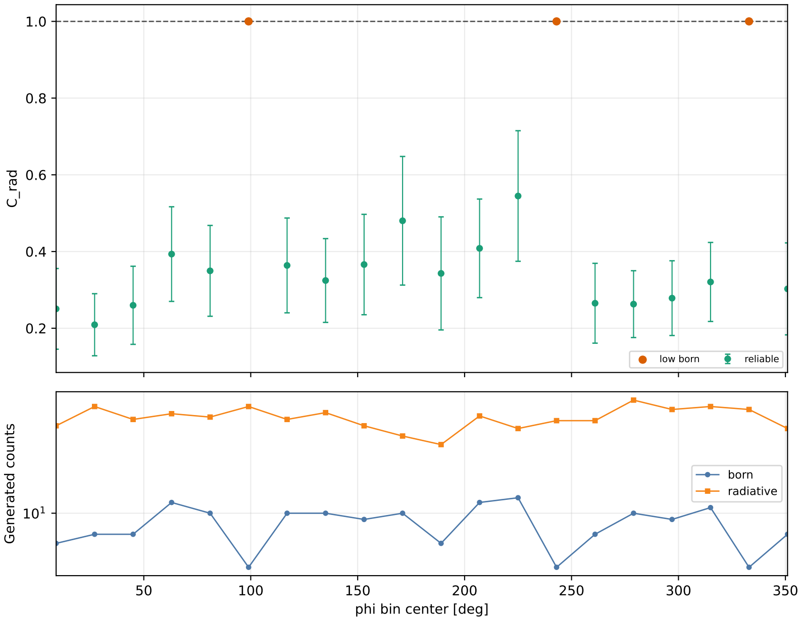
Radiative correction vs phi Q2 1.5-2, xB 0.1-0.15, -t 0.09-0.15
