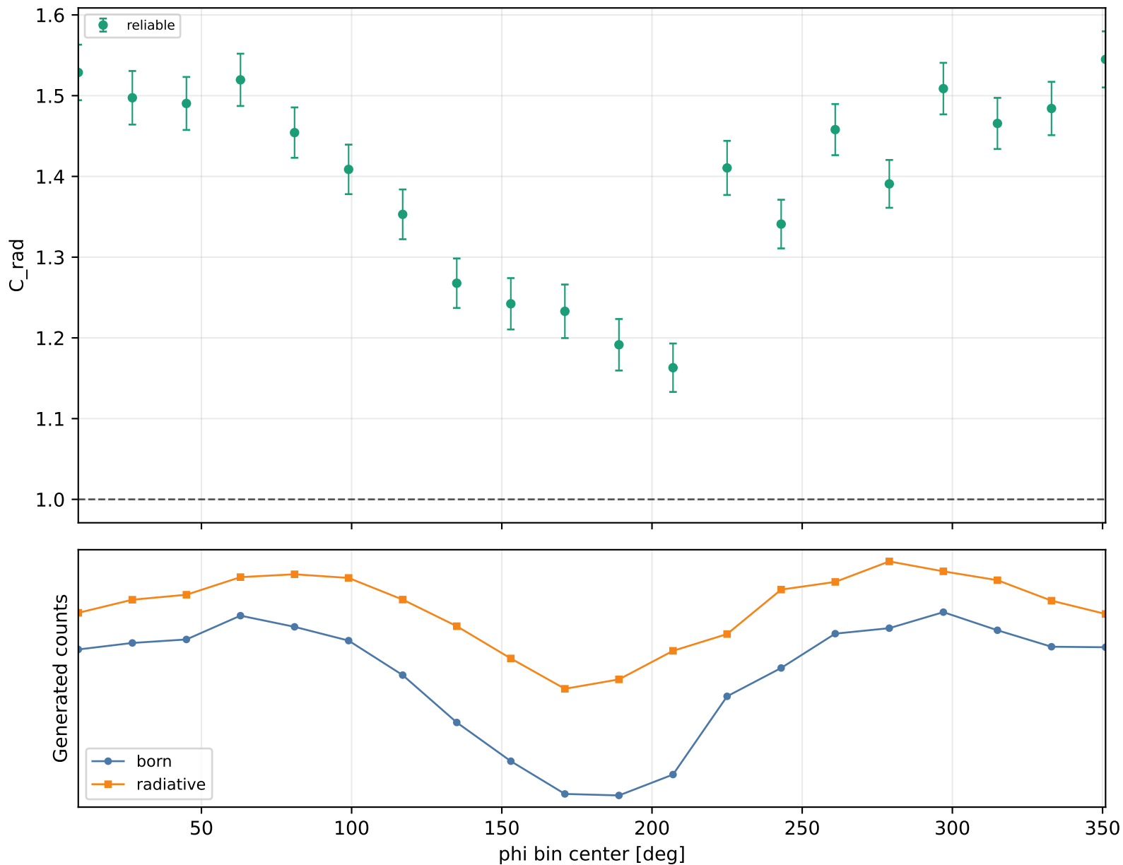
Radiative correction vs phi Q2 2-2.5, xB 0.38-0.48, -t 0.2-0.3
