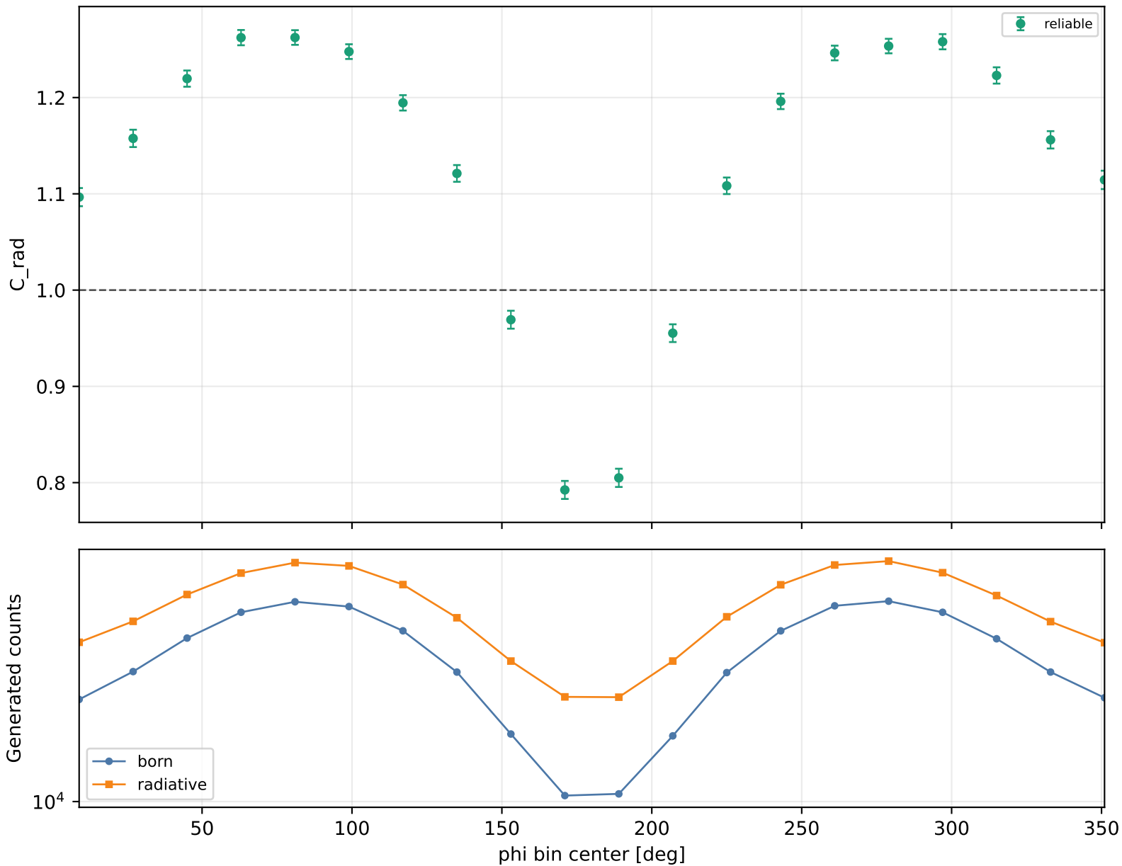
Radiative correction vs phi Q2 1.5-2, xB 0.3-0.38, -t 0.4-0.6
