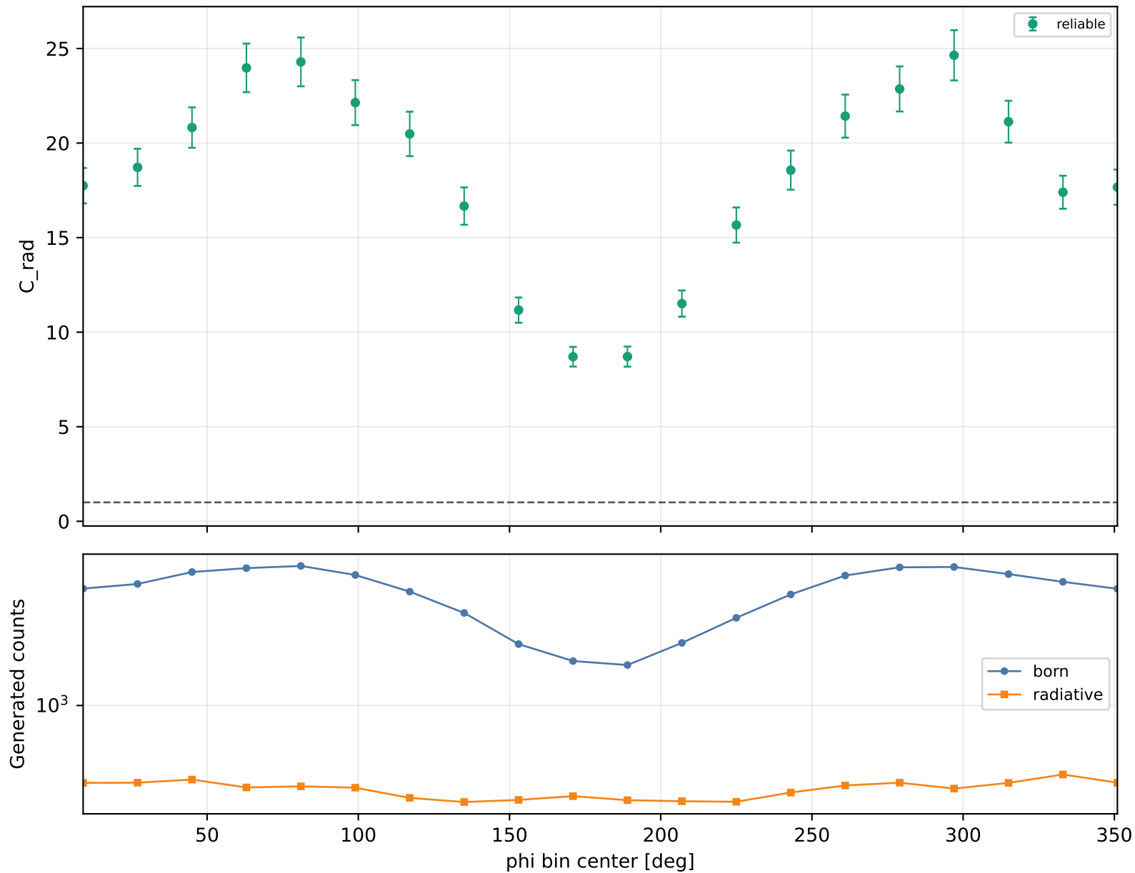
Radiative correction vs phi Q2 1.5-2, xB 0.48-0.58, -t 0.3-0.4
