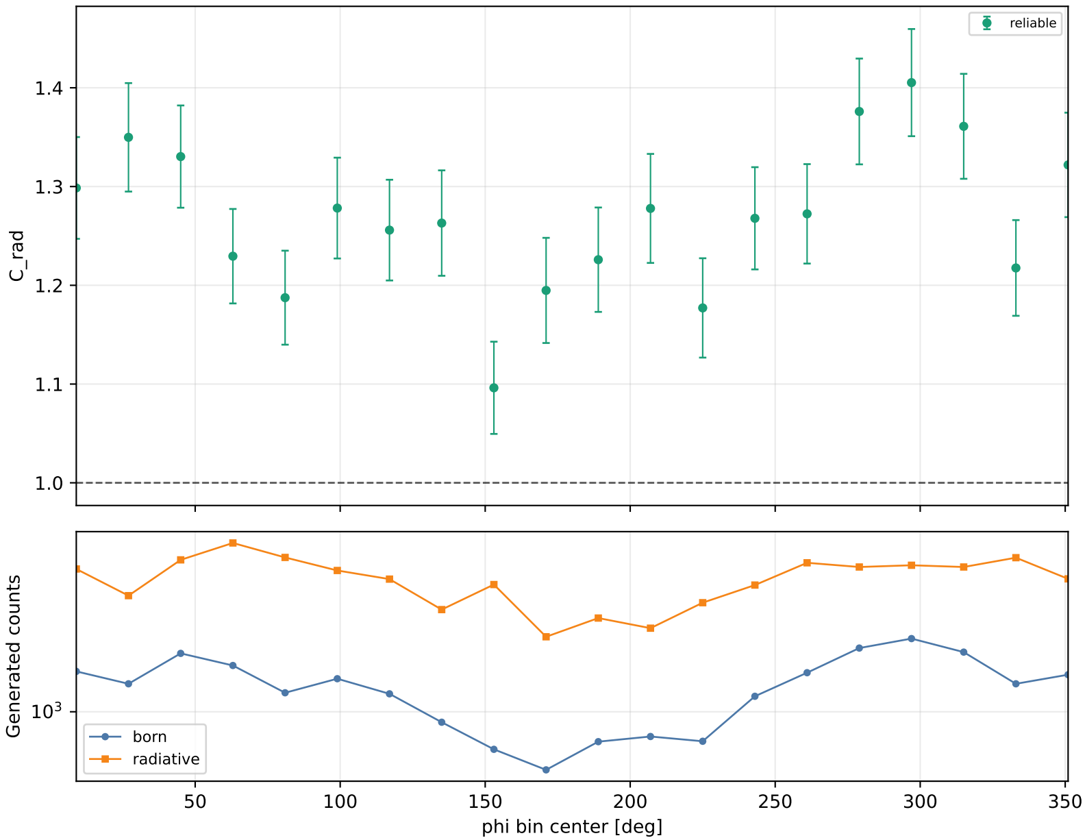
Radiative correction vs phi Q2 2.5-3, xB 0.3-0.38, -t 0.15-0.2
