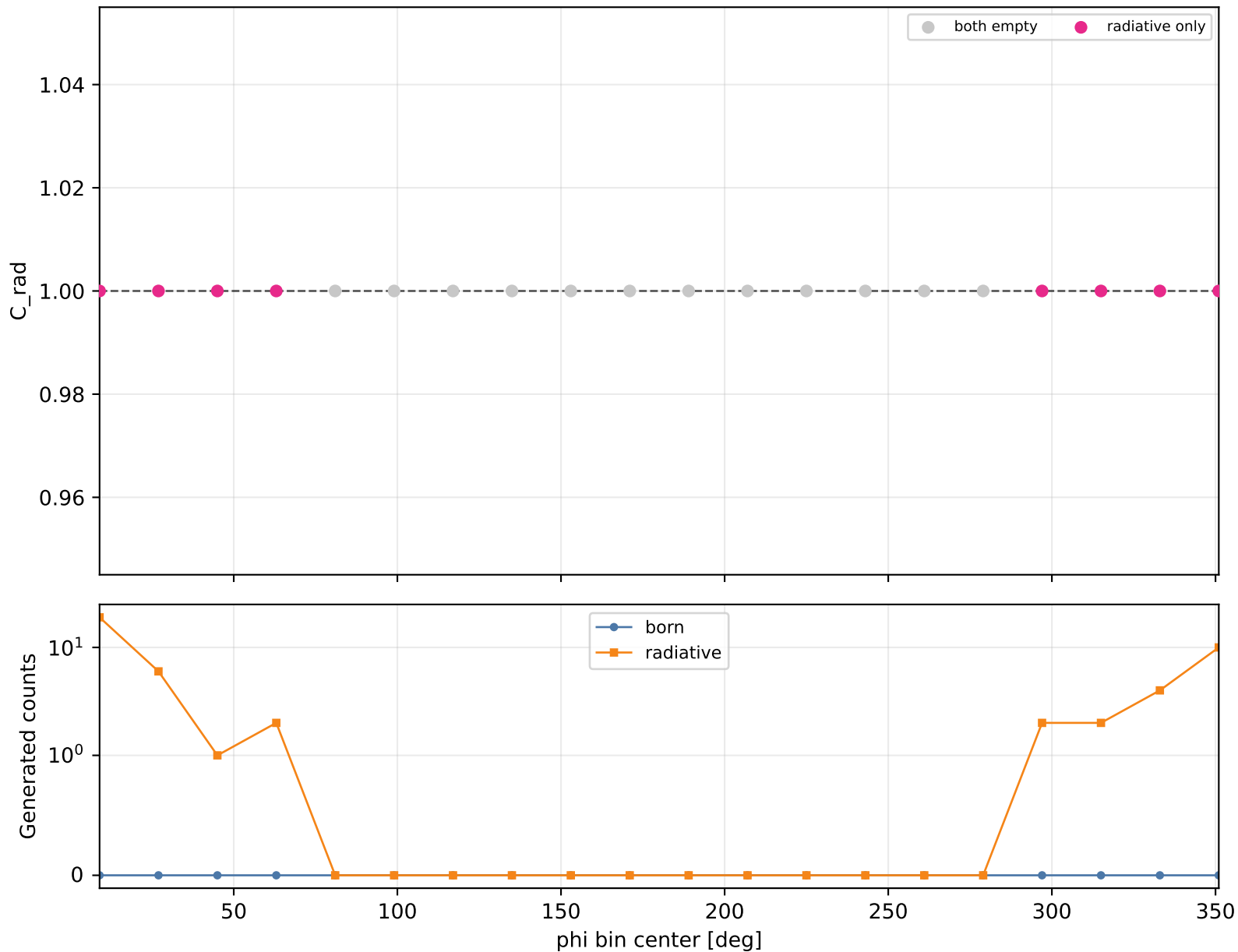
Radiative correction vs phi Q2 5.5-6.535, xB 0.58-0.7, -t 1.5-2
