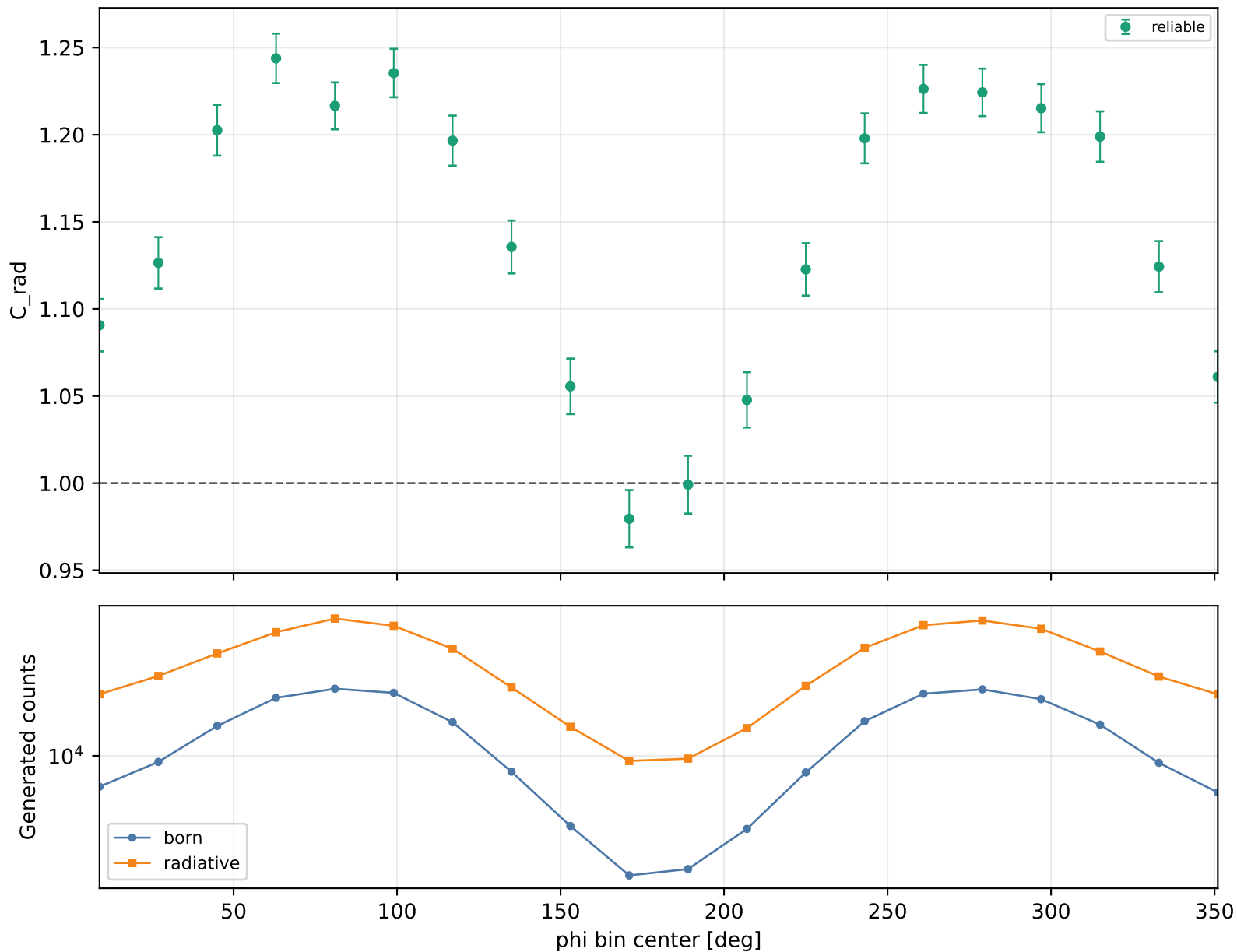
Radiative correction vs phi Q2 2-2.5, xB 0.3-0.38, -t 0.4-0.6
