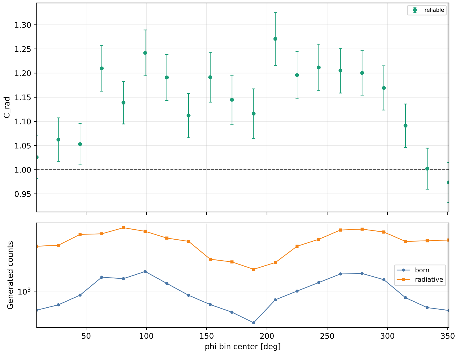
Radiative correction vs phi Q2 4.6-5.5, xB 0.48-0.58, -t 1-1.5
