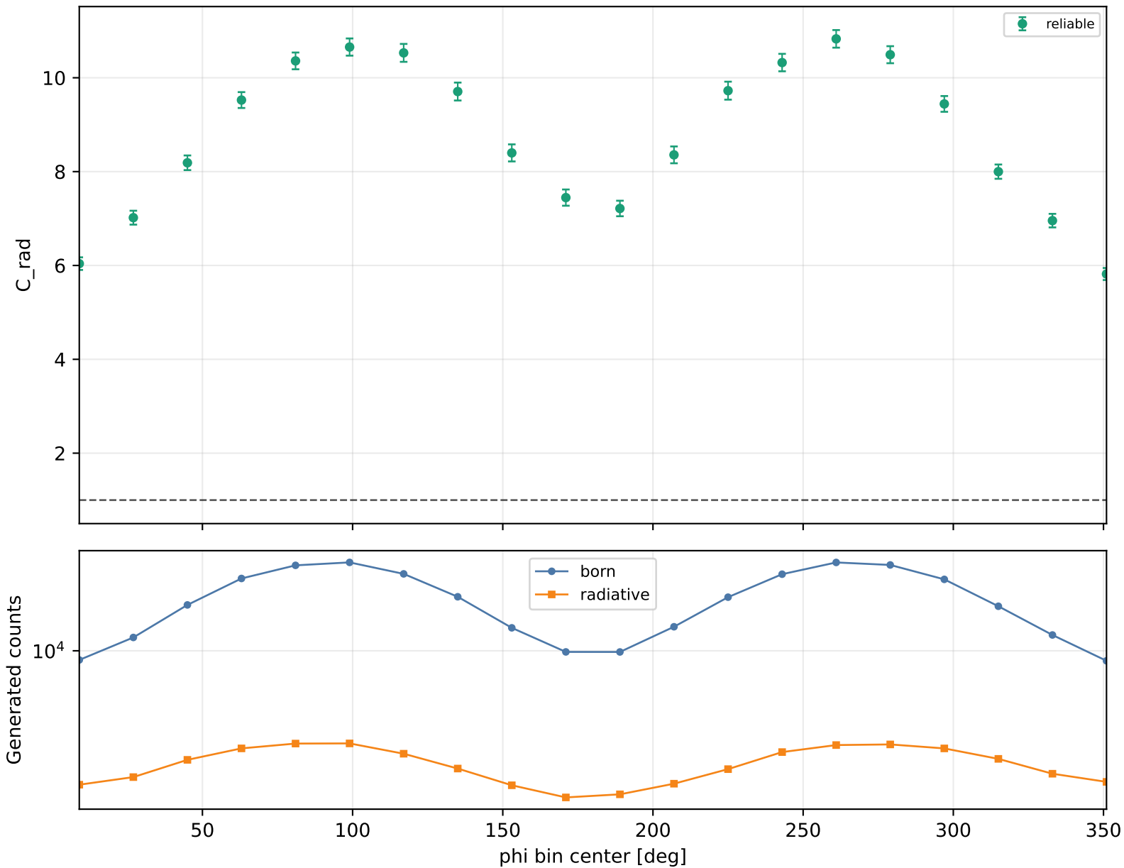
Radiative correction vs phi Q2 3.5-4, xB 0.58-0.7, -t 1-1.5
