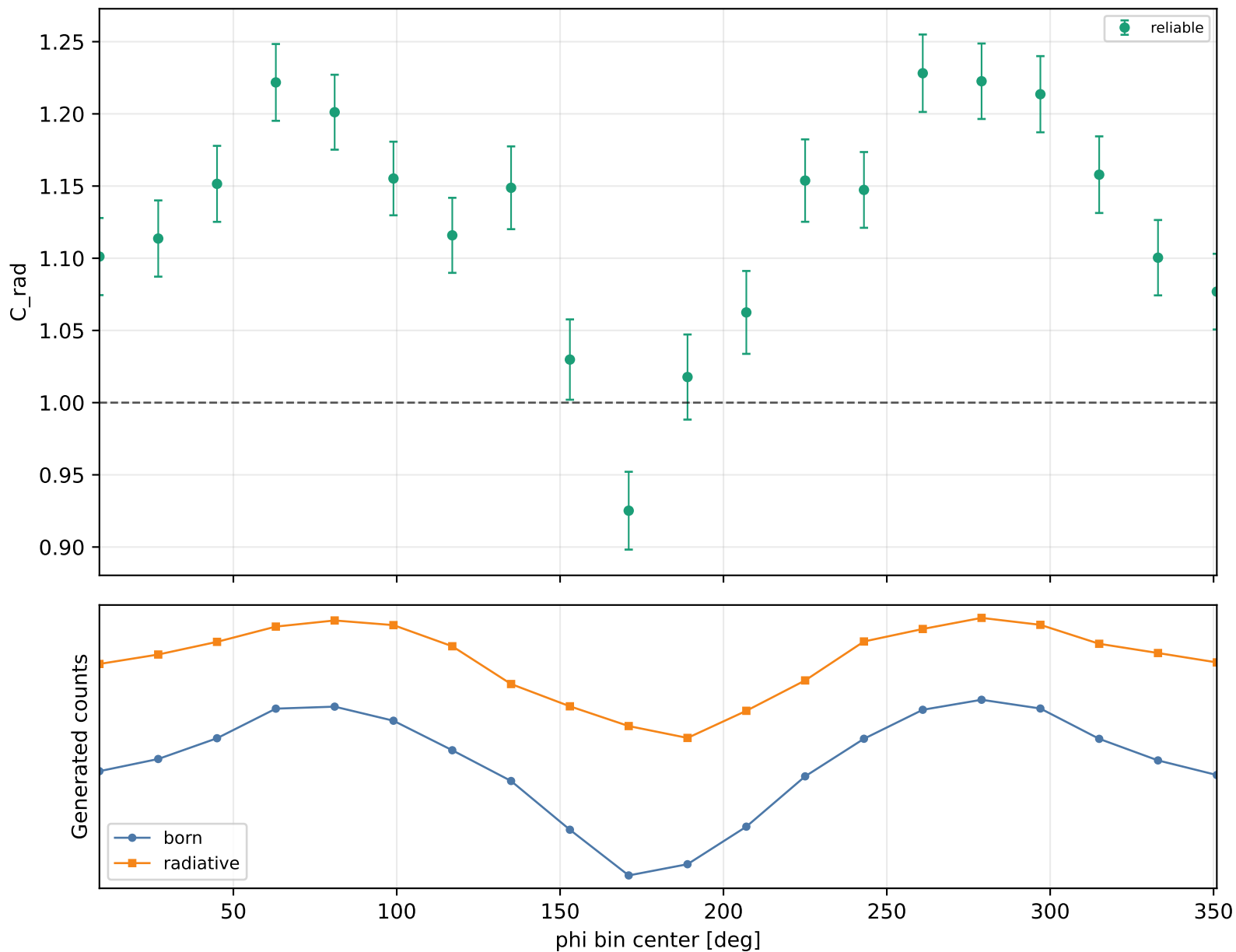
Radiative correction vs phi Q2 2-2.5, xB 0.25-0.3, -t 0.3-0.4
