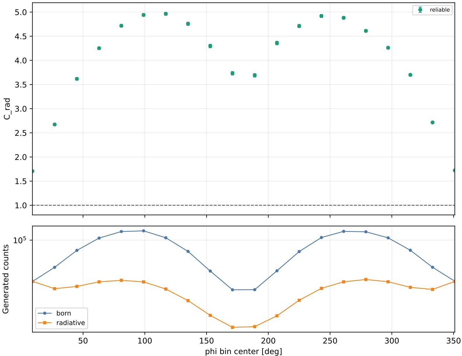
Radiative correction vs phi Q2 1-1.5, xB 0.3-0.38, -t 1-1.5
