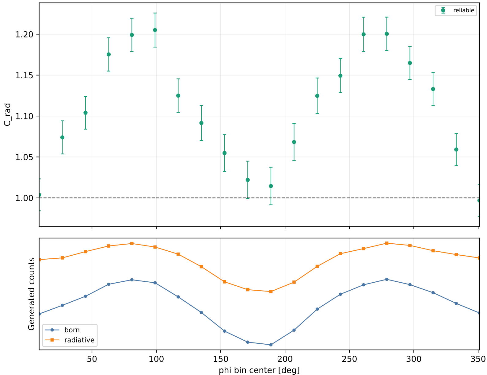
Radiative correction vs phi Q2 2-2.5, xB 0.25-0.3, -t 0.4-0.6
