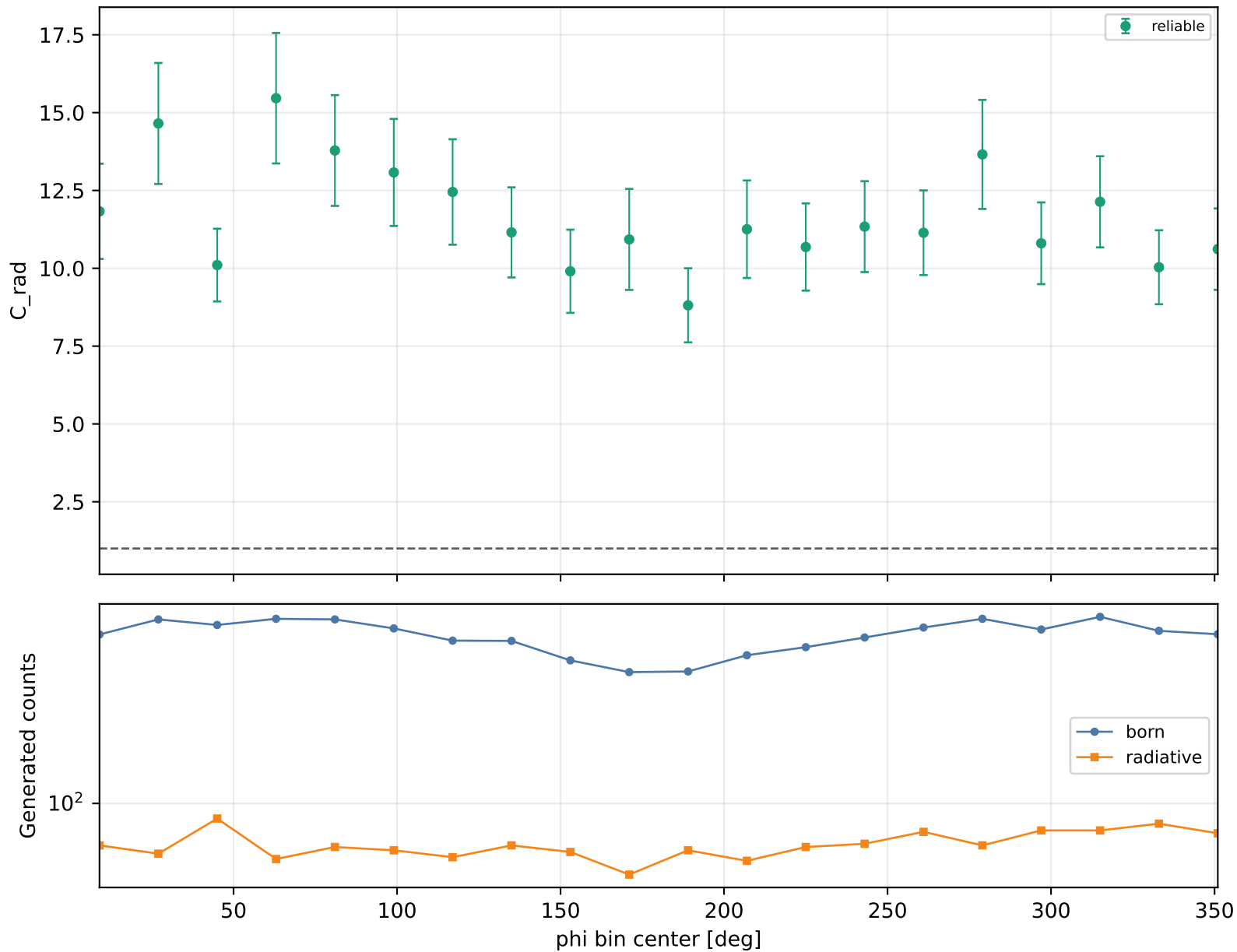
Radiative correction vs phi Q2 2.5-3, xB 0.58-0.7, -t 0.4-0.6
