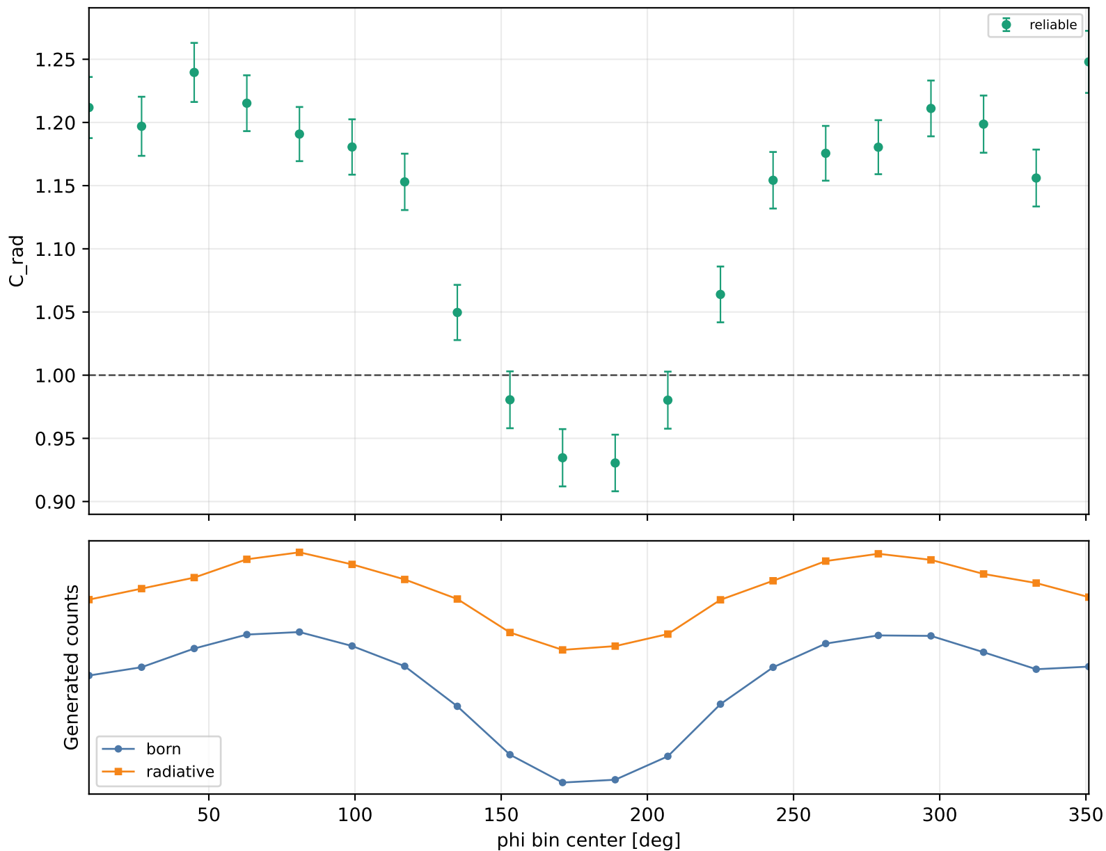
Radiative correction vs phi Q2 1.5-2, xB 0.2-0.25, -t 0.09-0.15
