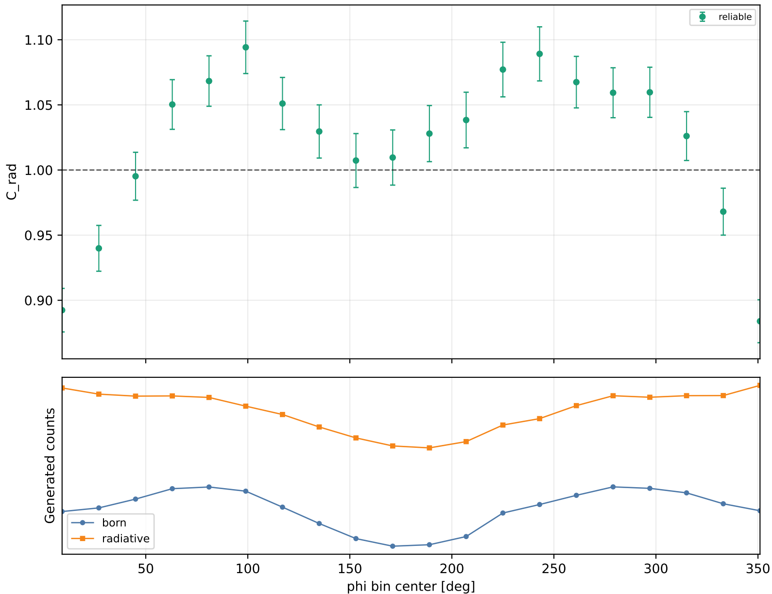
Radiative correction vs phi Q2 1.5-2, xB 0.15-0.2, -t 0.6-1
