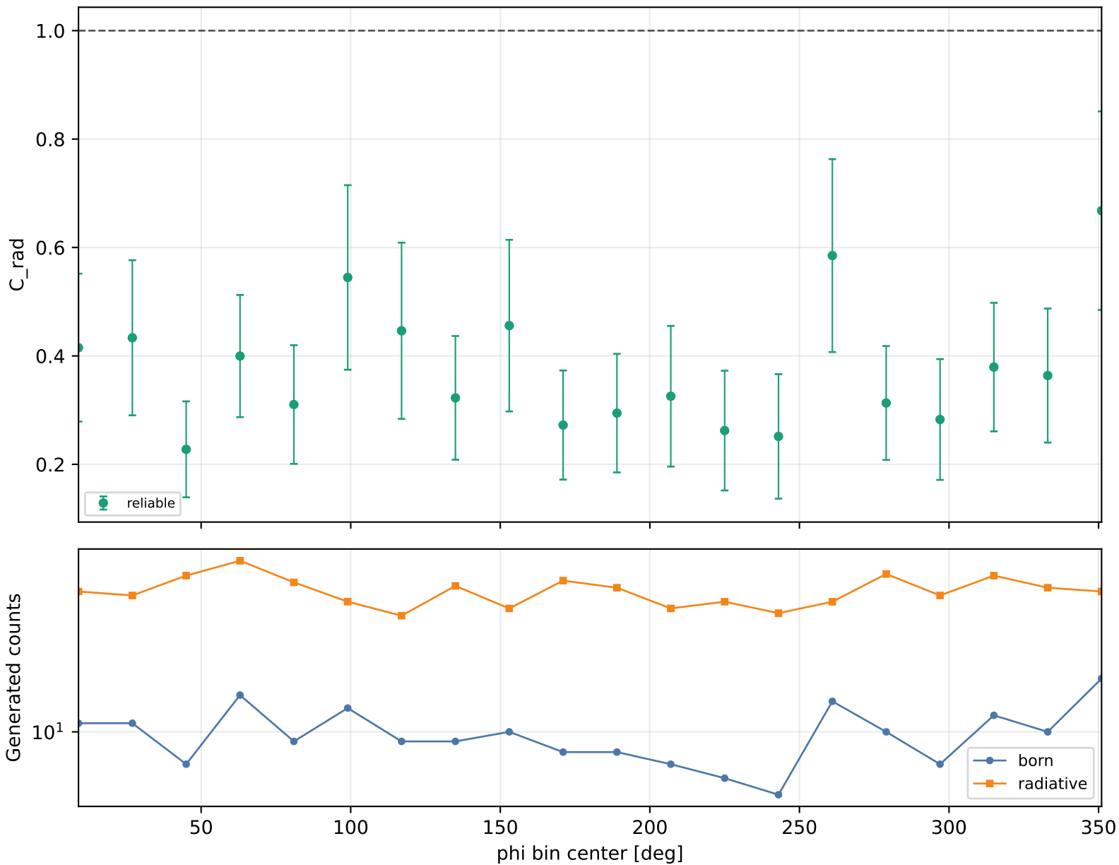
Radiative correction vs phi Q2 2-2.5, xB 0.15-0.2, -t 0.3-0.4
