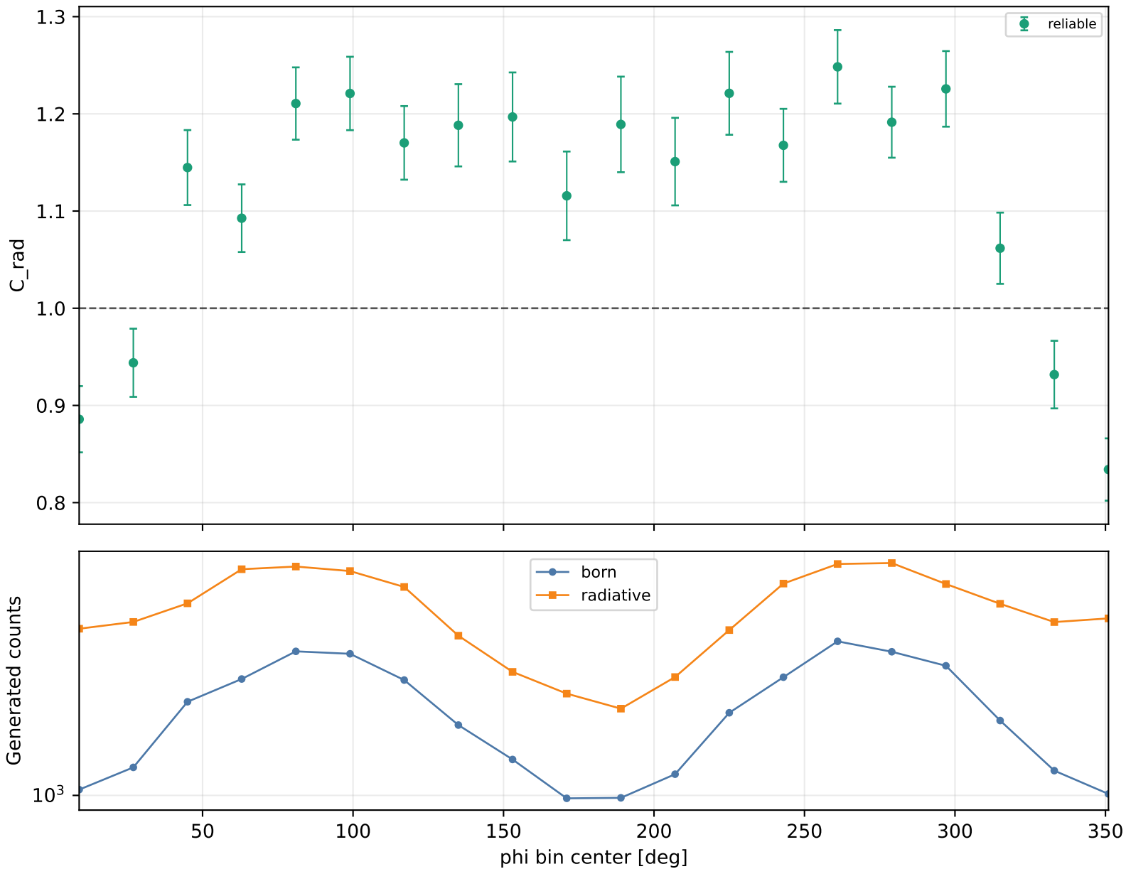
Radiative correction vs phi Q2 4-4.6, xB 0.48-0.58, -t 1.5-2
