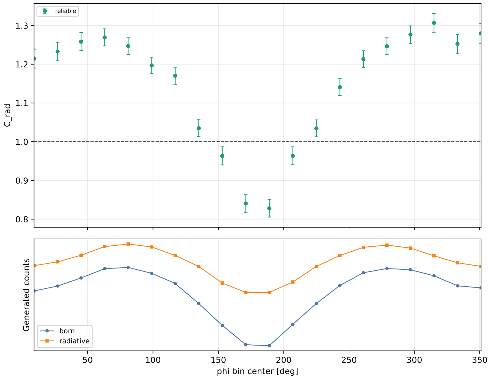
Radiative correction vs phi Q2 1.5-2, xB 0.25-0.3, -t 0.15-0.2
