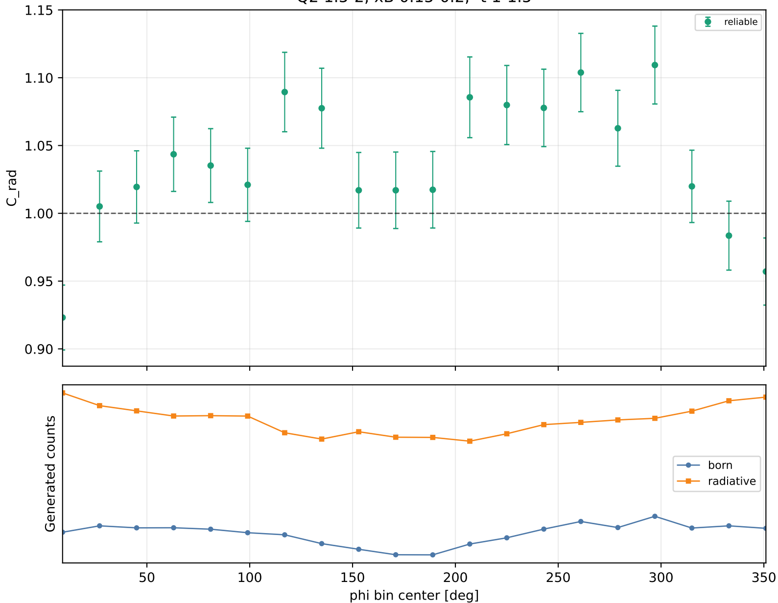
Radiative correction vs phi Q2 1.5-2, xB 0.15-0.2, -t 1-1.5
