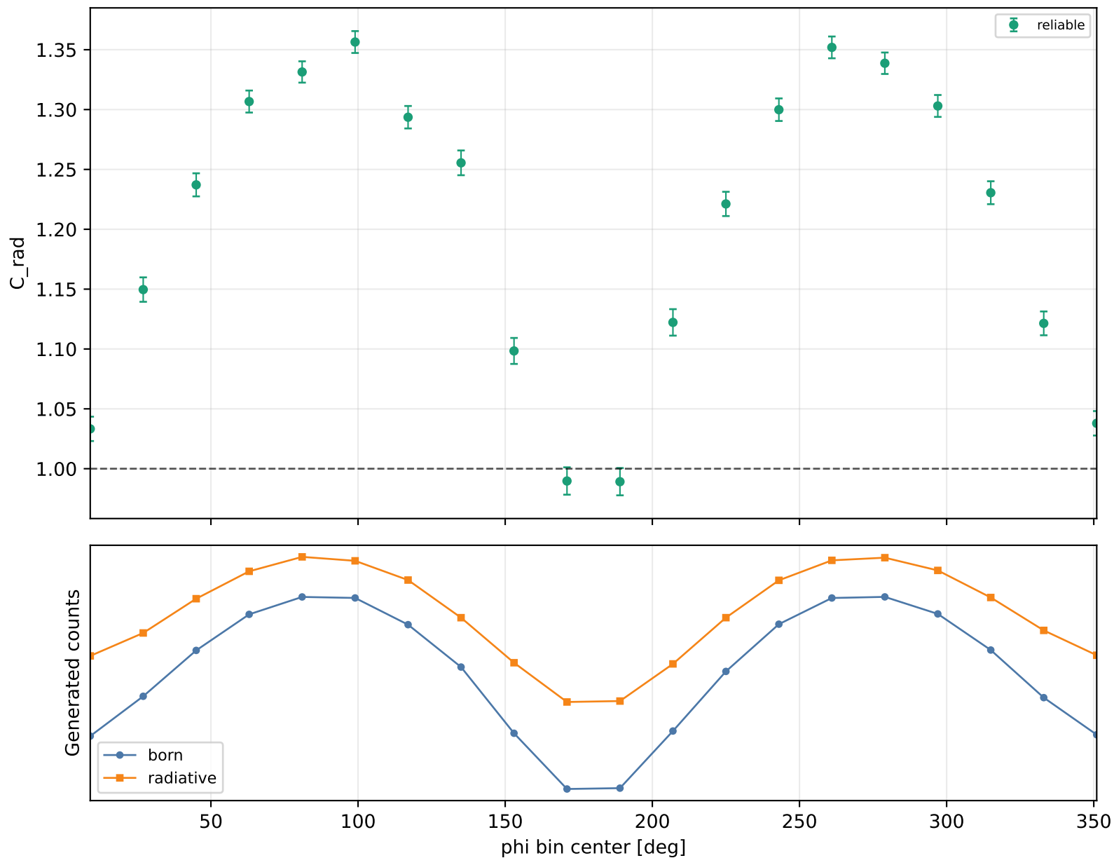
Radiative correction vs phi Q2 2-2.5, xB 0.38-0.48, -t 0.6-1
