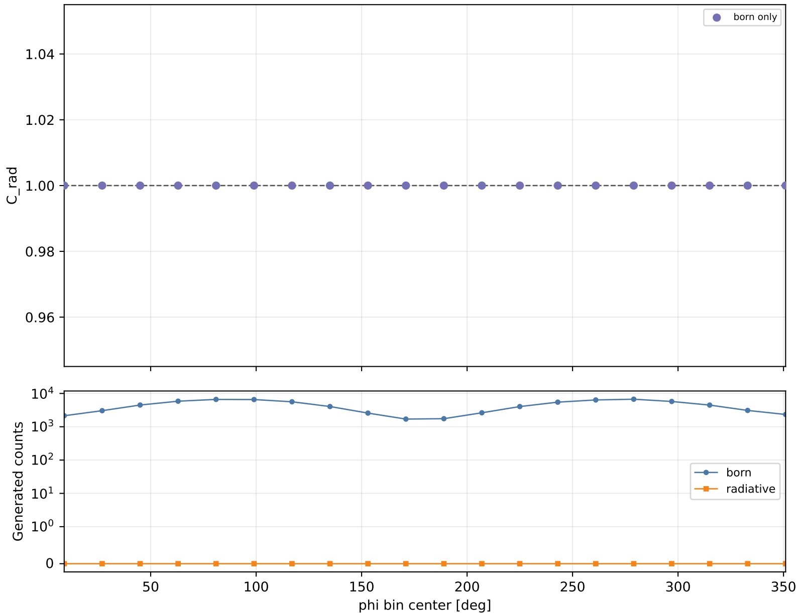
Radiative correction vs phi Q2 1-1.5, xB 0.48-0.58, -t 1-1.5
