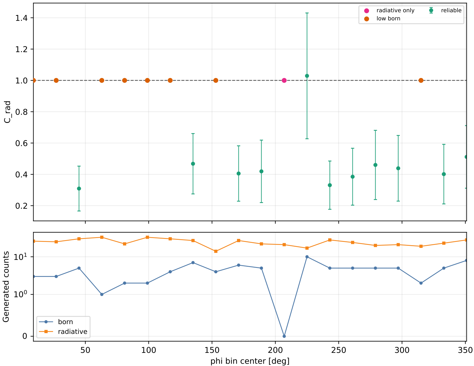
Radiative correction vs phi Q2 2.5-3, xB 0.2-0.25, -t 0.15-0.2
