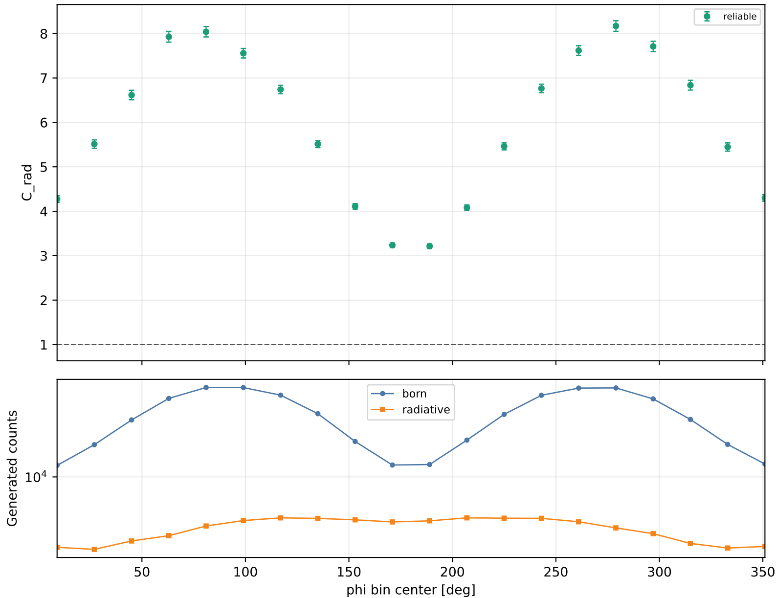
Radiative correction vs phi Q2 1.5-2, xB 0.48-0.58, -t 1.5-2
