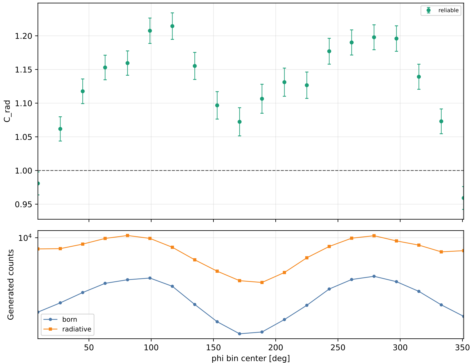
Radiative correction vs phi Q2 2.5-3, xB 0.3-0.38, -t 0.6-1
