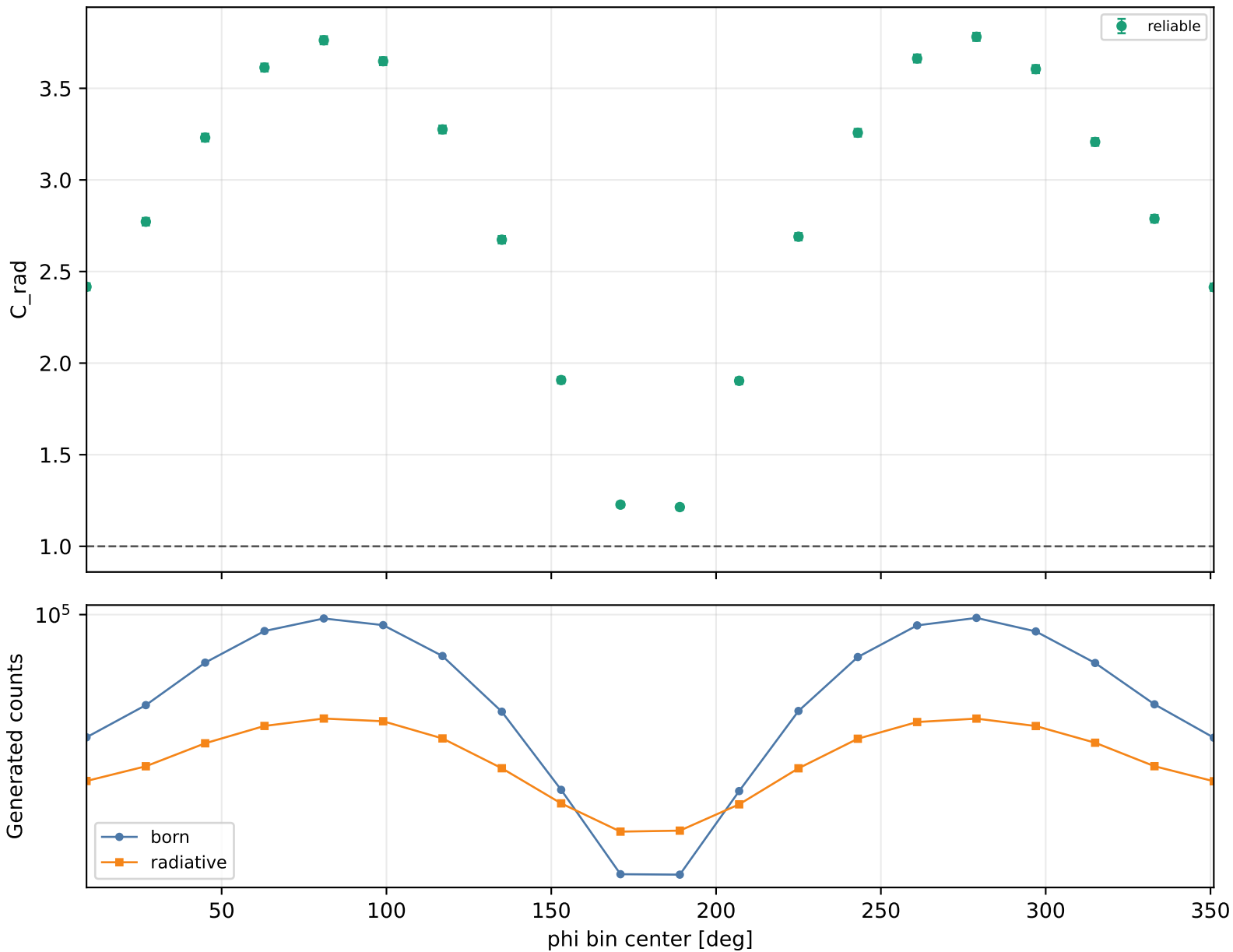
Radiative correction vs phi Q2 1.5-2, xB 0.38-0.48, -t 0.4-0.6
