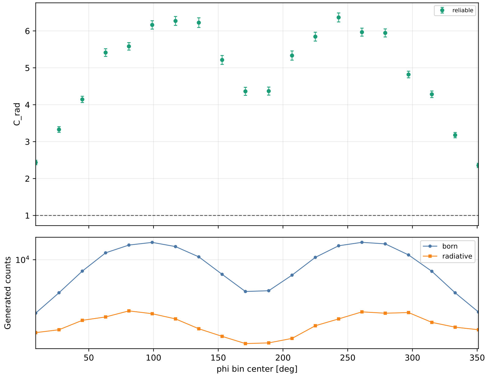
Radiative correction vs phi Q2 3.5-4, xB 0.58-0.7, -t 1.5-2
