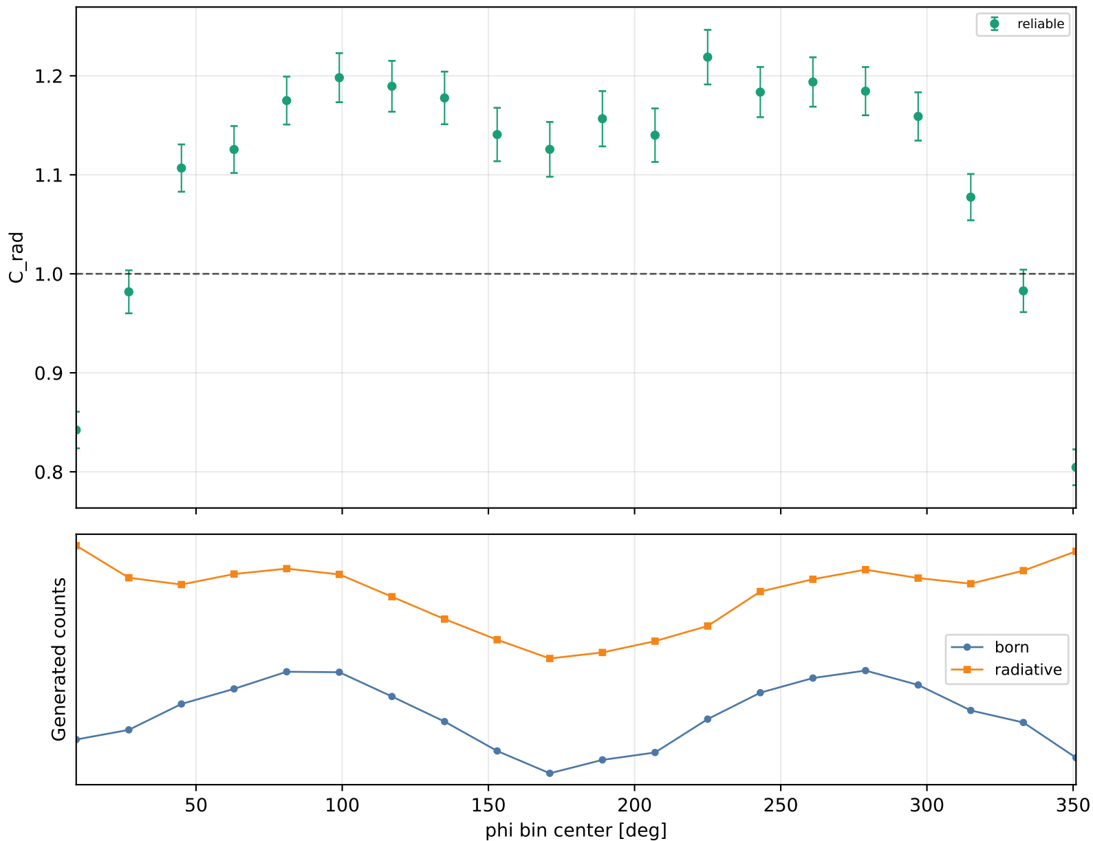
Radiative correction vs phi Q2 2.5-3, xB 0.3-0.38, -t 1-1.5
