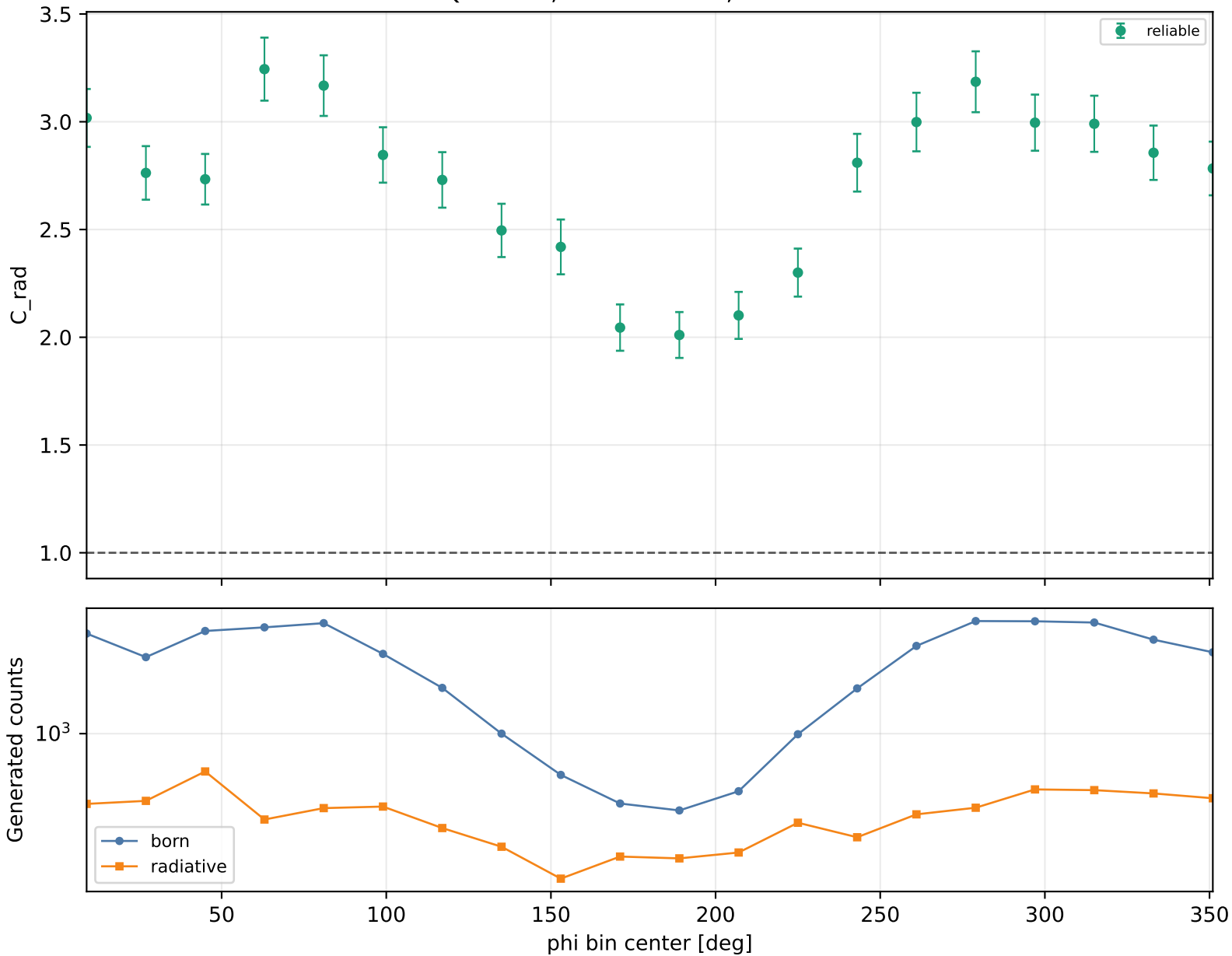
Radiative correction vs phi Q2 2-2.5, xB 0.48-0.58, -t 0.3-0.4
