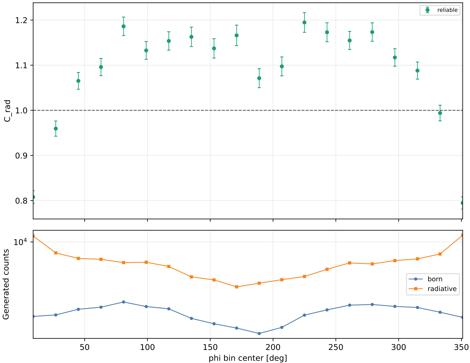
Radiative correction vs phi Q2 1.5-2, xB 0.2-0.25, -t 1-1.5
