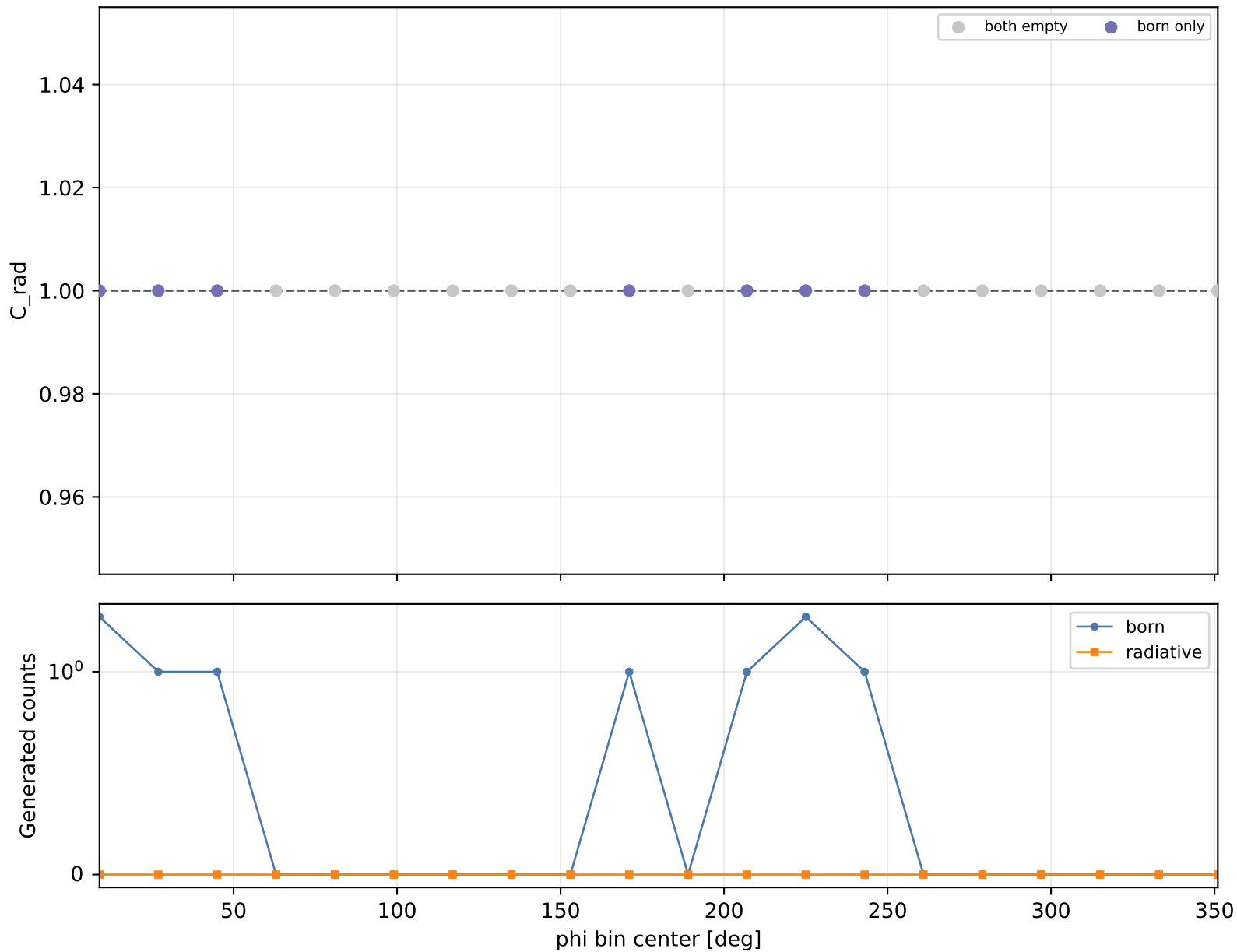
Radiative correction vs phi Q2 1.5-2, xB 0.48-0.58, -t 0.2-0.3
