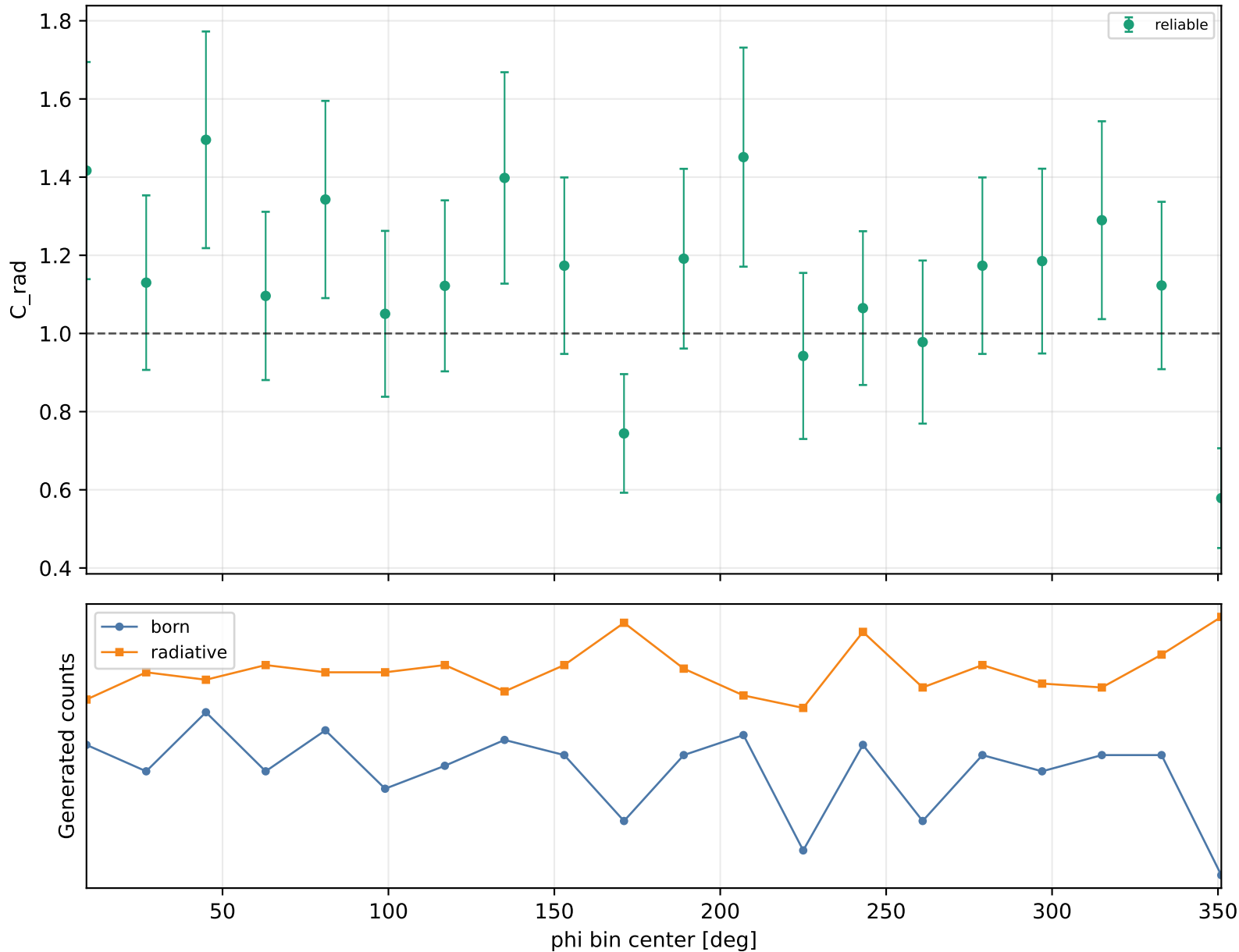
Radiative correction vs phi Q2 3.5-4, xB 0.3-0.38, -t 0.15-0.2
