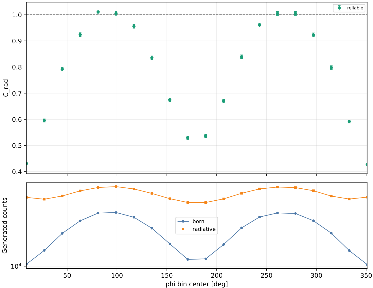
Radiative correction vs phi Q2 1.5-2, xB 0.38-0.48, -t 1.5-2
