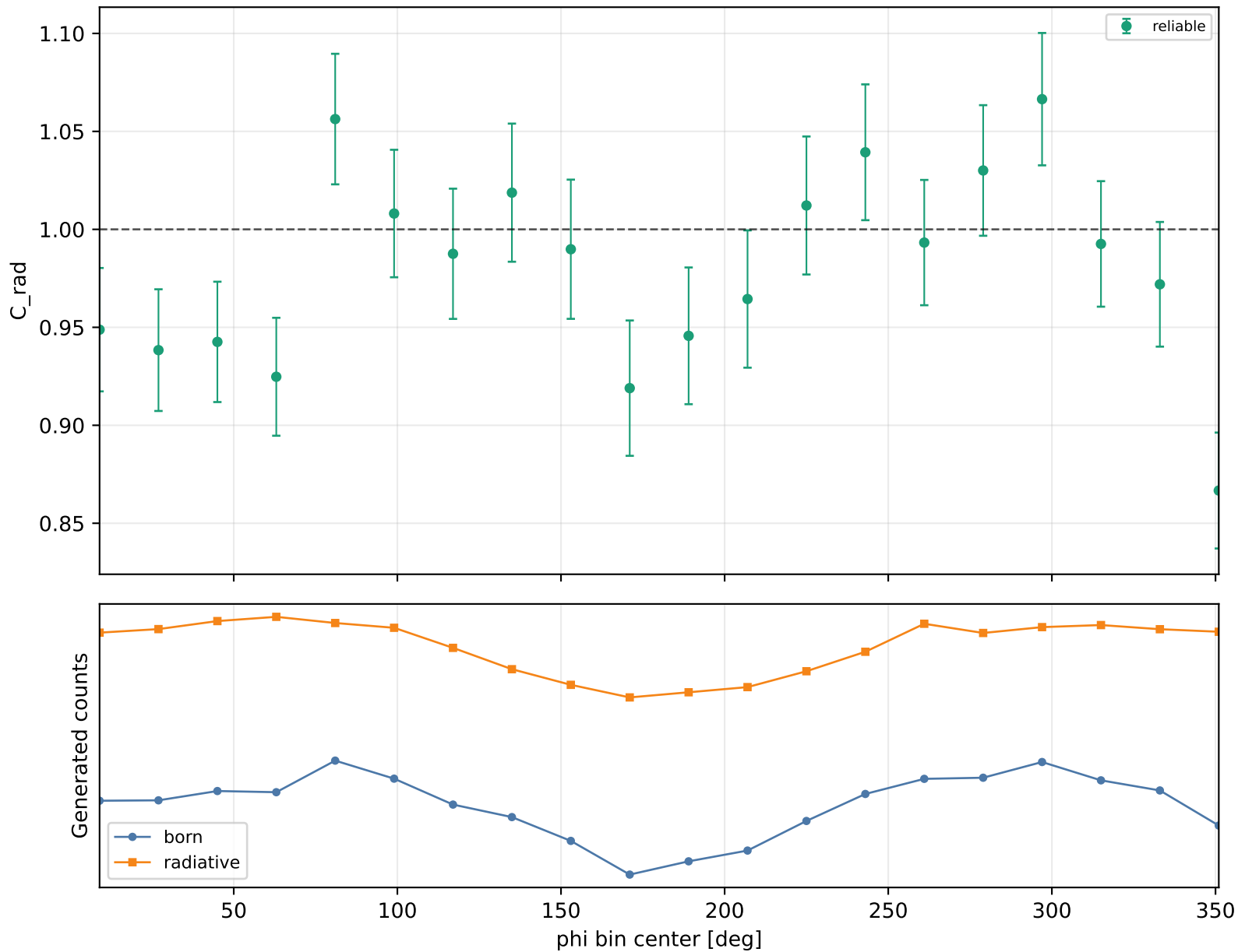
Radiative correction vs phi Q2 2.5-3, xB 0.25-0.3, -t 0.4-0.6
