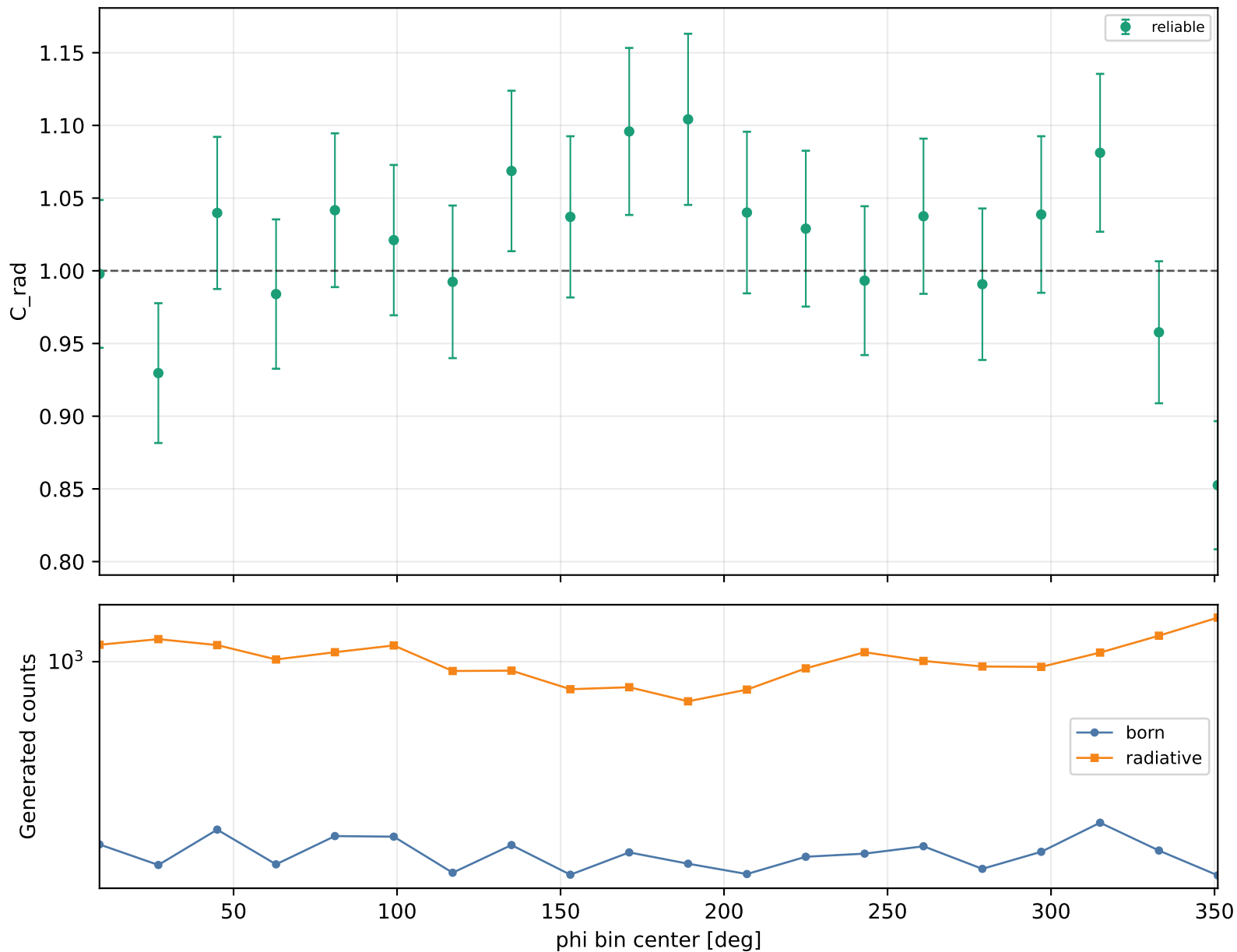
Radiative correction vs phi Q2 2-2.5, xB 0.2-0.25, -t 1.5-2
