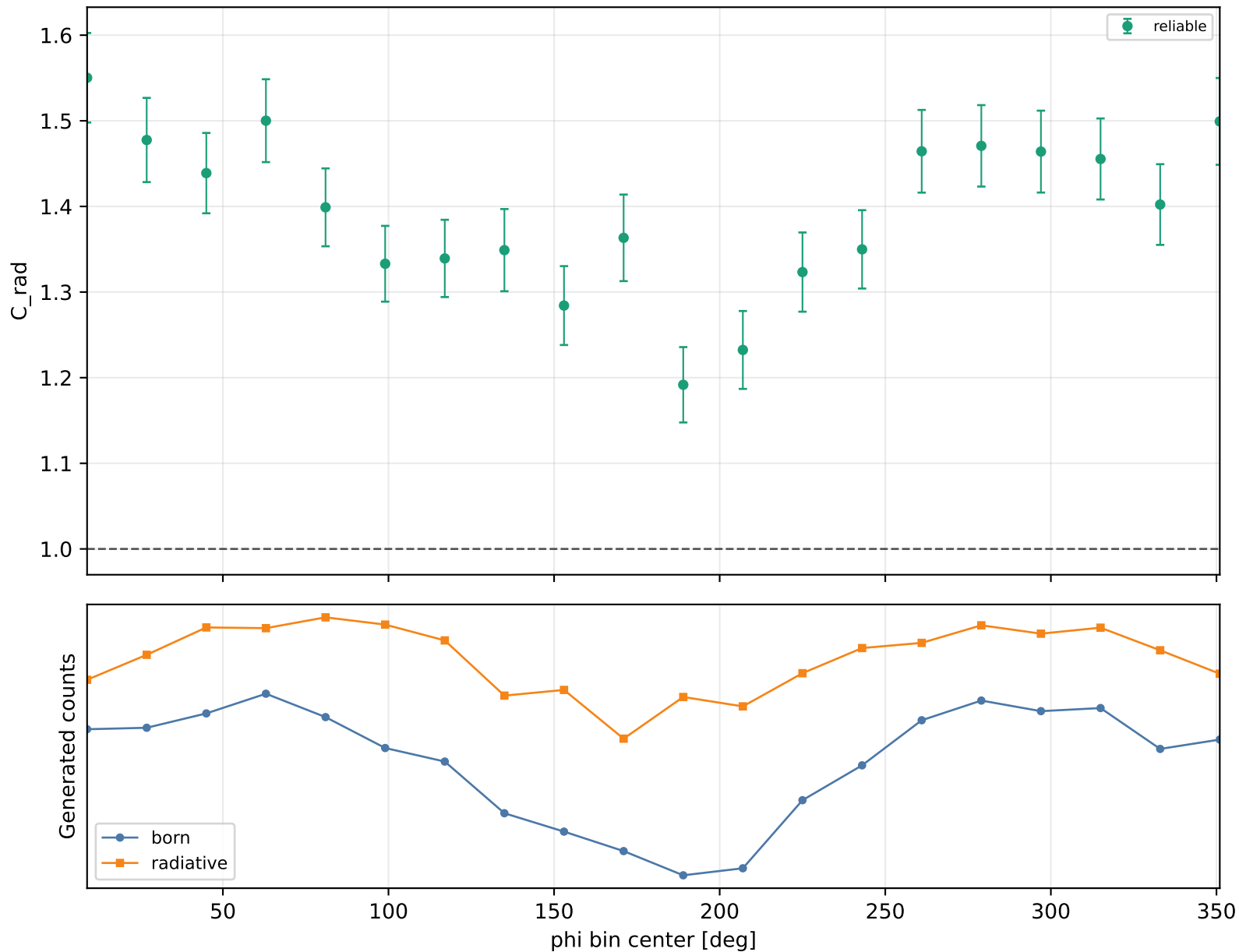
Radiative correction vs phi Q2 2.5-3, xB 0.38-0.48, -t 0.2-0.3
