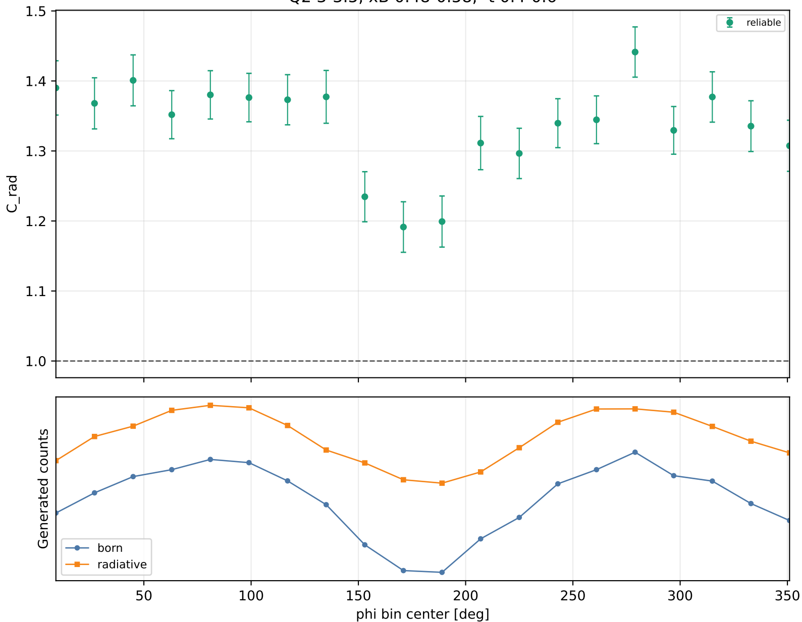
Radiative correction vs phi Q2 3-3.5, xB 0.48-0.58, -t 0.4-0.6
