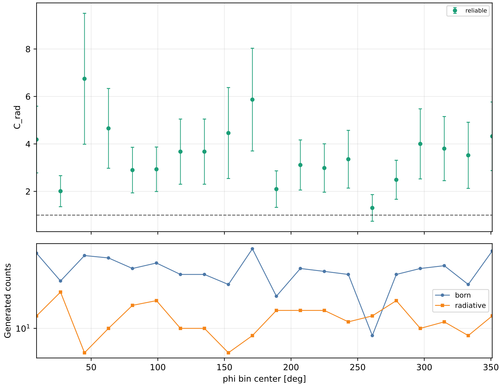
Radiative correction vs phi Q2 2.5-3, xB 0.38-0.48, -t 0.15-0.2
