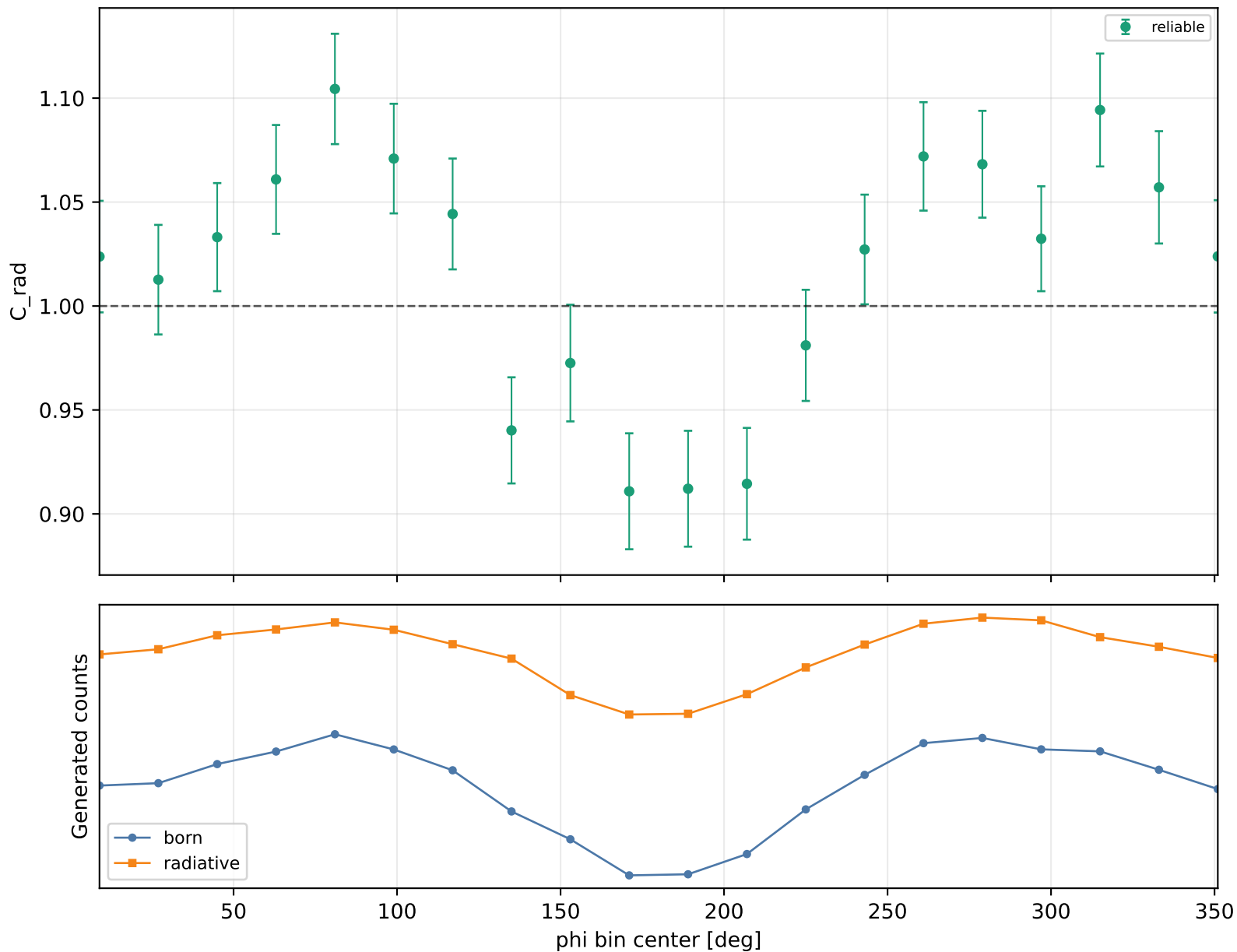
Radiative correction vs phi Q2 1.5-2, xB 0.15-0.2, -t 0.09-0.15
