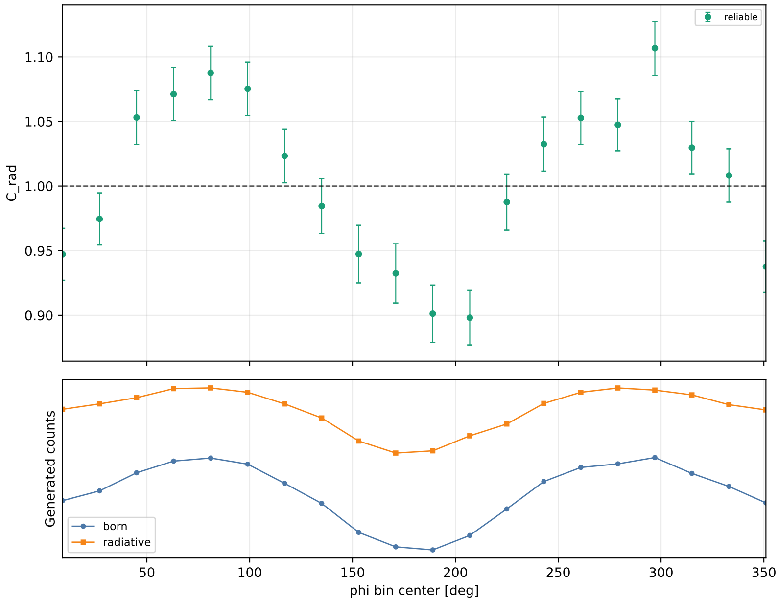
Radiative correction vs phi Q2 1.5-2, xB 0.15-0.2, -t 0.2-0.3
