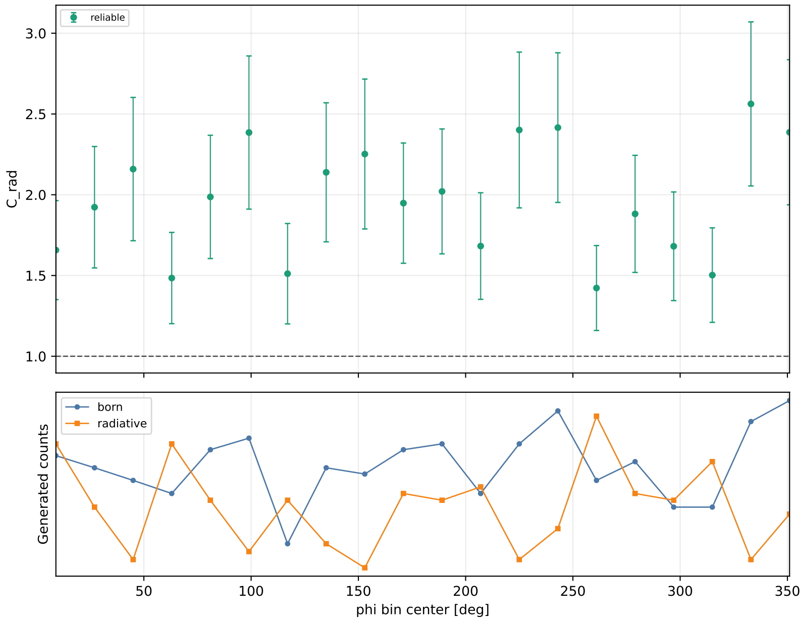
Radiative correction vs phi Q2 4-4.6, xB 0.48-0.58, -t 0.3-0.4
