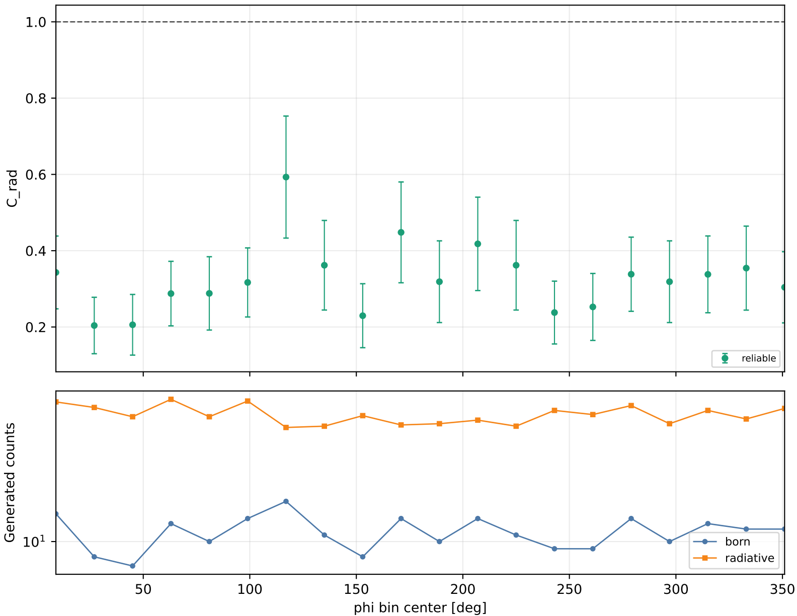
Radiative correction vs phi Q2 3-3.5, xB 0.25-0.3, -t 0.4-0.6
