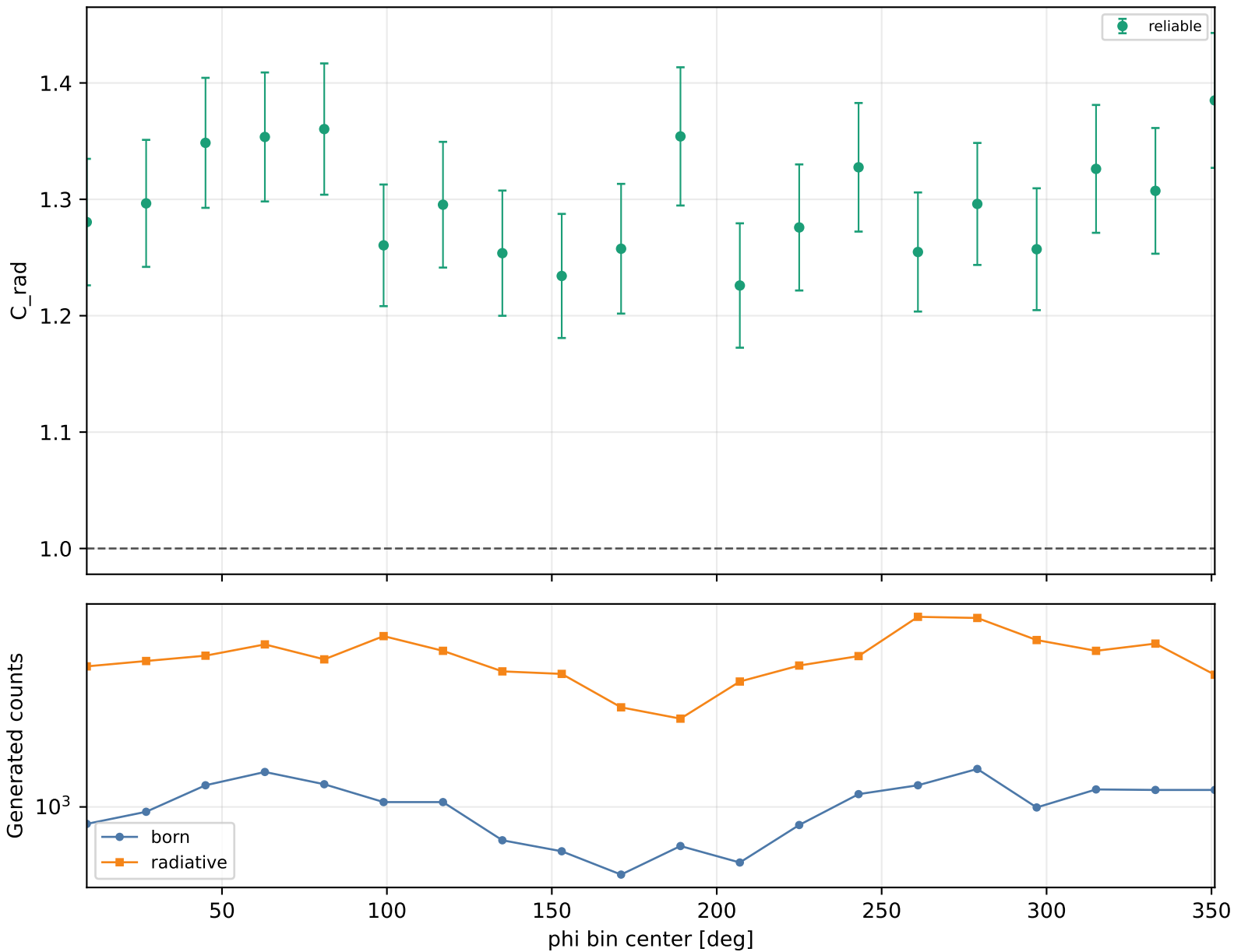
Radiative correction vs phi Q2 4-4.6, xB 0.48-0.58, -t 0.4-0.6
