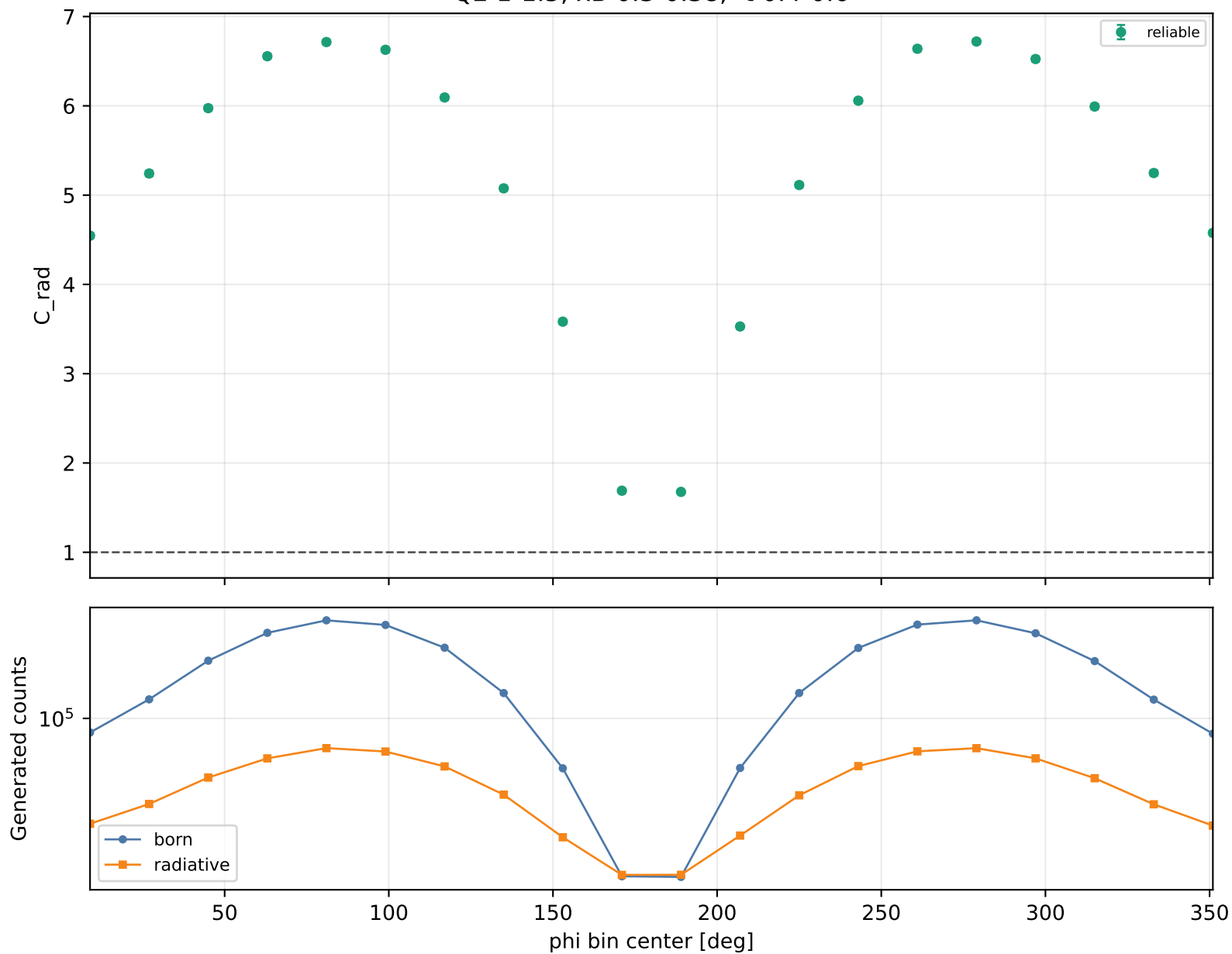
Radiative correction vs phi Q2 1-1.5, xB 0.3-0.38, -t 0.4-0.6
