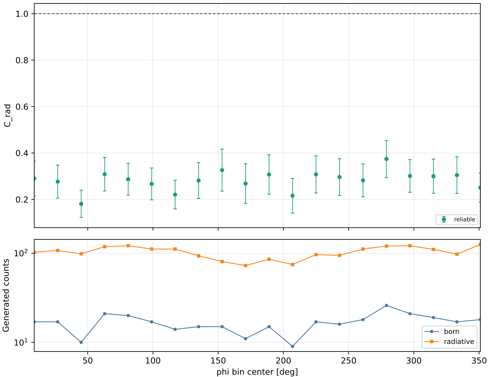
Radiative correction vs phi Q2 1-1.5, xB 0.05-0.1, -t 0.2-0.3
