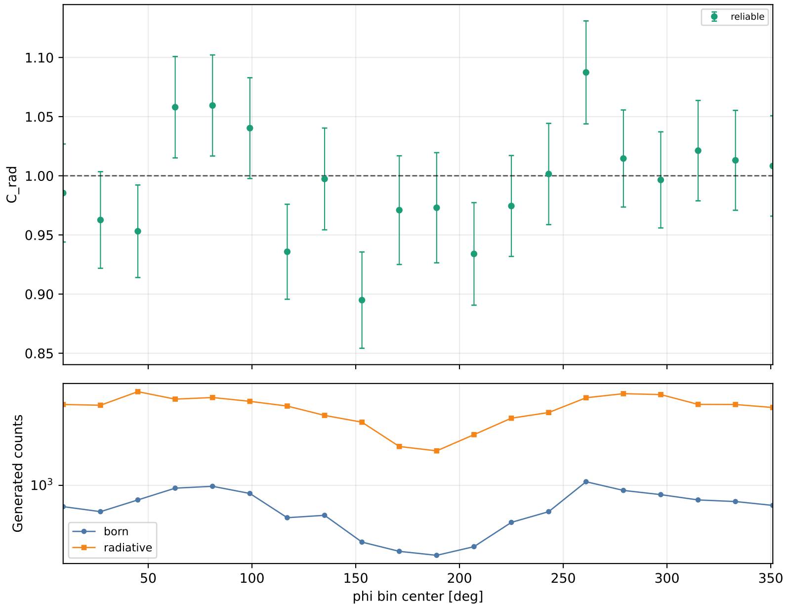
Radiative correction vs phi Q2 2.5-3, xB 0.25-0.3, -t 0.3-0.4
