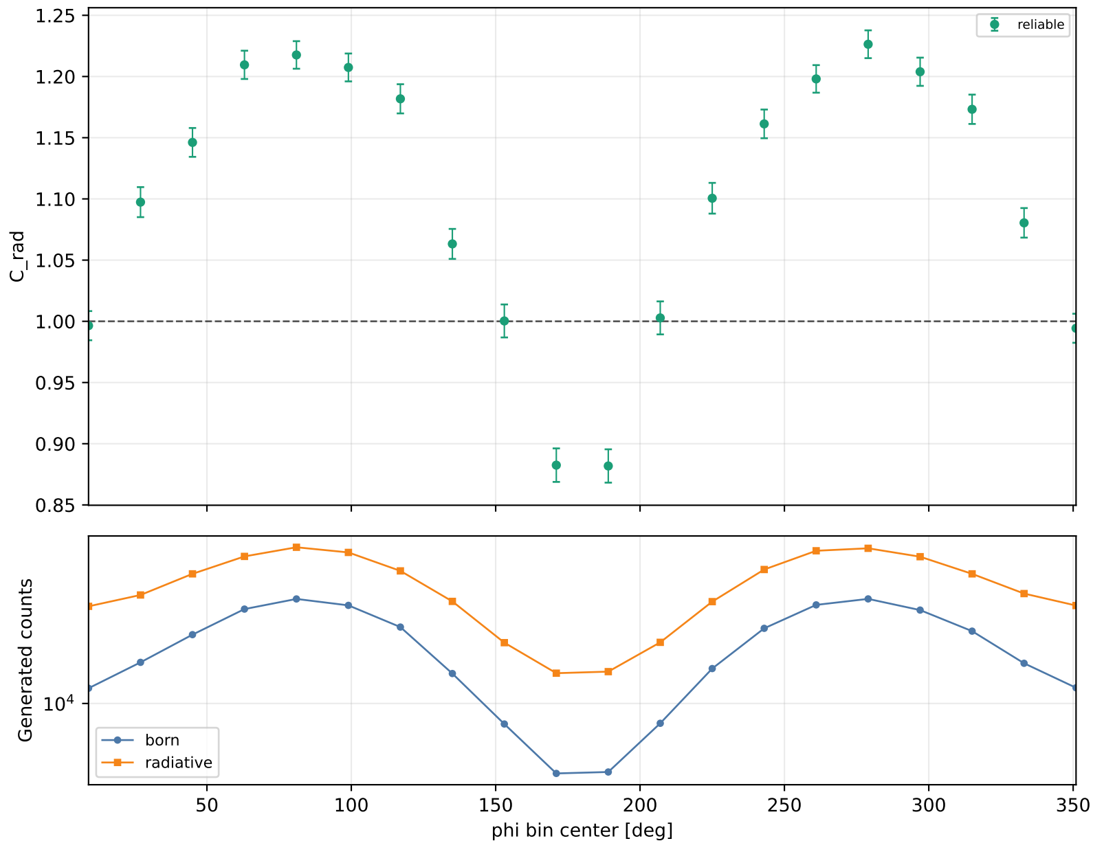
Radiative correction vs phi Q2 1.5-2, xB 0.25-0.3, -t 0.4-0.6
