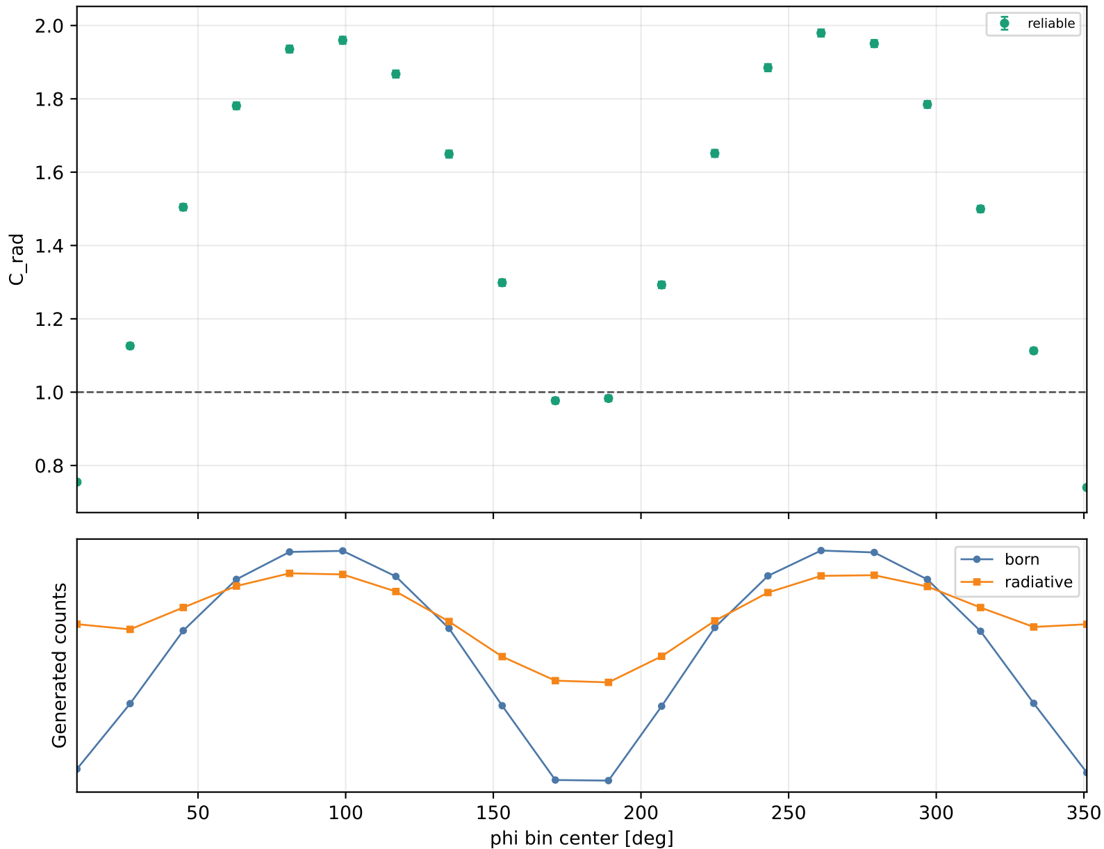
Radiative correction vs phi Q2 1.5-2, xB 0.38-0.48, -t 1-1.5
