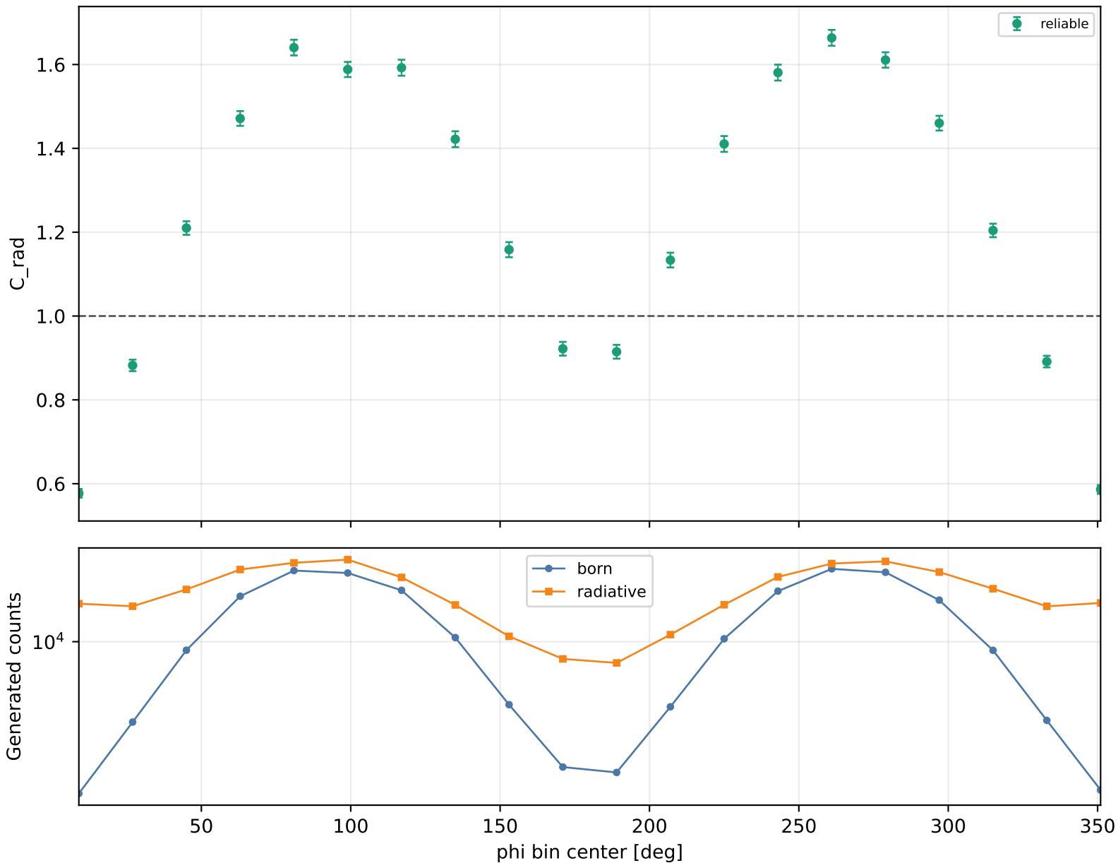
Radiative correction vs phi Q2 2.5-3, xB 0.48-0.58, -t 1.5-2
