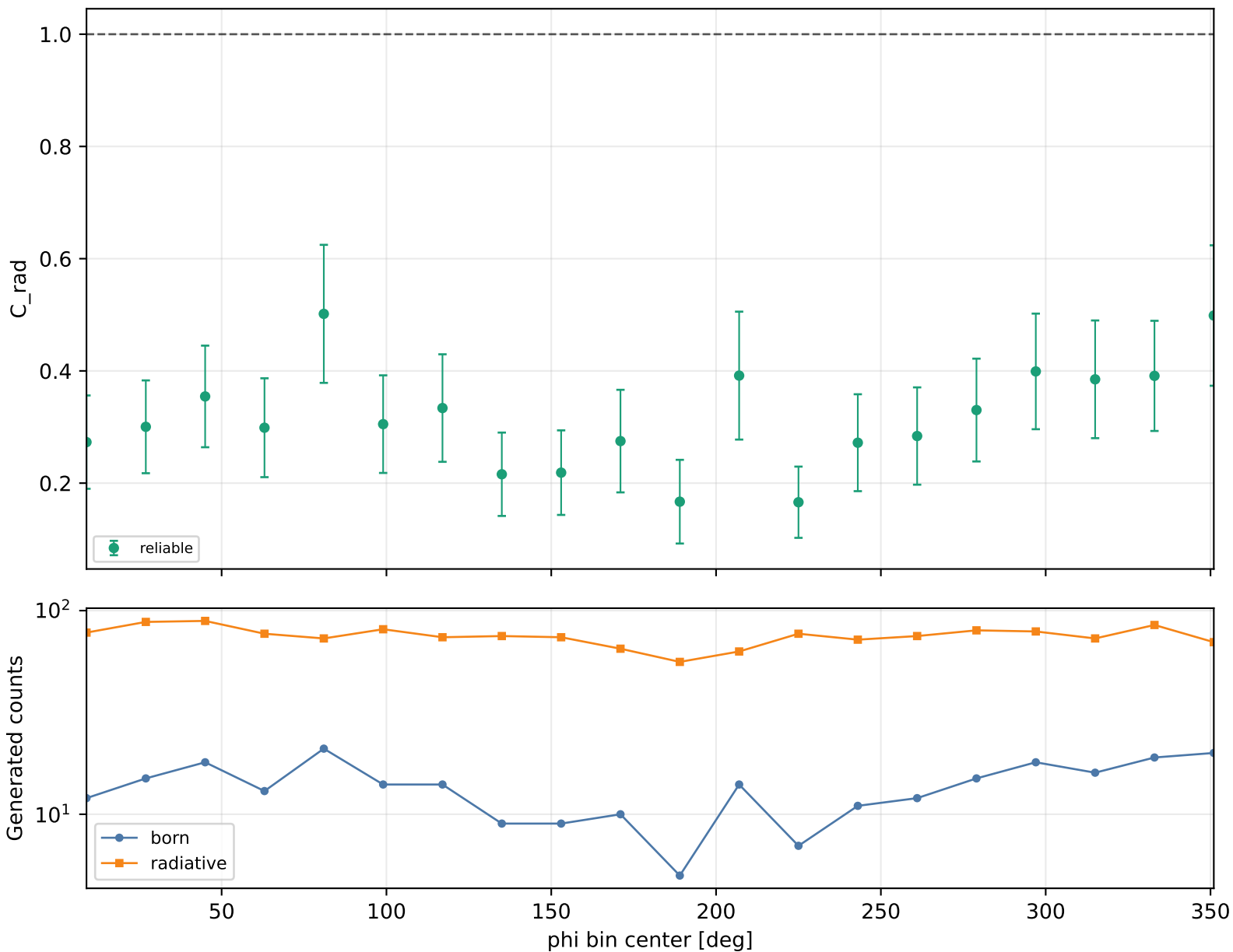
Radiative correction vs phi Q2 1.5-2, xB 0.1-0.15, -t 0.4-0.6
