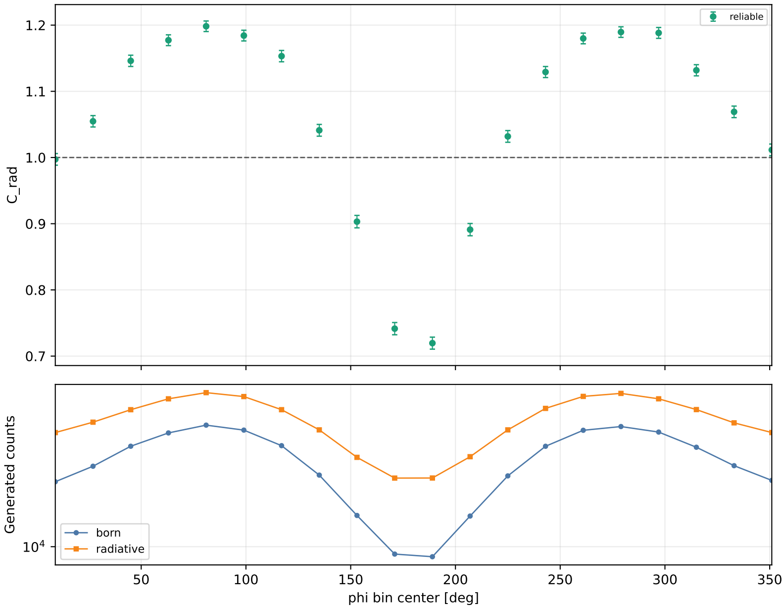
Radiative correction vs phi Q2 1-1.5, xB 0.15-0.2, -t 0.2-0.3
