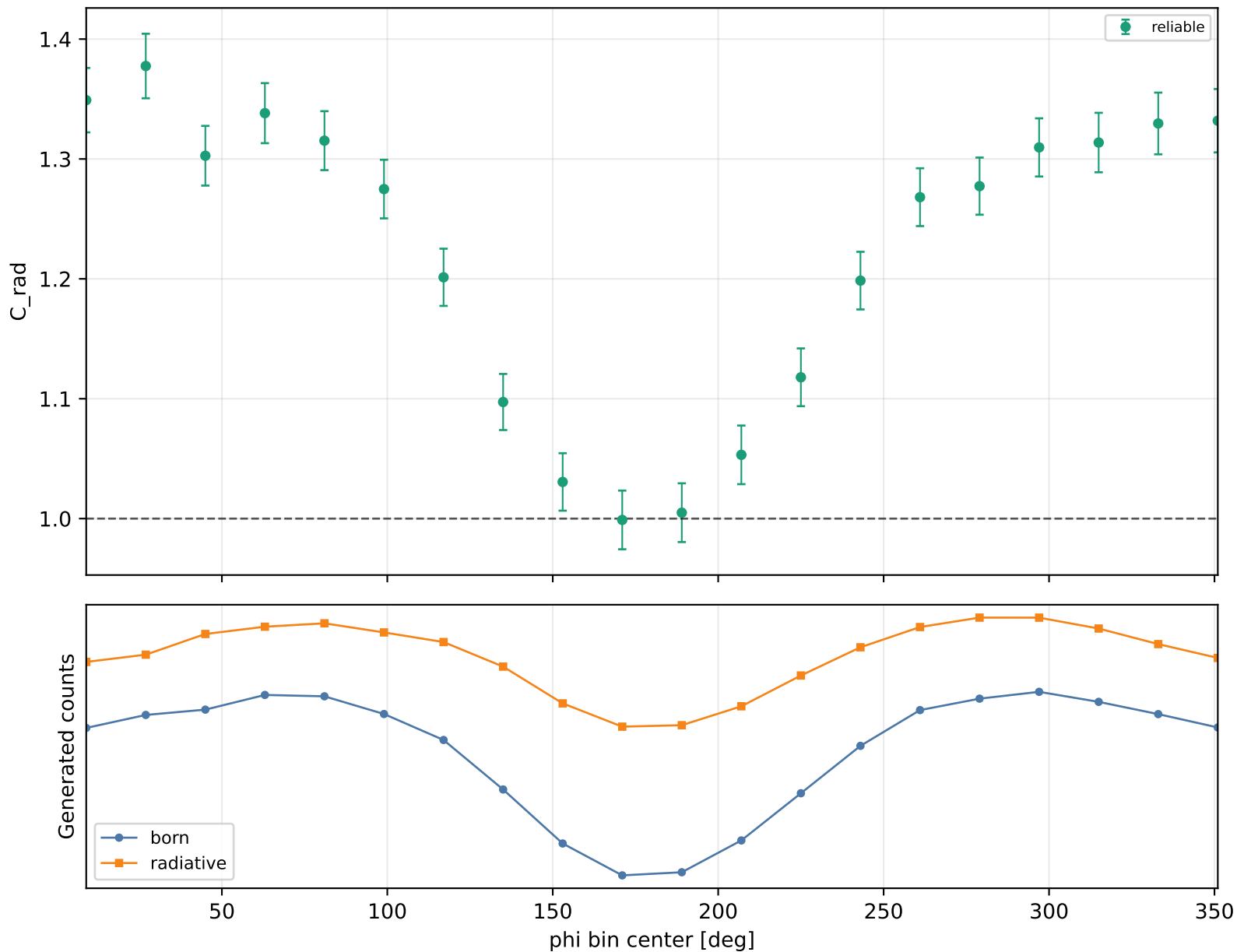
Radiative correction vs phi Q2 1.5-2, xB 0.25-0.3, -t 0.09-0.15
