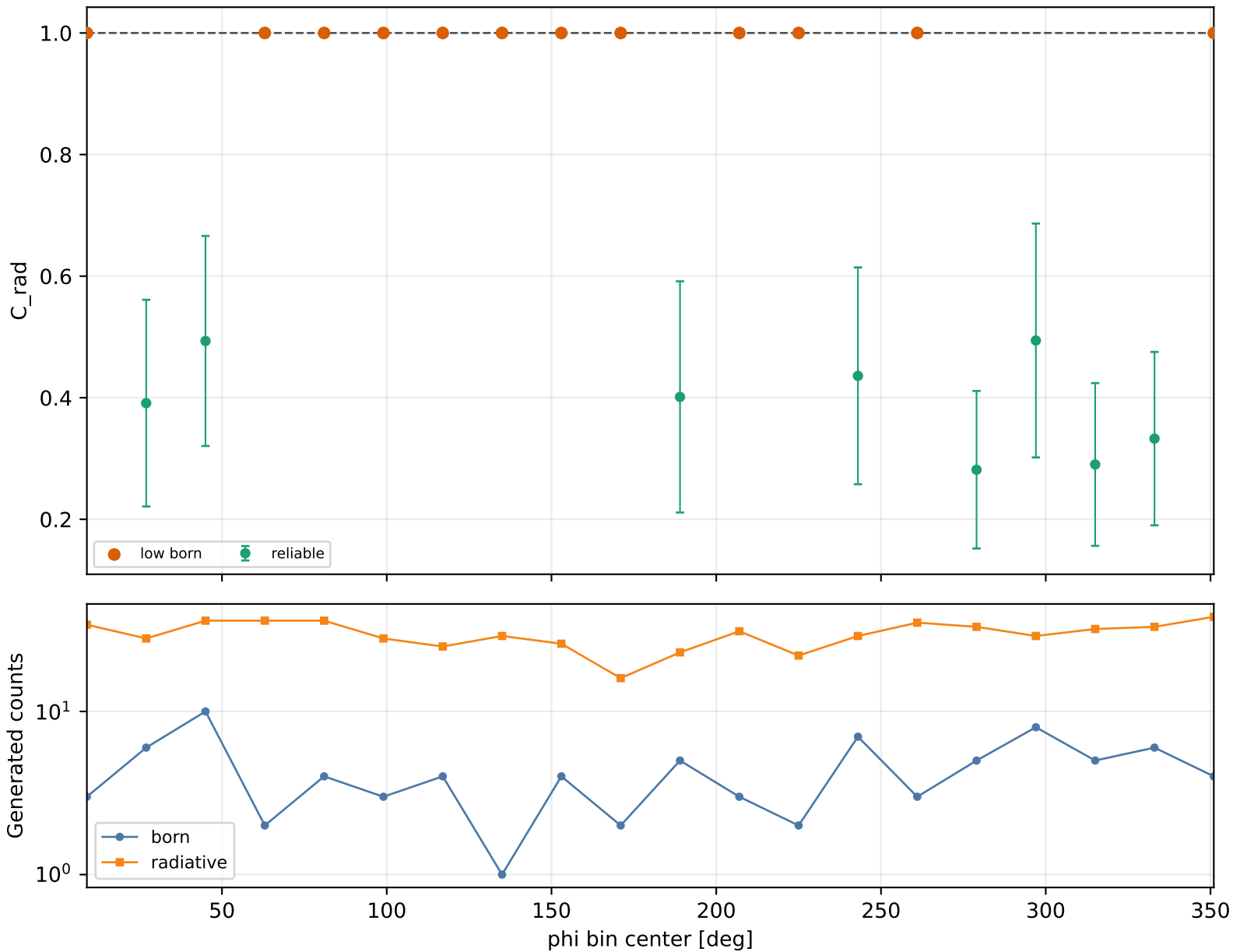
Radiative correction vs phi Q2 2-2.5, xB 0.15-0.2, -t 0.15-0.2
