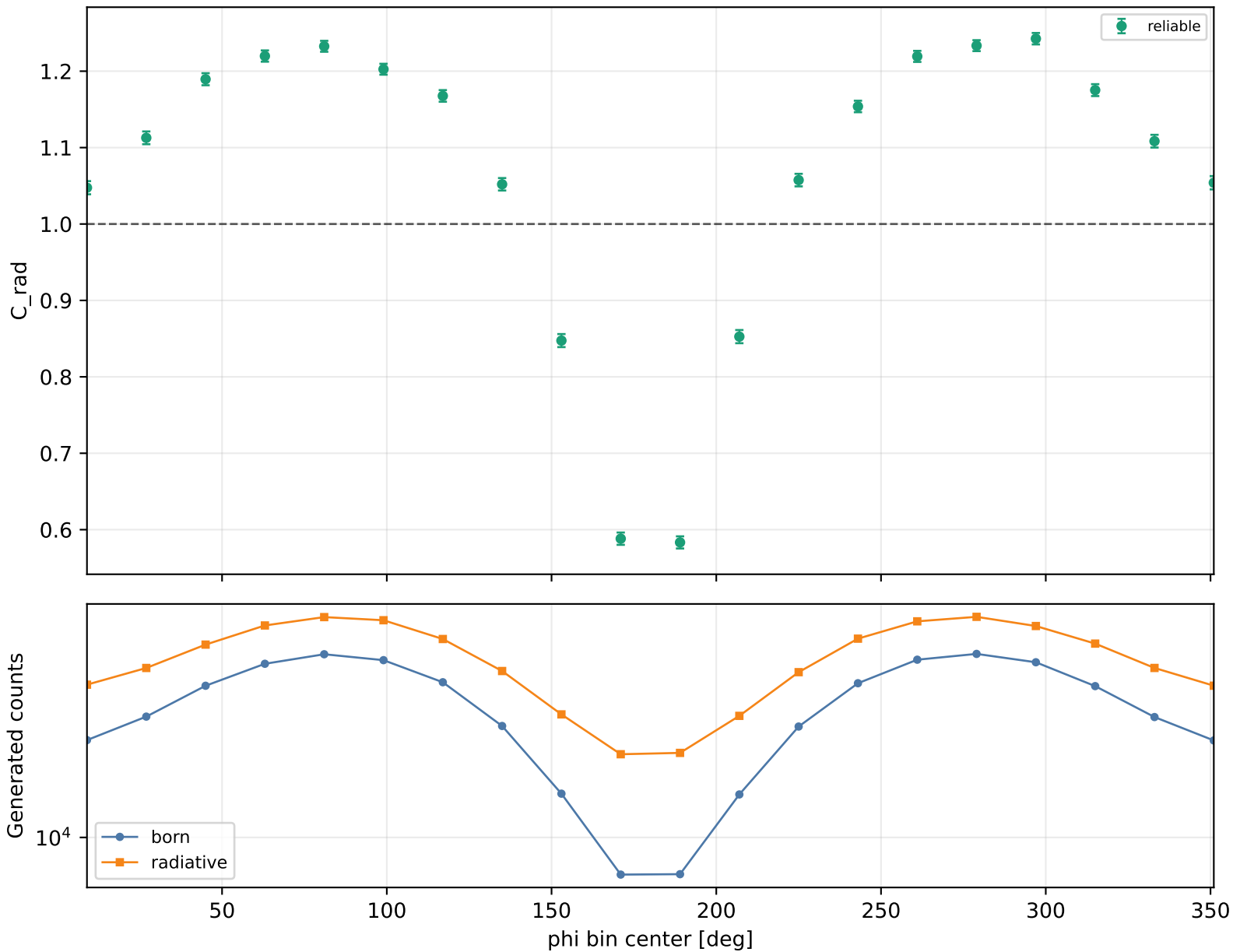
Radiative correction vs phi Q2 1-1.5, xB 0.2-0.25, -t 0.3-0.4
