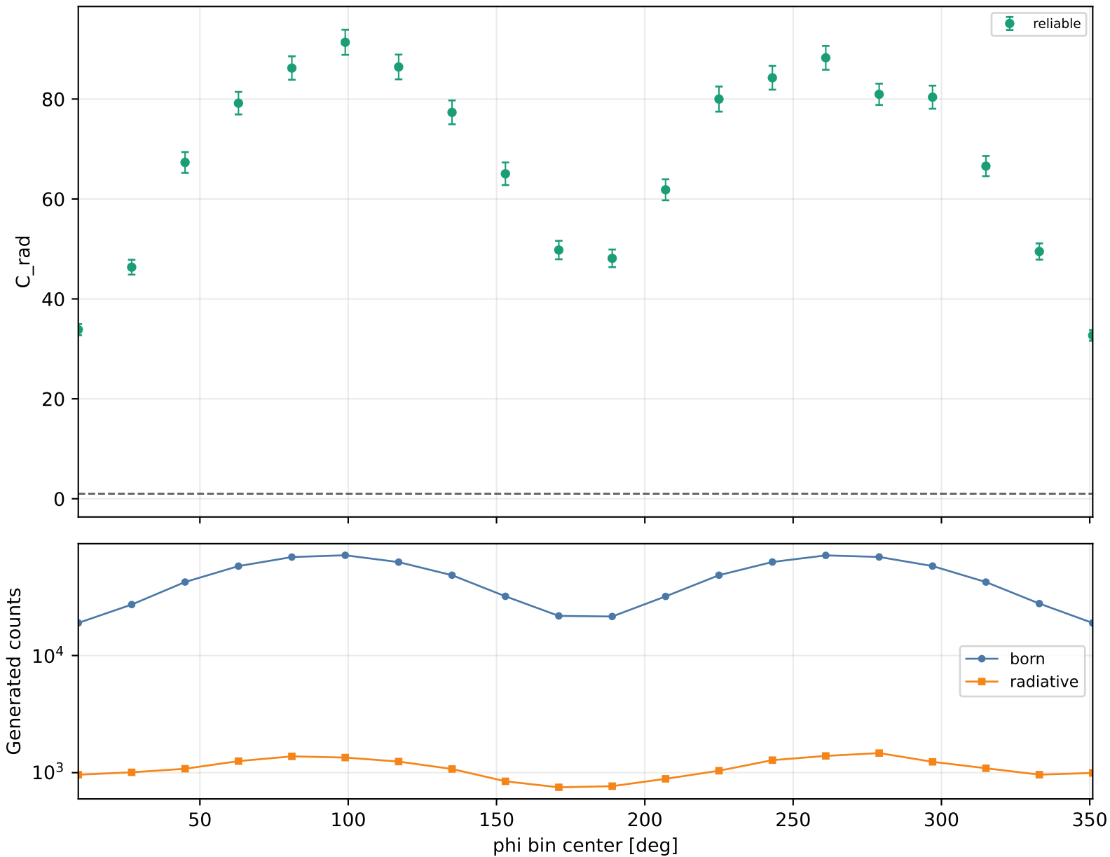
Radiative correction vs phi Q2 1-1.5, xB 0.38-0.48, -t 1-1.5
