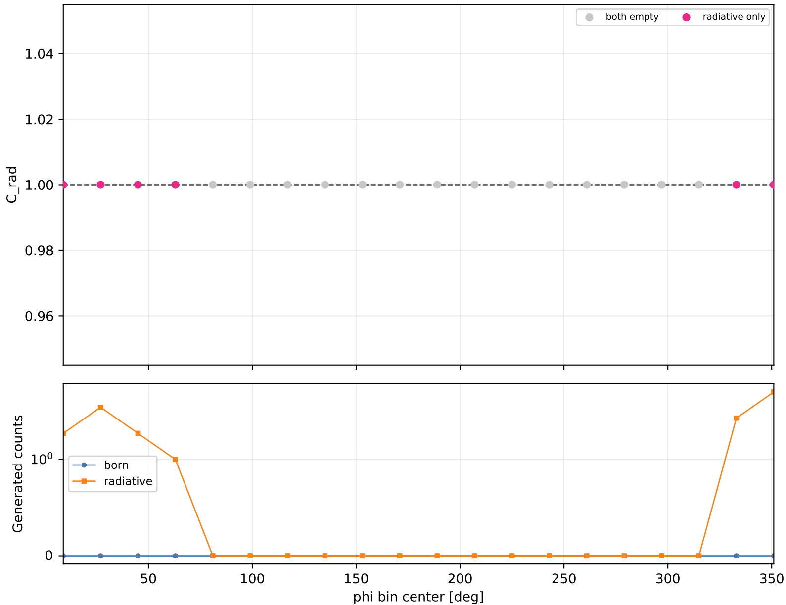
Radiative correction vs phi Q2 5.5-6.535, xB 0.48-0.58, -t 1-1.5
