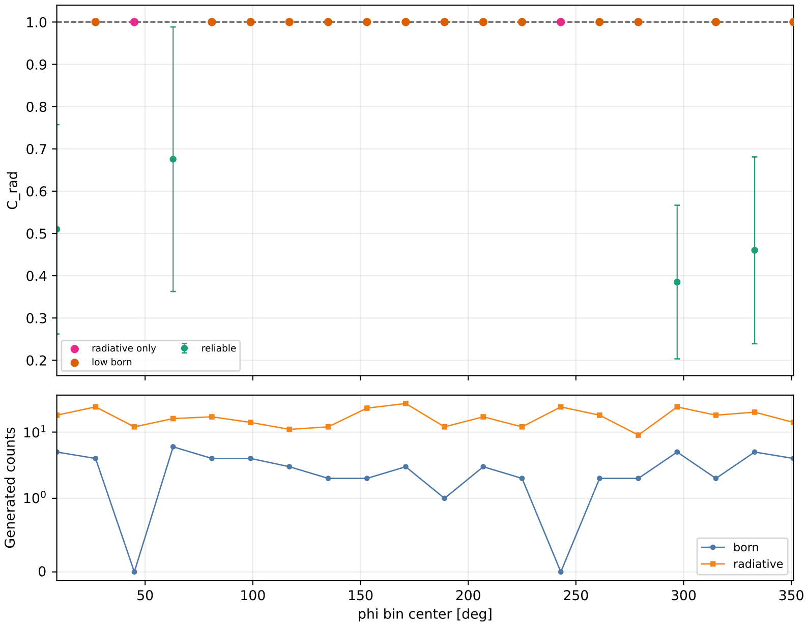
Radiative correction vs phi Q2 1-1.5, xB 0.05-0.1, -t 1.5-2
