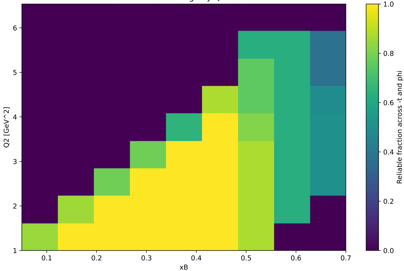
Reliable-bin coverage by Q2 and xB
