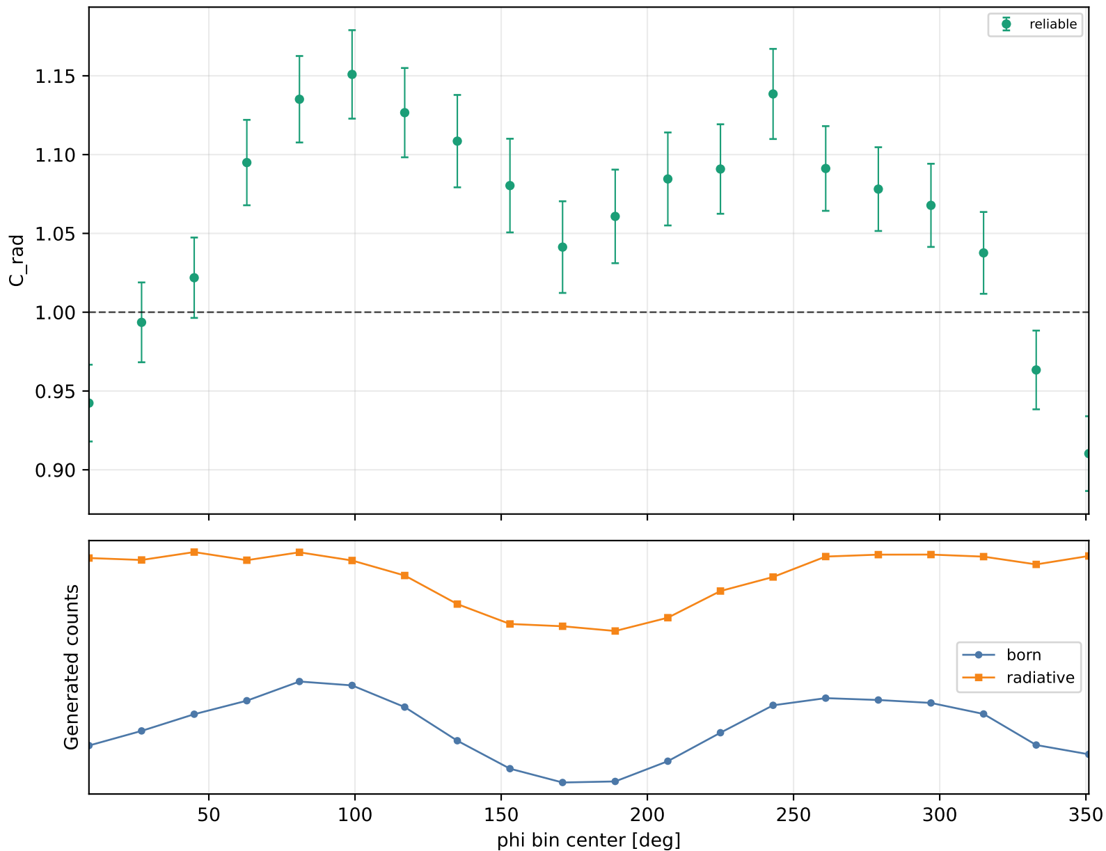
Radiative correction vs phi Q2 3-3.5, xB 0.3-0.38, -t 0.6-1
