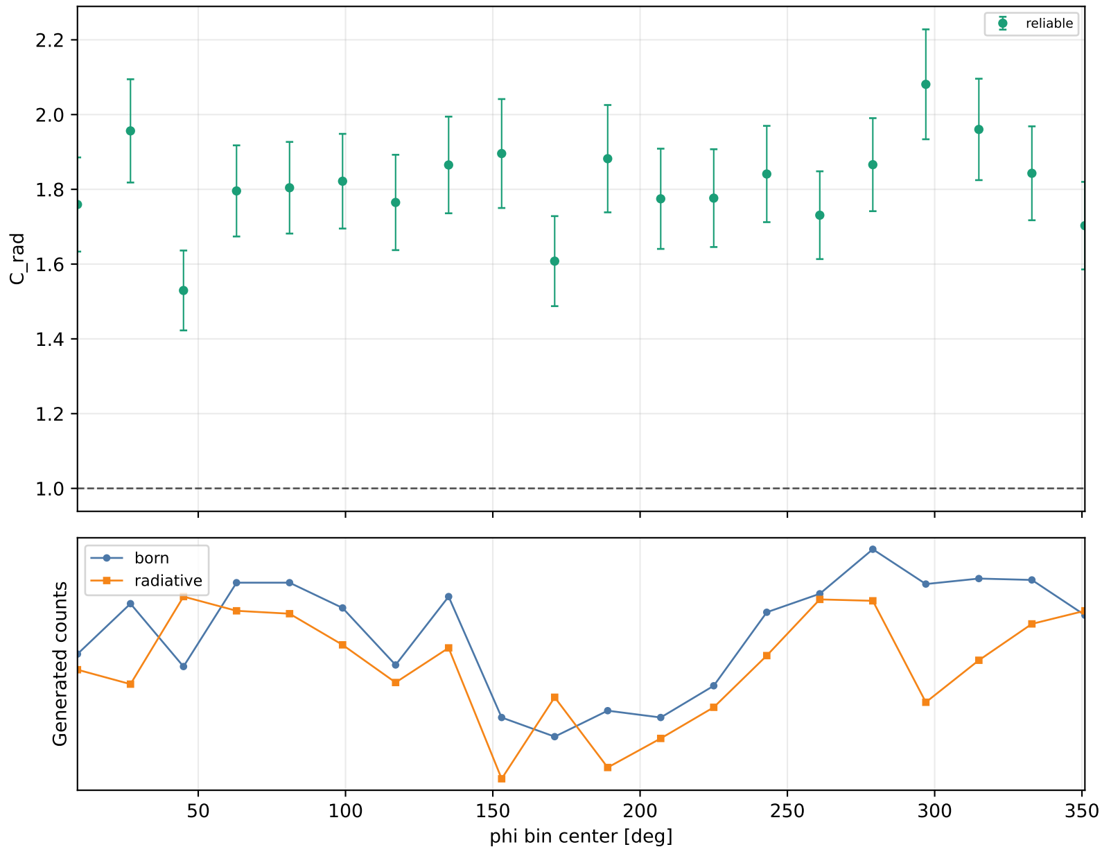
Radiative correction vs phi Q2 2.5-3, xB 0.48-0.58, -t 0.3-0.4
