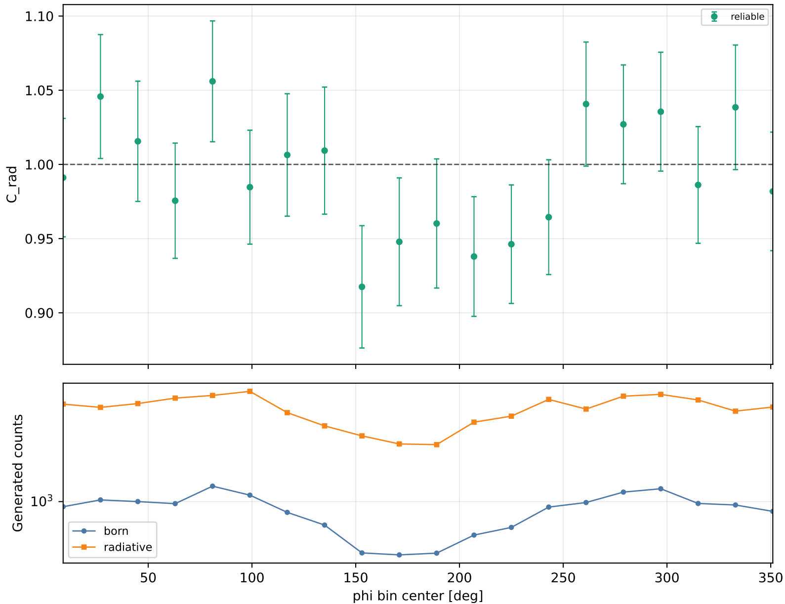
Radiative correction vs phi Q2 2.5-3, xB 0.25-0.3, -t 0.2-0.3
