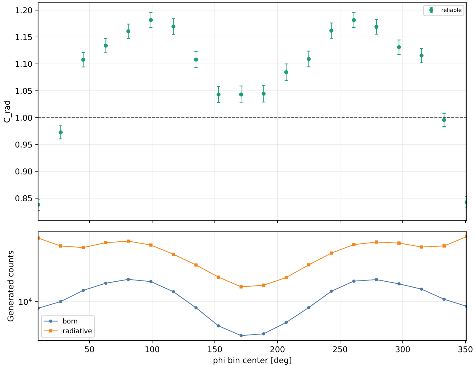
Radiative correction vs phi Q2 1.5-2, xB 0.2-0.25, -t 0.6-1
