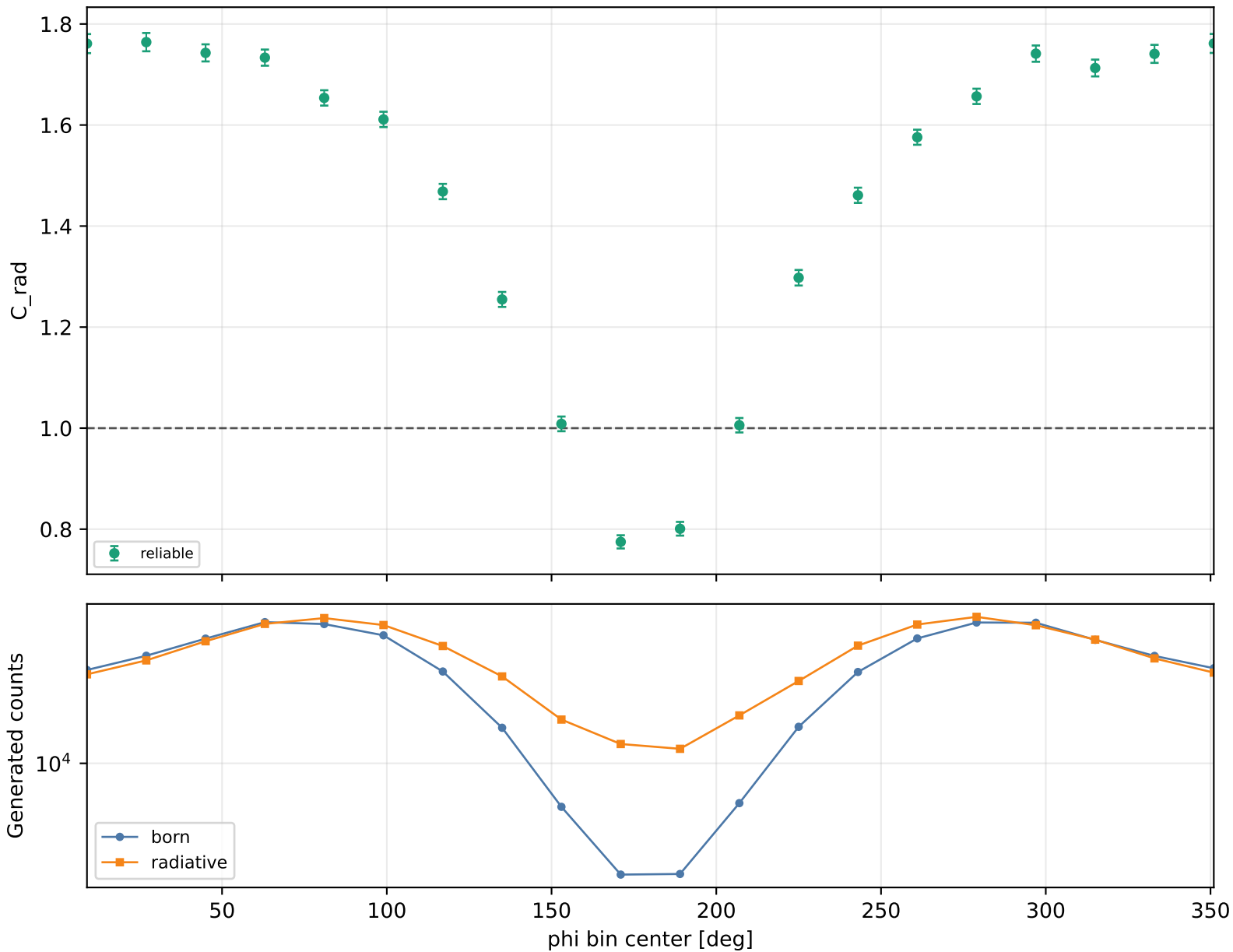
Radiative correction vs phi Q2 1-1.5, xB 0.25-0.3, -t 0.09-0.15
