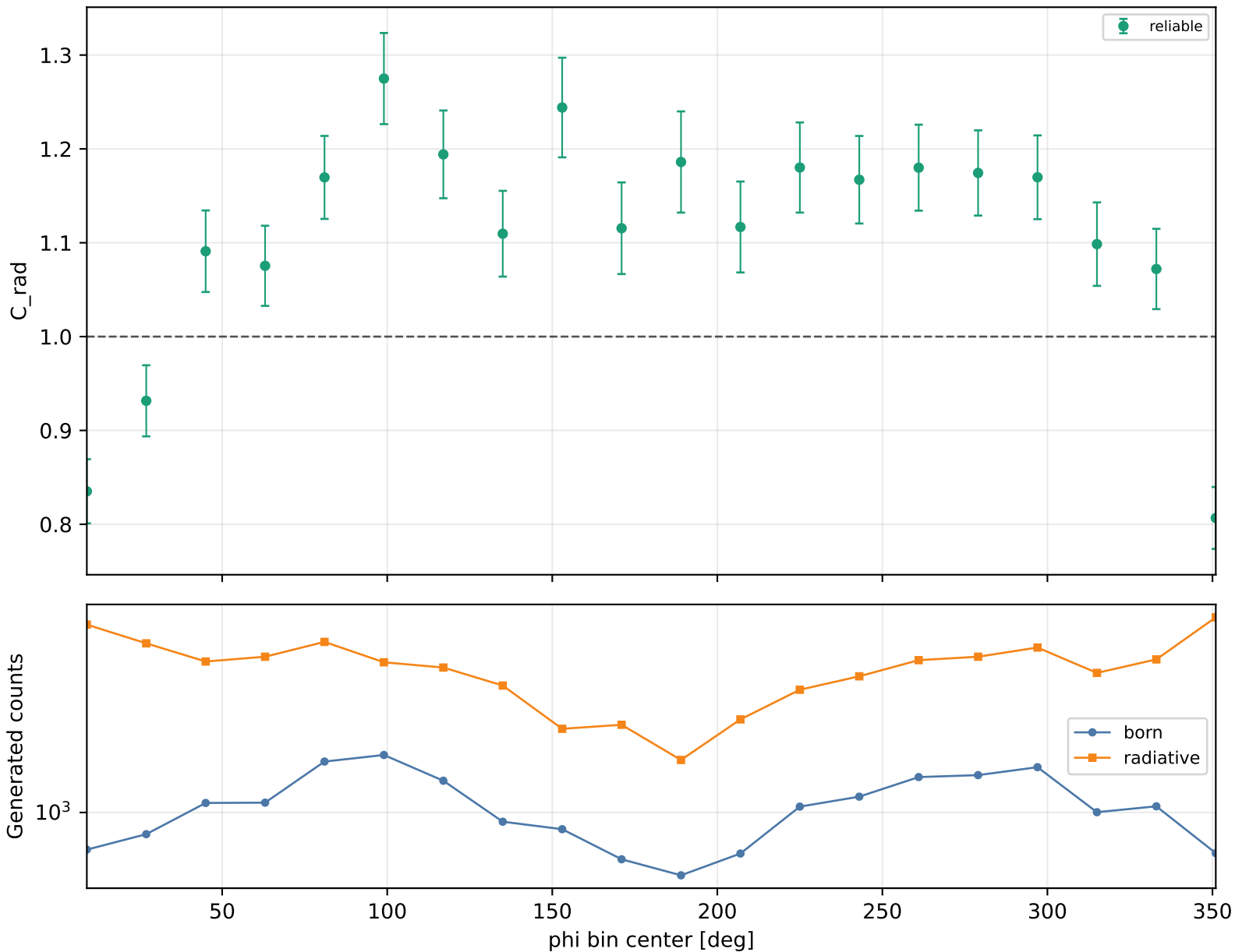
Radiative correction vs phi Q2 3.5-4, xB 0.38-0.48, -t 1.5-2
