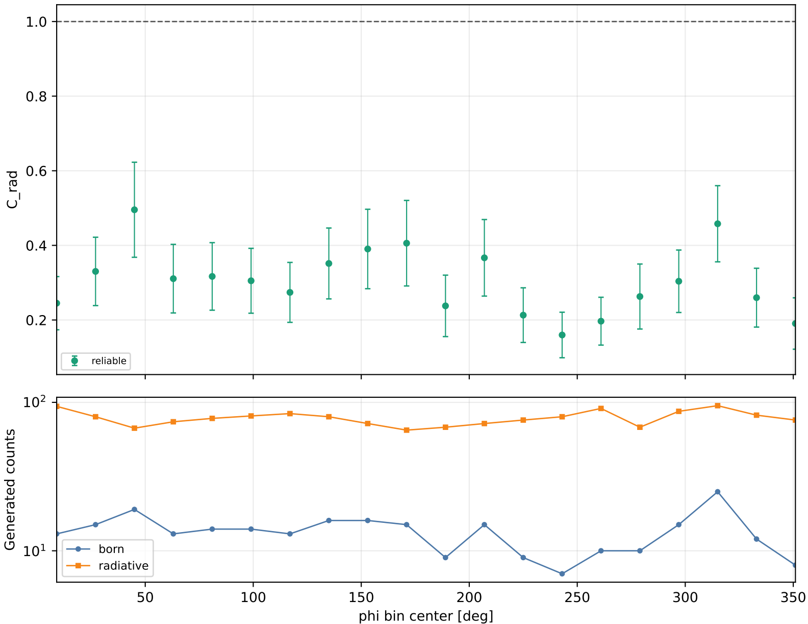
Radiative correction vs phi Q2 1-1.5, xB 0.05-0.1, -t 0.6-1
