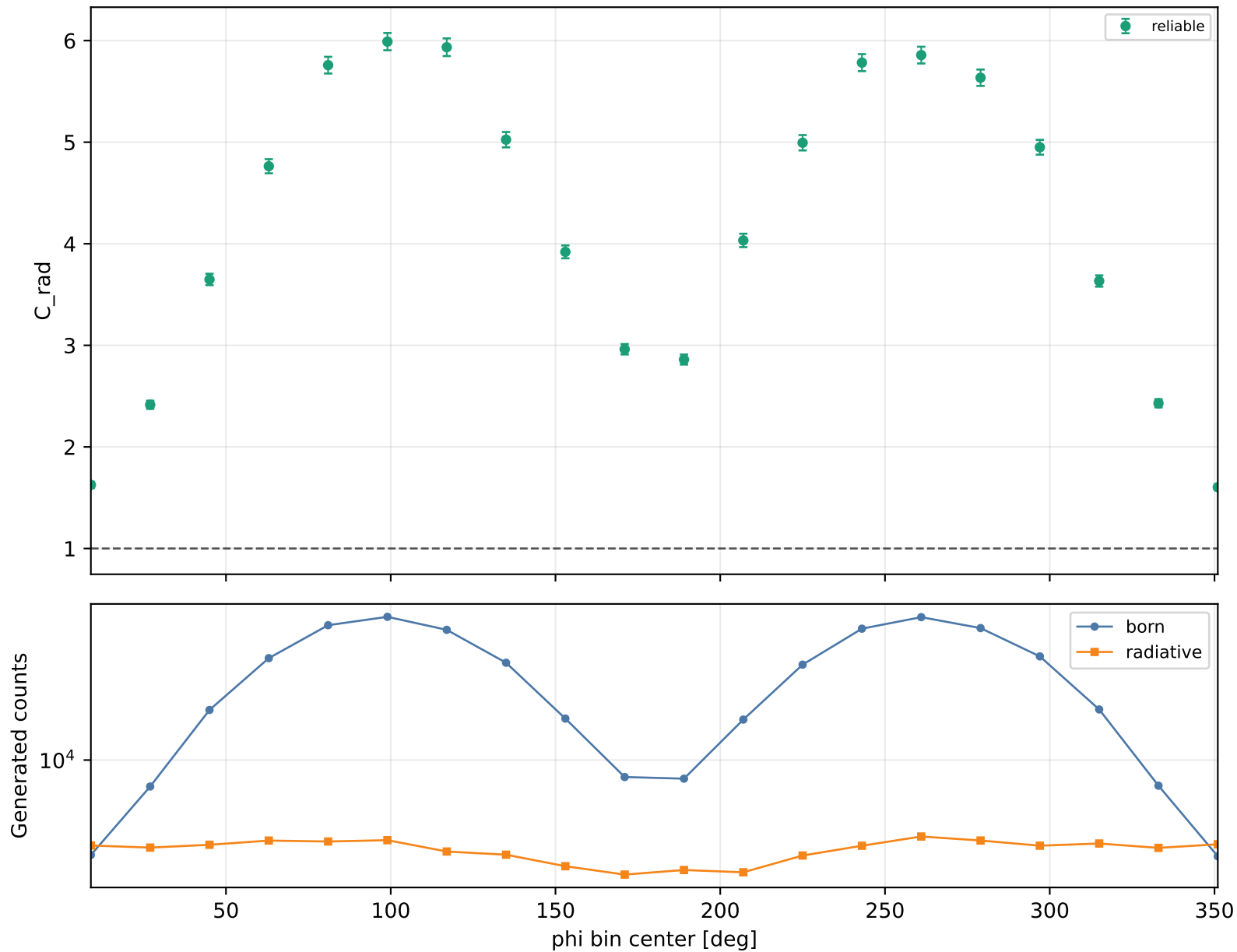
Radiative correction vs phi Q2 3-3.5, xB 0.58-0.7, -t 1.5-2
