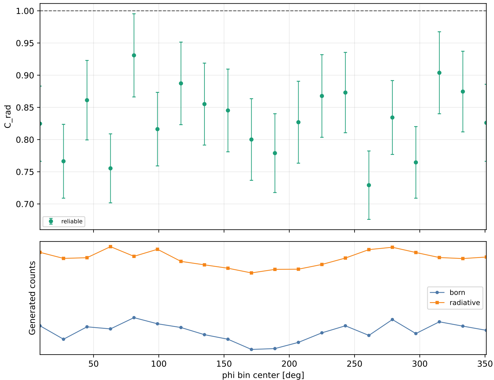
Radiative correction vs phi Q2 3.5-4, xB 0.3-0.38, -t 0.4-0.6
