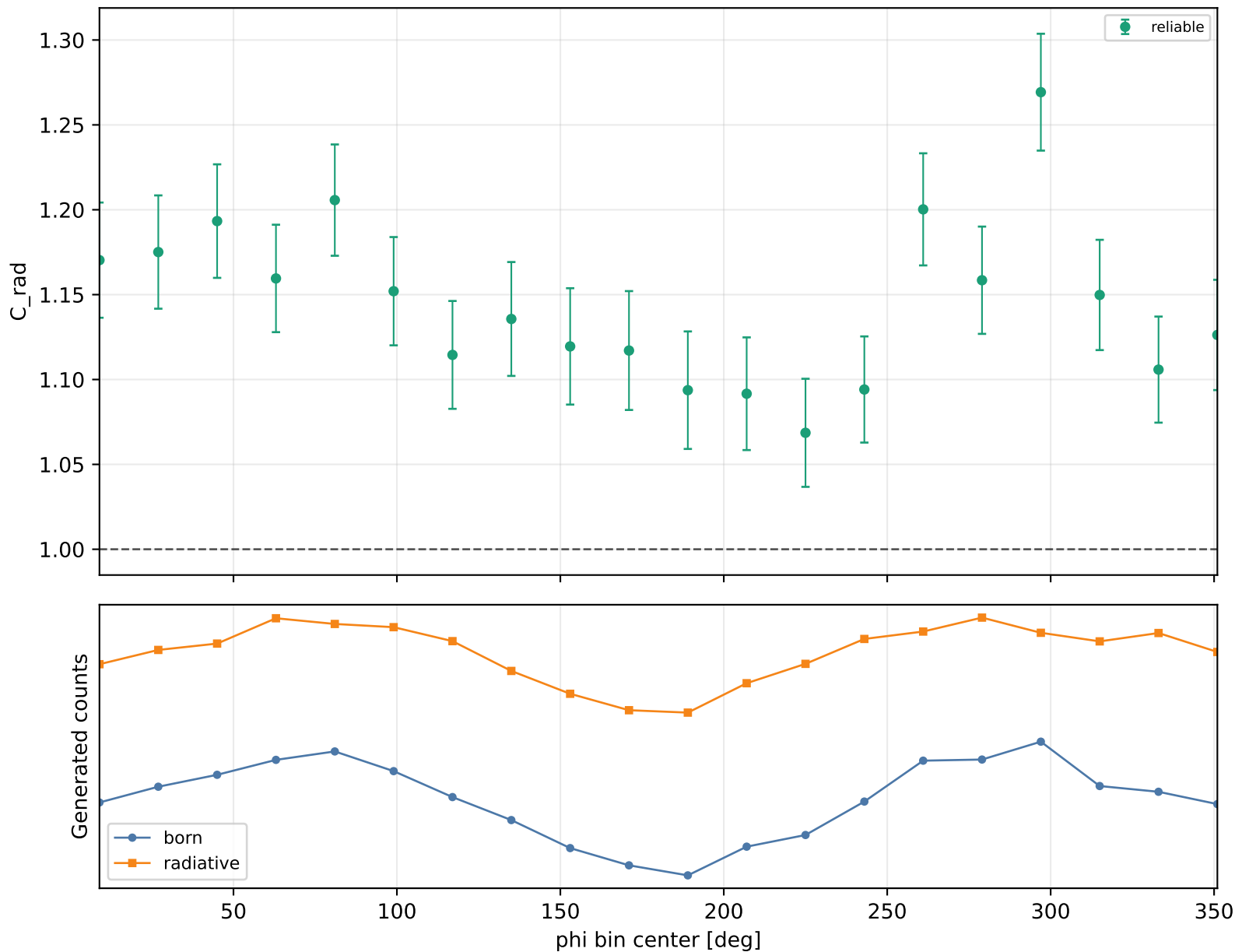
Radiative correction vs phi Q2 3.5-4, xB 0.38-0.48, -t 0.4-0.6
