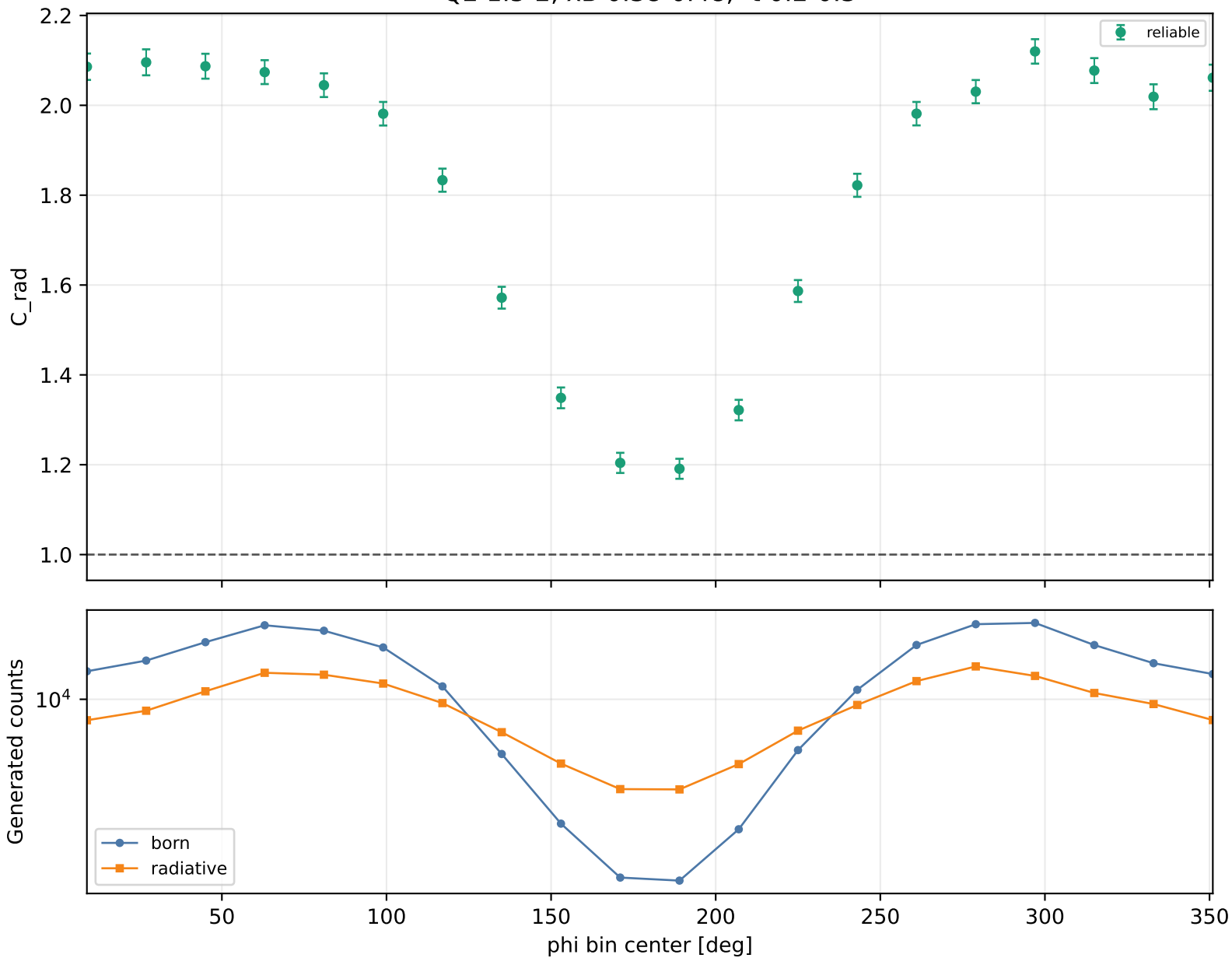
Radiative correction vs phi Q2 1.5-2, xB 0.38-0.48, -t 0.2-0.3
