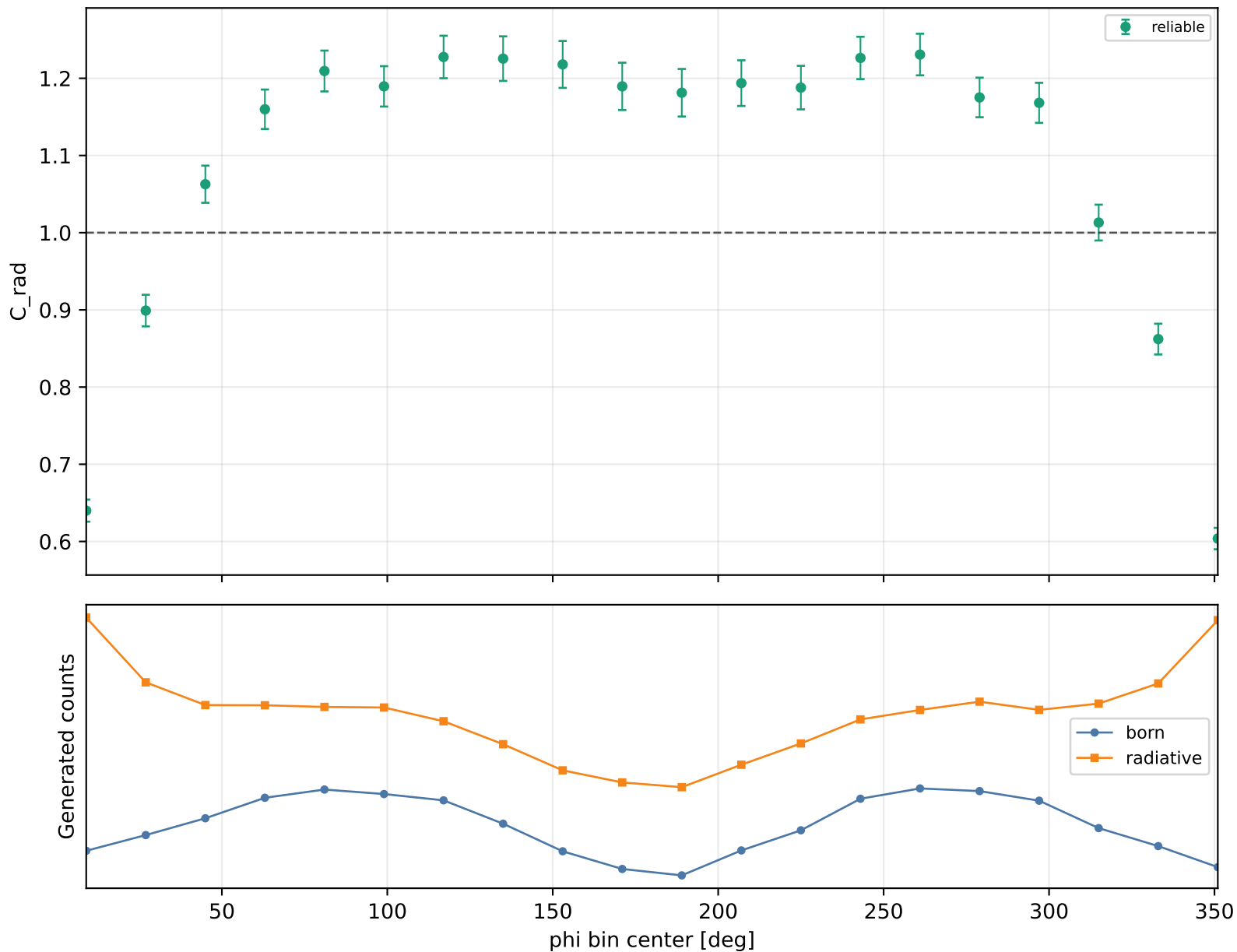
Radiative correction vs phi Q2 2-2.5, xB 0.3-0.38, -t 1.5-2
