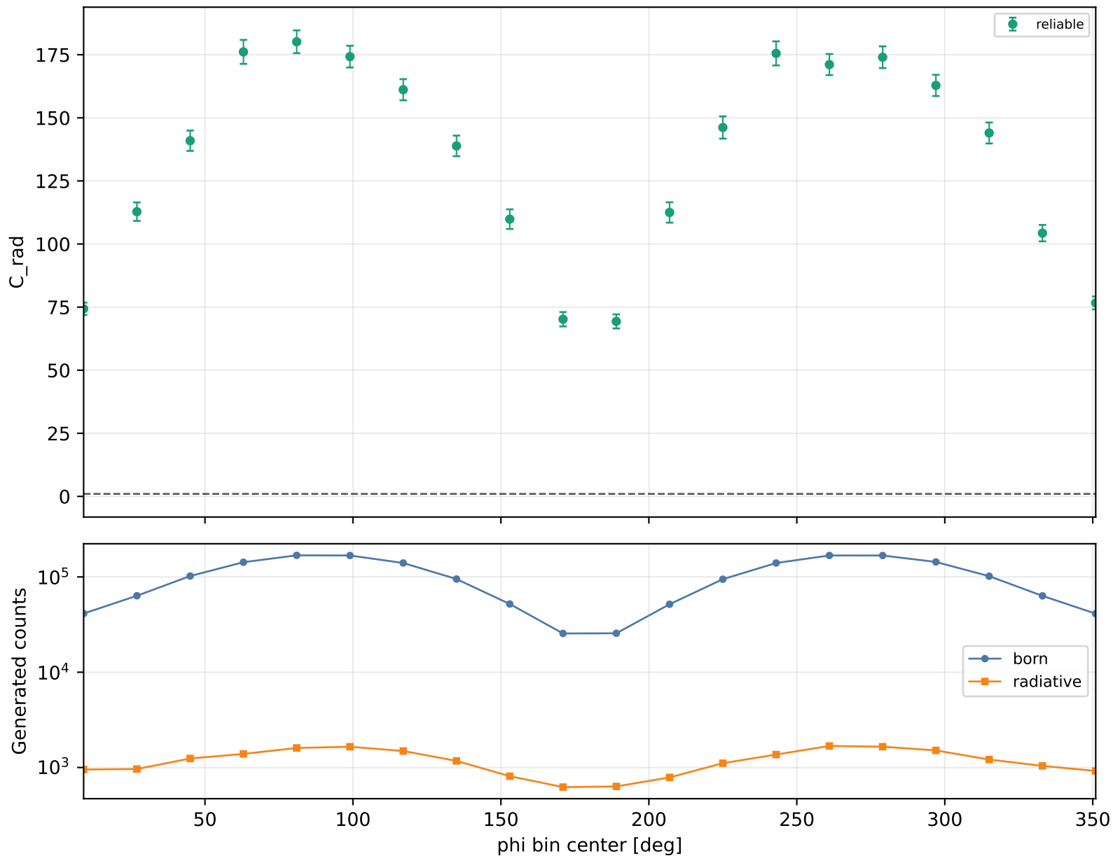
Radiative correction vs phi Q2 1-1.5, xB 0.38-0.48, -t 0.6-1
