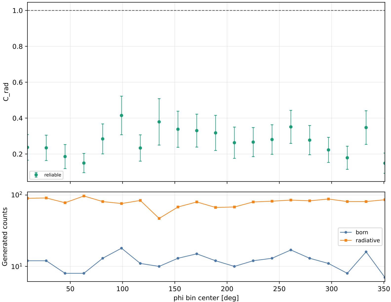
Radiative correction vs phi Q2 3-3.5, xB 0.25-0.3, -t 0.6-1
