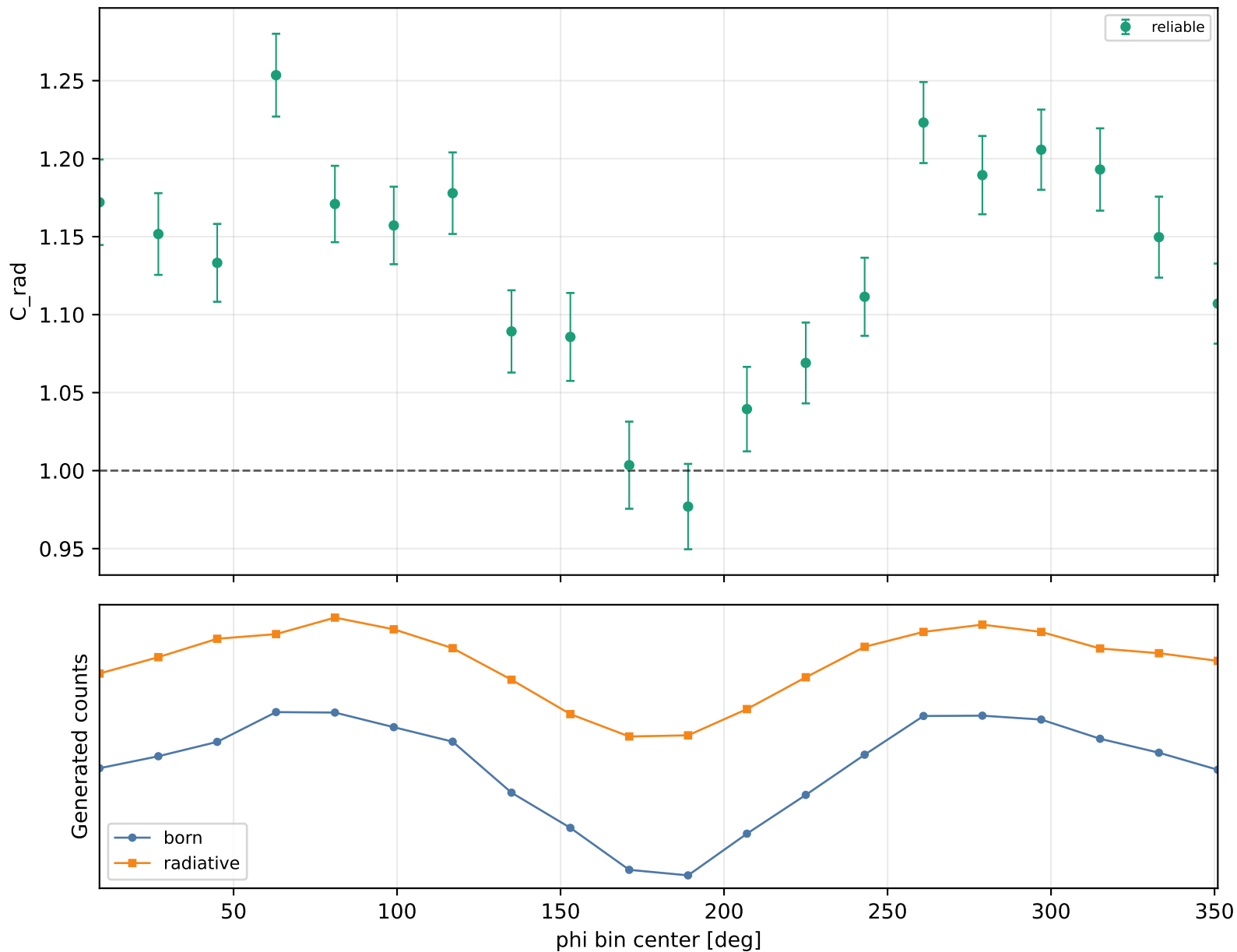
Radiative correction vs phi Q2 2-2.5, xB 0.25-0.3, -t 0.2-0.3
