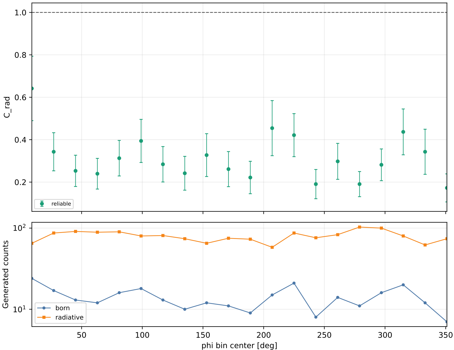
Radiative correction vs phi Q2 1-1.5, xB 0.05-0.1, -t 0.09-0.15
