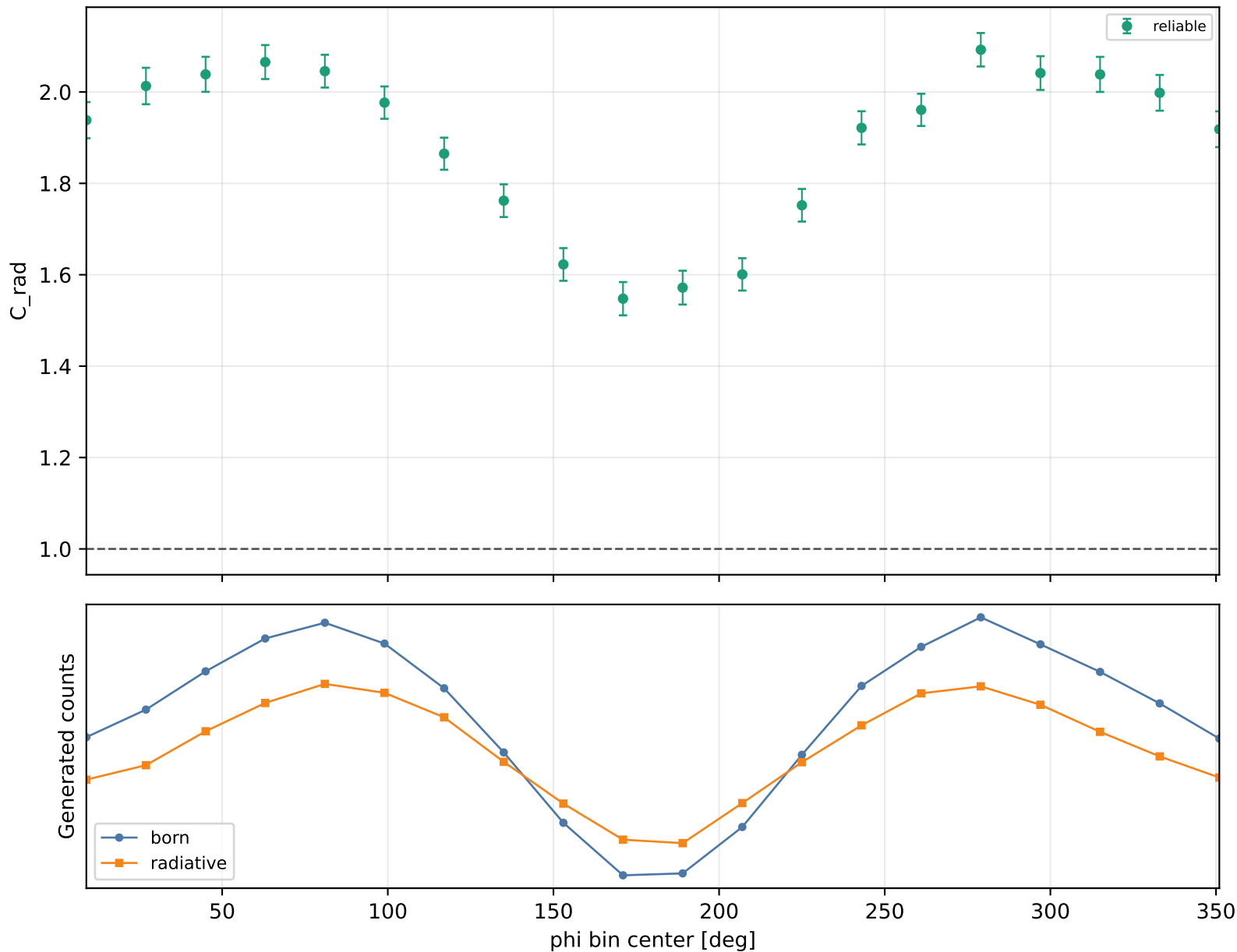
Radiative correction vs phi Q2 2.5-3, xB 0.48-0.58, -t 0.4-0.6
