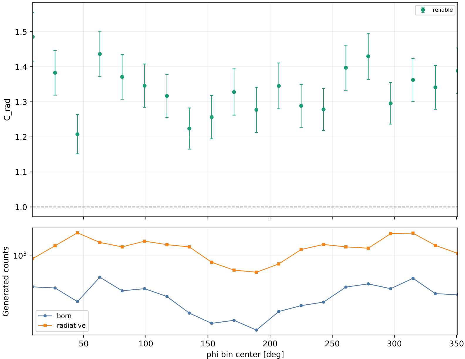
Radiative correction vs phi Q2 3-3.5, xB 0.38-0.48, -t 0.2-0.3
