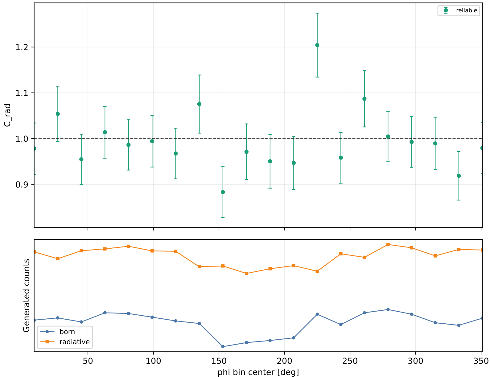
Radiative correction vs phi Q2 2.5-3, xB 0.25-0.3, -t 0.15-0.2
