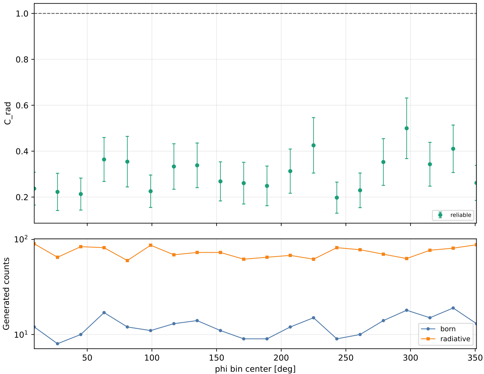
Radiative correction vs phi Q2 2-2.5, xB 0.15-0.2, -t 0.6-1
