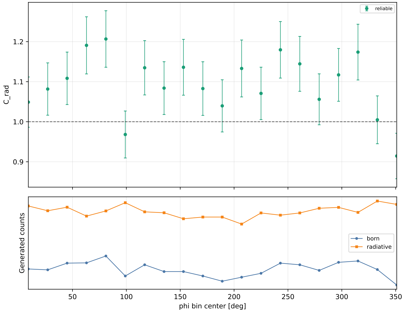
Radiative correction vs phi Q2 4-4.6, xB 0.38-0.48, -t 0.3-0.4
