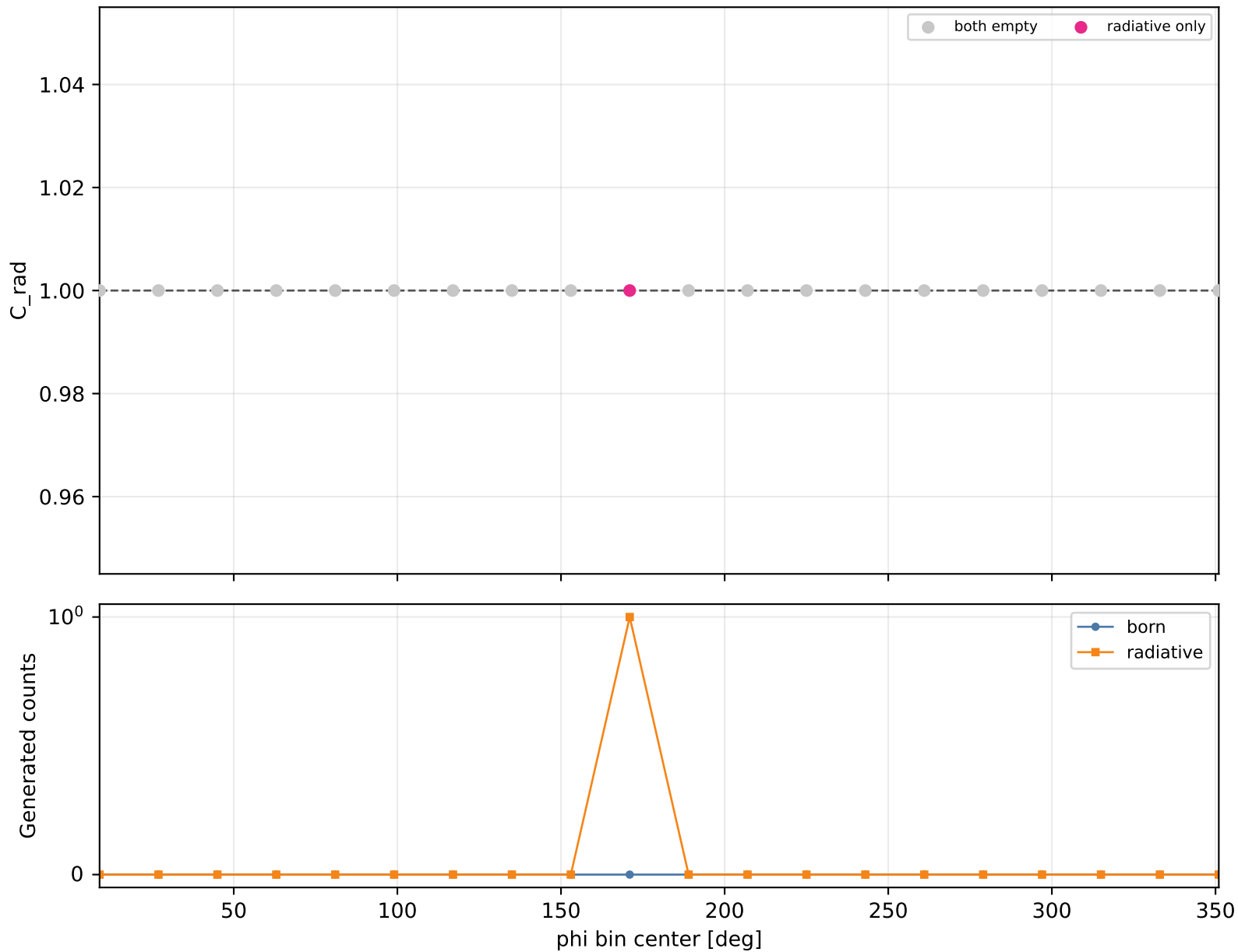
Radiative correction vs phi Q2 4.6-5.5, xB 0.38-0.48, -t 0.2-0.3
