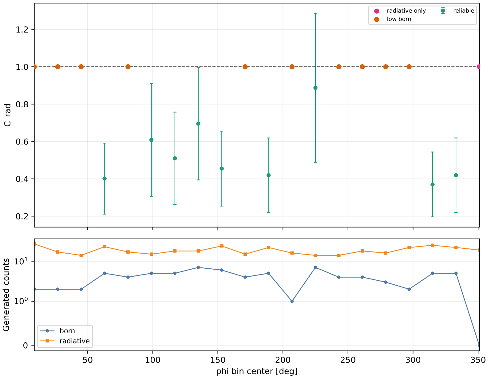
Radiative correction vs phi Q2 3-3.5, xB 0.25-0.3, -t 1.5-2
