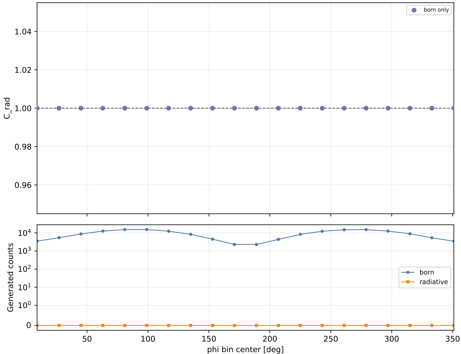
Radiative correction vs phi Q2 1-1.5, xB 0.48-0.58, -t 0.6-1
