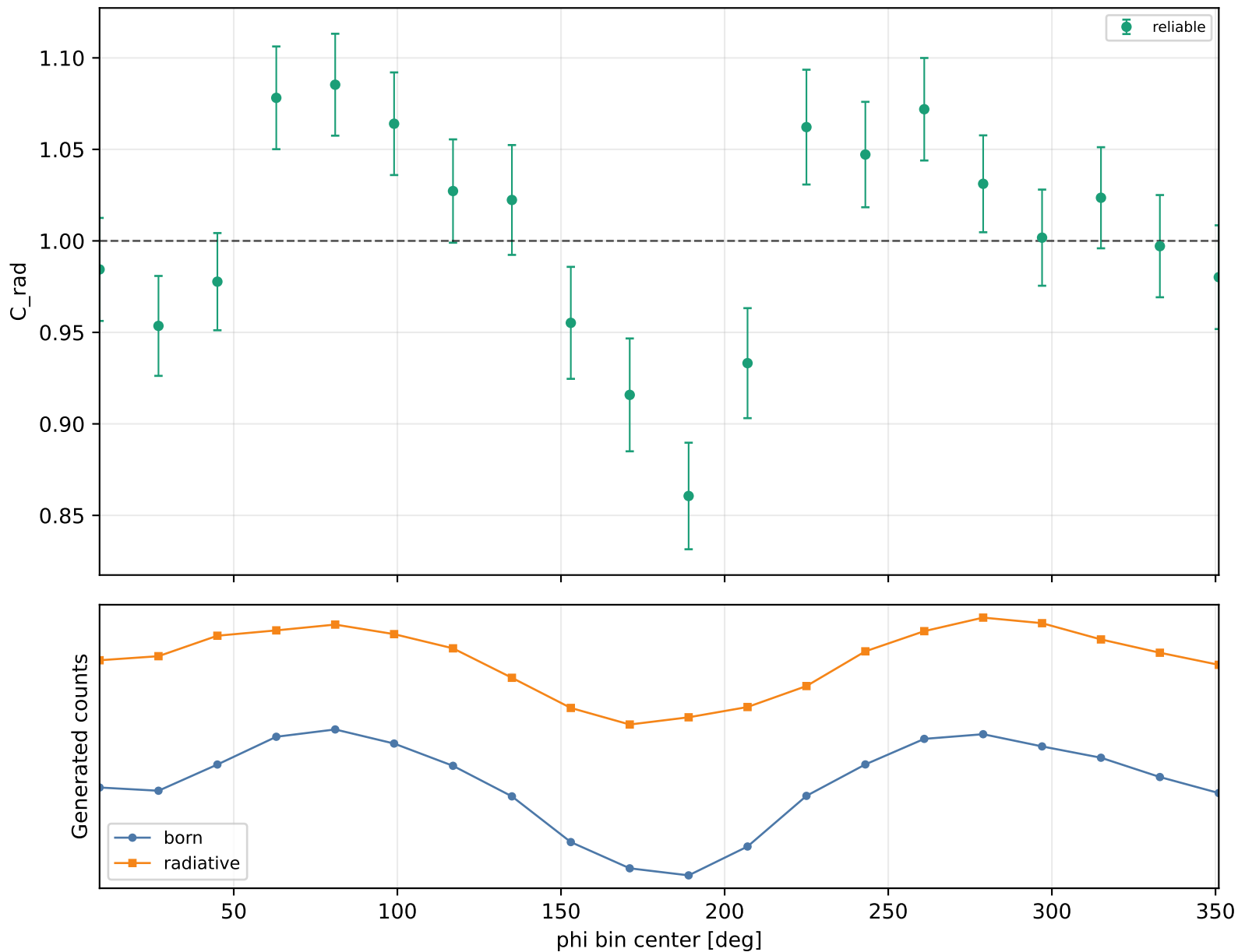
Radiative correction vs phi Q2 1.5-2, xB 0.15-0.2, -t 0.15-0.2
