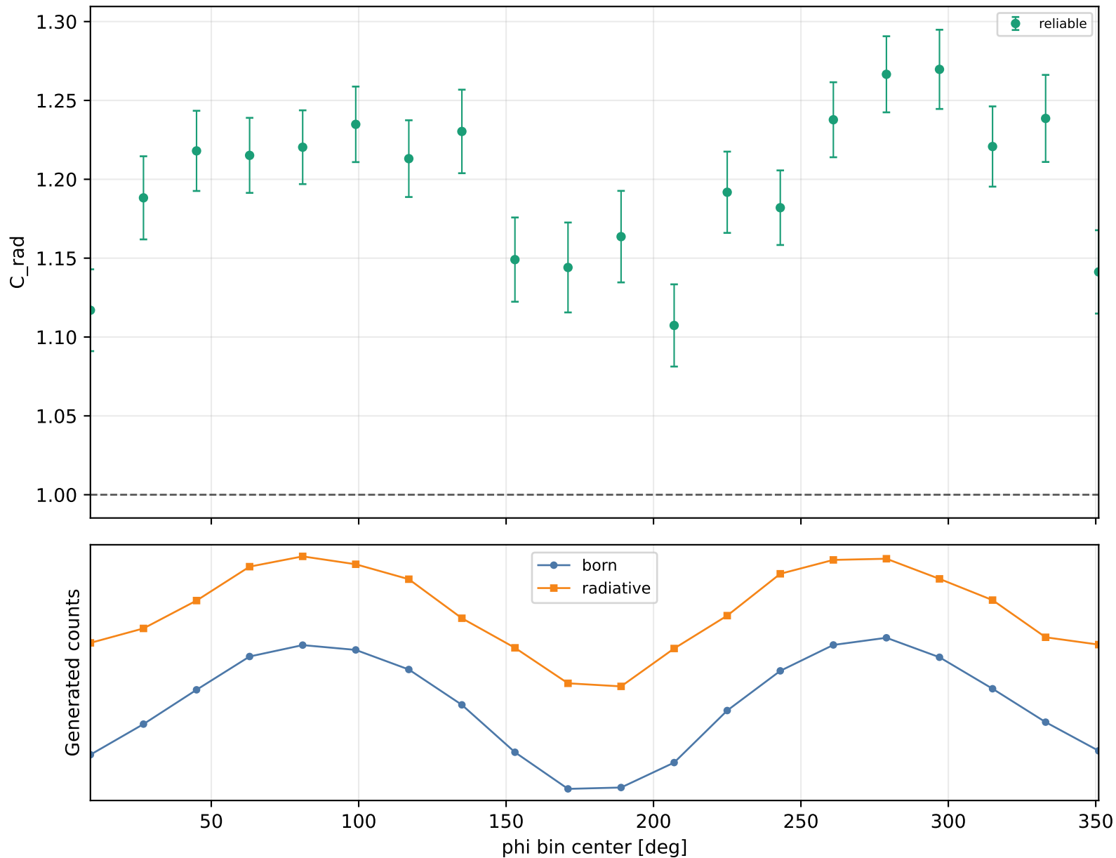
Radiative correction vs phi Q2 3.5-4, xB 0.48-0.58, -t 0.6-1
