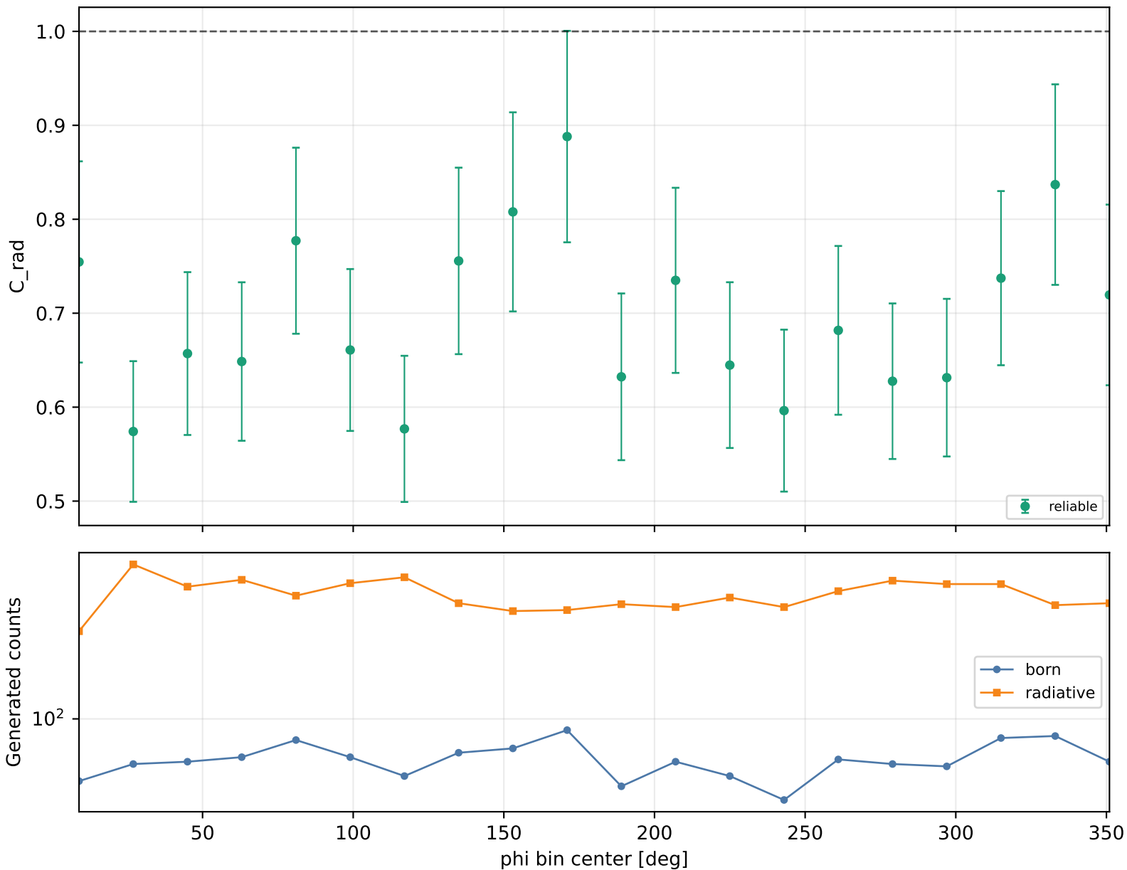
Radiative correction vs phi Q2 4.6-5.5, xB 0.38-0.48, -t 0.4-0.6
