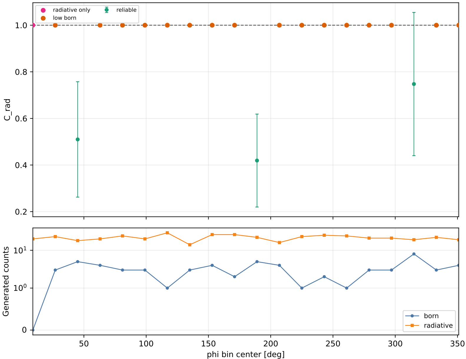
Radiative correction vs phi Q2 3-3.5, xB 0.25-0.3, -t 0.15-0.2
