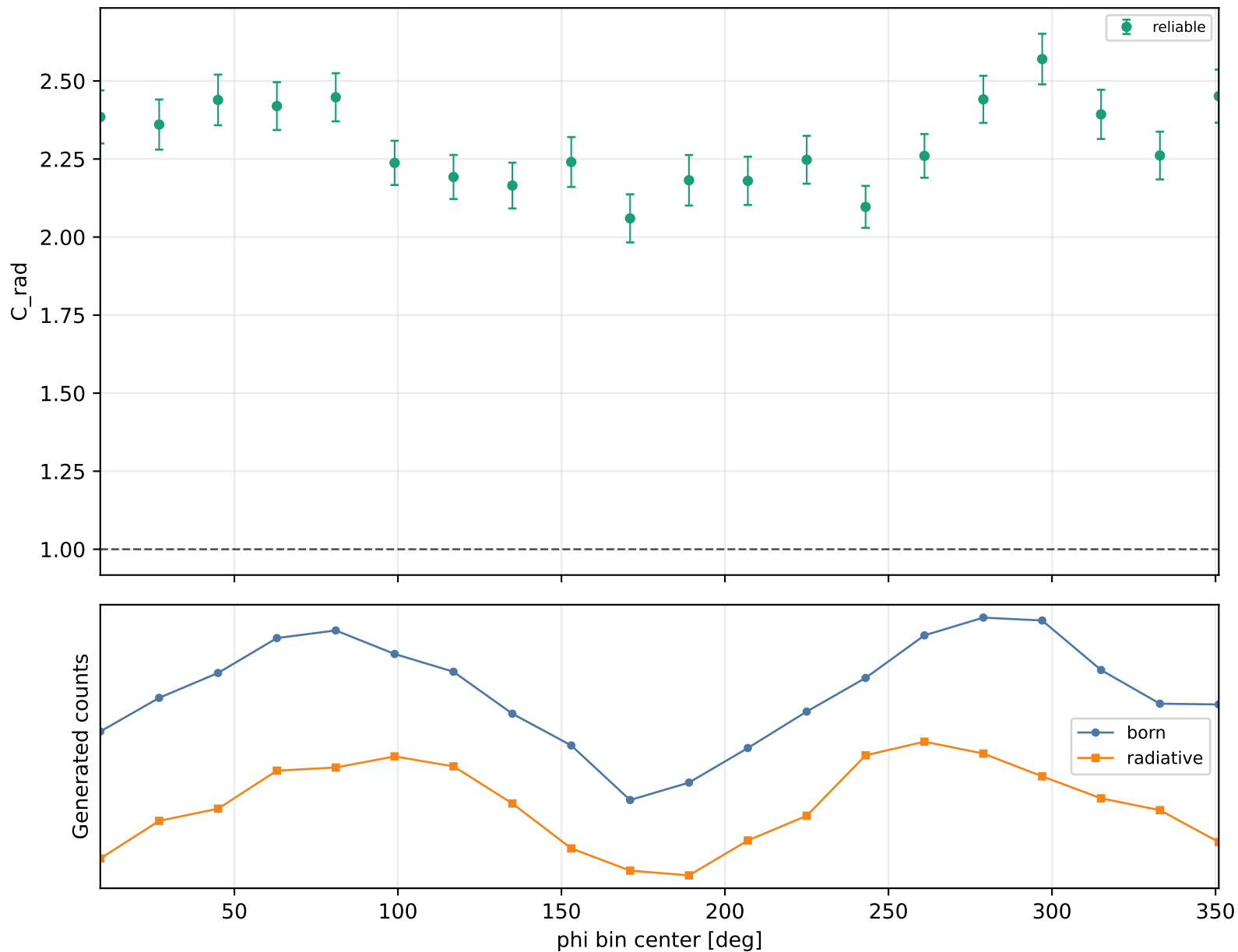
Radiative correction vs phi Q2 4-4.6, xB 0.58-0.7, -t 0.6-1
