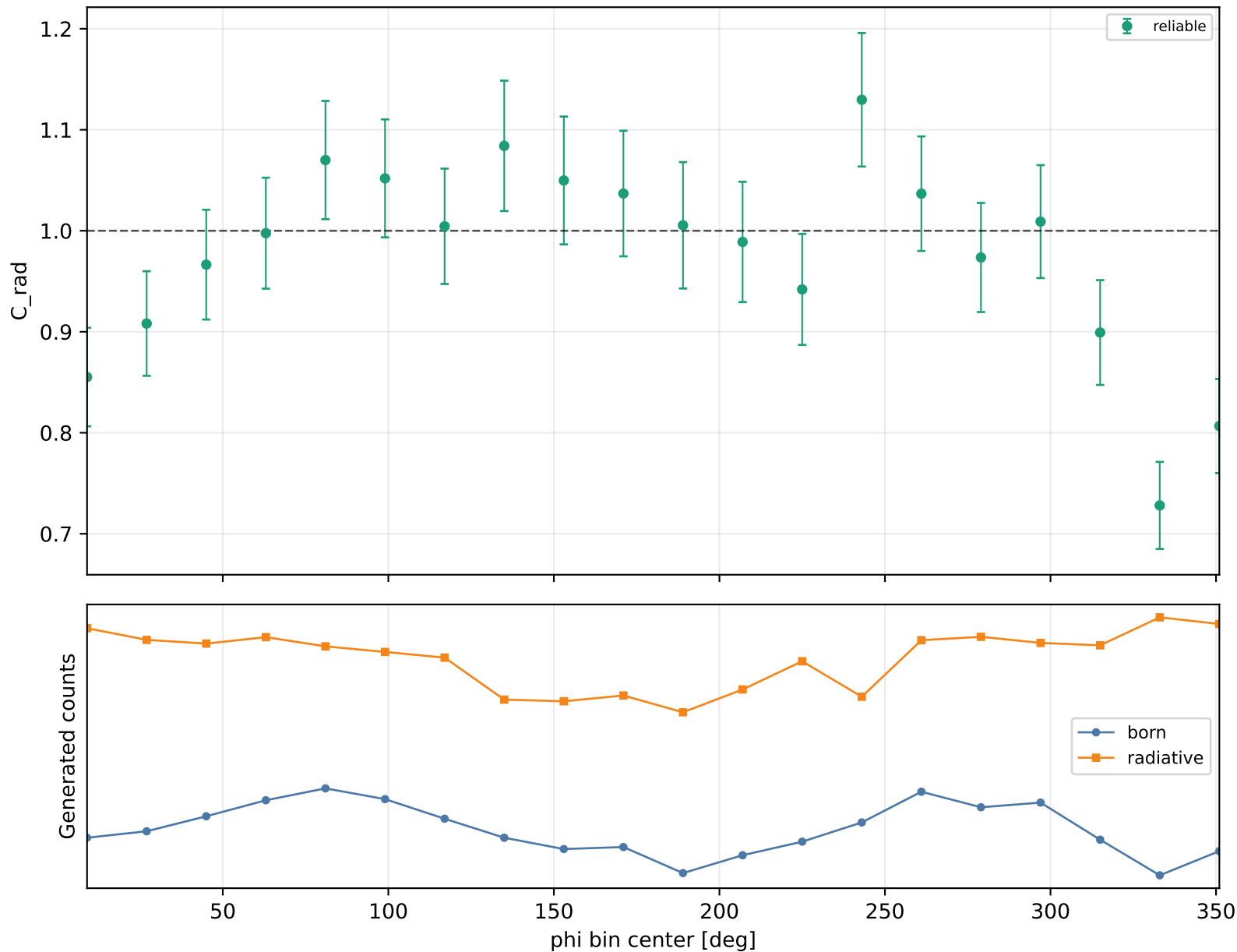
Radiative correction vs phi Q2 4-4.6, xB 0.38-0.48, -t 1.5-2
