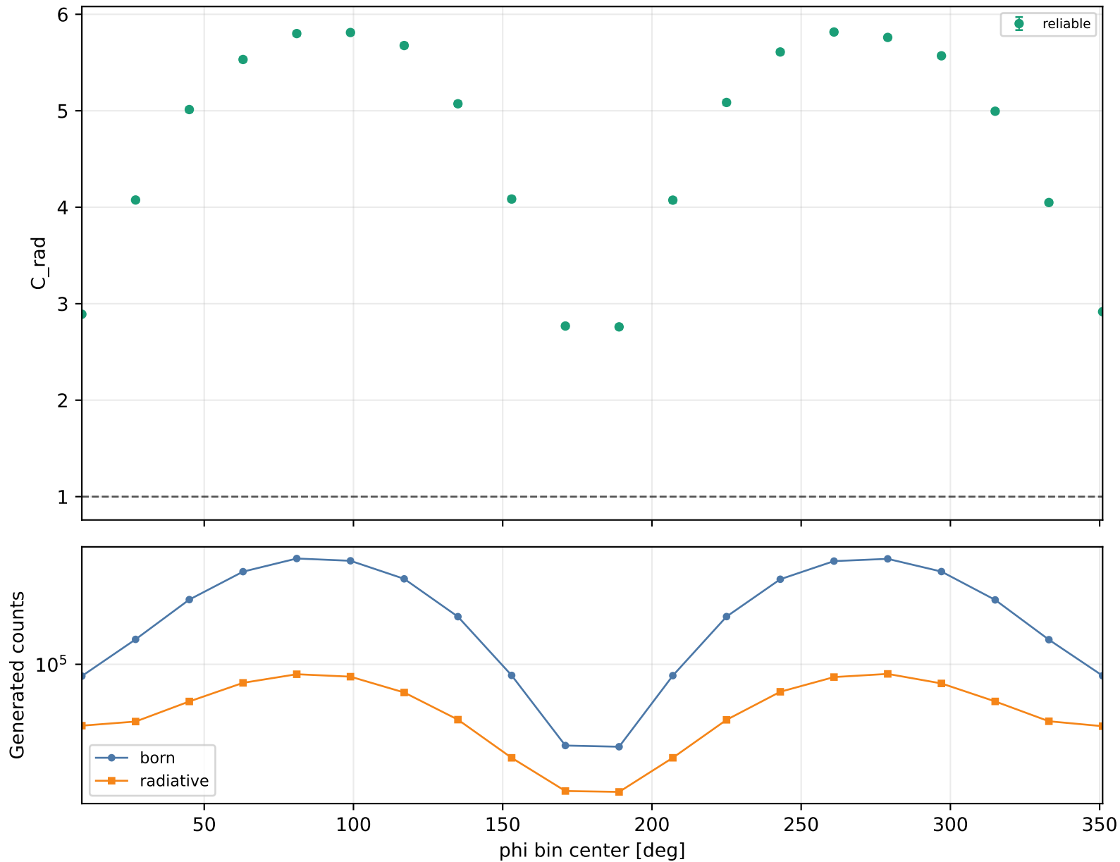
Radiative correction vs phi Q2 1-1.5, xB 0.3-0.38, -t 0.6-1
