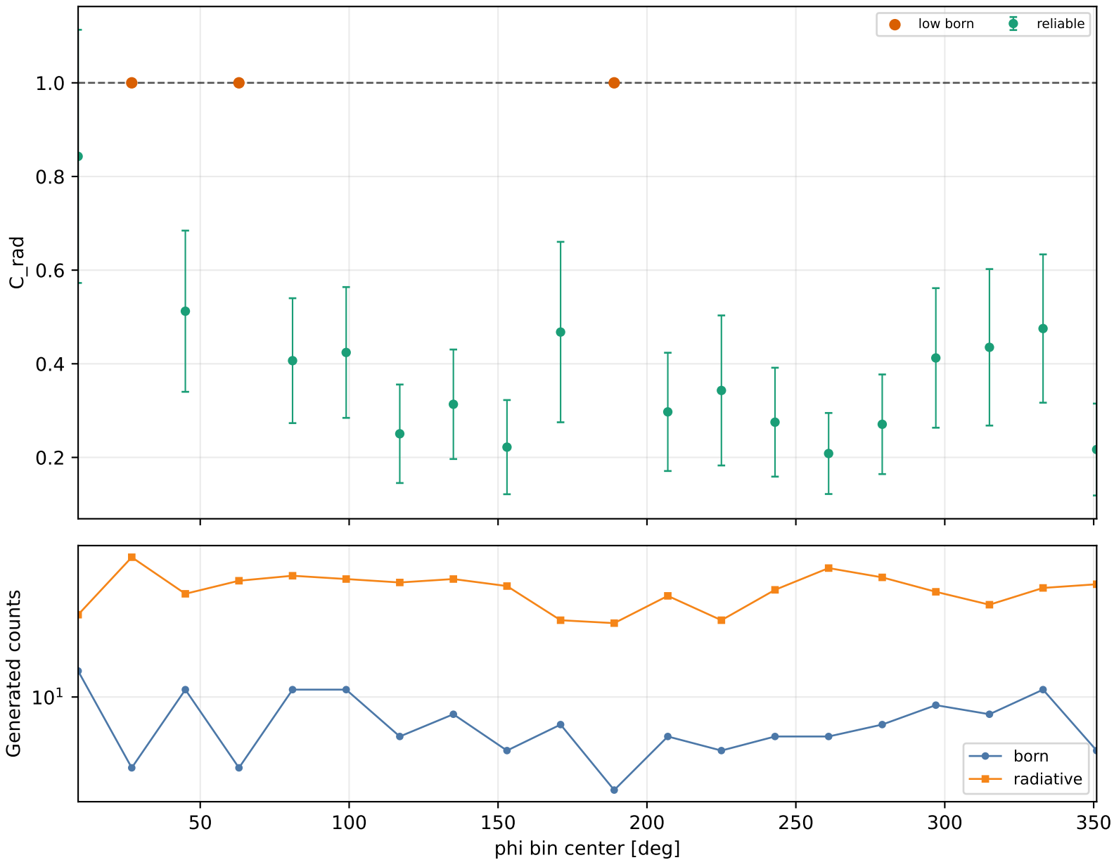
Radiative correction vs phi Q2 1.5-2, xB 0.1-0.15, -t 0.15-0.2
