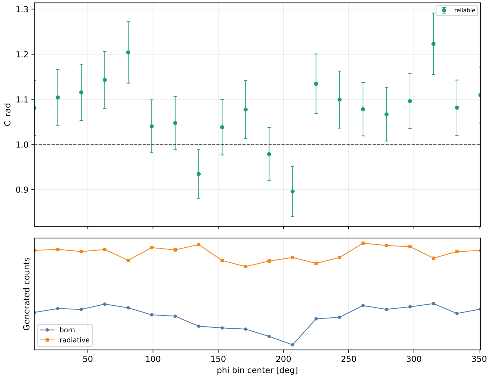
Radiative correction vs phi Q2 2.5-3, xB 0.25-0.3, -t 0.09-0.15
