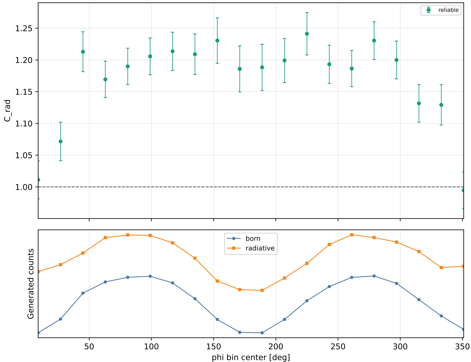
Radiative correction vs phi Q2 4-4.6, xB 0.48-0.58, -t 1-1.5
