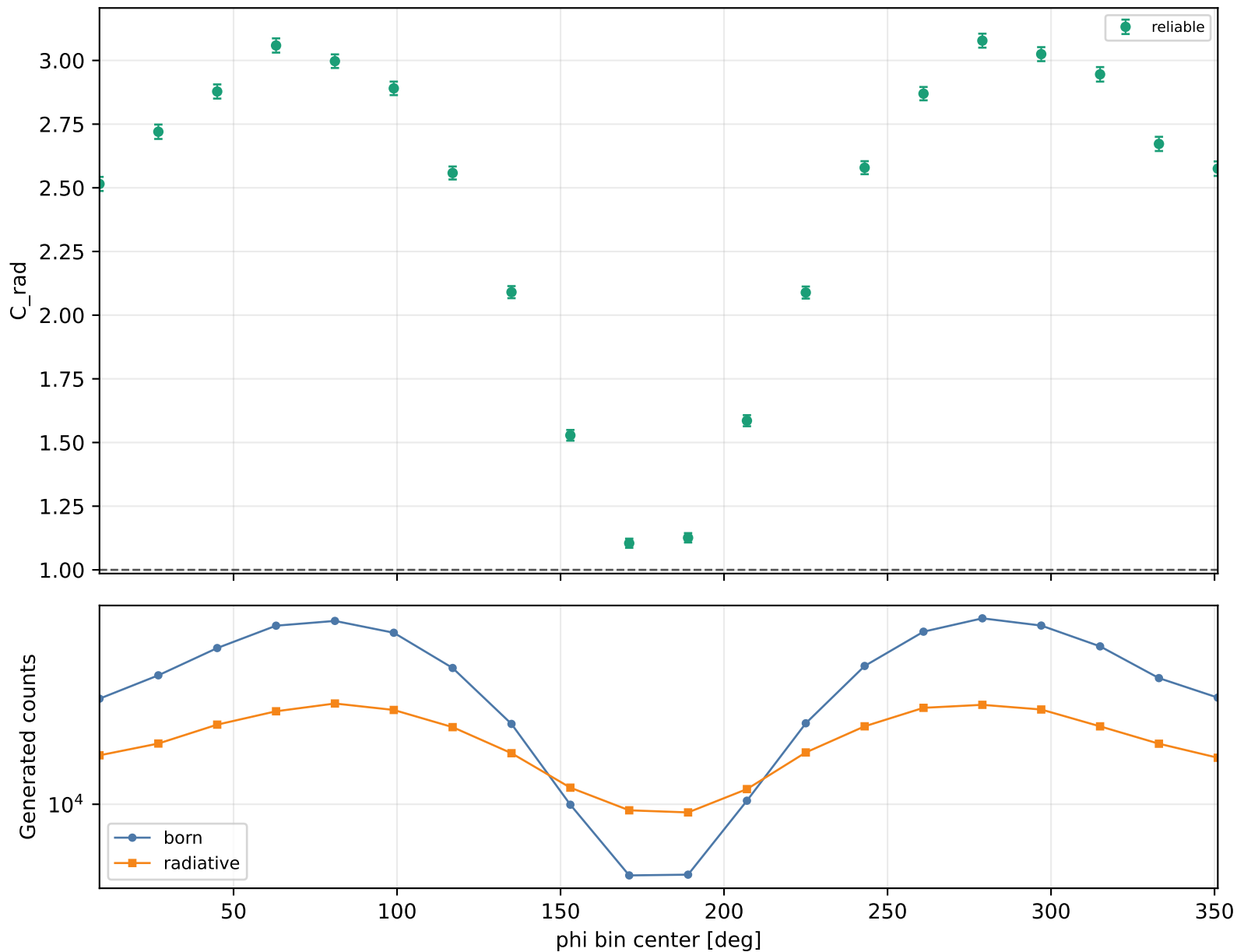
Radiative correction vs phi Q2 1.5-2, xB 0.38-0.48, -t 0.3-0.4
