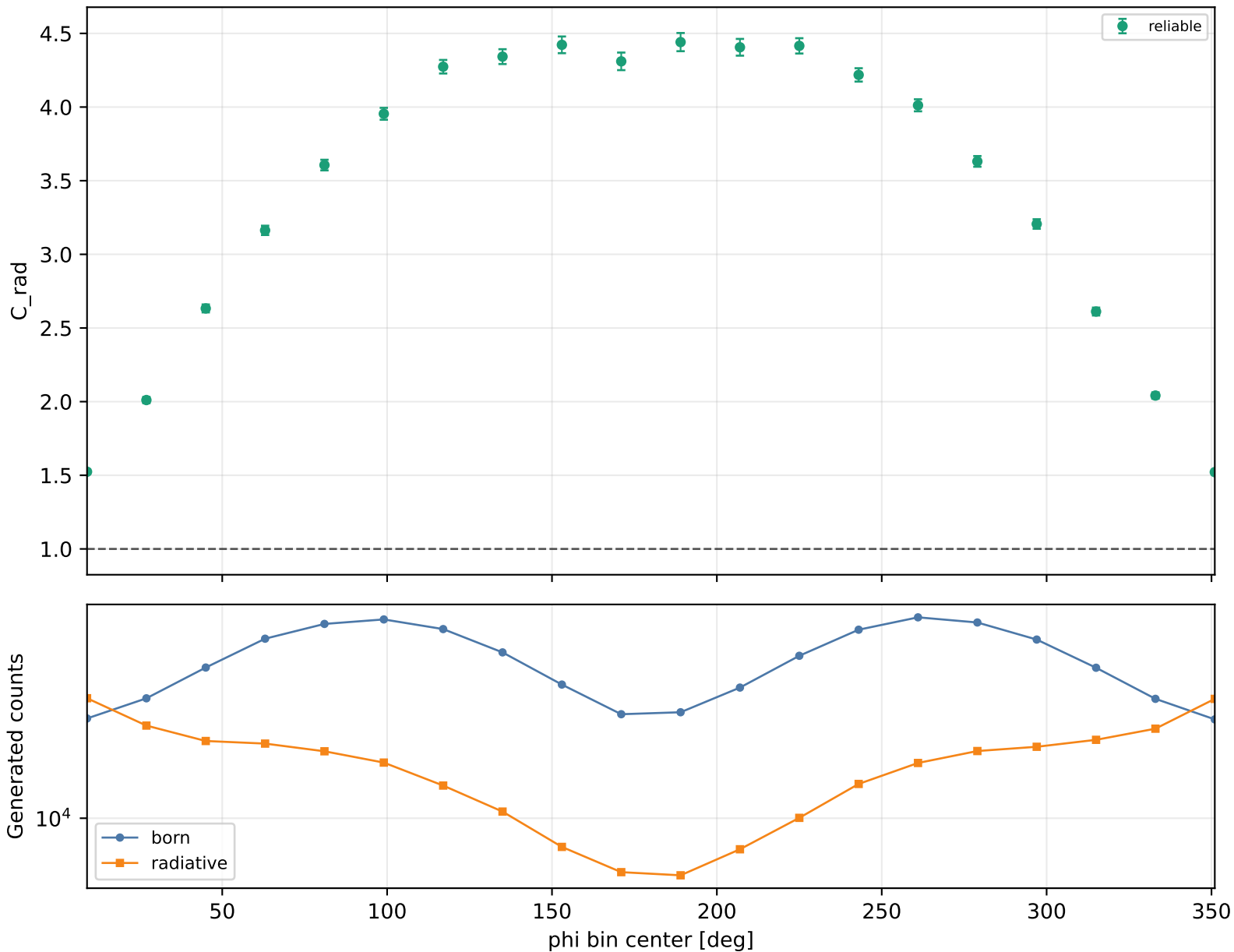
Radiative correction vs phi Q2 1-1.5, xB 0.3-0.38, -t 1.5-2
