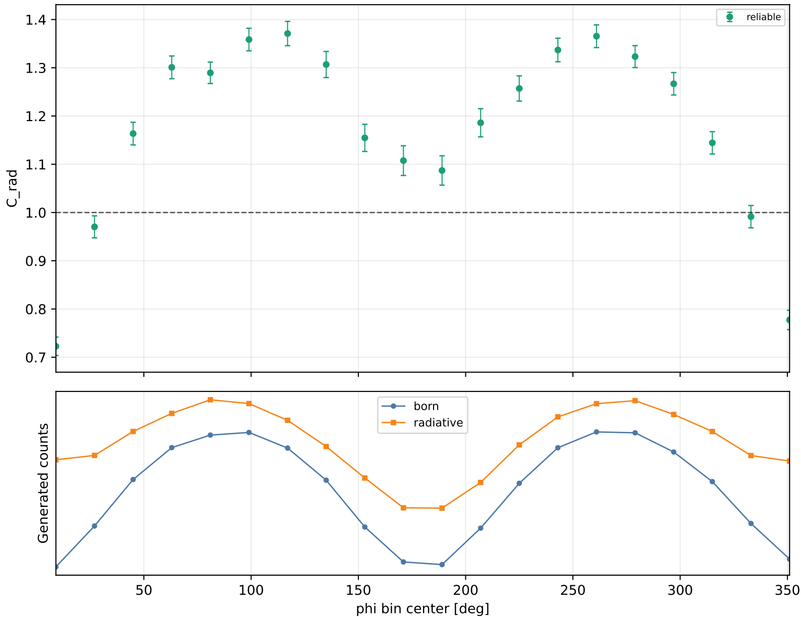
Radiative correction vs phi Q2 3-3.5, xB 0.48-0.58, -t 1.5-2
