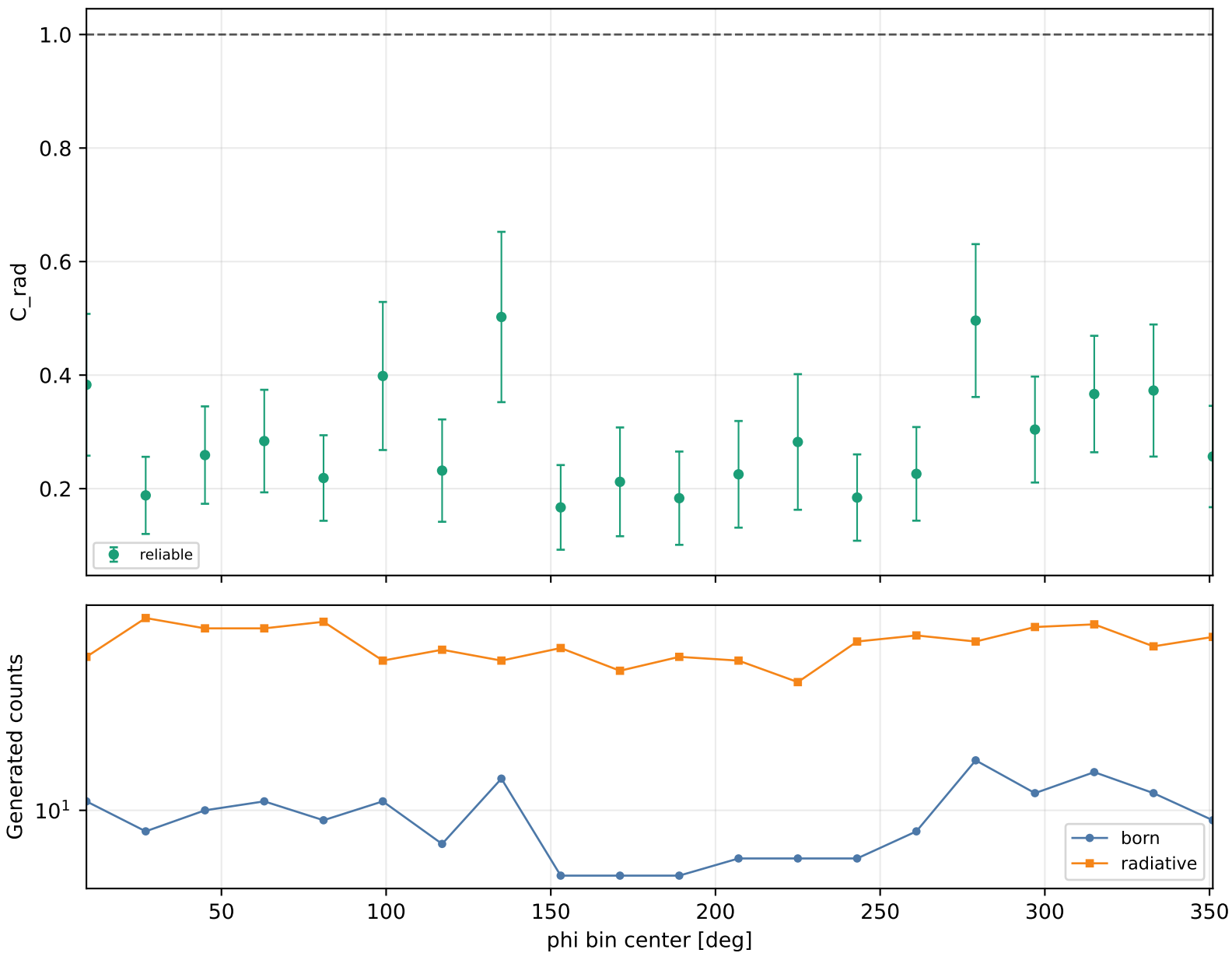
Radiative correction vs phi Q2 1.5-2, xB 0.1-0.15, -t 0.3-0.4
