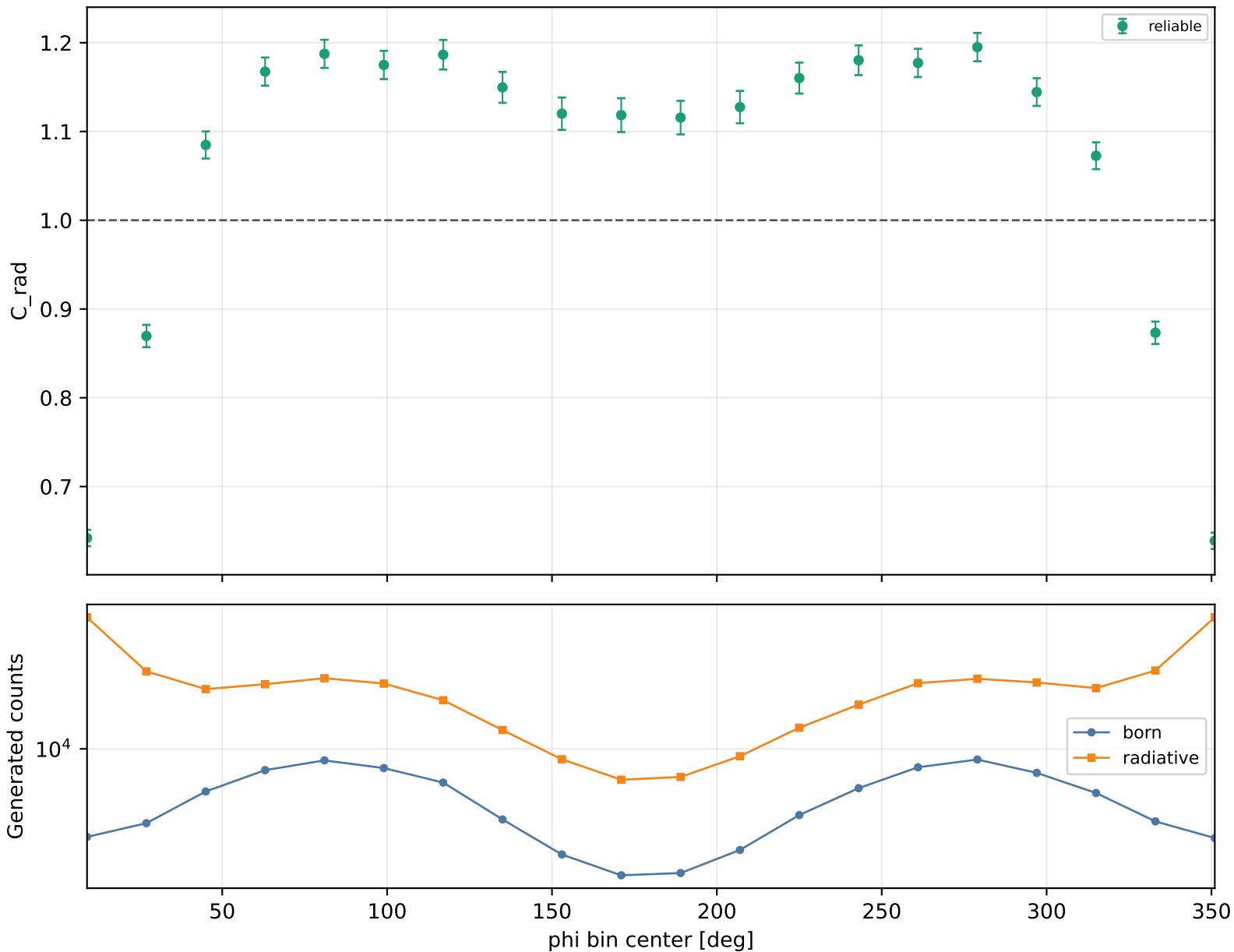
Radiative correction vs phi Q2 1.5-2, xB 0.25-0.3, -t 1-1.5
