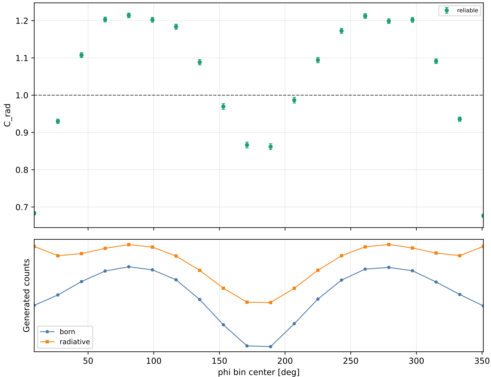
Radiative correction vs phi Q2 1-1.5, xB 0.2-0.25, -t 0.6-1
