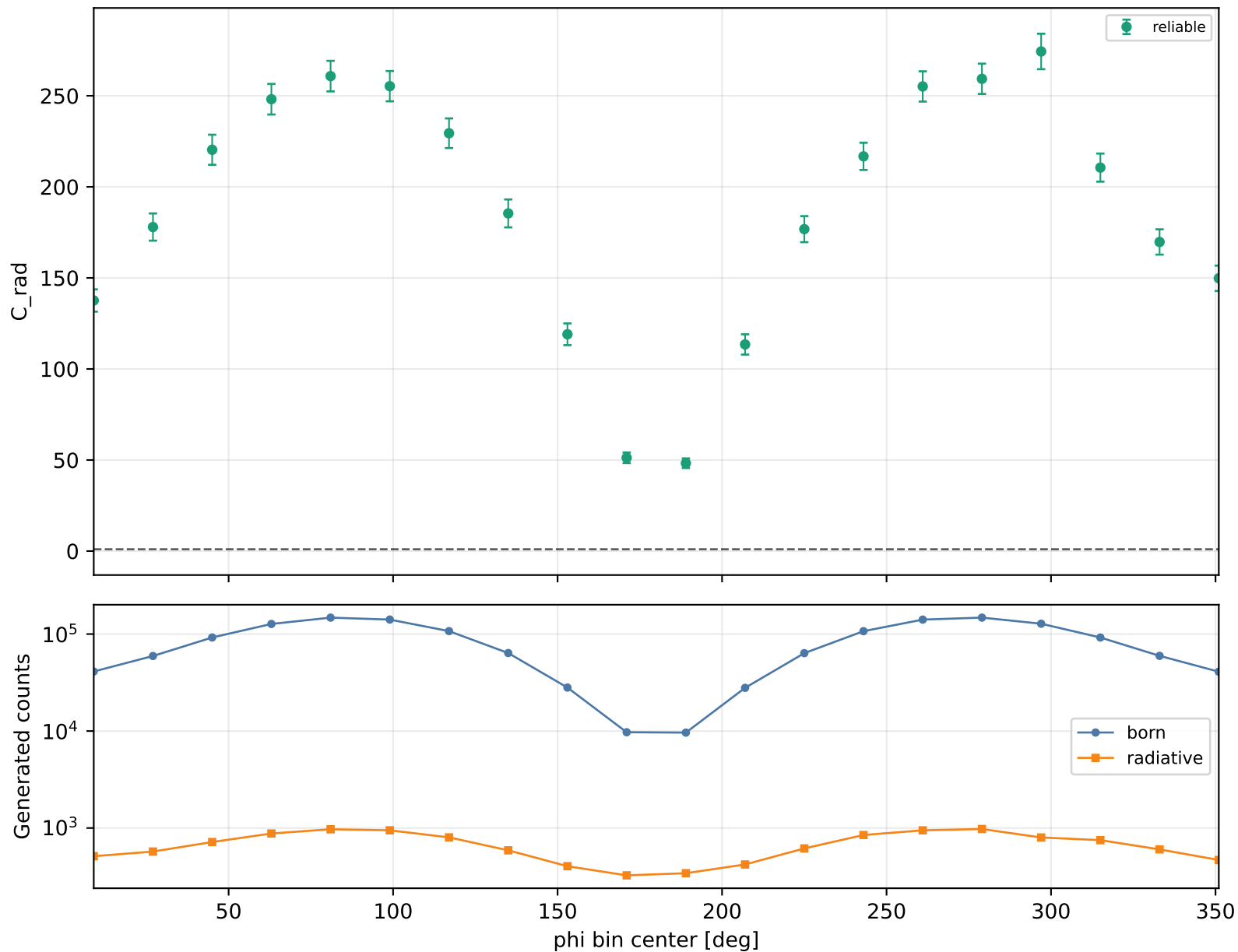
Radiative correction vs phi Q2 1-1.5, xB 0.38-0.48, -t 0.4-0.6
