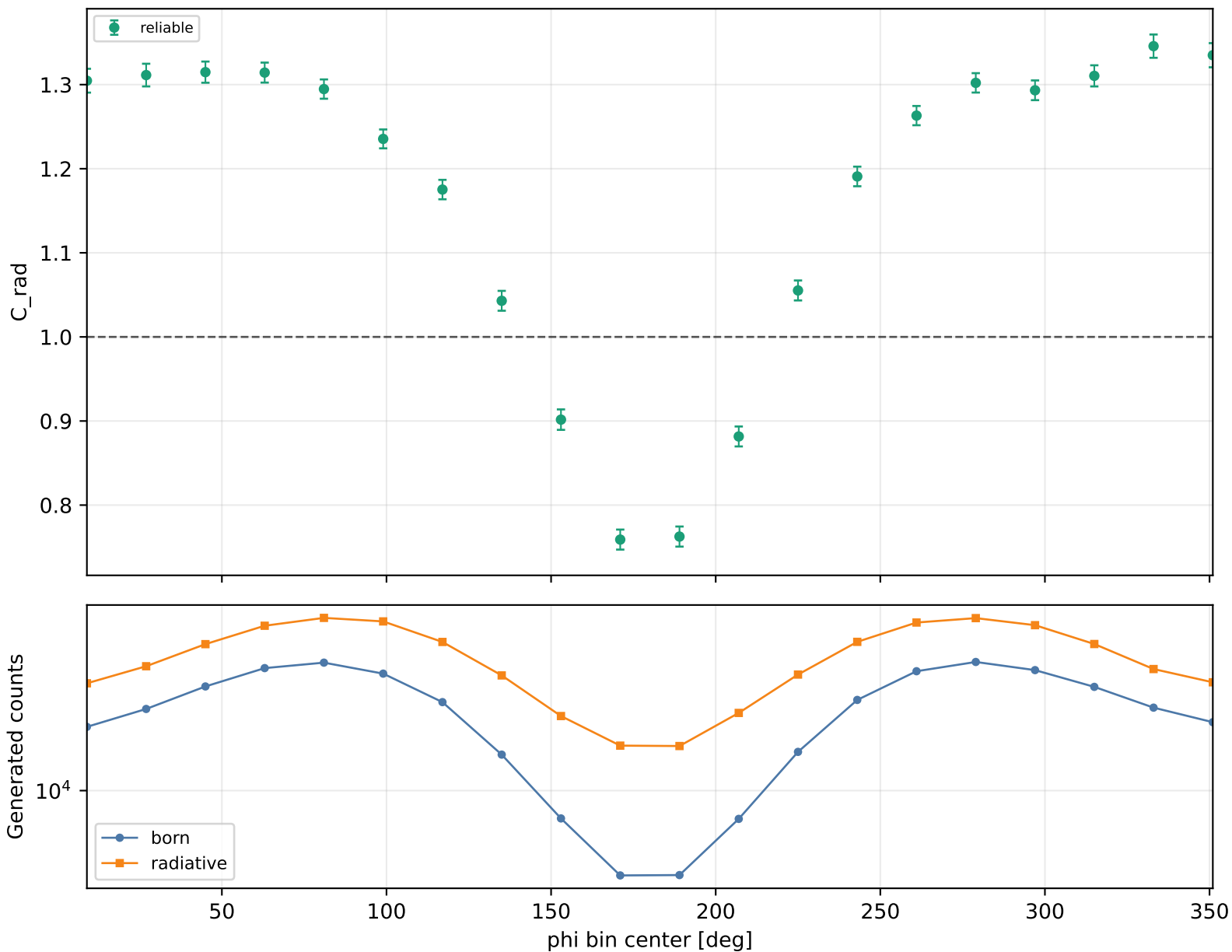
Radiative correction vs phi Q2 1.5-2, xB 0.3-0.38, -t 0.2-0.3
