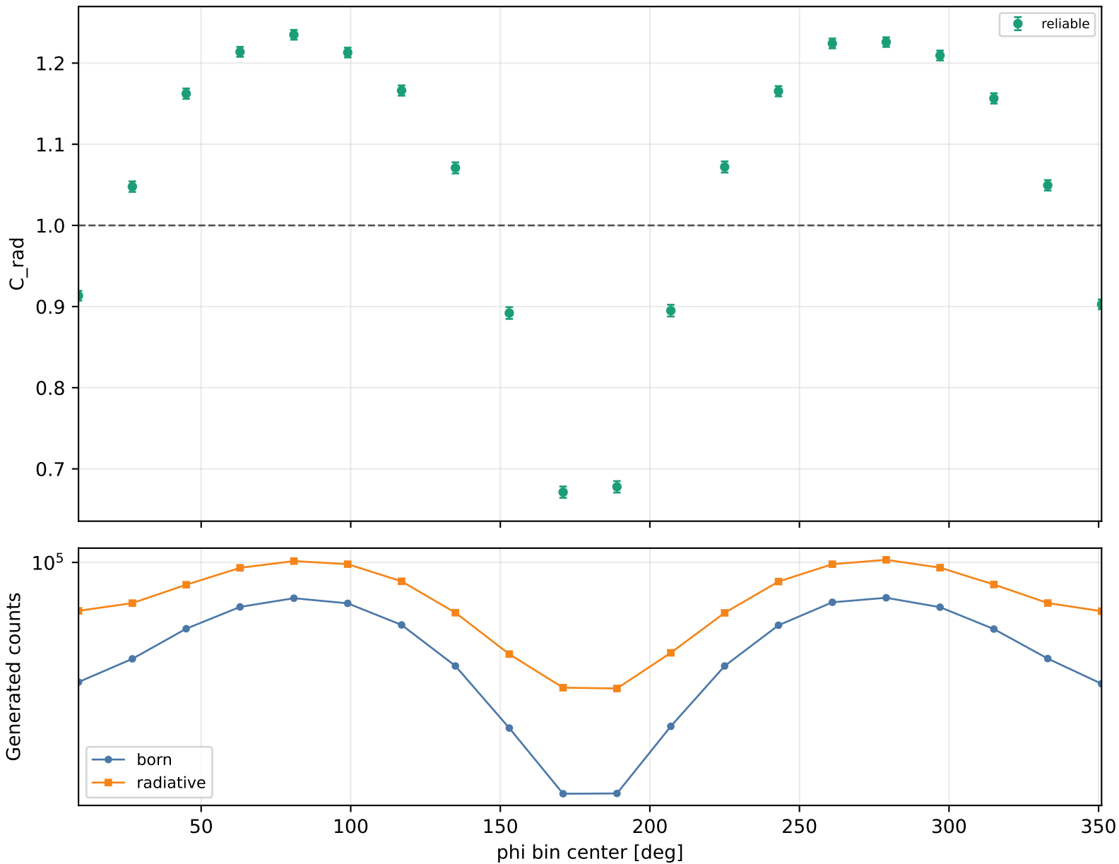
Radiative correction vs phi Q2 1-1.5, xB 0.2-0.25, -t 0.4-0.6
