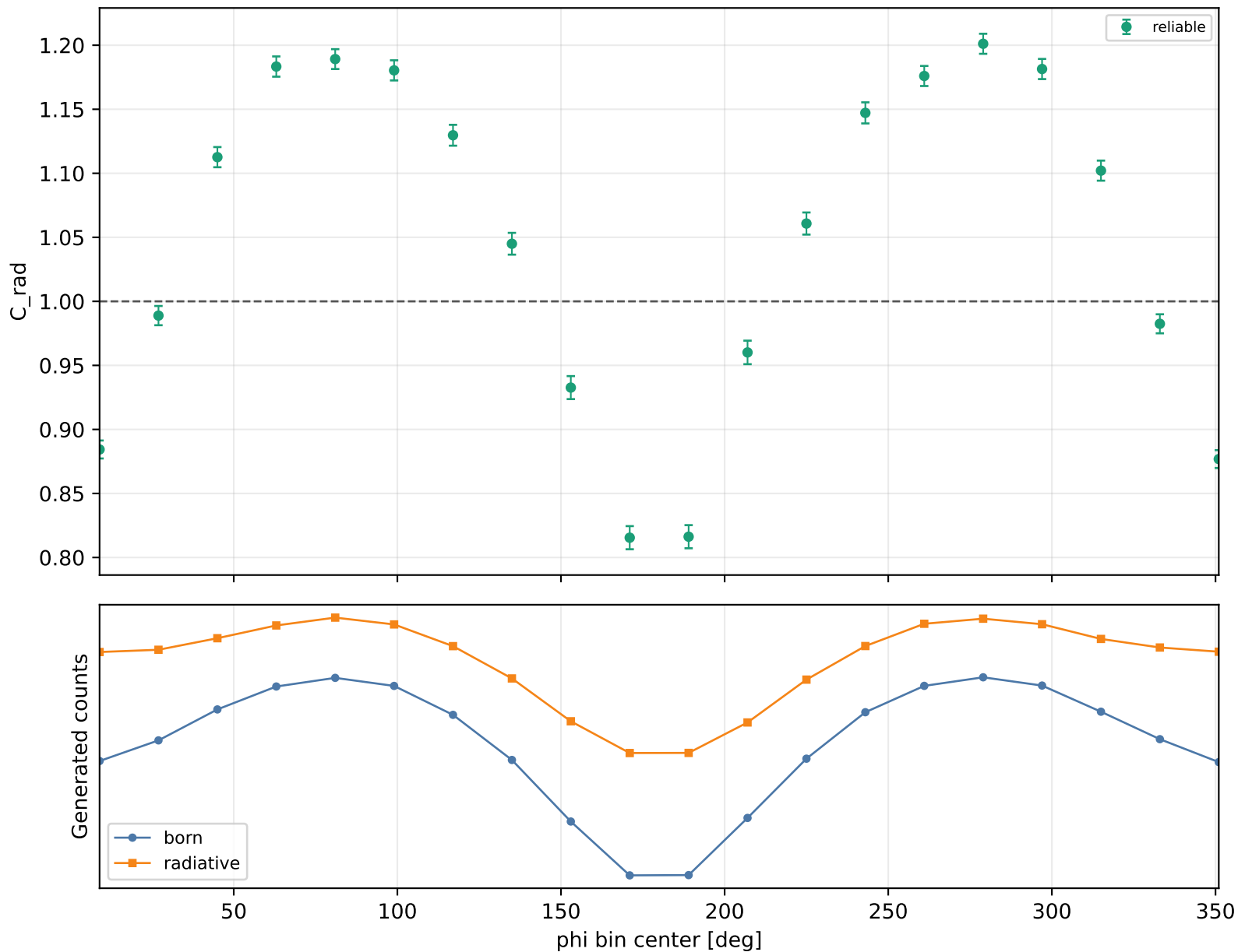
Radiative correction vs phi Q2 1-1.5, xB 0.15-0.2, -t 0.4-0.6
