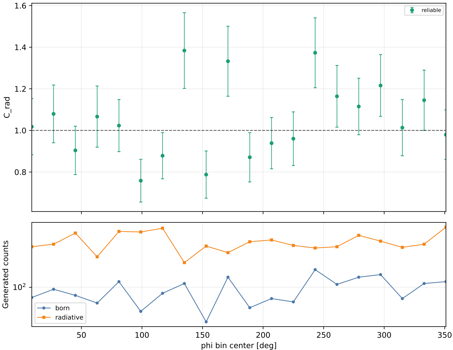
Radiative correction vs phi Q2 4-4.6, xB 0.38-0.48, -t 0.2-0.3
