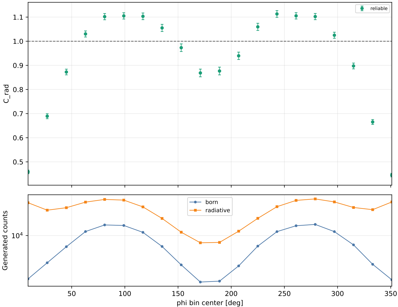
Radiative correction vs phi Q2 2-2.5, xB 0.38-0.48, -t 1.5-2
