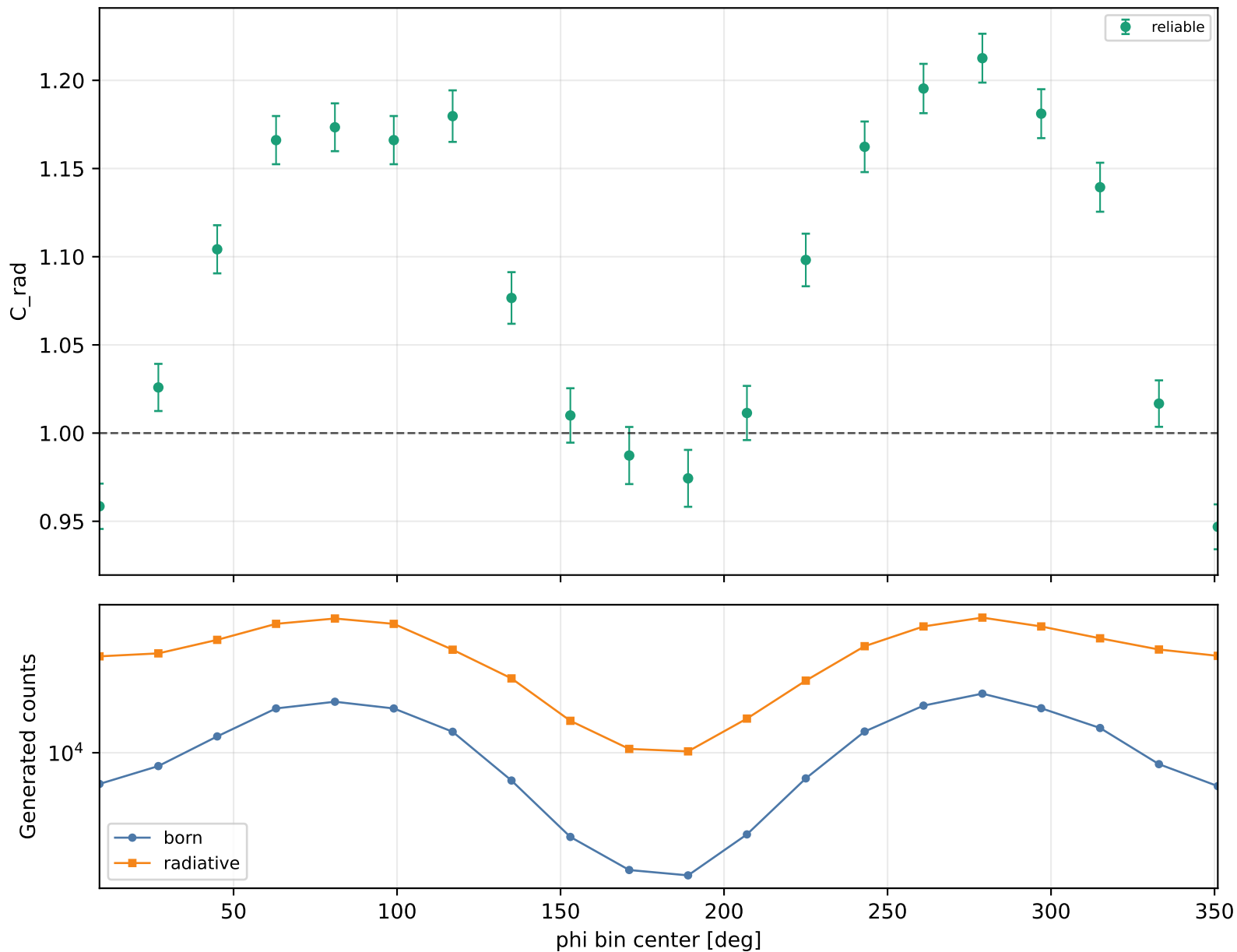
Radiative correction vs phi Q2 1.5-2, xB 0.2-0.25, -t 0.4-0.6
