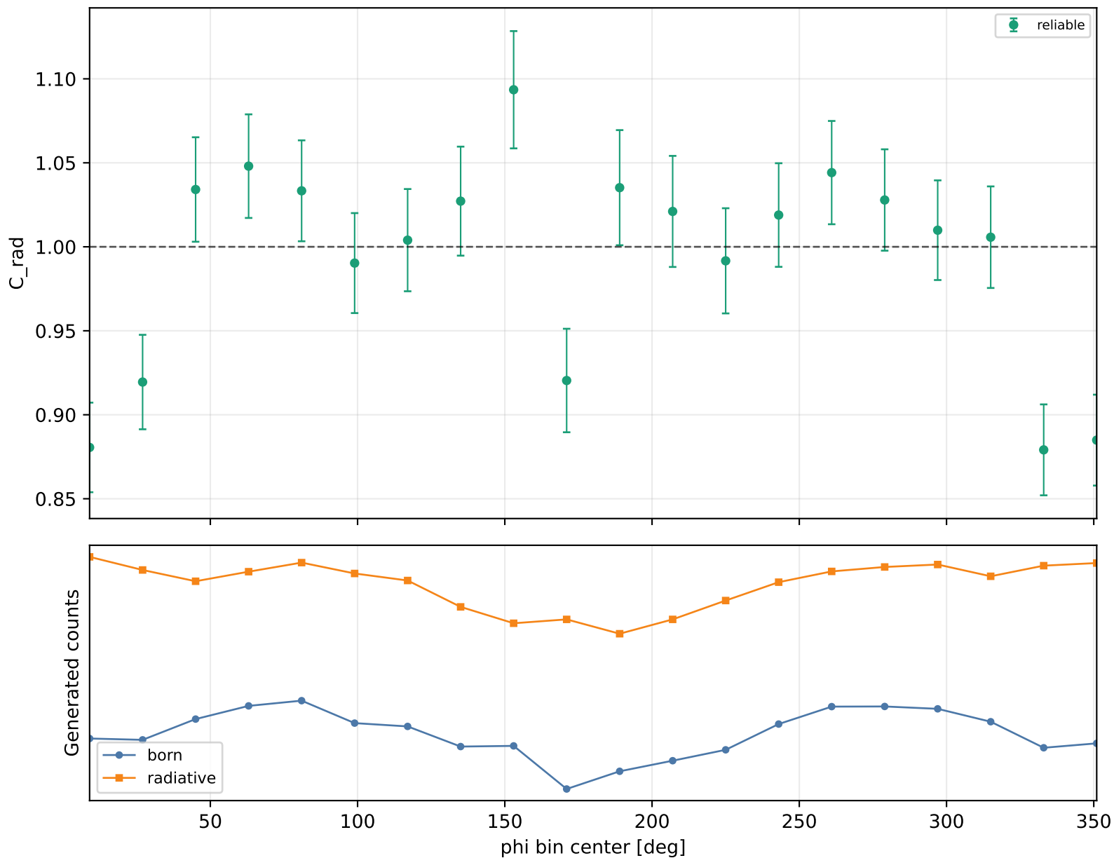
Radiative correction vs phi Q2 2.5-3, xB 0.25-0.3, -t 0.6-1
