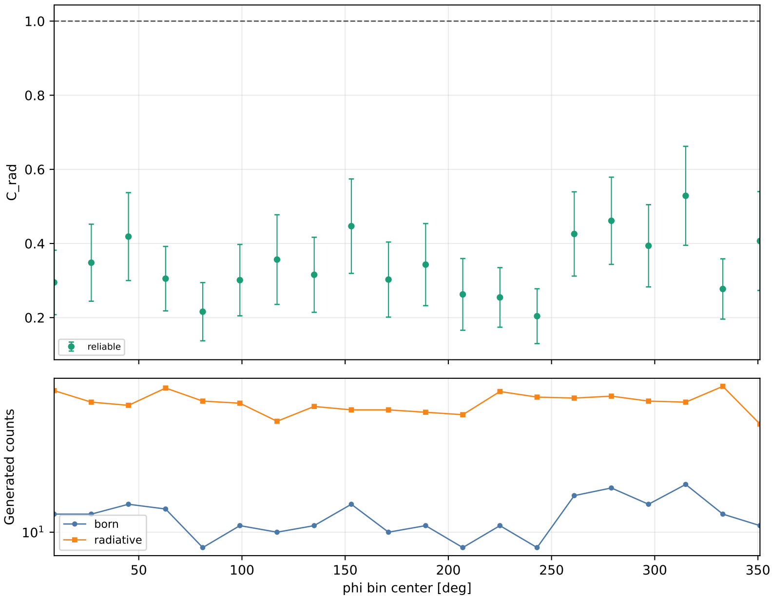
Radiative correction vs phi Q2 2.5-3, xB 0.2-0.25, -t 0.4-0.6
