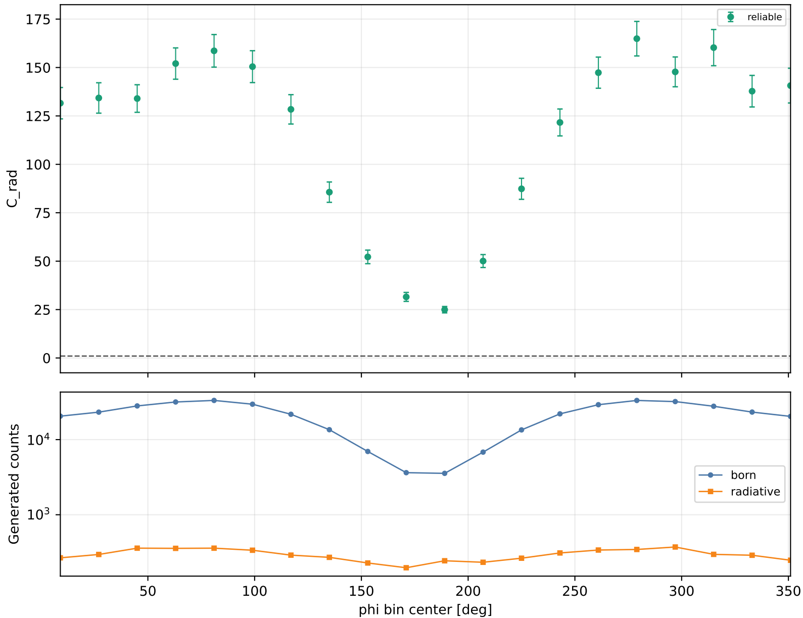
Radiative correction vs phi Q2 1-1.5, xB 0.38-0.48, -t 0.2-0.3
