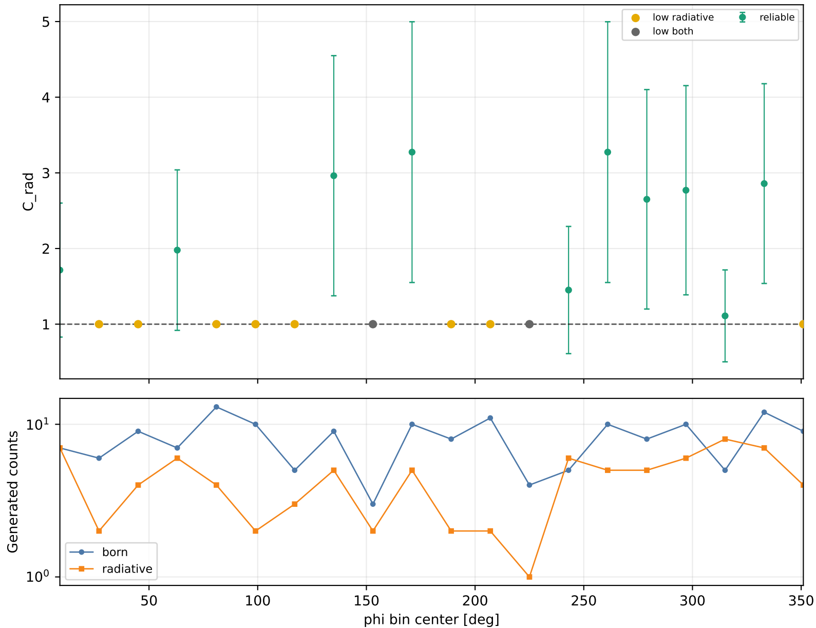
Radiative correction vs phi Q2 3-3.5, xB 0.38-0.48, -t 0.15-0.2
