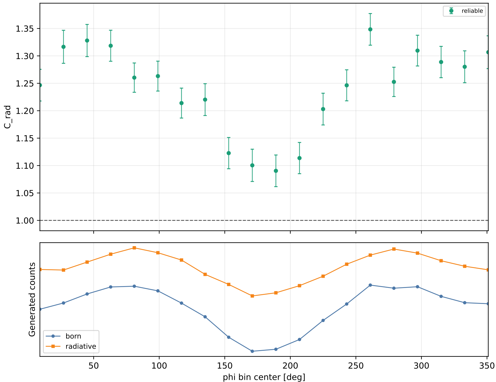
Radiative correction vs phi Q2 2.5-3, xB 0.38-0.48, -t 0.3-0.4
