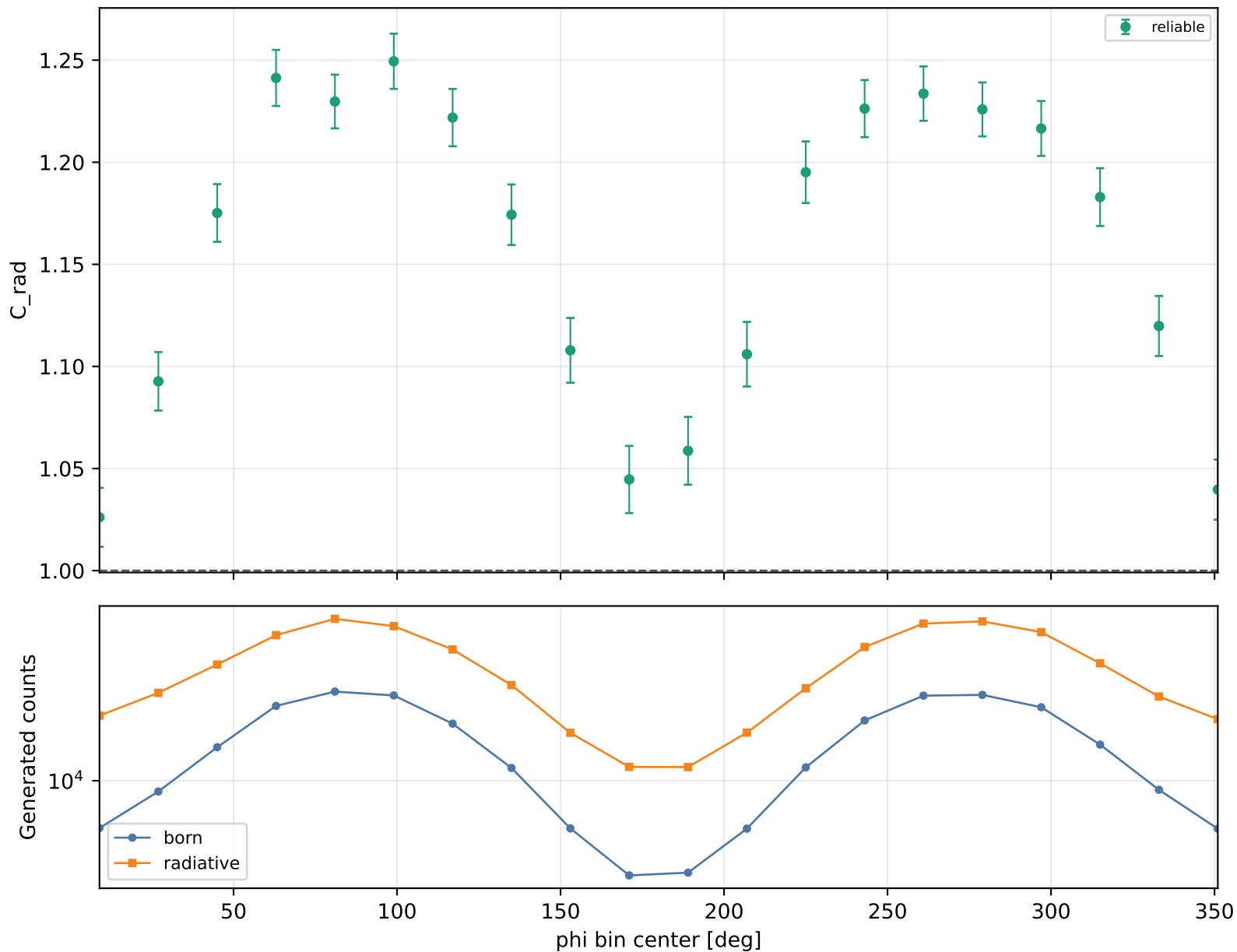
Radiative correction vs phi Q2 2.5-3, xB 0.38-0.48, -t 0.6-1
