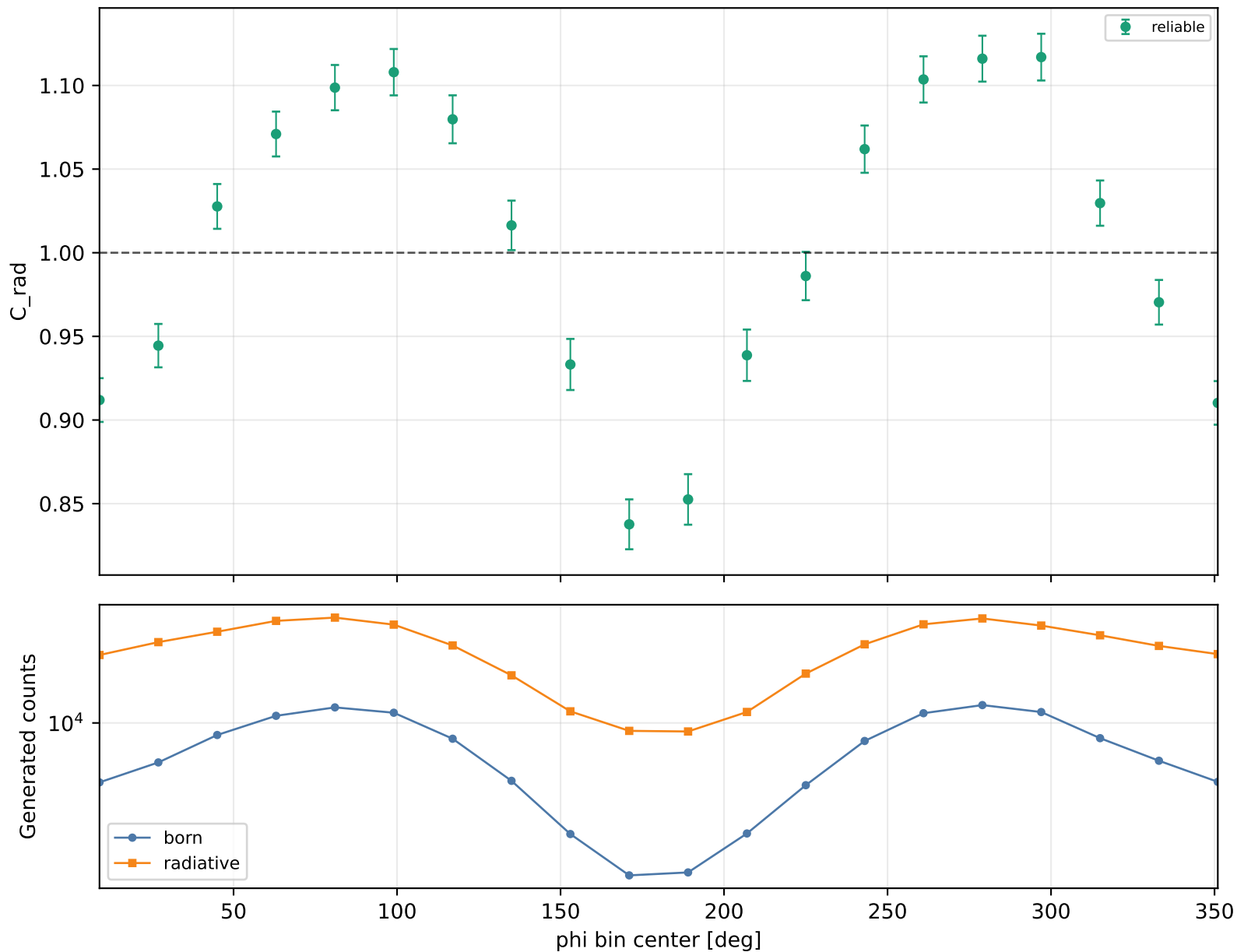
Radiative correction vs phi Q2 1-1.5, xB 0.1-0.15, -t 0.3-0.4
