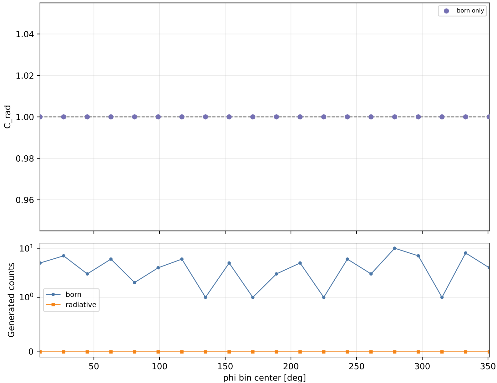
Radiative correction vs phi Q2 1-1.5, xB 0.48-0.58, -t 0.2-0.3
