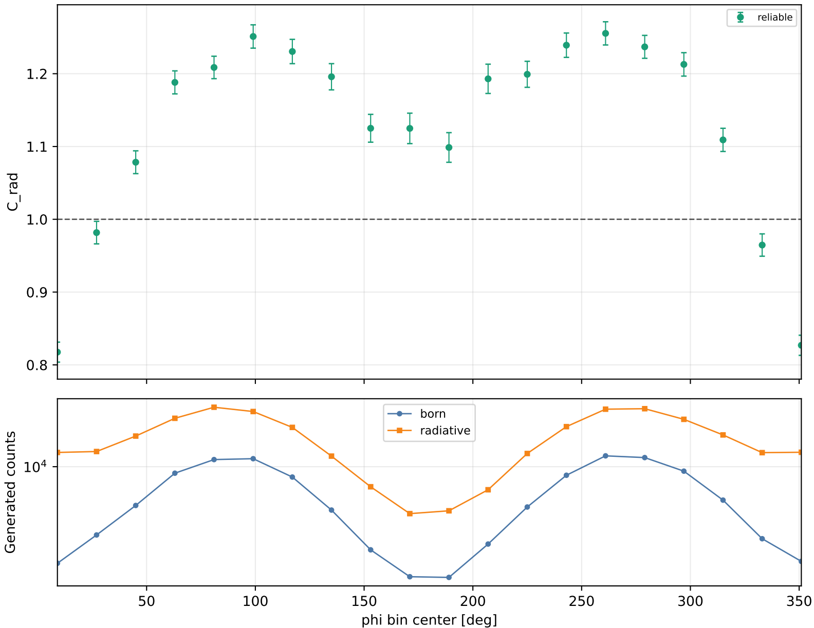
Radiative correction vs phi Q2 2.5-3, xB 0.38-0.48, -t 1-1.5
