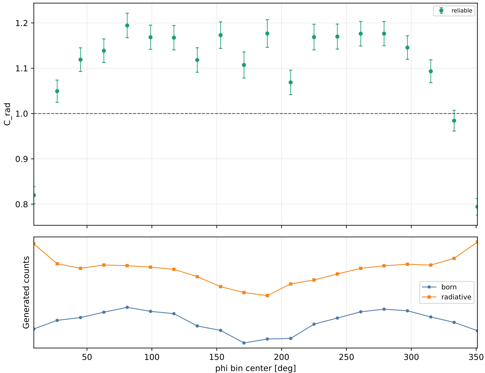
Radiative correction vs phi Q2 2-2.5, xB 0.25-0.3, -t 1-1.5
