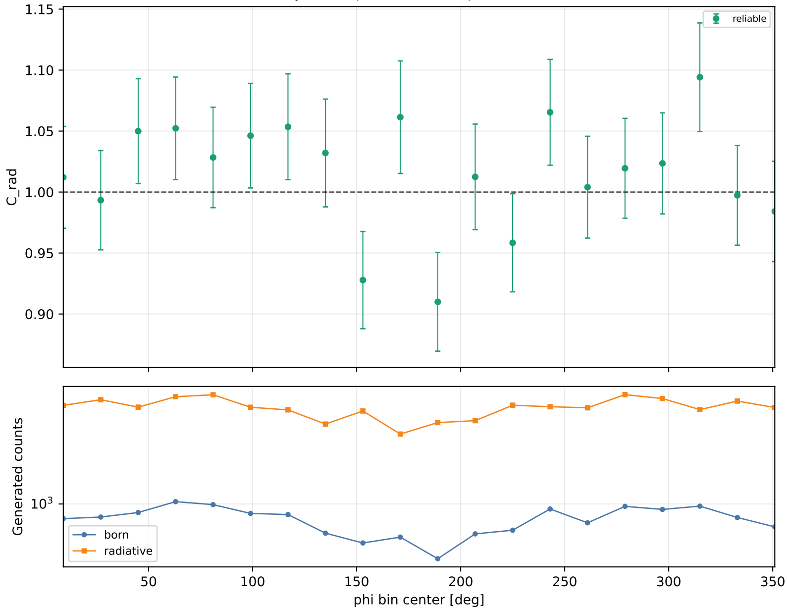
Radiative correction vs phi Q2 4-4.6, xB 0.38-0.48, -t 0.4-0.6
