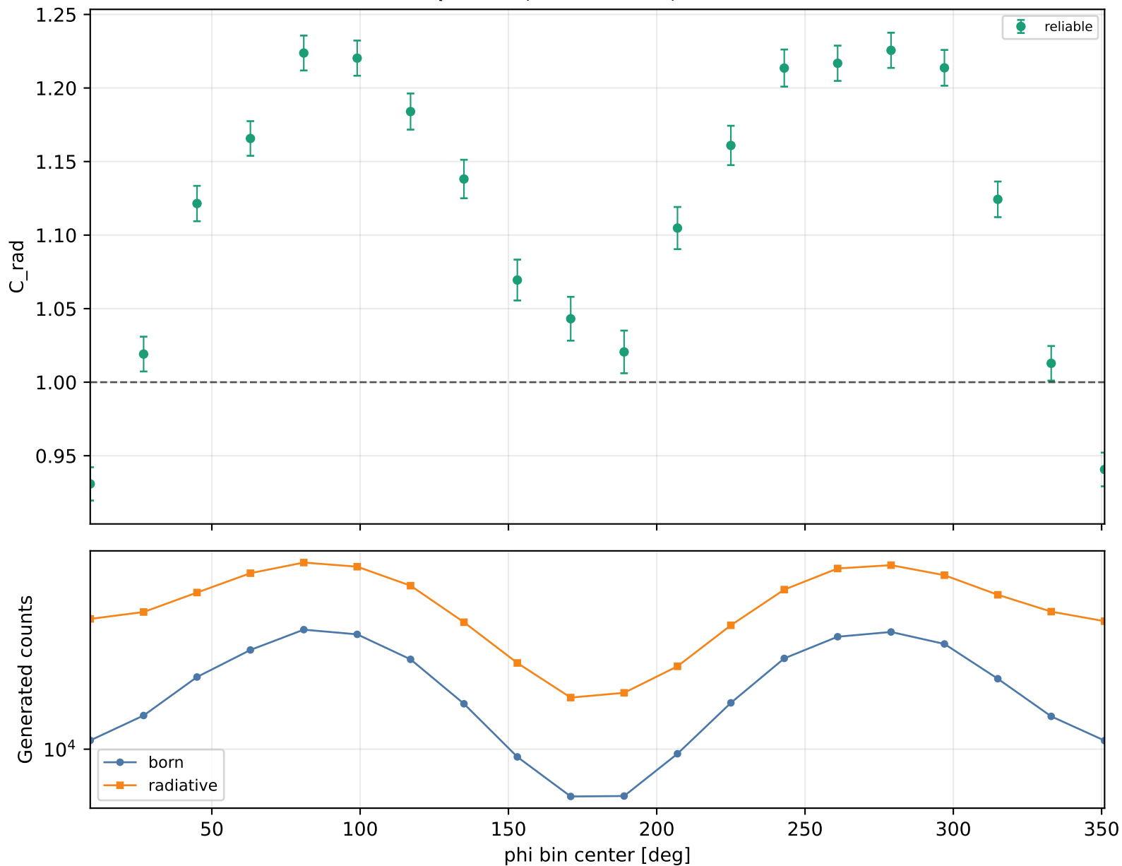
Radiative correction vs phi Q2 2-2.5, xB 0.3-0.38, -t 0.6-1
