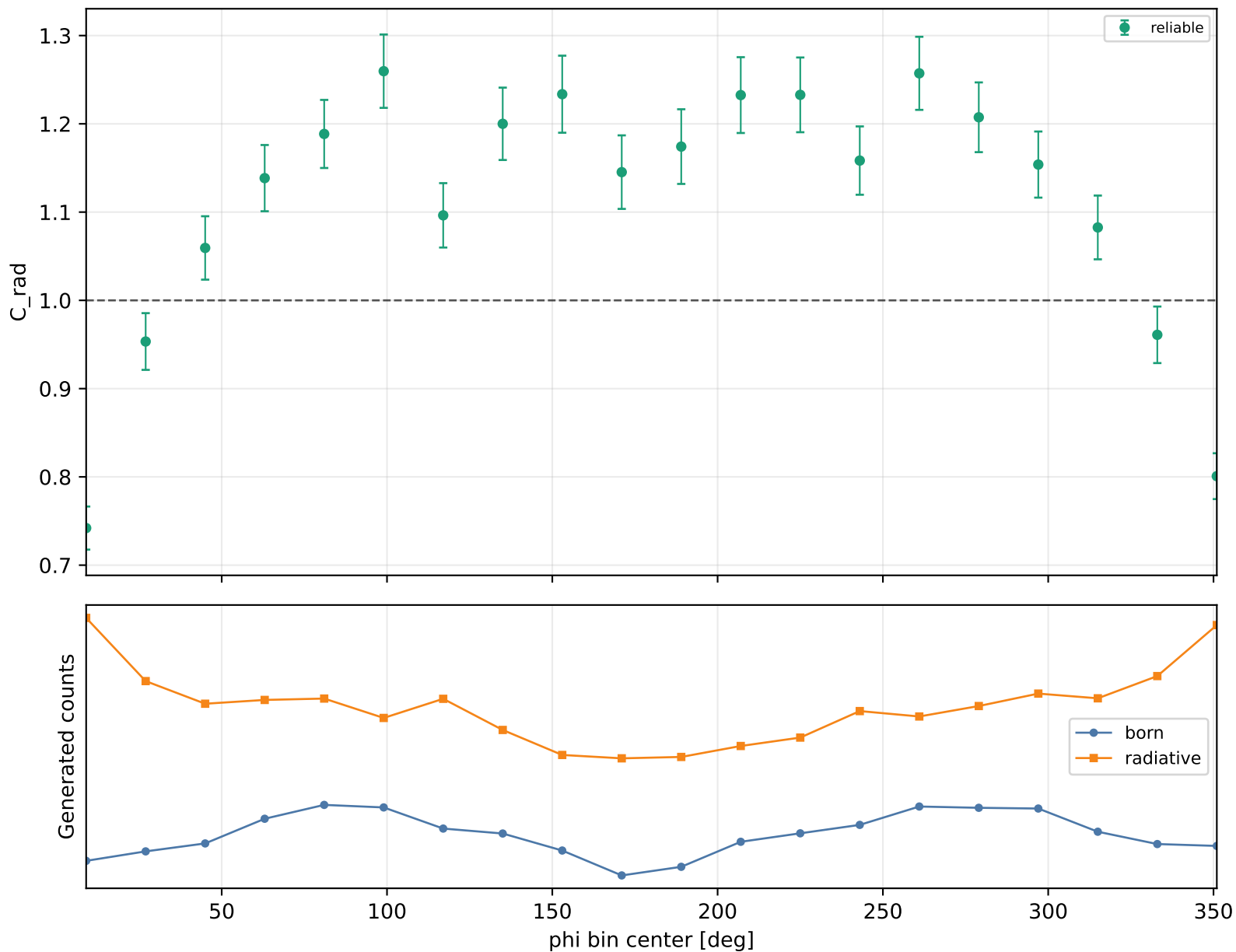
Radiative correction vs phi Q2 2.5-3, xB 0.3-0.38, -t 1.5-2
