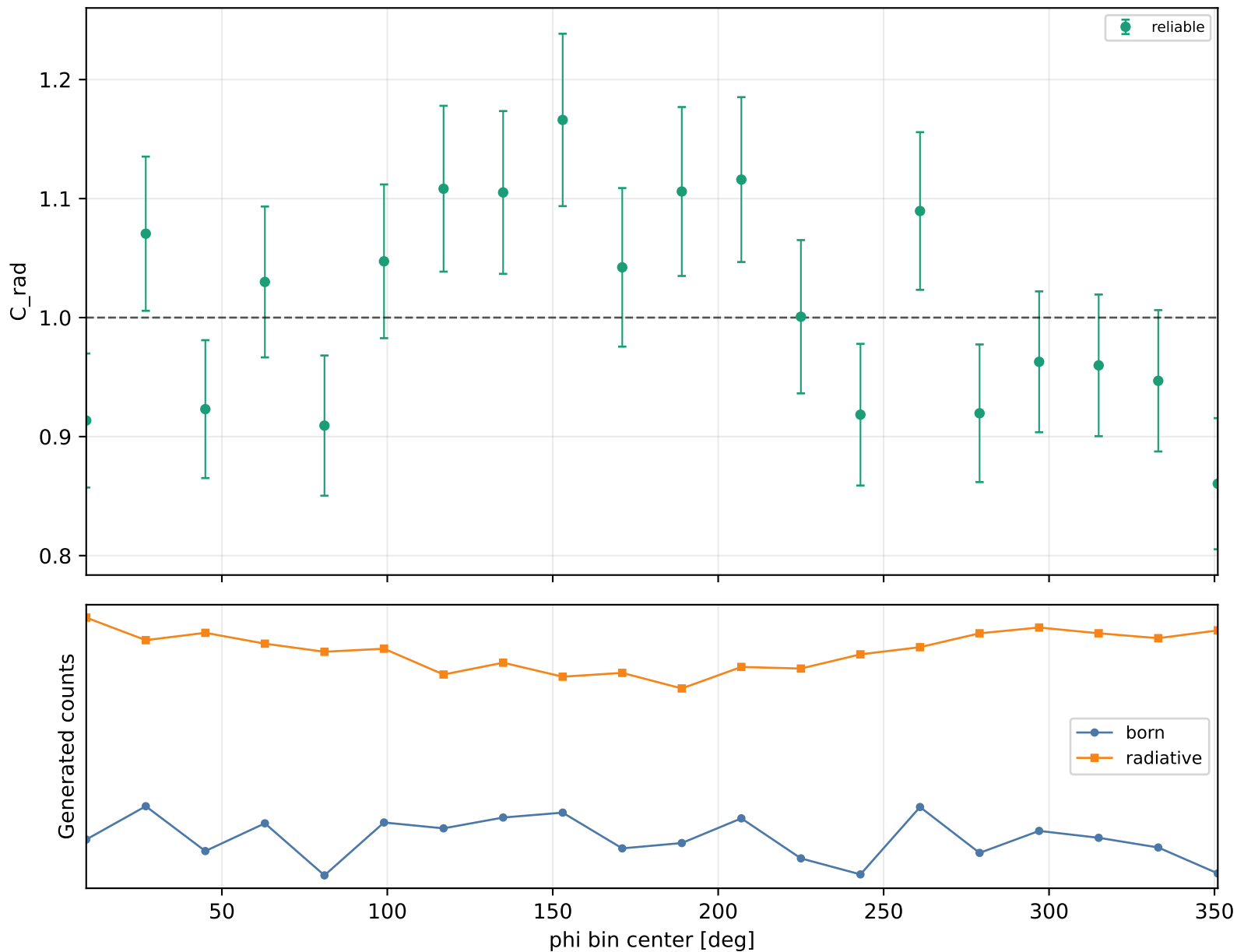
Radiative correction vs phi Q2 2.5-3, xB 0.25-0.3, -t 1.5-2
