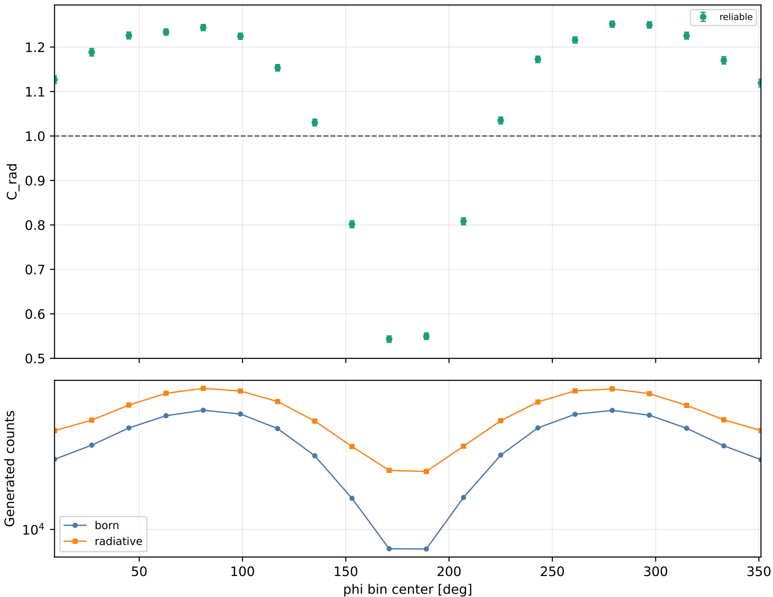
Radiative correction vs phi Q2 1-1.5, xB 0.2-0.25, -t 0.2-0.3
