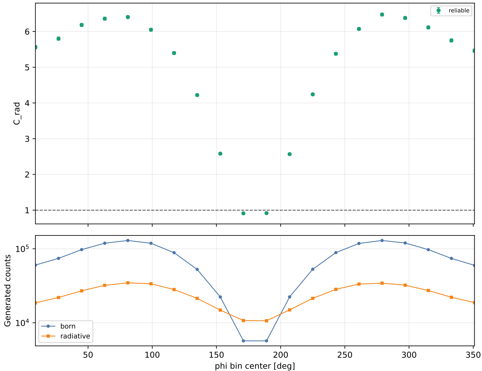
Radiative correction vs phi Q2 1-1.5, xB 0.3-0.38, -t 0.2-0.3
