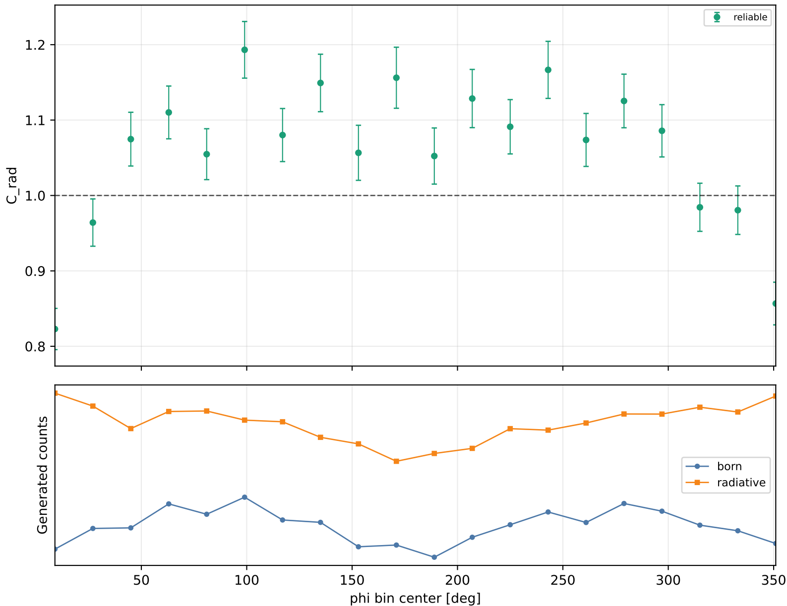
Radiative correction vs phi Q2 3-3.5, xB 0.3-0.38, -t 1-1.5
