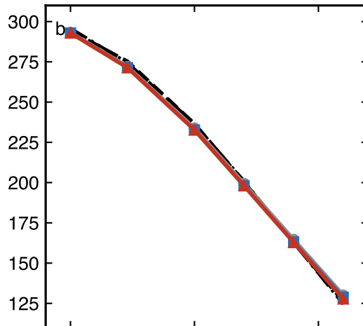
downwelling stellar at surface (Sun)
