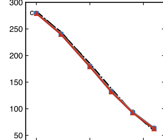
downwelling stellar at surface (3400 K)
