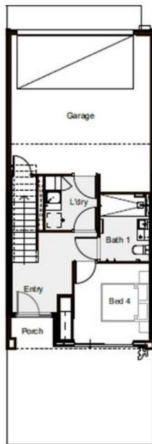
Ground / 1st floor
