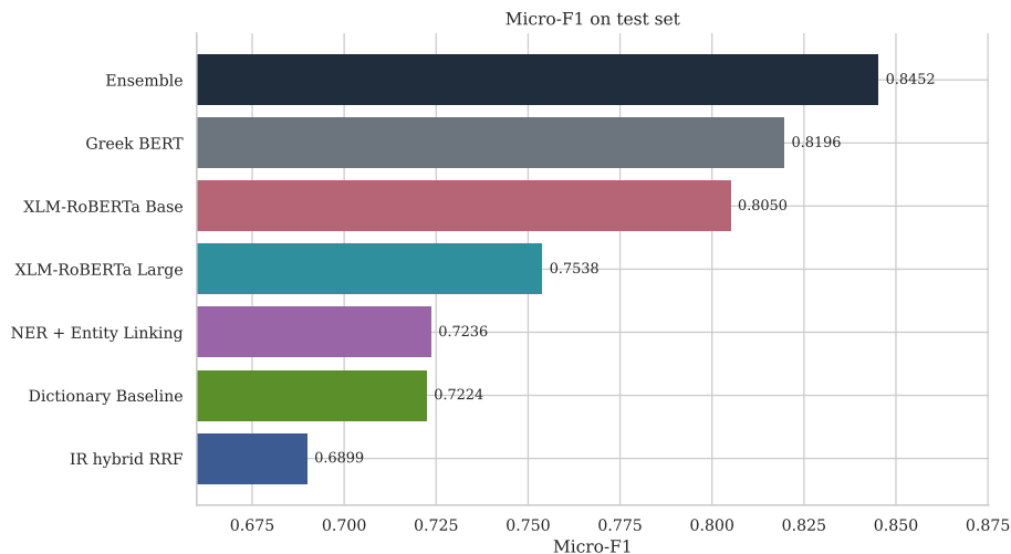
Fig. 2. Standalone micro-F1 on our test set for each system component.
