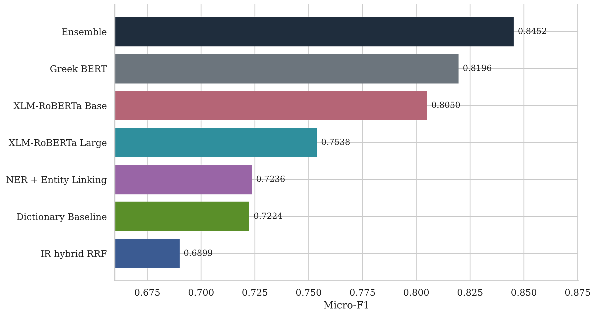
Micro-F1 on test set
