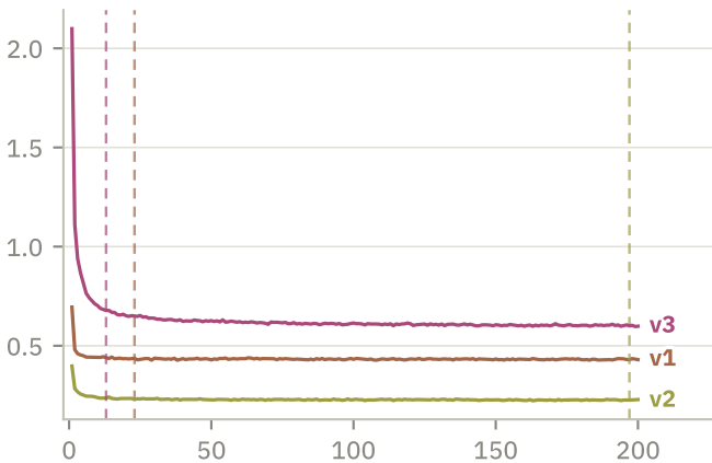
Train loss
