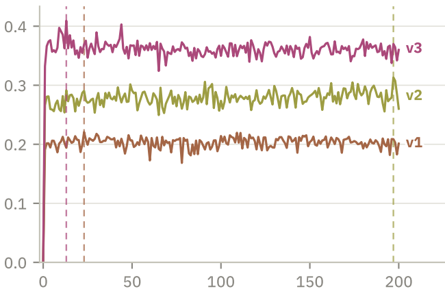
MRR
