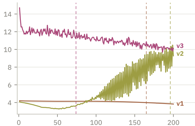
Train loss
