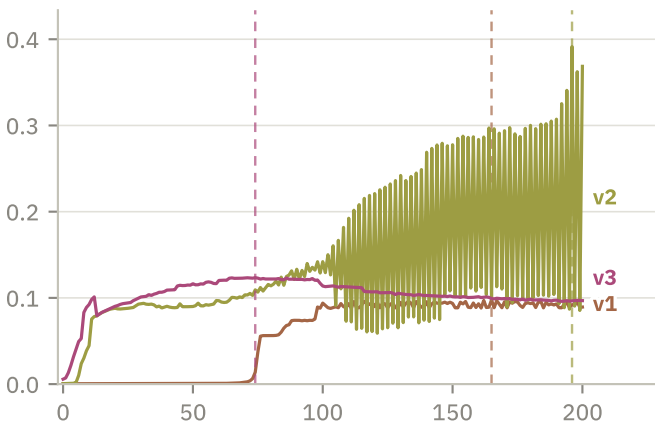
MRR
