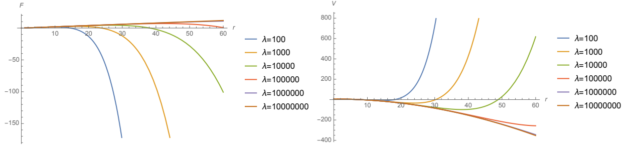
Figure 6: Finite temperature force (left) and potential (right) with respect to the radial coordinate r (or equivalently temperature T ). We observe a similar behaviour as in figure 5. We have set for the horizon r_0 = 1 and g_{YM} = 1 .
