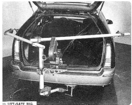
11. LIFT-GATE RIG.
