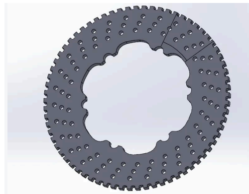
Rear rotor CAD — slotting and vane pattern set by thermal mass and inertia.
