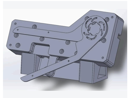
V7 — the final fixture, with the support that braces the inner plates when the wrench is fully open.
