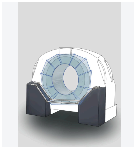
Liner architecture: gantry frustum, faces and rear collection.
