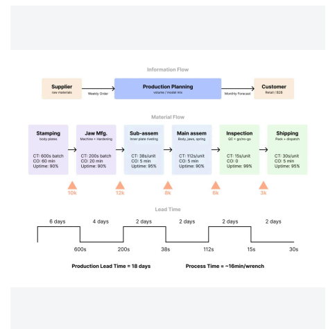
Value stream map — 18-day lead time against ~16 min of process time.
