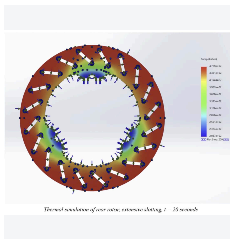
Thermal simulation of the rear rotor at t = 20 s of braking.
