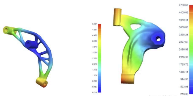
Figures 5a, 5b: Initial Topology Optimization on Design Spaces for Left and Right Calipers
