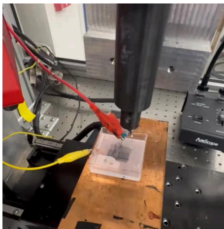
Near-field electrospinning at 10 kV, AIM Lab
