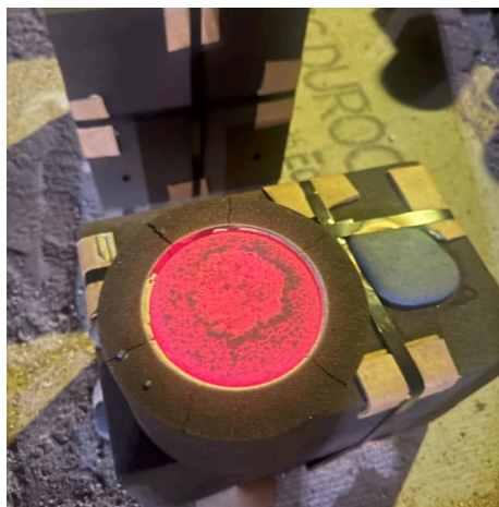
Sand mold during an iron pour
