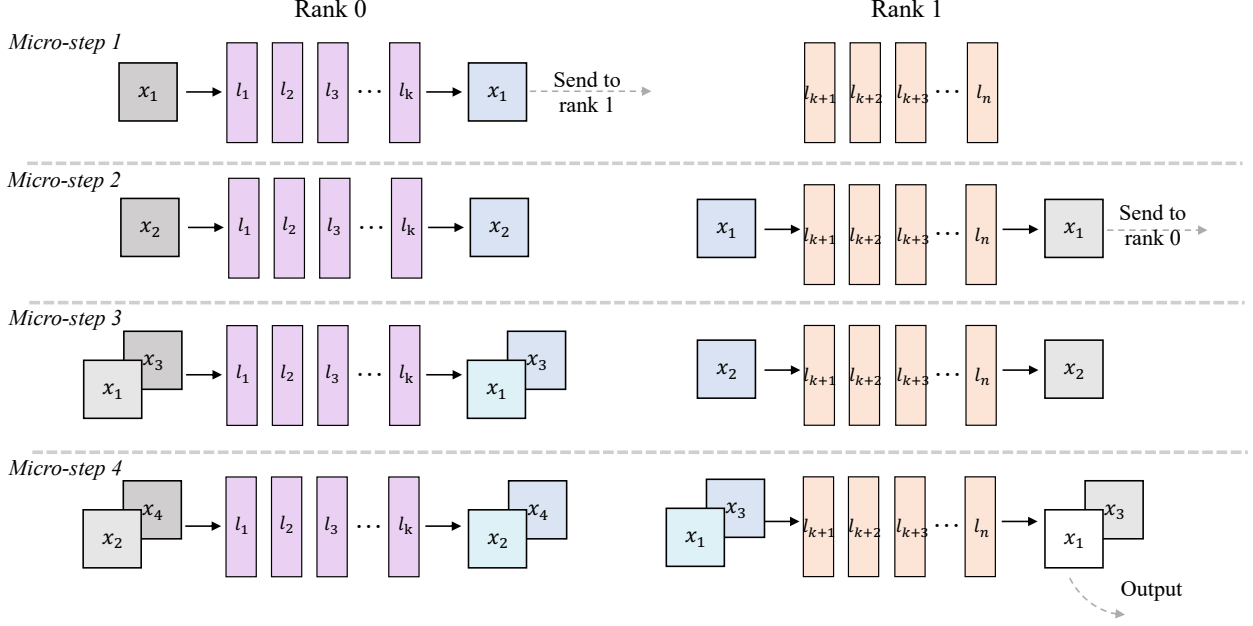
Figure 7 The detailed design of our Pipeline-parallel Stream-Batch architecture. The DiT blocks are distributed across multiple devices for pipeline parallelism, while the Stream-Batch strategy is applied within each stage. Different colors denote distinct latent streams, illustrating the communication structure, and the depth indicates the corresponding noise levels. Our implementation guarantees the generation of a clean latent at every micro-step during inference.
