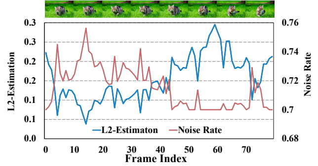
Figure 8 Example of motion estimation and dynamic noise rate. The curves indicate the L2-estimation and its corresponding noise rate of the video.
