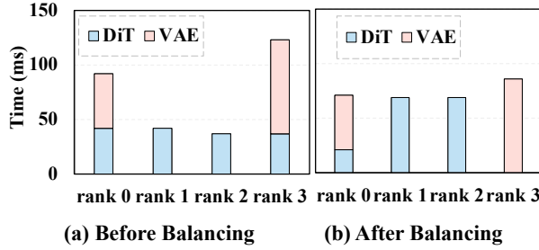
Figure 13 Time consumption before and after the balancing schedule. (a) Time consumption among various devices before balancing. (b) Time consumption after balancing. We present the 4-step denoising results on NVLink-connected H100 GPUs.
