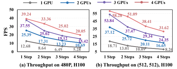
Figure 11 The throughput results of the 14B model on H100 GPUs (communicate through NVLink) among different denoising steps and various resolutions.
