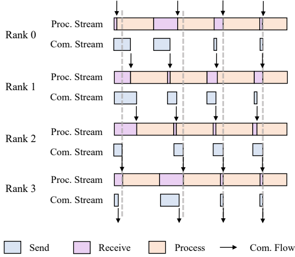
Figure 16 Execution timeline of the Pipeline-orchestration architecture.
