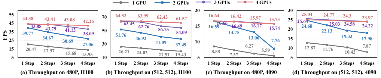
Figure 9 The throughput results of the 1.3B model on H100 GPUs (with NVLink) and 4090 GPUs (with PCIe) among different denoising steps and various resolutions. We report the result without batching on 4090 because of the memory limitation.
