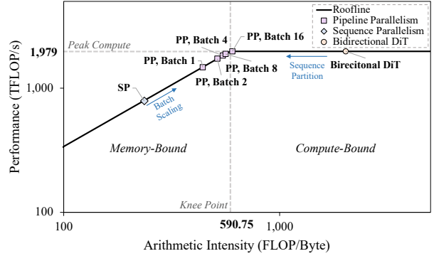
Figure 4 Roofline analysis of sequence parallelism and our pipeline orchestration. We compare the Sequence Parallelism and Pipeline Parallelism under varying batch sizes in the causal DiT, compared with the bidirectional DiT. The results demonstrate that our approach operates near the knee point of the roofline, effectively avoiding compute under-utilization as seen in the bidirectional DiT and memory bandwidth limitations in Sequence Parallelism. The model is profiled on an NVIDIA H100 SXM GPU with a peak performance of 1,979 TFLOP/s and a knee point at an arithmetic intensity (AI) of 590.75 FLOP/Byte. The token length is 1,536 (a 4-frame chunk at 480P resolution).
