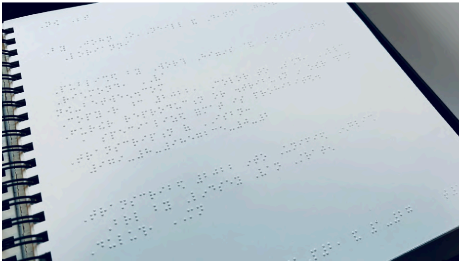
Figure 7. The Braille was printed on Braille paper instead of another material because it was the best option for ensuring that the dots met the standard height of 0.48 millimeters, providing the best reading experience for Braille readers. © John O'Neill and Deanna Geneva Lorianni of Color to Sound, LLC
