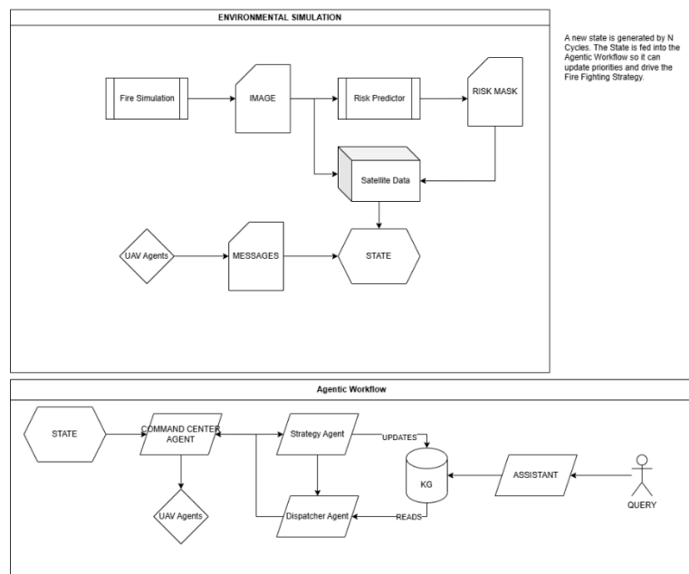
Figure 6 Agentic Workflow
