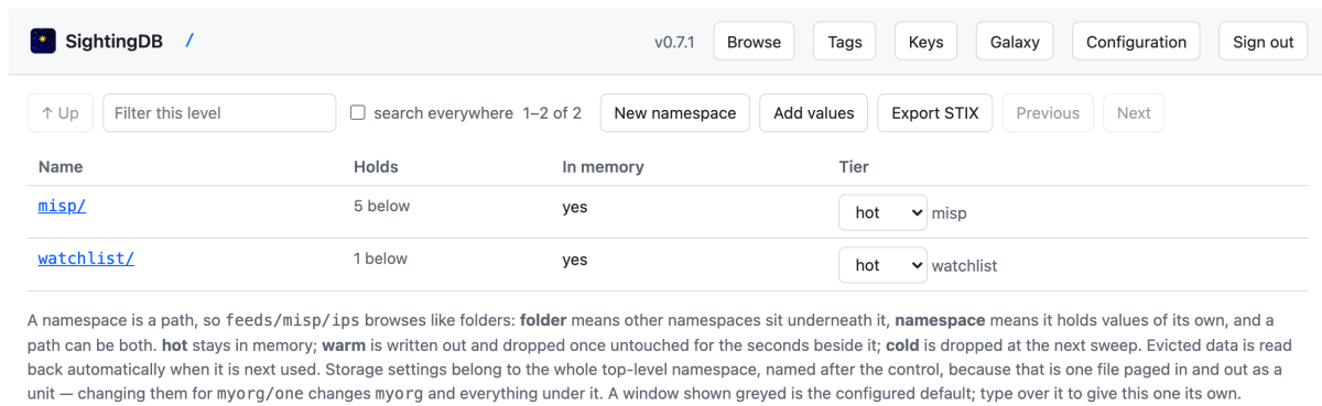
Figure 2.1: The namespace tree. A path is a folder and a namespace at once.
