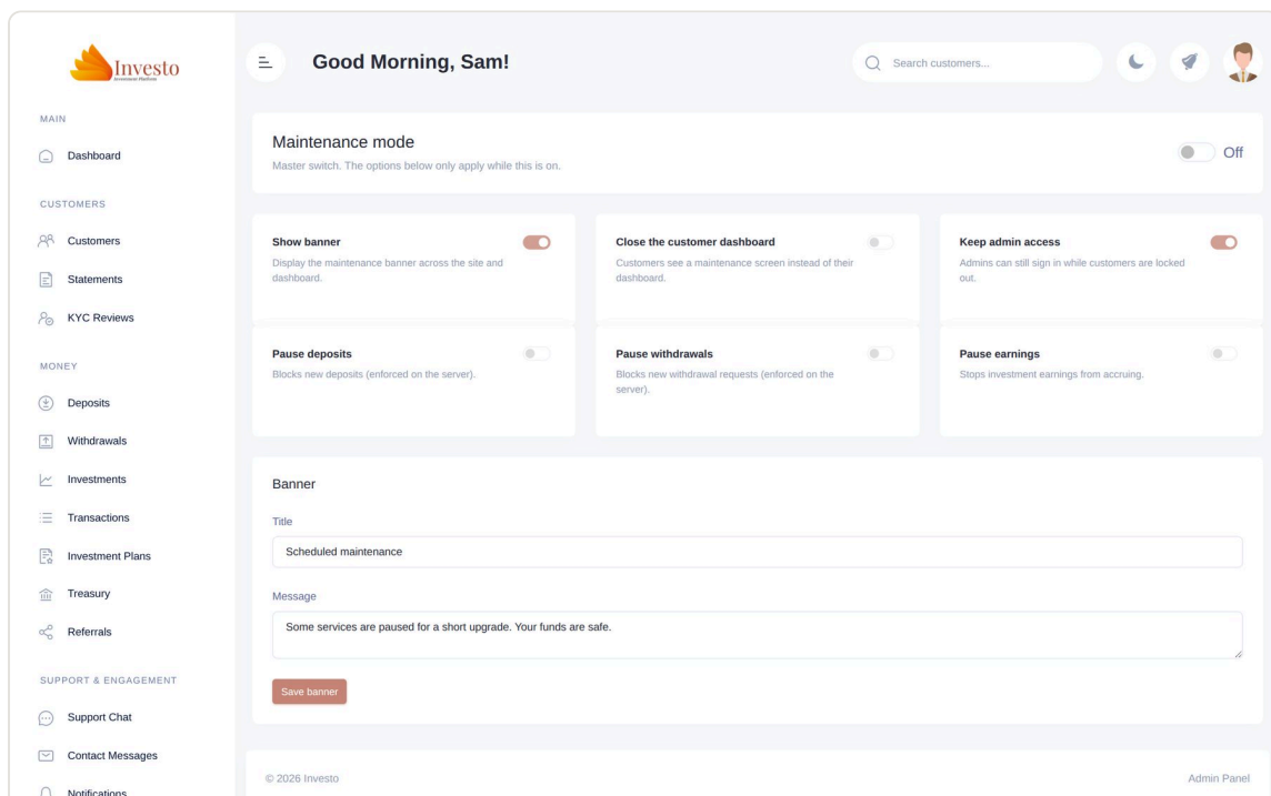
Figure 75. Maintenance.
