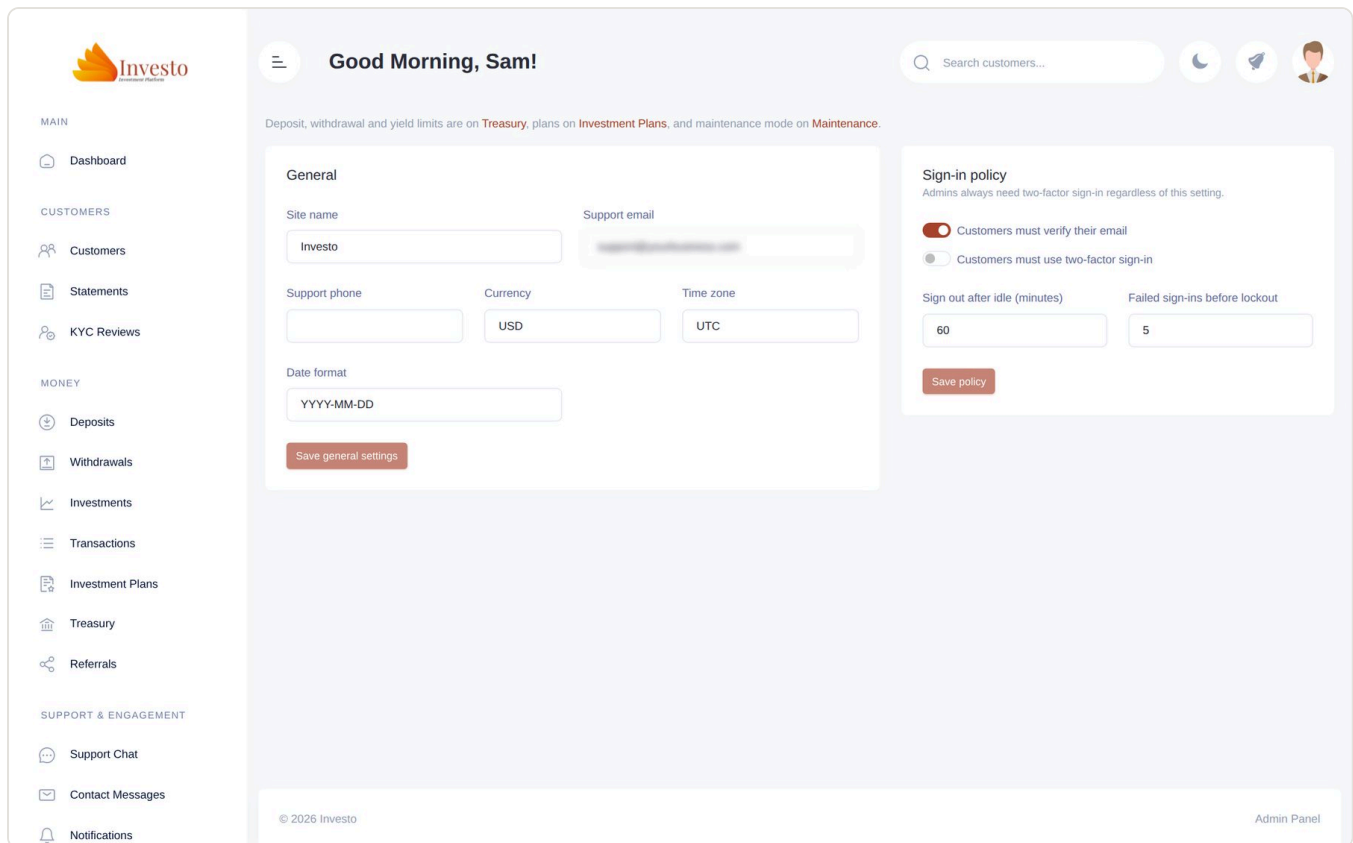
Figure 74. Settings.
