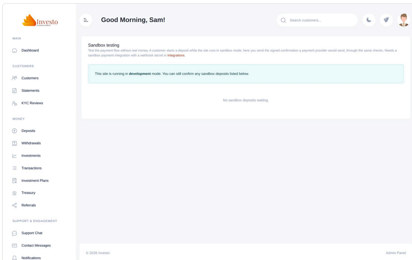
Figure 76. Sandbox Testing.
