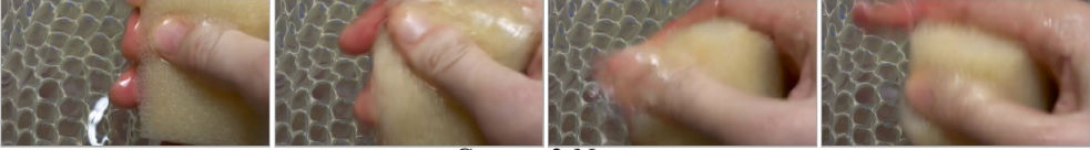
Cosmos3-Nano
