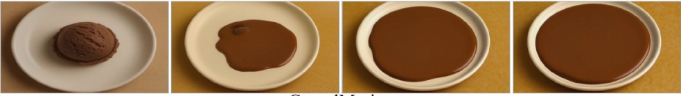
CausalMotion
