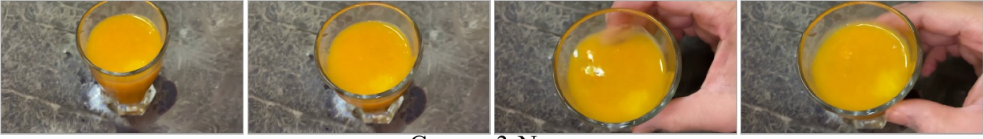
Cosmos3-Nano
