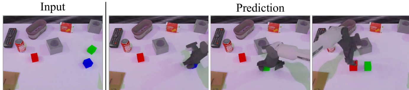
Wan2.2
