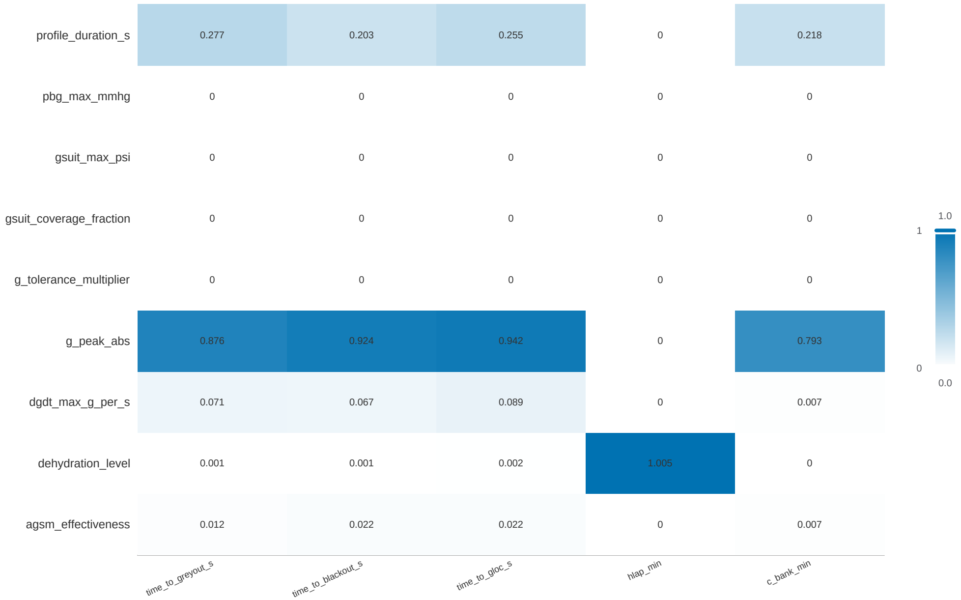
Total-Order Sobol Indices (ST)
