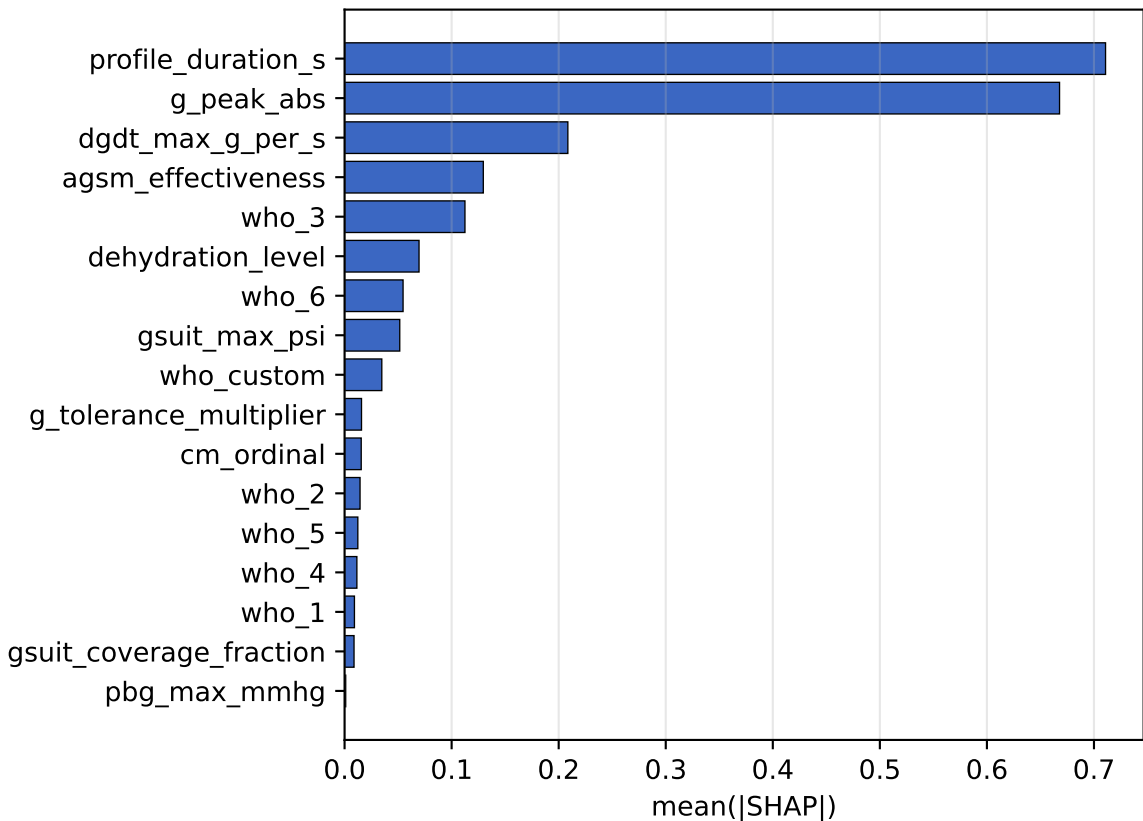
SHAP TreeExplainer | target: time_to_greyout_s (n_test = 84)
