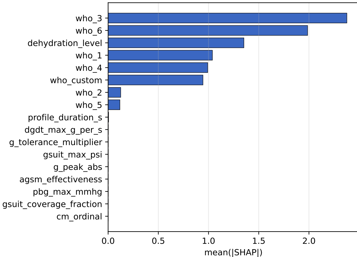
SHAP TreeExplainer | target: hlap_min (n_test = 487)
