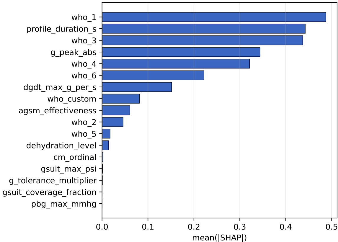
SHAP TreeExplainer | target: time_to_gloc_s (n_test = 36)
