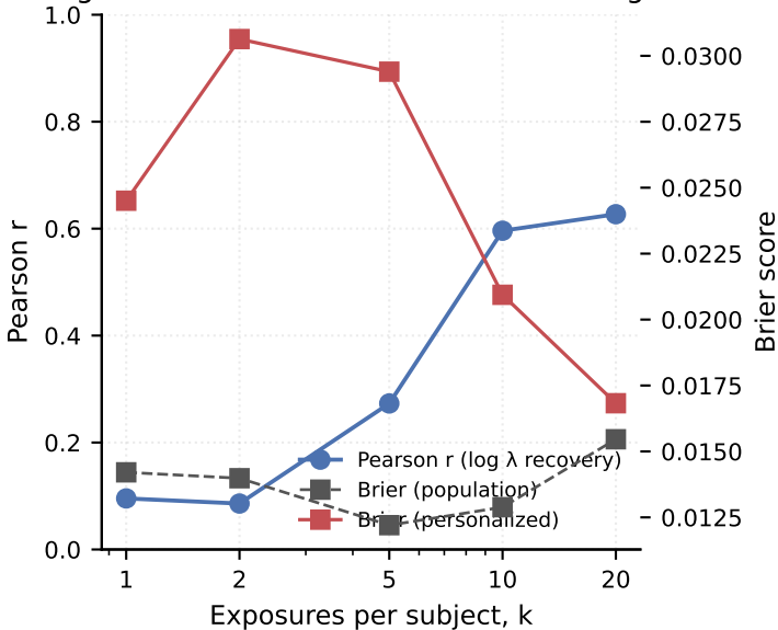
Figure 4 · Personalization information gain
