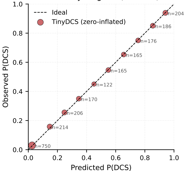
Reliability diagram (test fold)
