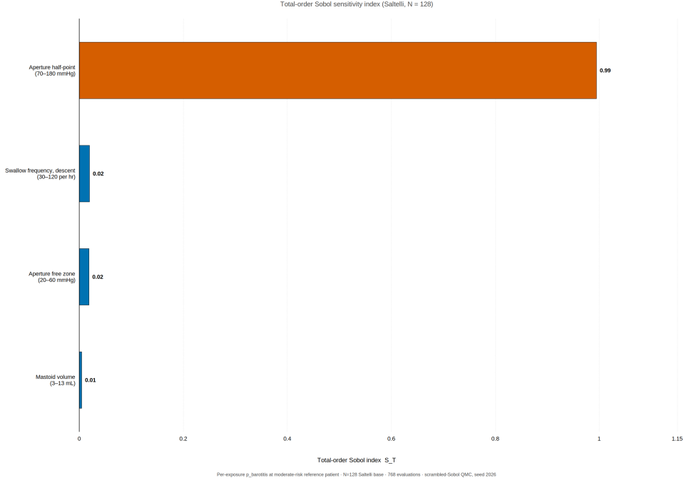
Figure 2: Saltelli-Sobol total-order sensitivity index over four model parameters evaluated at a moderate-risk reference patient ( N = 128 Saltelli base samples; 768 model evaluations; scrambled-Sobol QMC sequence, seed 2026). The aperture half-point dominates ( S_T \approx 0.99 ), approximately fifty-fold above descent-phase swallow frequency ( S_T = 0.020 ), aperture free-zone threshold ( S_T = 0.019 ), and mastoid volume ( S_T = 0.005 ). The three secondary parameters are indistinguishable from each other within Monte-Carlo noise
