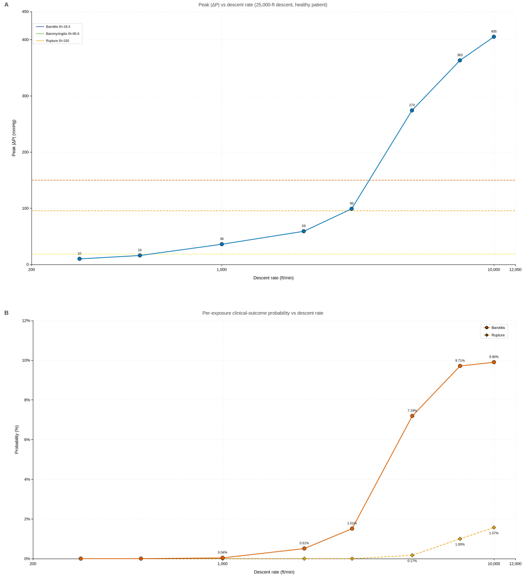
Figure 1: Descent-rate sensitivity for a healthy patient on a 25,000-ft descent. Peak |\Delta P| (top panel) grows monotonically with descent rate, approaching \sim 400 mmHg at 10,000 \text{ ft}\cdot\text{min}^{-1} . Per-exposure barotitis probability (bottom panel) increases across the full 500\text{--}10,000 \text{ ft}\cdot\text{min}^{-1} range because the dose-time integral does not saturate as sharply as the peak
