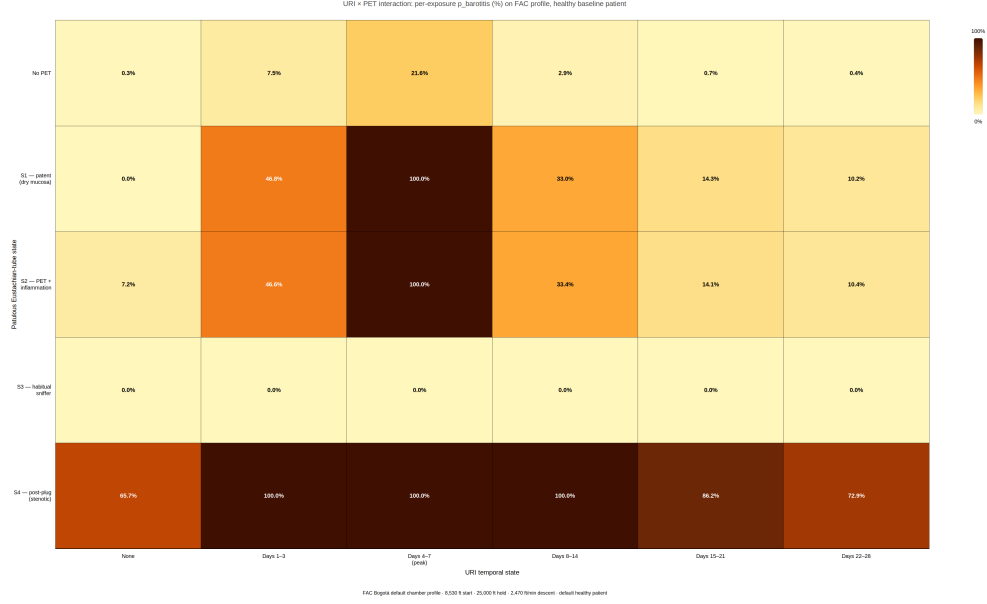
Figure 4: Joint dependence of per-exposure barotitis probability on Patulous Eustachian-tube state (5 levels: No PET, S1 baseline patent and dry mucosa, S2 PET with inflammation, S3 habitual sniffer, S4 post-Kobayashi plug or stenotic-equivalent) and upper-respiratory-infection temporal state (6 levels: none, days 1–3, 4–7, 8–14, 15–21, 22–28). Each cell is the model output for a default healthy baseline patient on the FAC Bogot  chamber profile (8,530 ft start, 25,000 ft hold, 2,470 ft·min −1 descent), varying only the URI and PET states; values were computed by barotrauma.v2.simulate over the full 5 × 6 grid. The peak-URI window (days 4–7) dominates each PET row. PET-S1 (rupture-protective in the original Kanick-Doyle 2005 binary treatment) is converted to high risk by URI exposure, matching the PET-with-inflammation pathophysiology in the Japan Otological Society criteria. PET-S4 saturates regardless of URI state. PET-S3 returns uniformly low risk on this profile because the negative resting-pressure bias offsets the descent-side \Delta P integral; this model behavior is profile-specific and should not be interpreted as habitual sniffing being clinically protective
