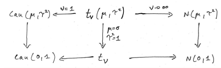
Figure 5.7: The location-scale t -distribution and its relatives.
