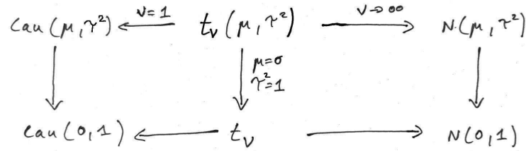
Figure 5.9: The location-scale t -distribution and its relatives.
