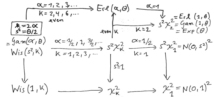
Figure 5.5: The gamma distribution and the univariate Wishart distribution and their relatives.
