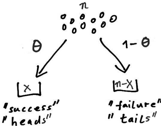
Figure 5.1: Binomial model.
