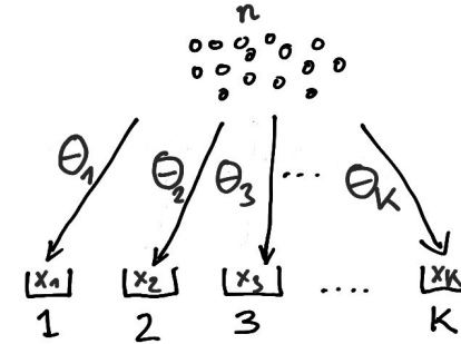
Figure 6.1: Multinomial model.
