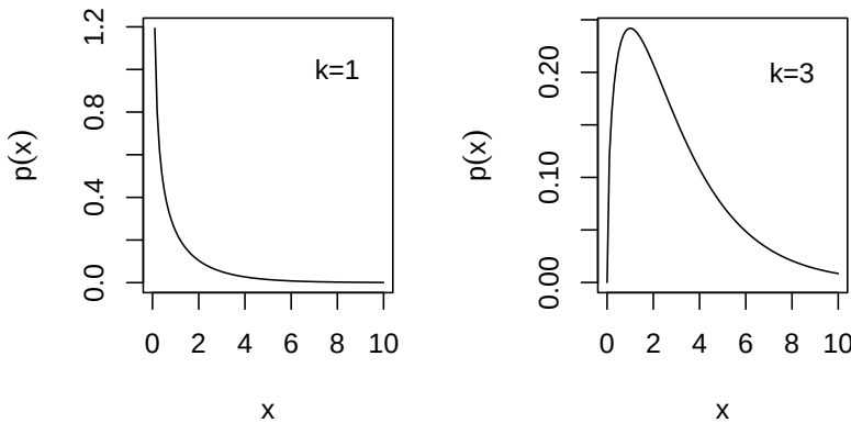
Figure 5.6: Probability density function of the chi-squared distribution.
