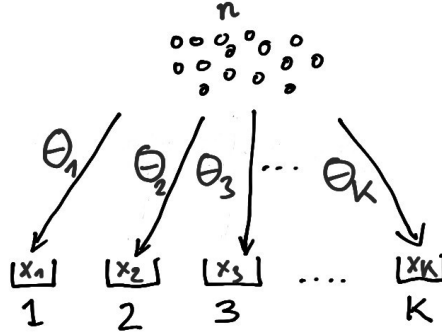
Figure 6.1: Multinomial model.
