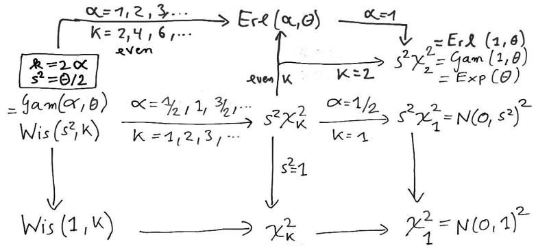
Figure 5.5: The gamma distribution and the univariate Wishart distribution and their relatives.
