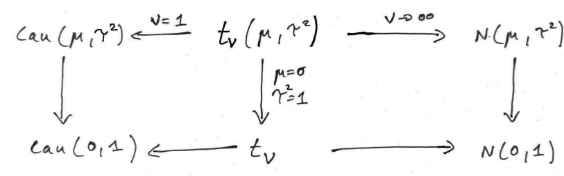
Figure 5.7: The location-scale t -distribution and its relatives.
