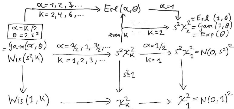
Figure 5.5: The gamma and the univariate Wishart distribution and their relatives.
