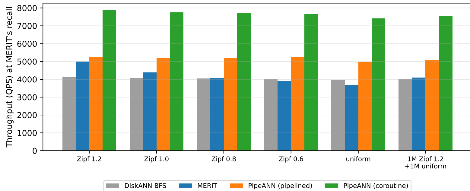
(a) Throughput, equal memory (~31 GB RSS), 20 threads
