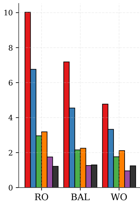
(c) Longitudes
