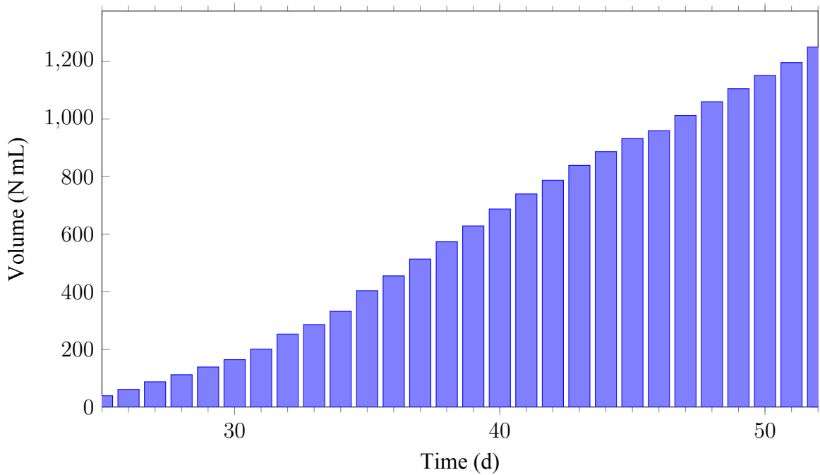
Figure 5.7: Cumulative volume of CH 4 N mL (co-digestion of food waste and crude glycerol)
