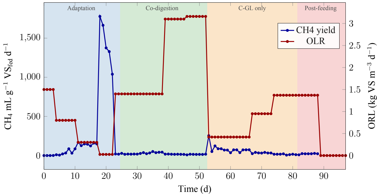
Figure 5.18: Daily yield of CH 4
