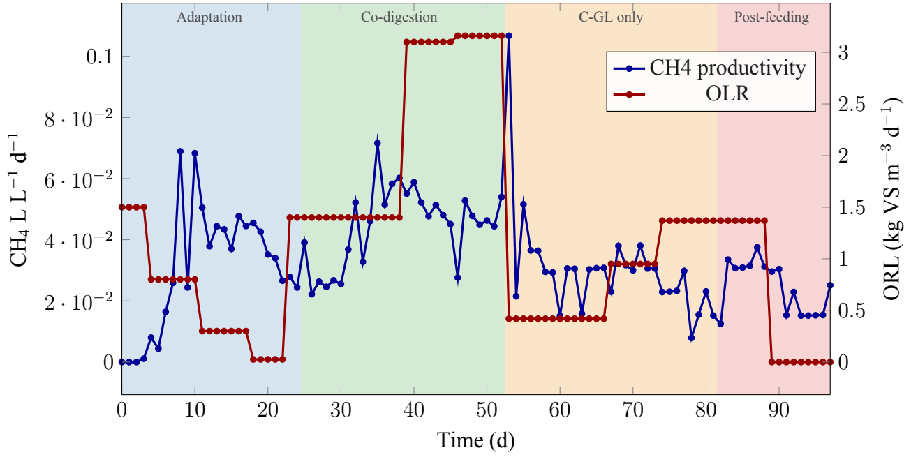
Figure 5.19: Volumetric productivity of CH 4
