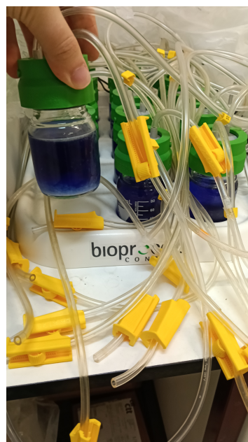
(b) AMPTS II CO 2 trap
