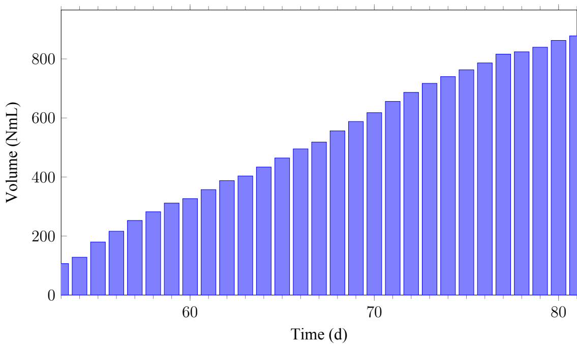
Figure 5.10: Cumulative volume of CH 4 NmL (Anaerobic digestion of C-GL)
