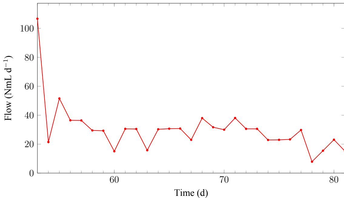
Figure 5.11: Volume flow of CH 4 NmL d -1 (Anaerobic digestion of C-GL)
